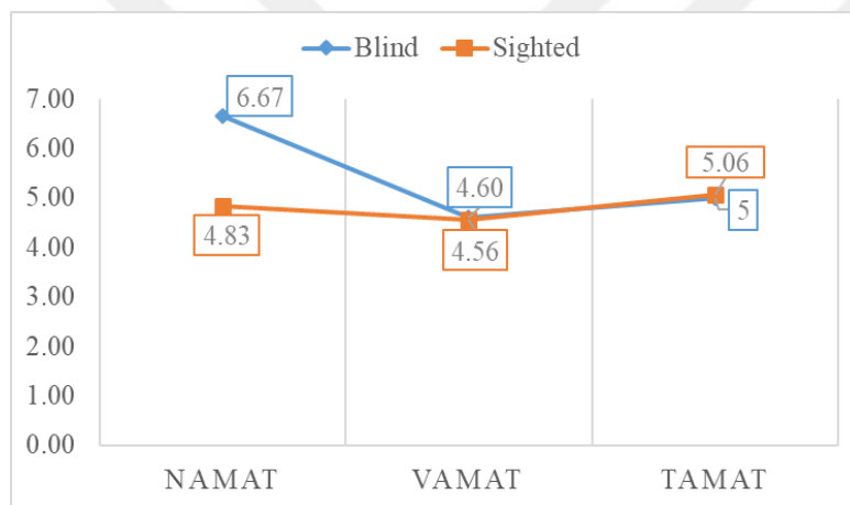
Figure 4.4 Mean scores of sighted and the blind students physics achievement on non-accommodated, verbal descriptions and tactile graphics testing accommodations conditions of Motion Achievement Test
