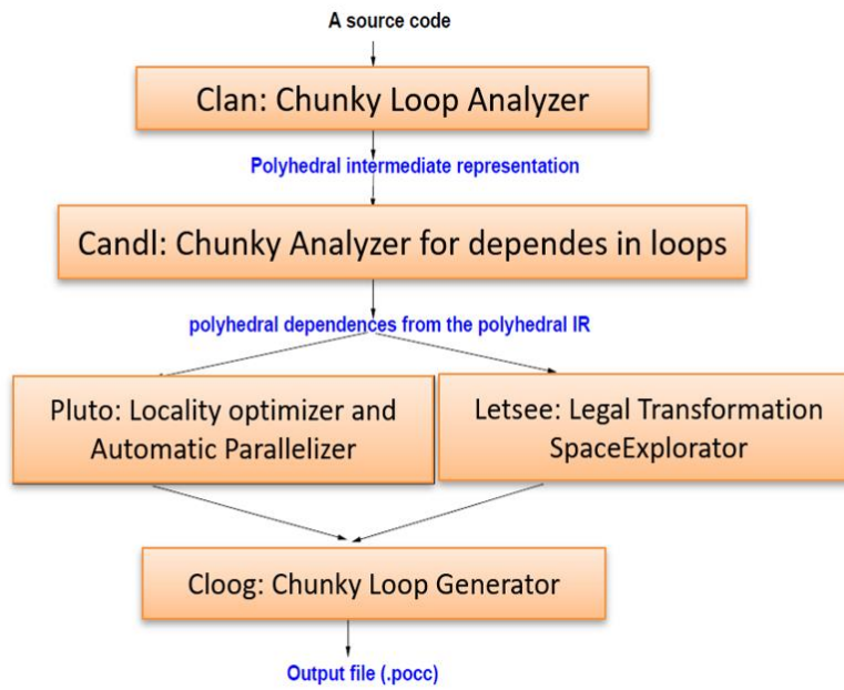
Figure 6.4. Tool Flow of POCC
