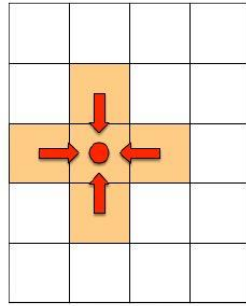
Figure 7.9. Jacobi 2D Computational Kernel
