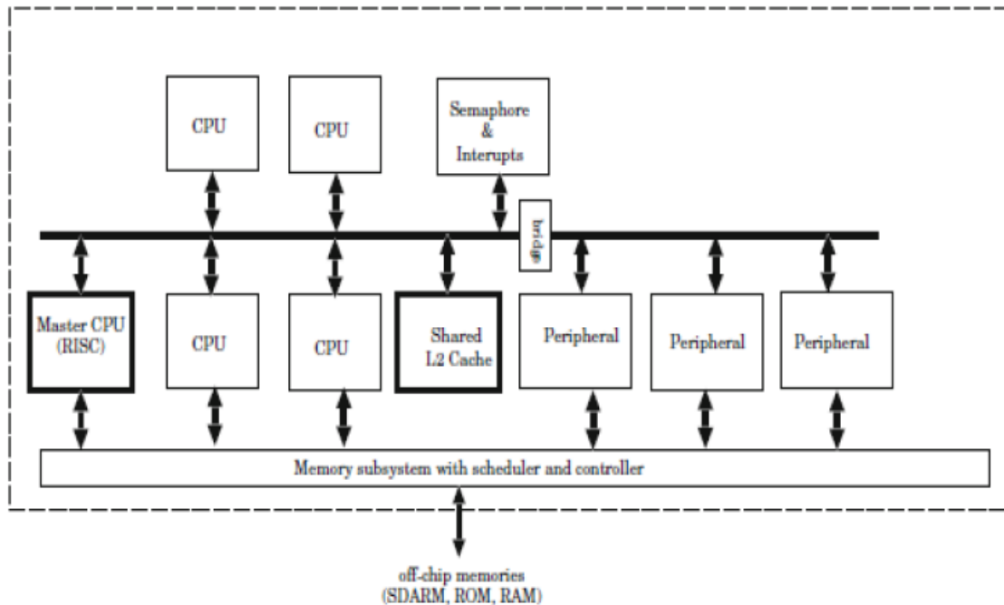
Figure 2.1. Typical Homogeneous MPSoC Architecture Example
