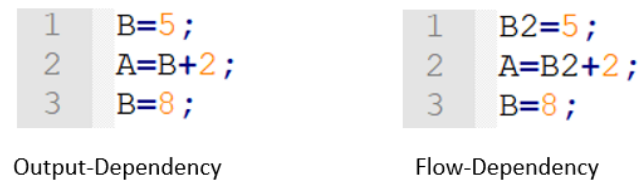
Figure 4.5. Output-Dependency vs Flow-Dependency
