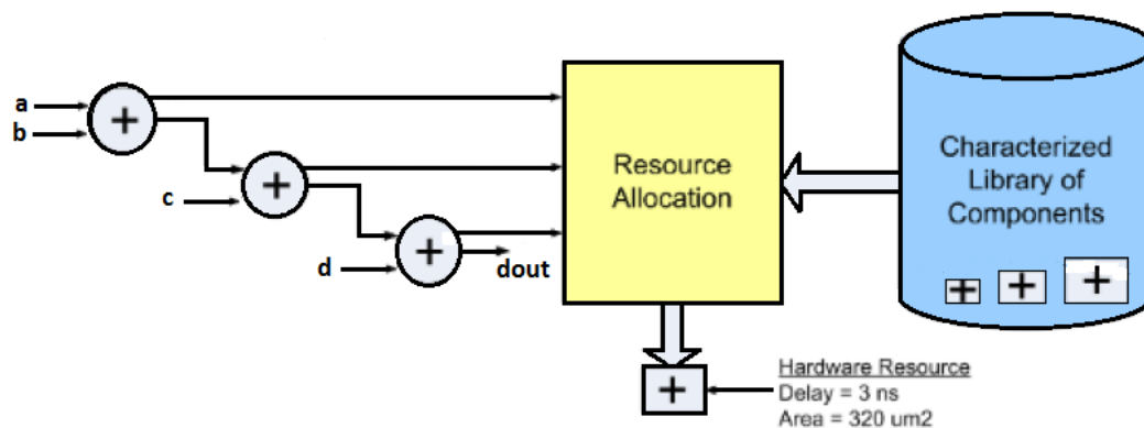
Figure 3.4. Resource Allocation of dout=a+b+c+d
