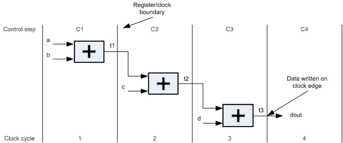
Figure 3.5. Scheduled Design of dout = a + b + c + d
