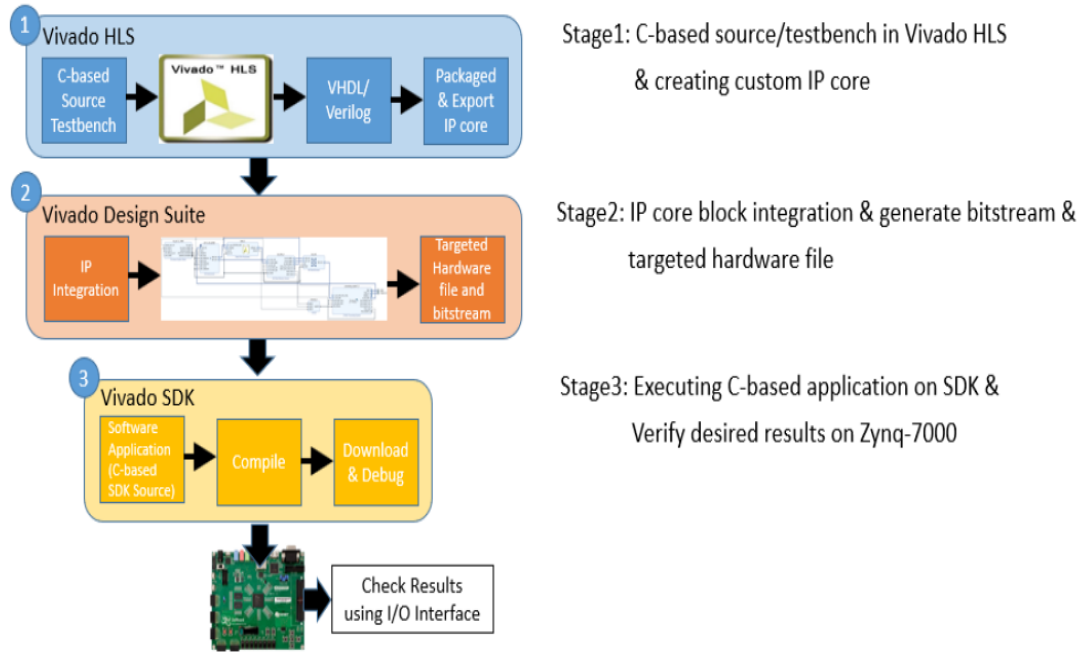
Figure 3.6. HLS design flow in Vivado
