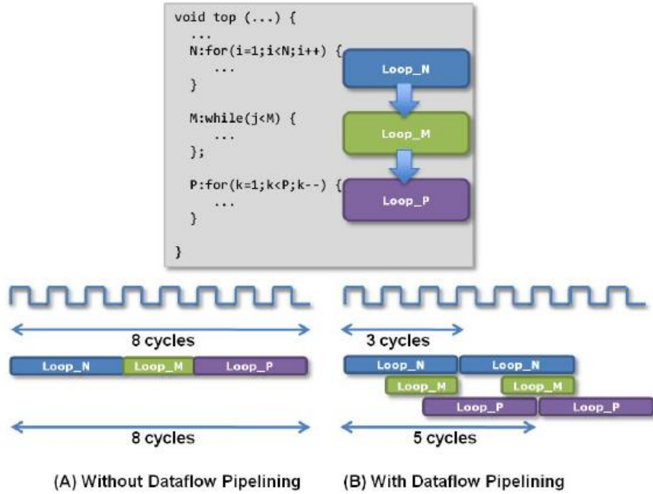
Figure 3.12. Loop Dataflow Pipelining
