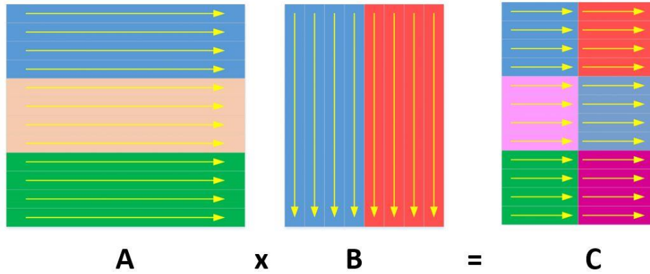
Figure 6.8. Divide and Conquer Matrix Multiplication
