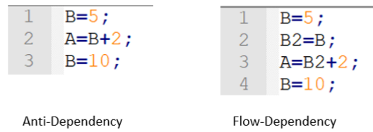
Figure 4.4. Anti-Dependency vs Flow-Dependency
