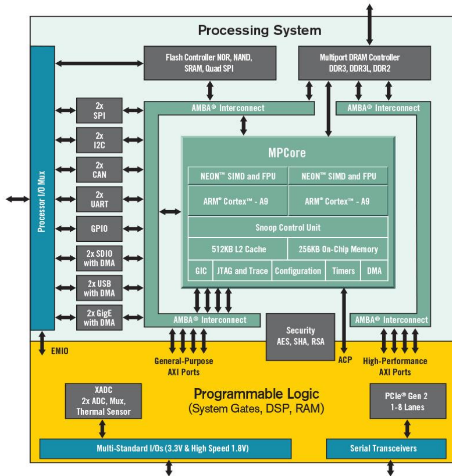
Figure 7.2. Block Diagram of Zynq-7000
