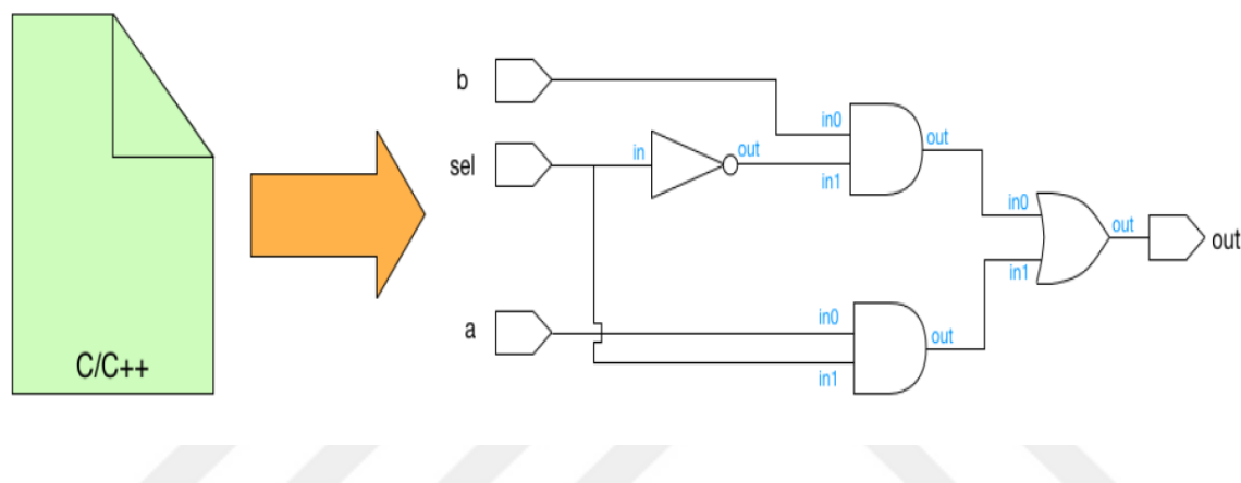
Figure 2.5. Possible Hardware Implementation of If Statement
