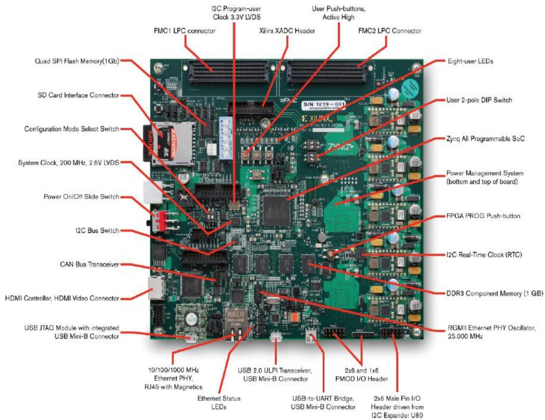
Figure 7.1. ZC-702 Evaluation Board
