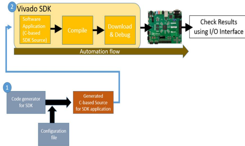
Figure 6.7. Vivado SDK Design Flow
