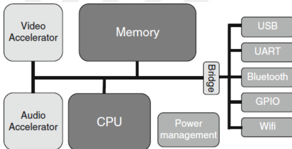
Figure 2.2. Example of Typical Heterogeneous MPSoC Architecture
