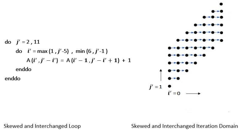
Figure 6.17. Skewed-Interchanged Code and Iteration Domain
