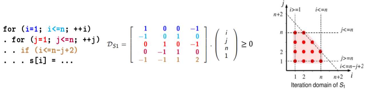
Figure 4.2. Iteration Domain Example
