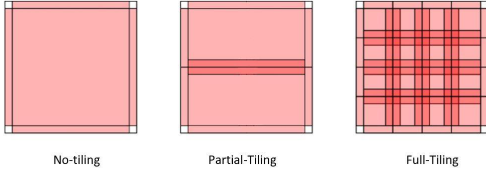
Figure 6.10. Tiling in 2D Iteration Domain
