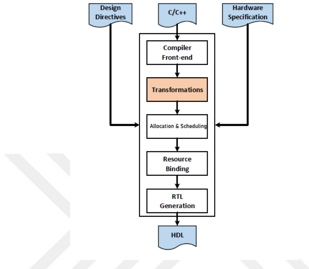
Figure 3.1. Standard HLS Tool Flow
