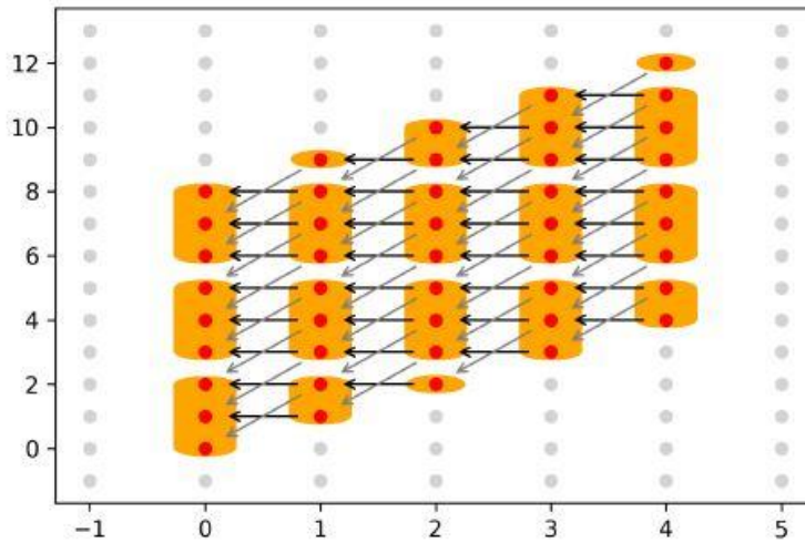
Figure 6.18. Skewed Tiling Iteration Space
