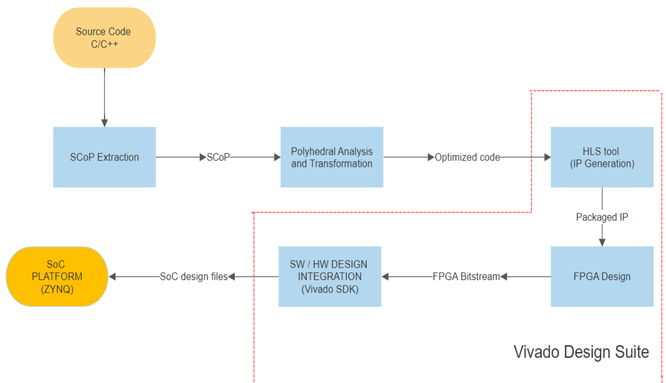
Figure 6.1. Flow Diagram of Proposed Architecture
