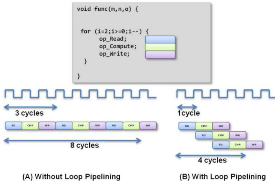
Figure 3.11. Loop Pipelining Example
