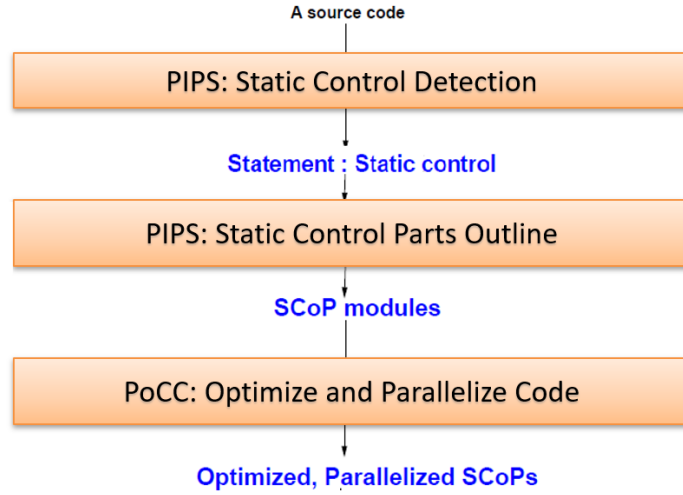
Figure 6.5. Summary of Front-End Operations of HLS
