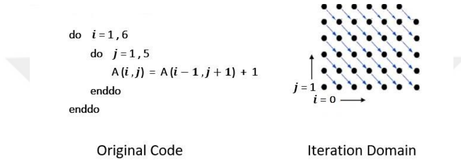
Figure 6.15. Loop Skewing Example Code
