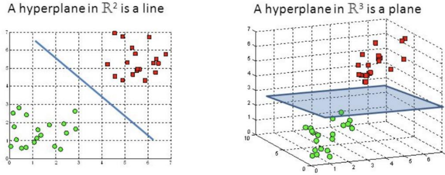
Figure 4.1. A Hyperplane in 2D and 3D Space
