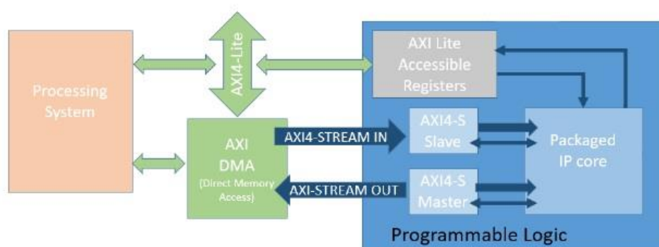
Figure 7.3. AXI Interface on Zynq SoC
