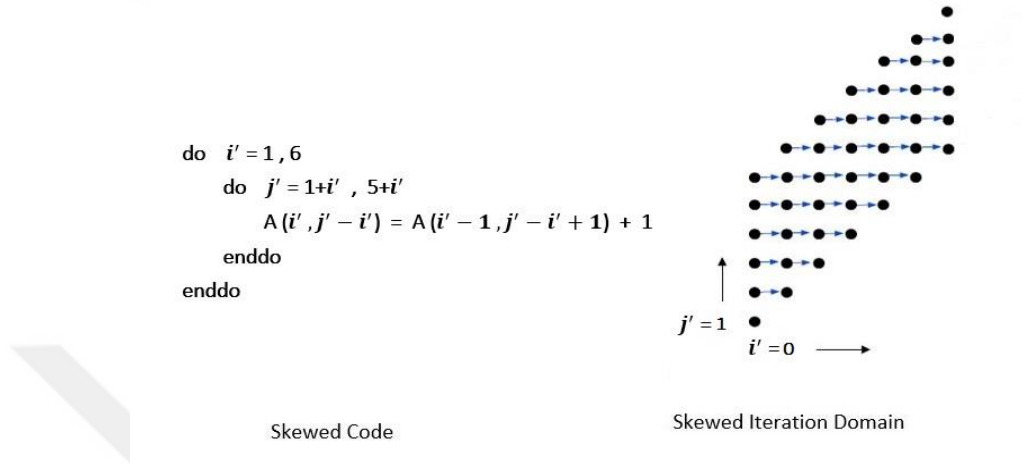
Figure 6.16. Skewed Code and Iteration Domain
