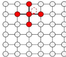
Figure 6.12. 5-Point 2D ISL
