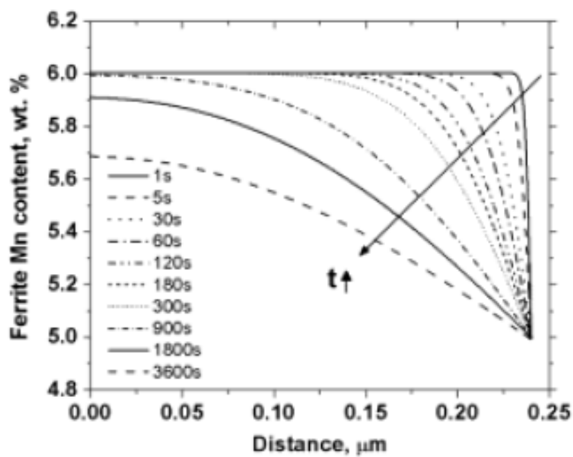
Figure 2.19. Mn profile in ferrite in a 0.1C-6Mn steel at 650°C [57].
