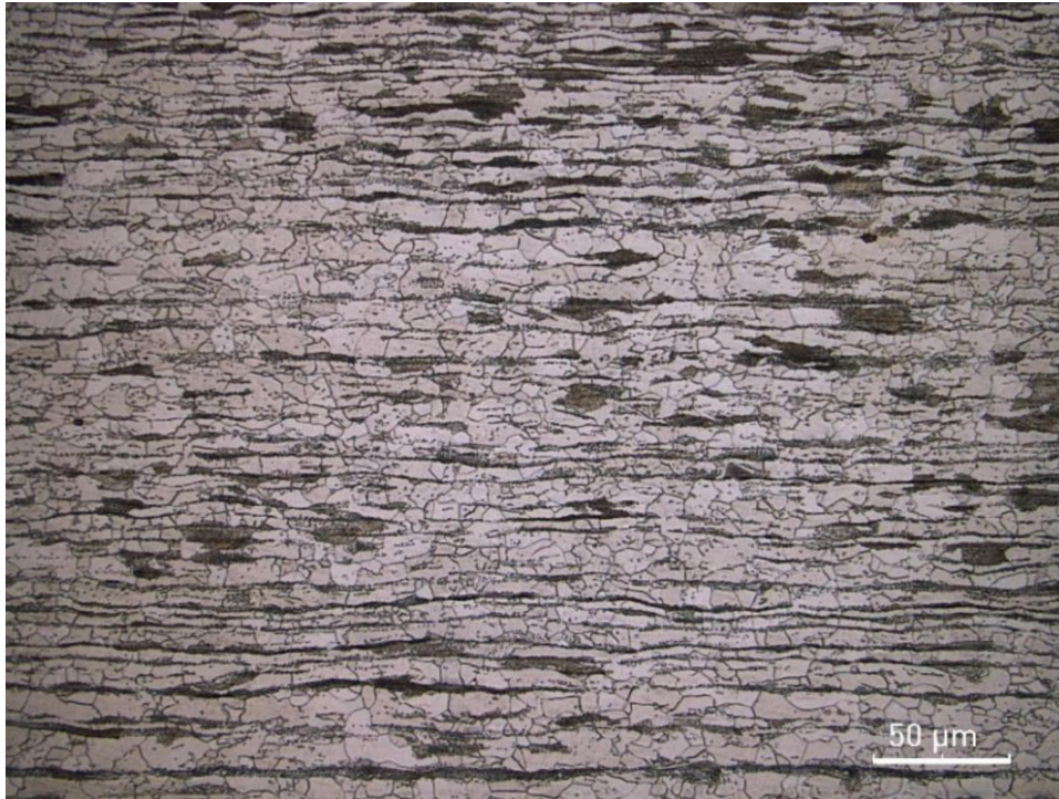
Figure 5.2. Light Microscope image of 680-45-5. Dark regions are pearlite, white regions are ferrite.
