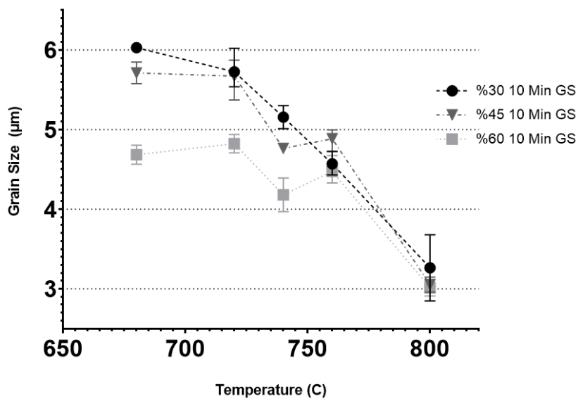
Figure 4.33. Ferrite grain sizes of 10 minute annealed samples
