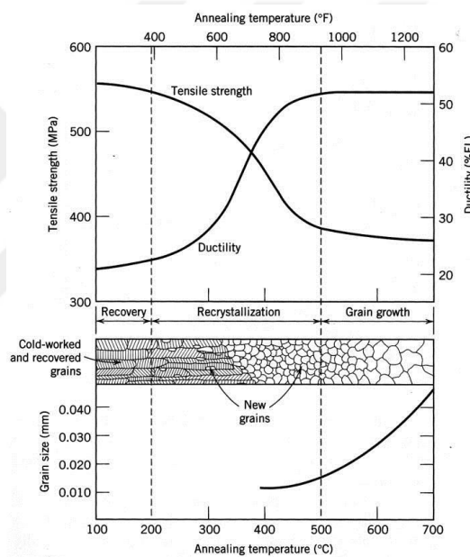
Figure 2.7. Schematic representation of cold worked grains during recovery recrystallization and grain growth [17].
