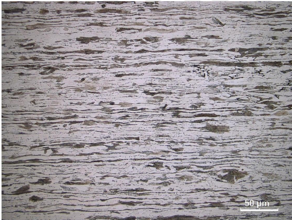
Figure 4.8. 45% CR specimen before heat treatment.
