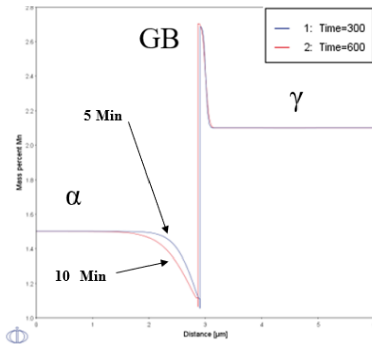
Figure 5.13. Mn partitioning during annealing at 760°C.
