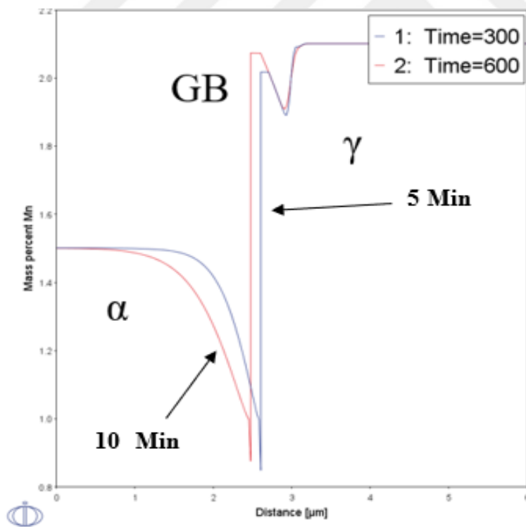
Figure 5.14. Mn partitioning during annealing at 780°C.
