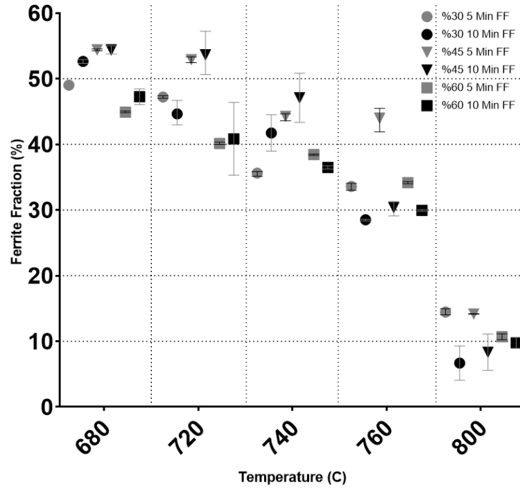
Figure 5.19. Ferrite fraction of annealed samples.
