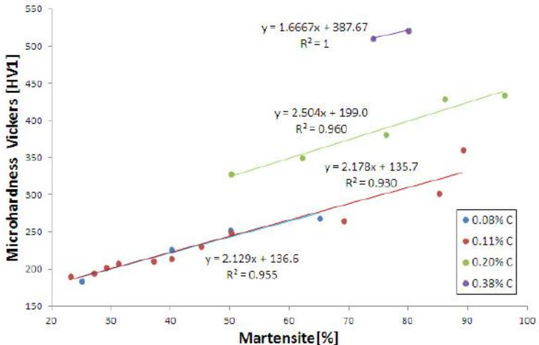
Figure 2.15. Microhardness of martensite depending on the C content [55].
