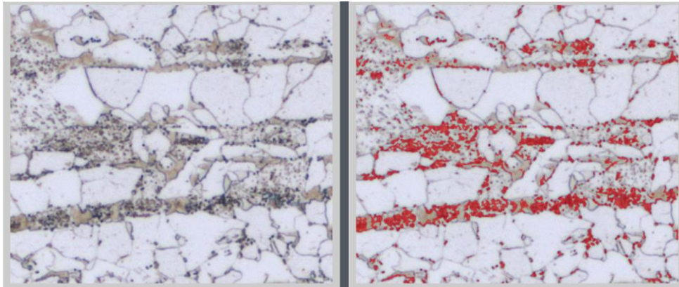
Figure 5.11. Carbide fraction determination with MIPAR in 720-NR-5.
