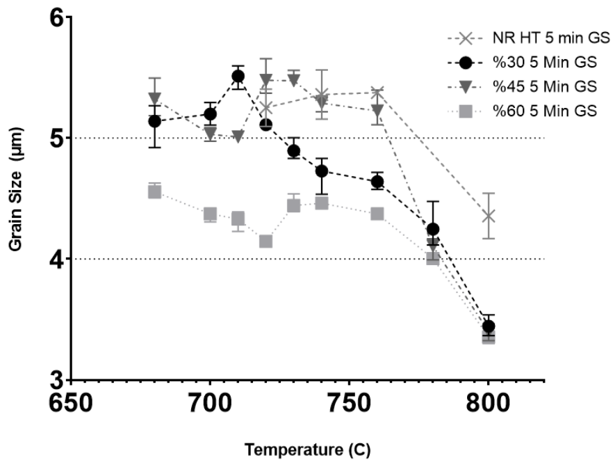
Figure 4.28. Ferrite grain sizes of 5 minute soaked samples.
