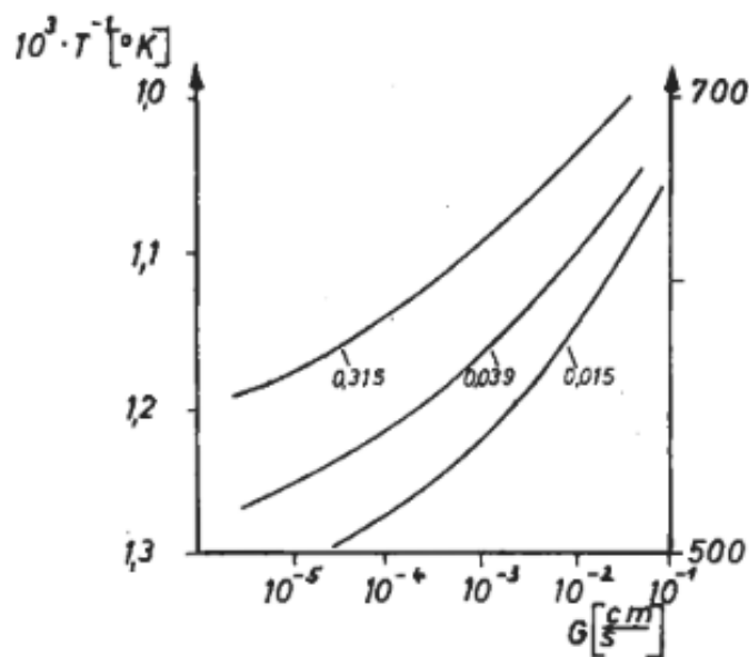
Figure 2.9. Effect of Mo addition on the ferrite grain interface front speed. Horizontal axis indicates the interface front speed, left axis indicates the temperature [41].
