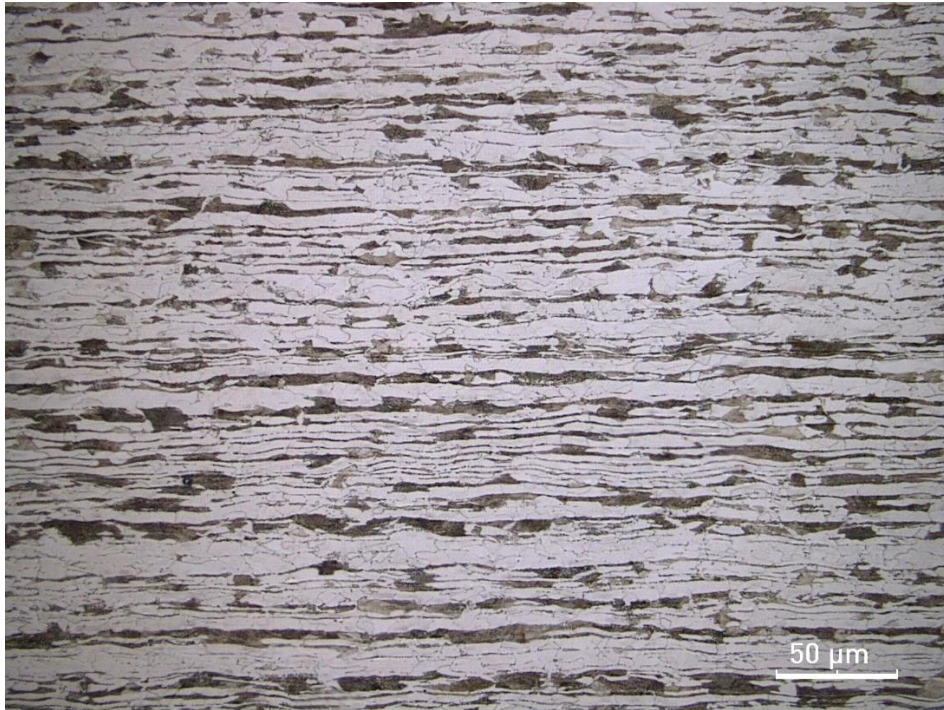
Figure 4.7. 30% CR specimen before heat treatment.
