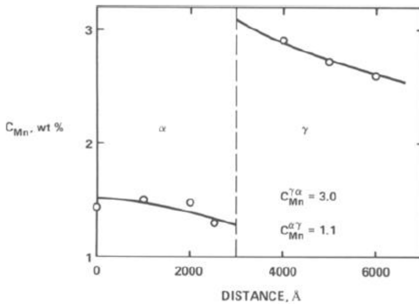
Figure 2.21. Mn concentration of ferrite and austenite phases in 0.06C-1.5Mn steel after 1h annealing at 740°C [60].
