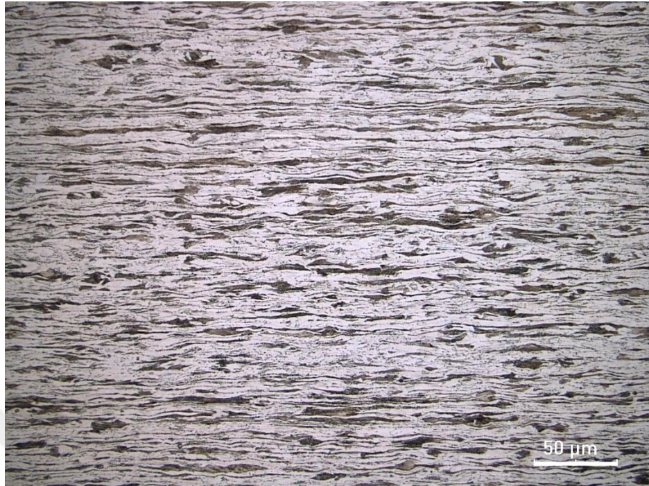
Figure 4.9. 60% CR specimen before heat treatment.
