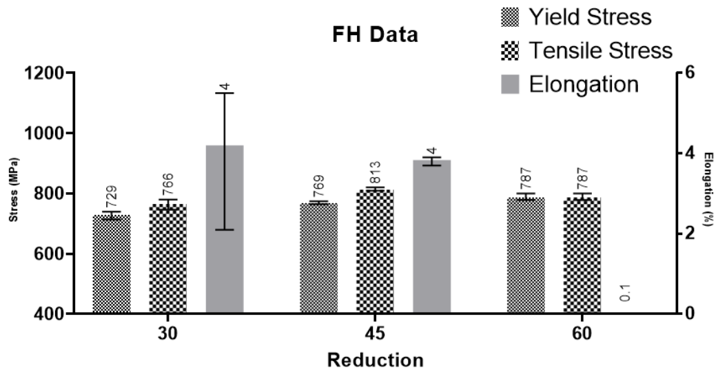
Figure 4.10. Yield strength, tensile strength and elongation of samples after cold rolling.
