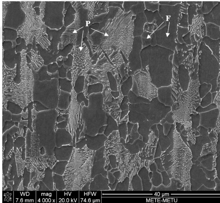
Figure 4.4. SEM image of Part2. F represents ferrite, P represents pearlite.
