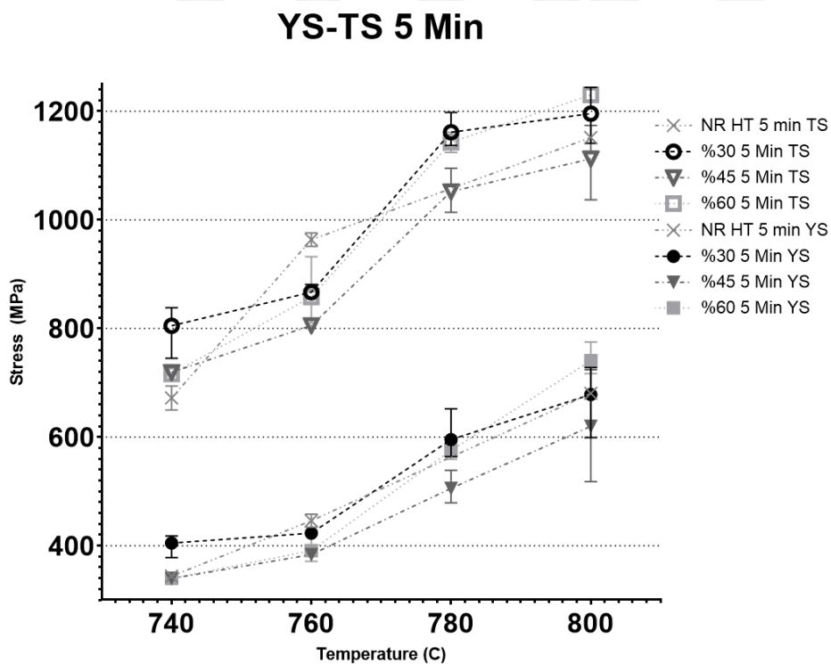
Figure 4.26. Yield strength and tensile strength of 5 minute annealed samples above 740°C.
