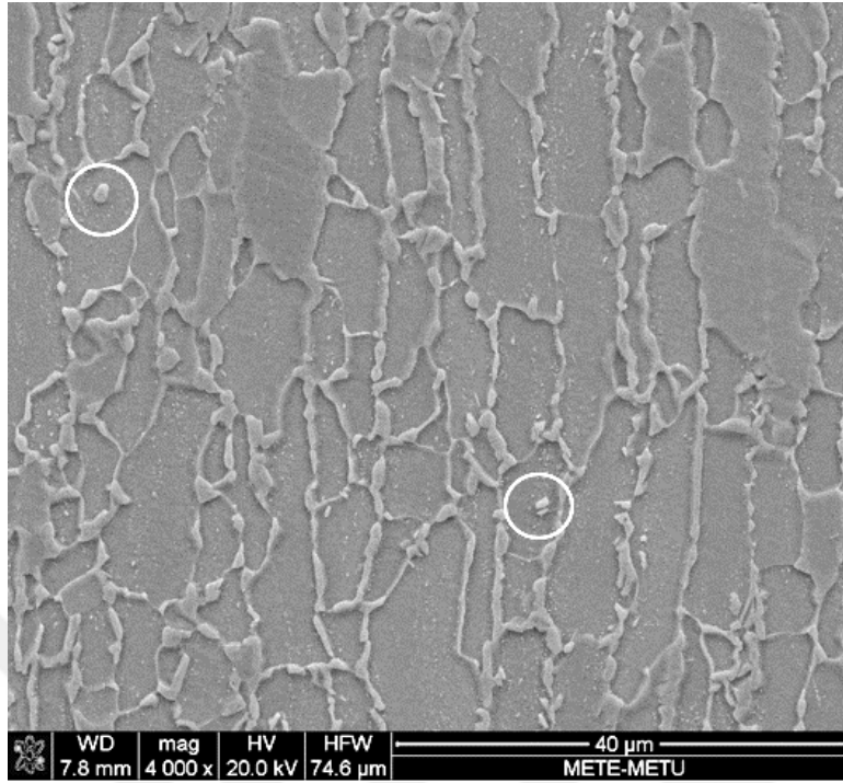
Figure 5.9. SEM image of 720-60-5. White circles represent austenite formation from agglomeration of fragmented cementite particles. Note that these particles are considerably lower in amount than 30% and 45% CR samples.
