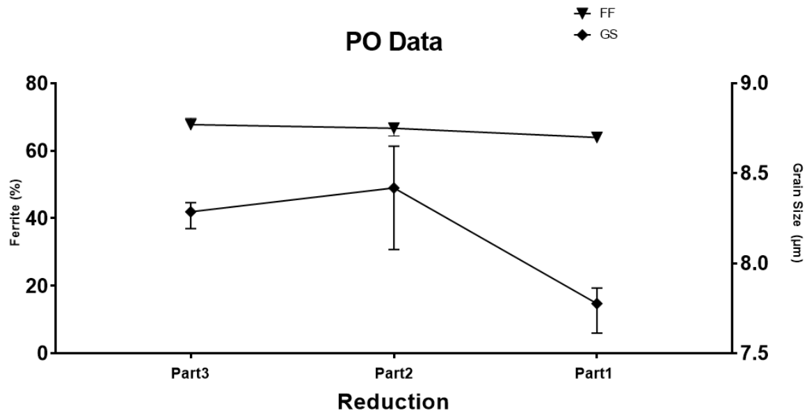
Figure 4.5. Ferrite fraction and grain size of each part prior to cold rolling.
