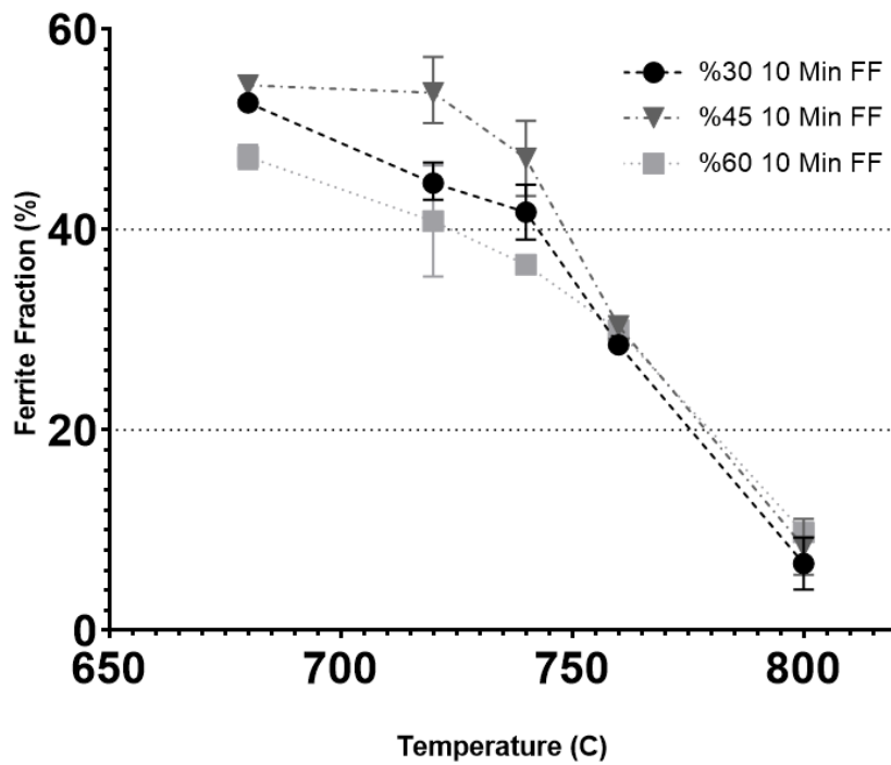
Figure 4.32. Ferrite fractions of 10 minute annealed samples.
