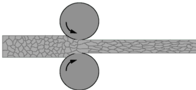
Figure 2.4. Typical grain structure after cold rolling of steel [30].
