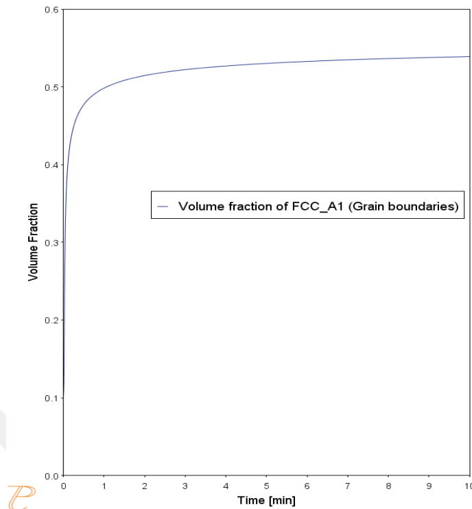
Figure 5.24. Volume fraction of austenite in 0.14C-1.98Mn steel.
