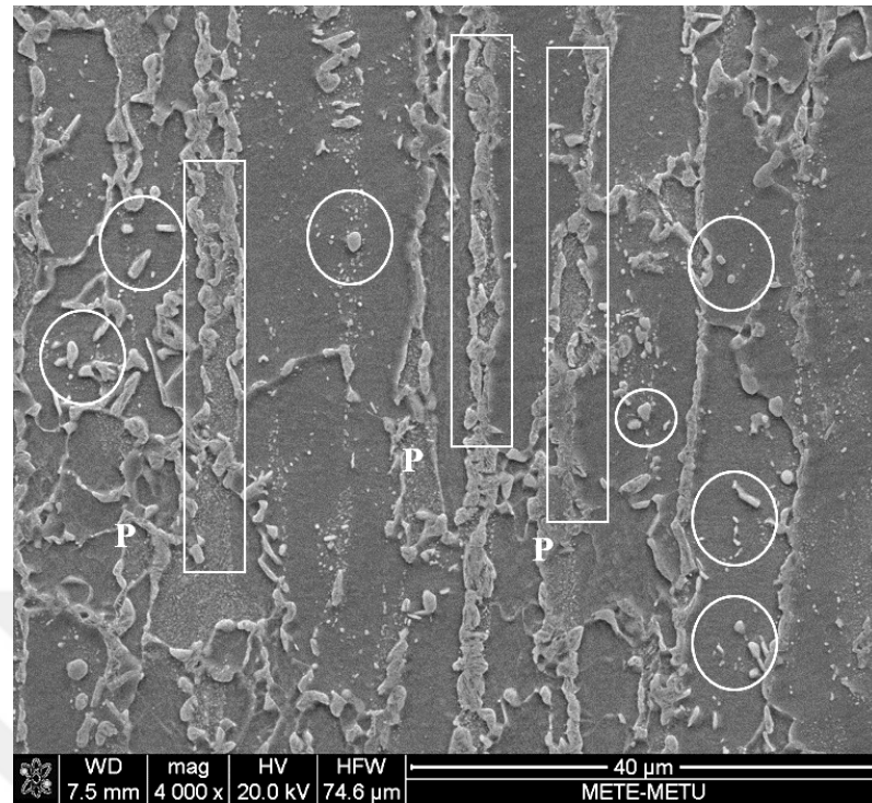
Figure 5.7. SEM image of 720-30-5. White circles represent austenite formation from agglomeration of fragmented cementite particles, white rectangles represent prior pearlite bands, P represents Pearlite.
