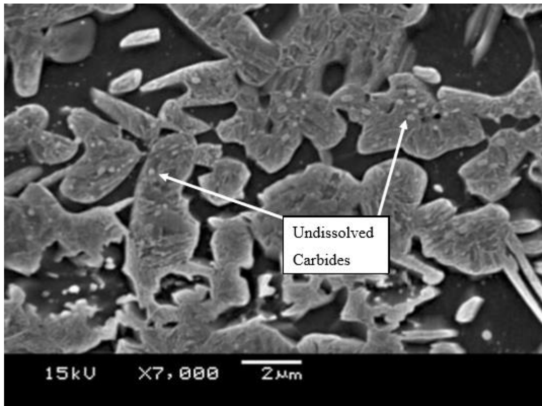
Figure 2.10. Undissolved Carbide precipitates in martensite grains [13].
