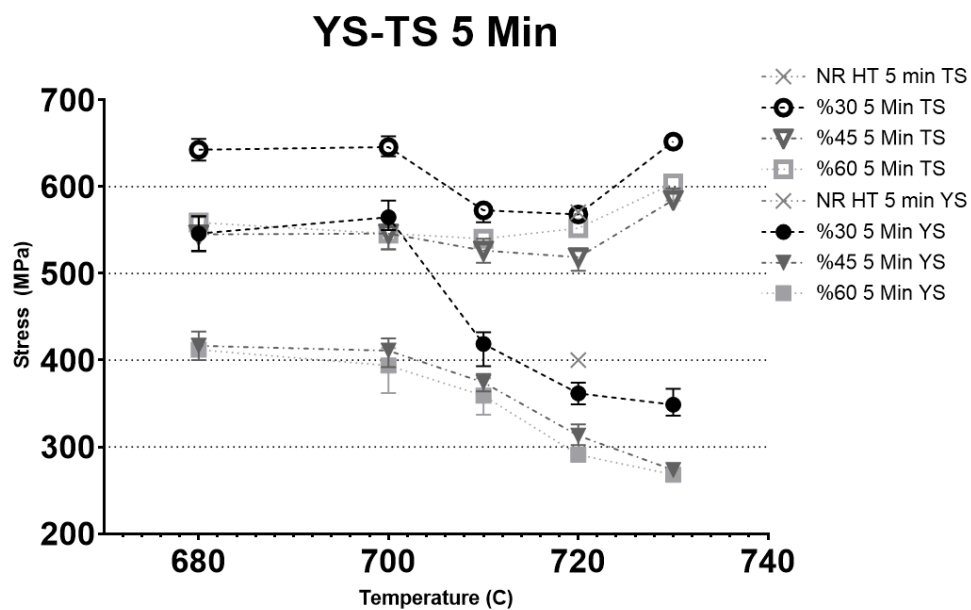
Figure 4.25. Yield Strength and Tensile Strength of 5 minute annealed samples below 740°C.
