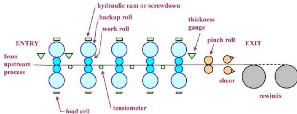
Figure 2.2. Tandem cold rolling mill [26]
