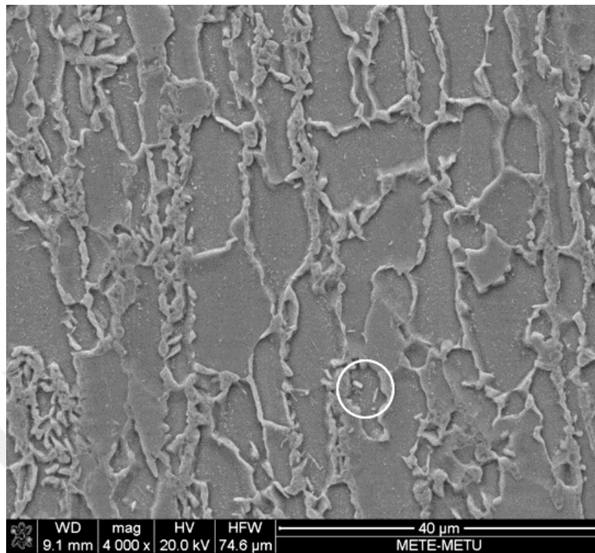
Figure 5.23. SEM image of 730-60-5. White arrows represent martensite inside the grains.
