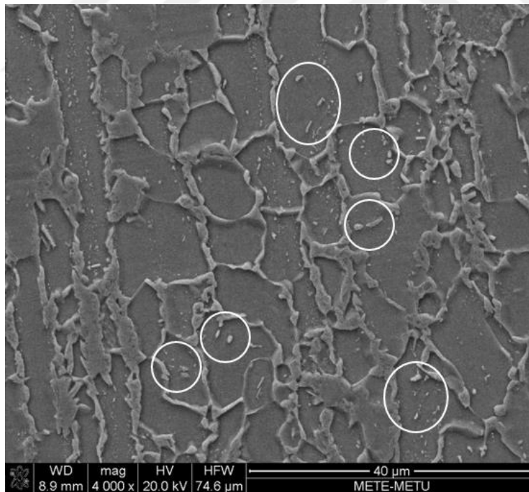
Figure 5.22. SEM image of 730-45-5. White arrows represent martensite inside the grains.
