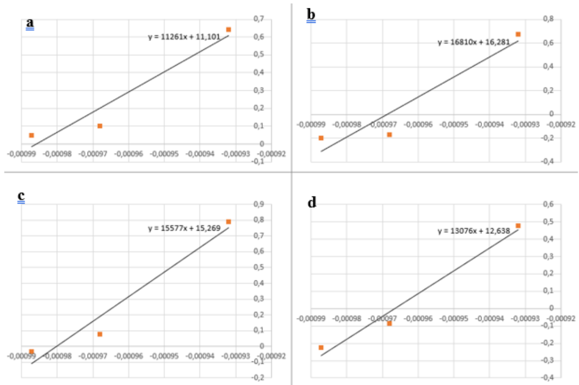
Figure 5.10. Plotted graphs for calculation of Q values. a) 30% CR, b) 45% CR, c) 60% CR, d) NR HT. Vertical lines correspond the \ln function in Eq.10, horizontal lines correspond the -1/T values.
