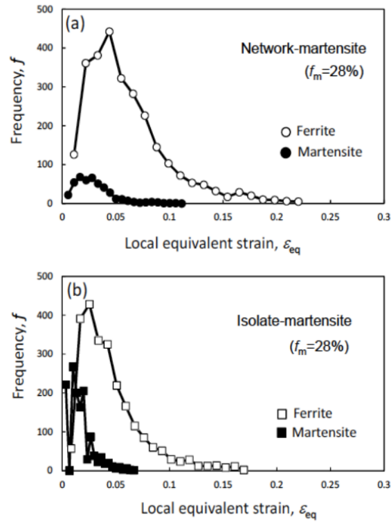
Figure 5.26. Strain distribution between ferrite and martensite in networked and isolated martensite structures [89].
