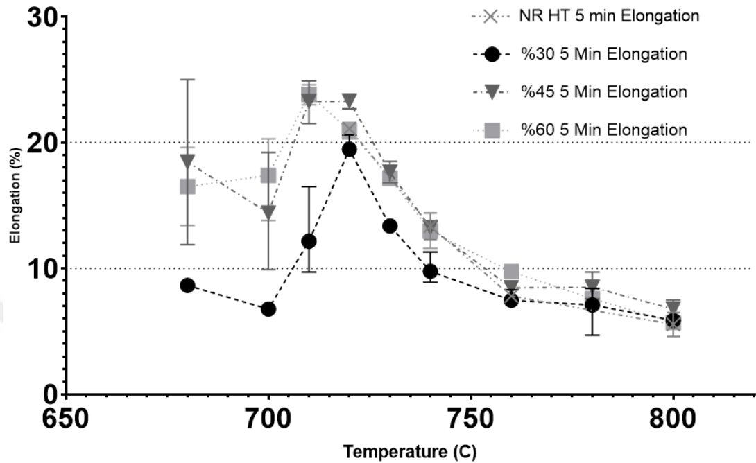
Figure 4.29. Temperature versus elongation for 5 minute annealed samples.
