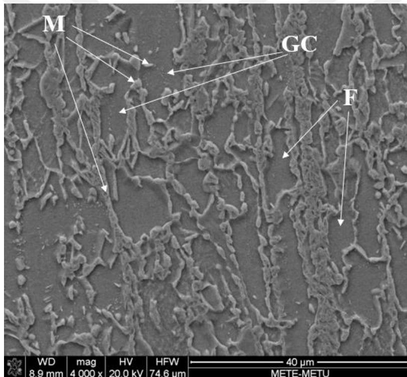
Figure 4.17. SEM image of 730-30-5.
