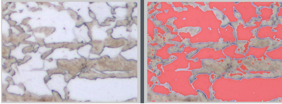
Figure 3.8. Ferrite fraction detection using MIPAR.
