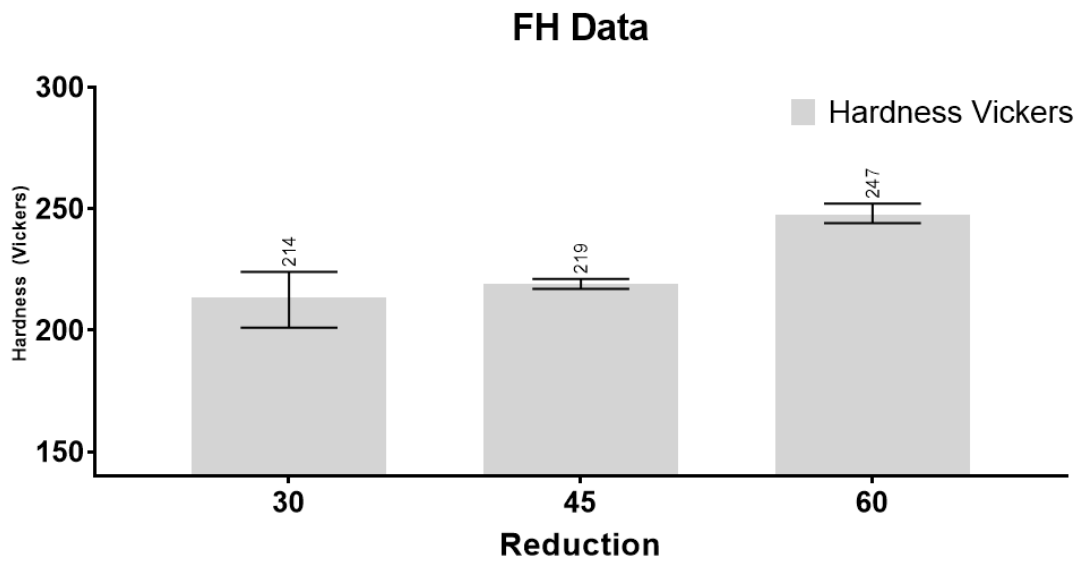
Figure 4.11. Hardness Vickers versus cold reduction ratio.
