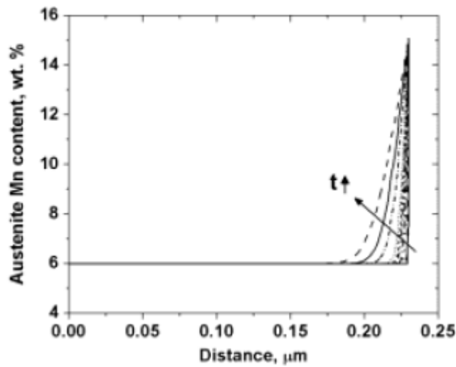
Figure 2.20. Mn profile in austenite in a 0.1C-6Mn steel at 650°C [57].
