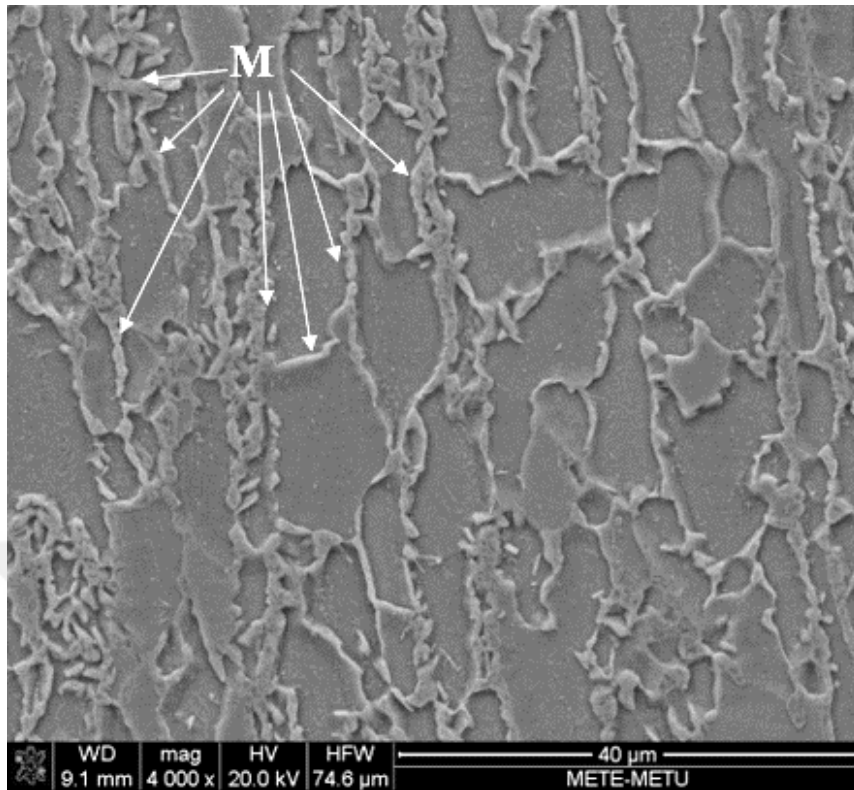
Figure 5.18. SEM image of 730-60-5. Almost all grain boundaries are covered with martensite (M).
