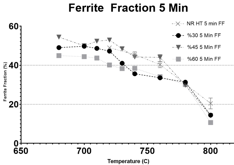
Figure 4.27. Ferrite fraction of 5 minute annealed samples.
