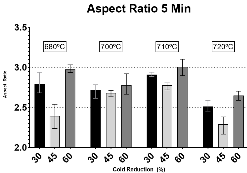
Figure 5.3. Ferrite aspect ratios of 5 minute annealed samples up to 720°C.
