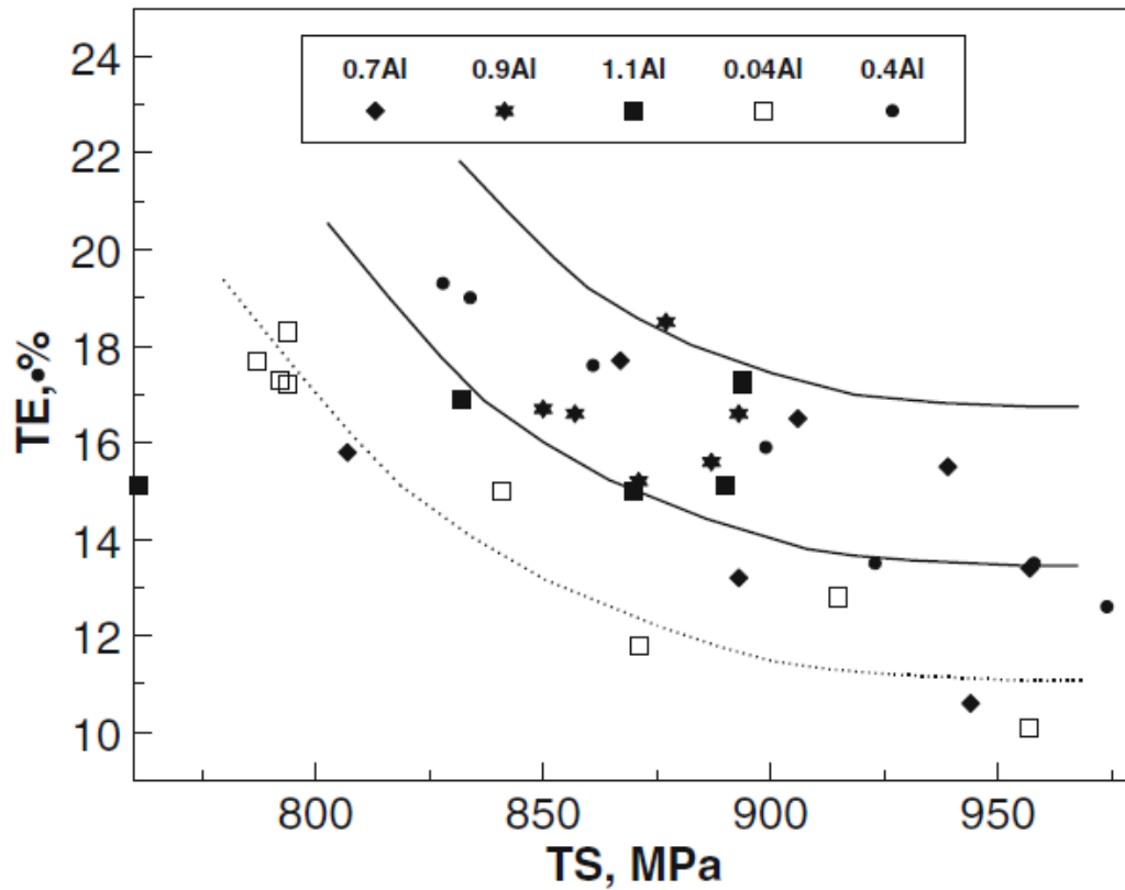
Figure 2.26. Tensile strength-elongation relationship with different amount of Al content in a dual phase steel [66].
