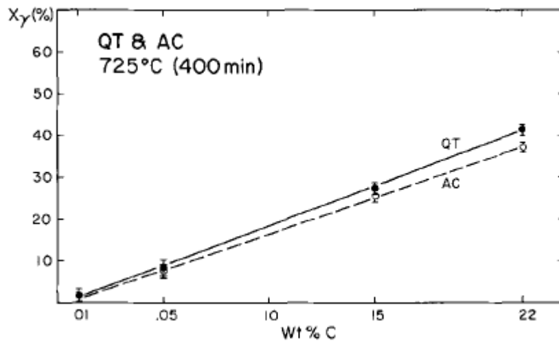
Figure 2.17. C content vs austenite fraction formed in 1.50Mn steel with two different starting microstructures [46].
