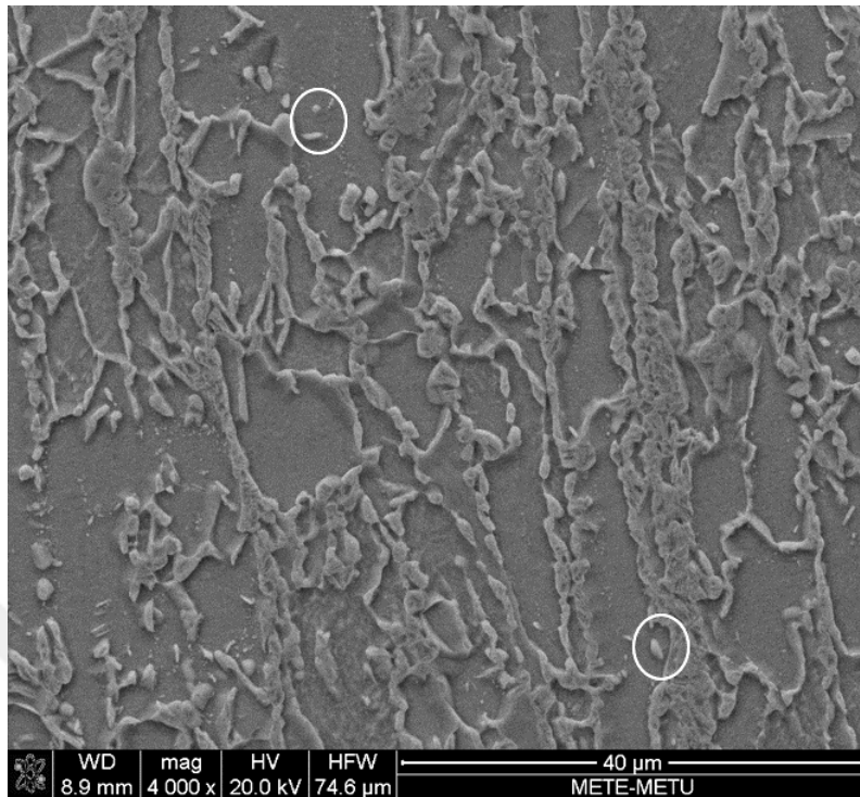
Figure 5.21. SEM image of 730-30-5. White arrows represent martensite inside the grains.
