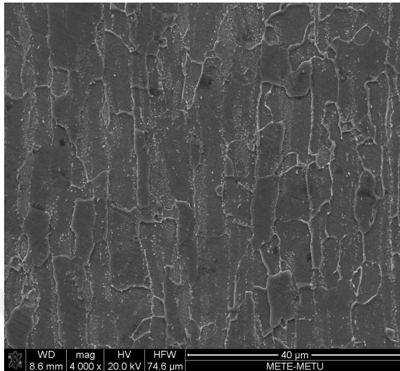
Figure 5.5. SEM image of 700-60-5 at 4000x. No deformed ferrite is observed.
