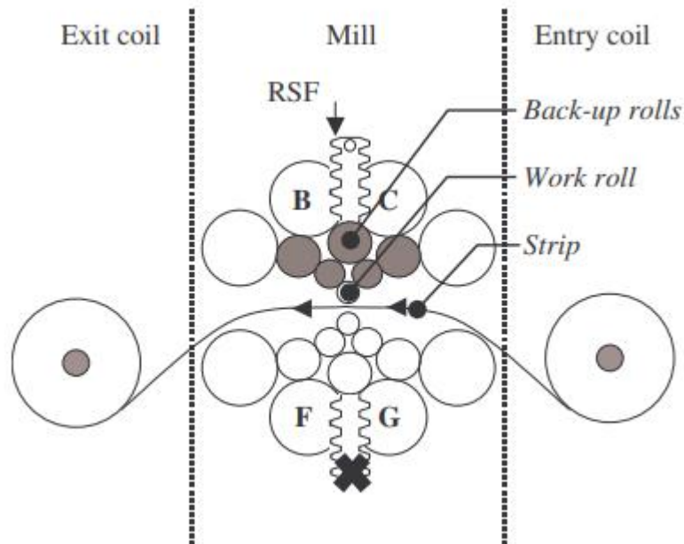
Figure 2.3. Reversible cold rolling mill [27].
