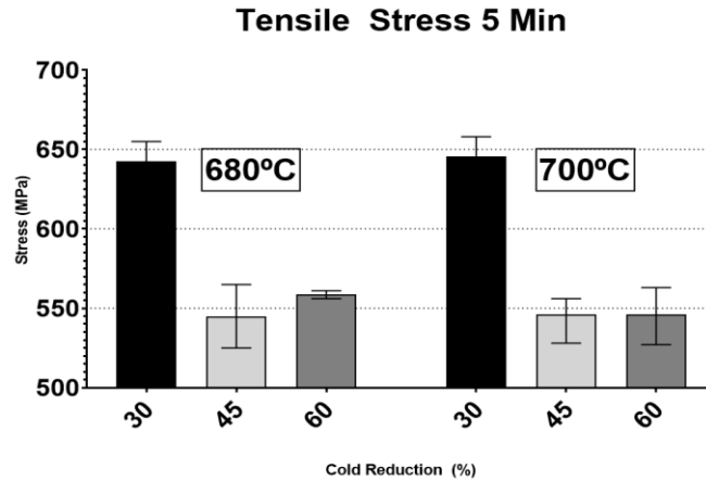
Figure 5.6. Tensile strength of samples at 680°C and 700°C.
