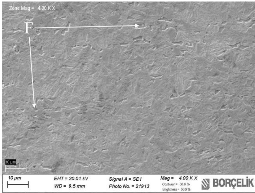
Figure 4.24. SEM image of 800-60-5.
