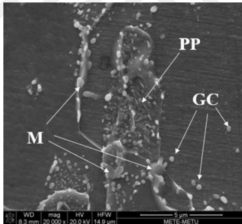
Figure 4.13. High magnification image of 700-30-5. M represents martensite, PP represents prior pearlite, GC represents globular cementite.
