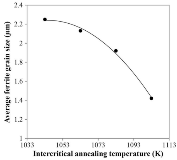
Figure 5.16. Ferrite grain size versus intercritical annealing temperature, from the study of Mazaheri et al [75].
