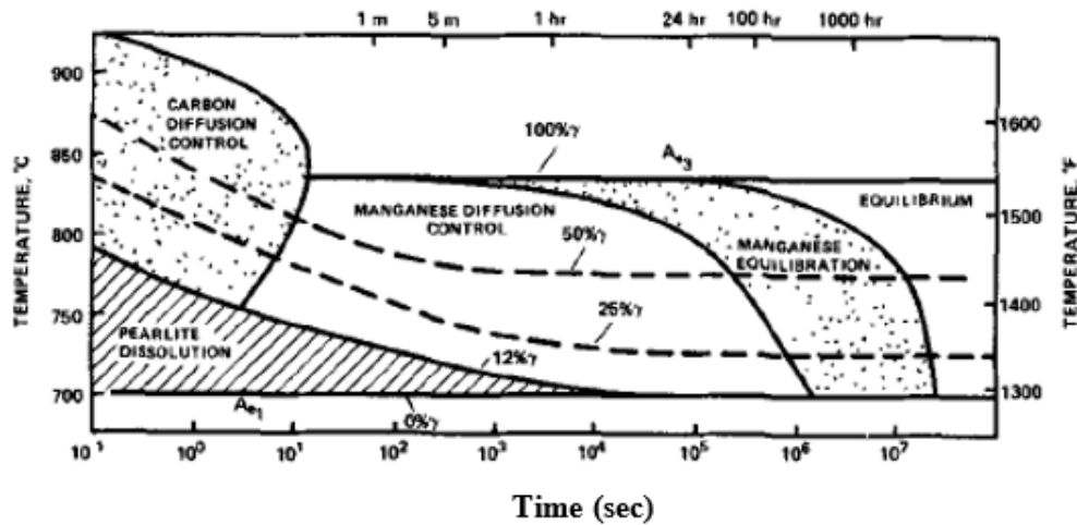
Figure 2.24. Austenite formation diagram for 0.12C-1.5Mn steel [60].
