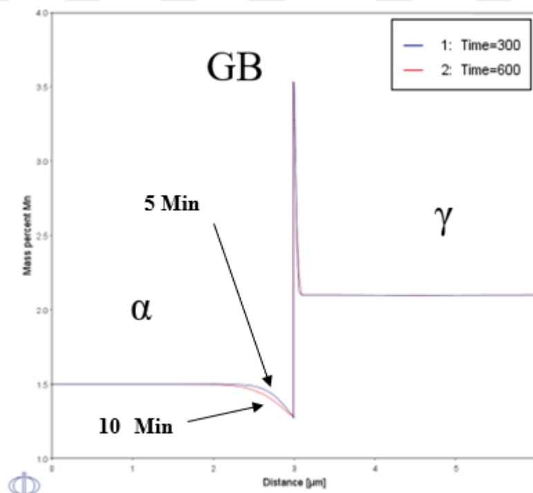
Figure 5.12. Mn partitioning during annealing at 740°C.
