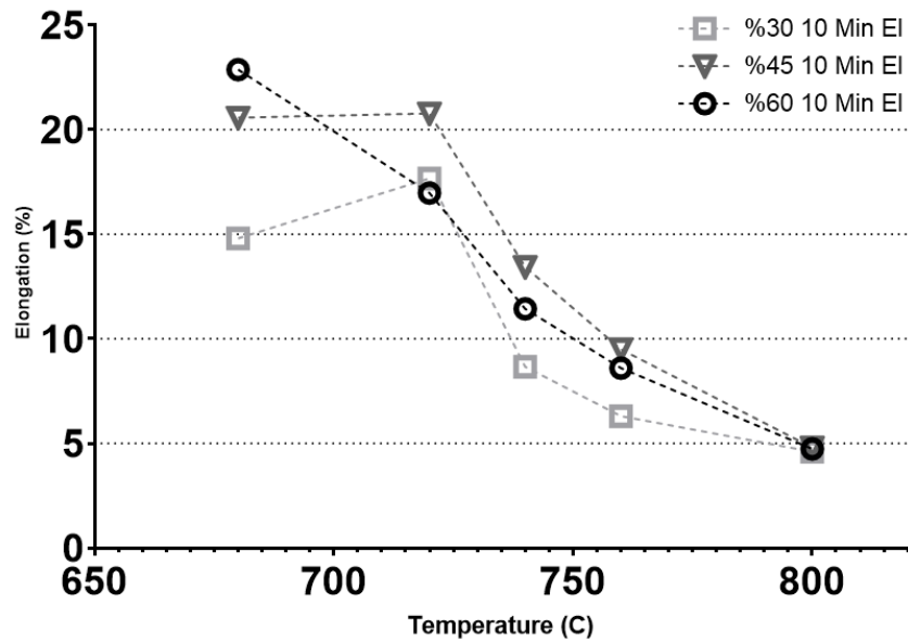
Figure 4.31. Temperature-Elongation plot of 10 minute annealed samples.
