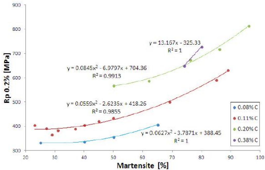
Figure 2.16. Yield strength of DP steels depending on C content [55]
