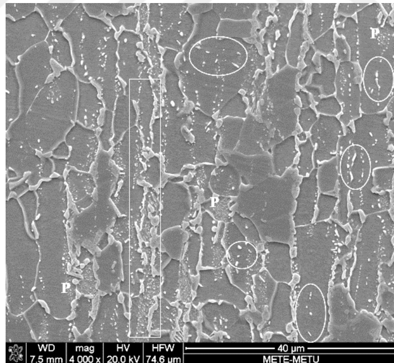
Figure 5.8. SEM image of 720-45-5. White circles represent austenite formation from agglomeration of fragmented cementite particles, white rectangles represent prior pearlite bands, P represents Pearlite.
