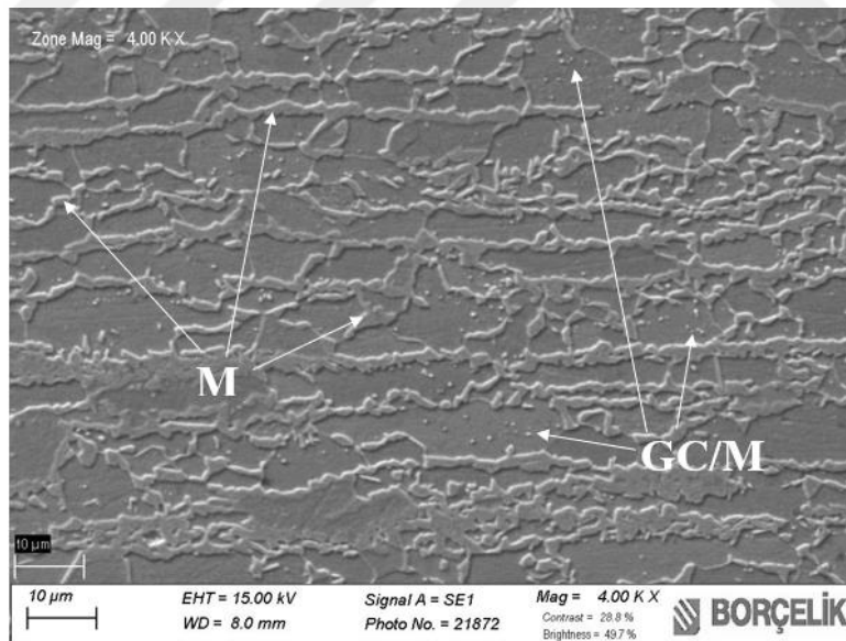
Figure 4.21. SEM micrograph of 740-45-10.
