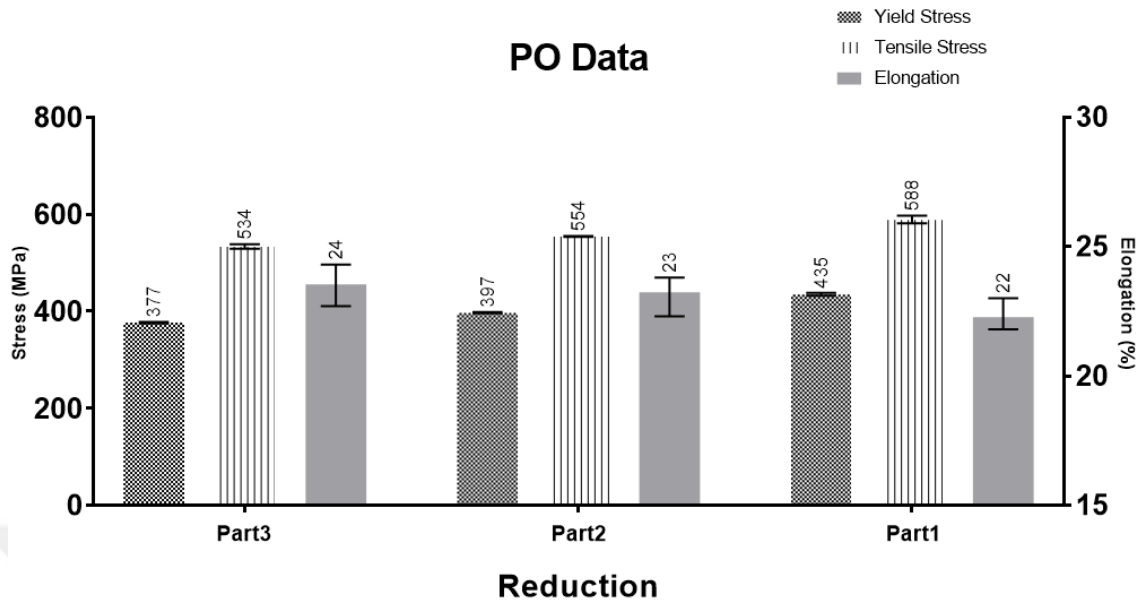
Figure 4.6. Mechanical properties of each part of the PO.
