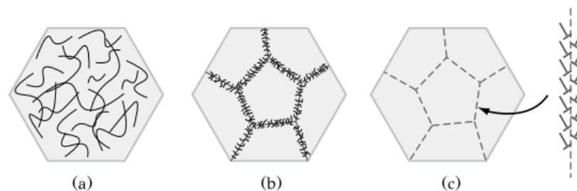
Figure 2.8. Microstructural changes during recovery [38].
