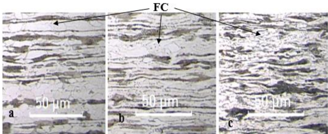
Figure 5.20. The degree of elongation of grains and cementite fragmentation in a) 30%, b) 45%, c) 60% as rolled samples. FC represents fragmented cementite.
