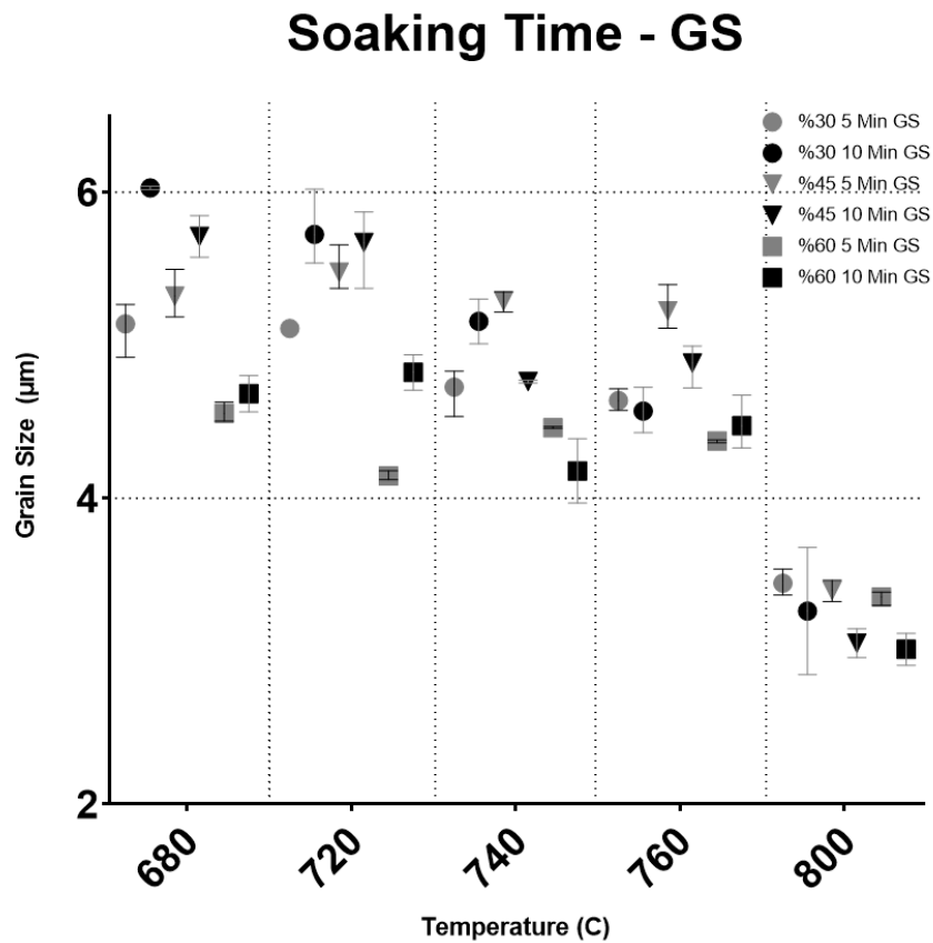
Figure 5.15. Grain sizes of annealed samples.
