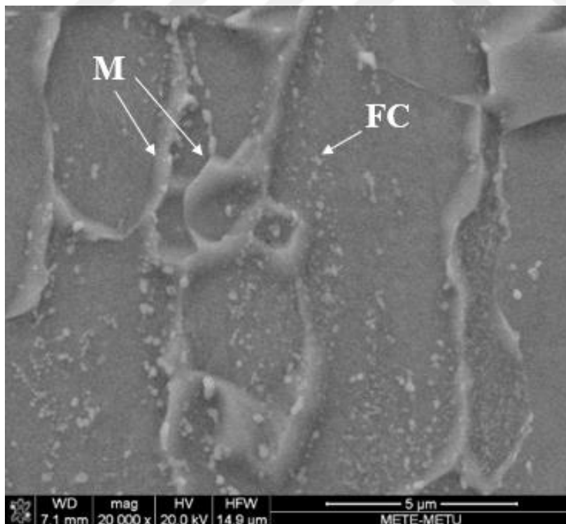
Figure 4.15. SEM micrograph of 700-60-5. M represents martensite, FC represents fragmented cementite.
