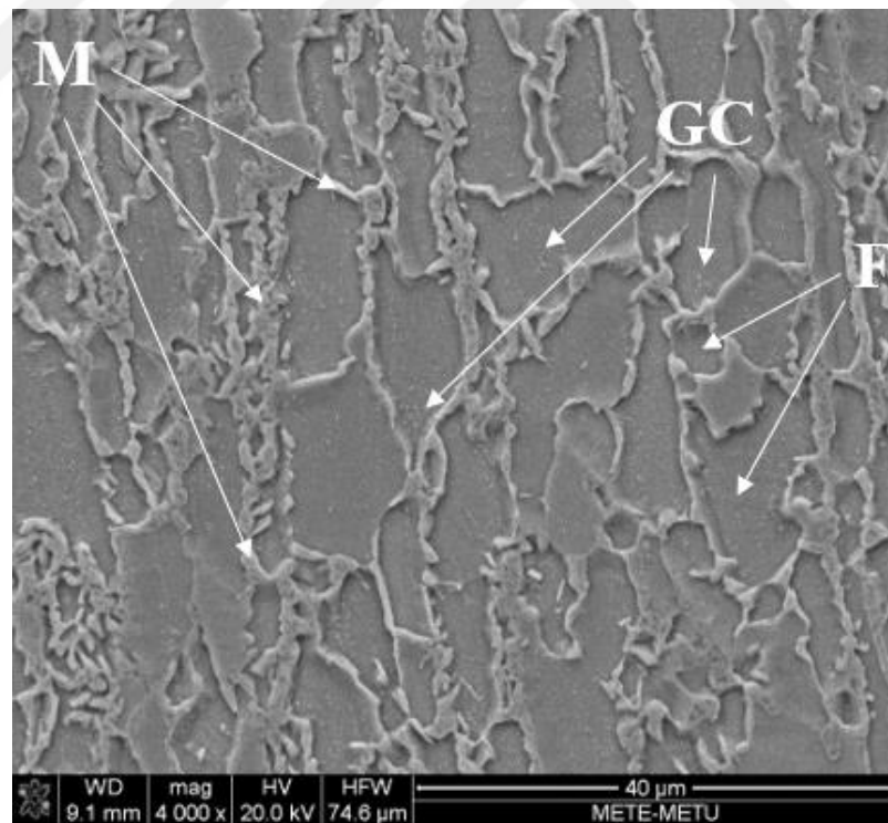
Figure 4.19. SEM image of 730-60-5.
