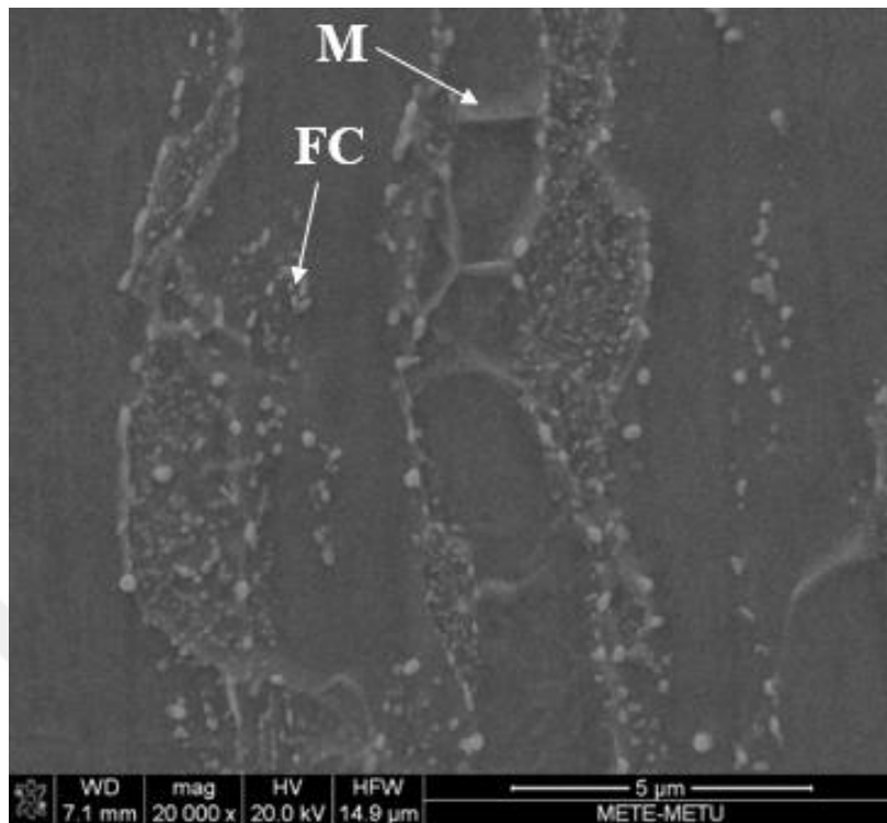
Figure 4.14. SEM micrograph of 700-45-5. M represents martensite, FC represents fragmented cementite.
