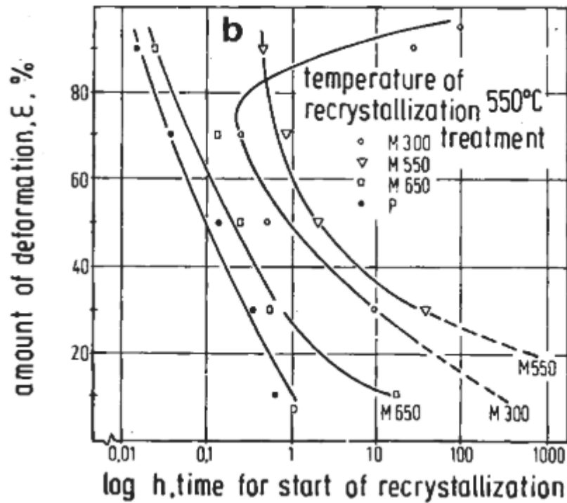
Figure 2.6. Recrystallization of steel with 0.22C with different martensite tempering temperatures and pearlitic microstructure [29].
