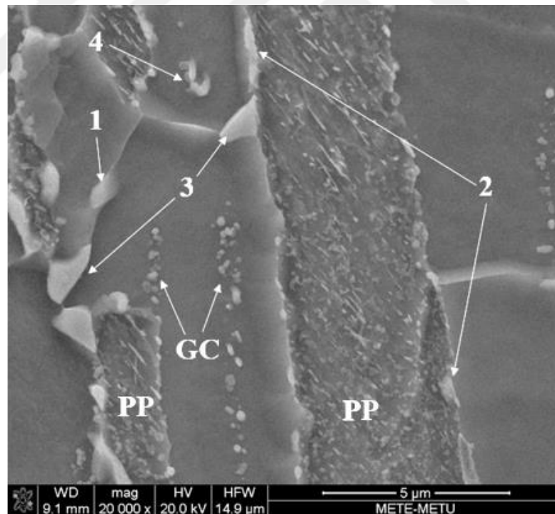
Figure 4.16. SEM image of 710-45-5. GC represents globular cementite, PP represents prior pearlite.
