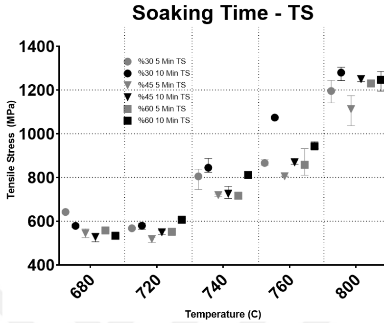
Figure 5.25. Tensile strengths of 5 minute and 10 minute annealed samples .
