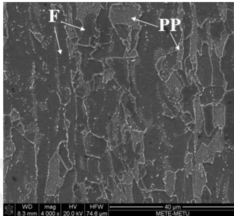
Figure 4.12. Microstructure of 700-30-5. F represents ferrite, PP represents prior pearlite.
