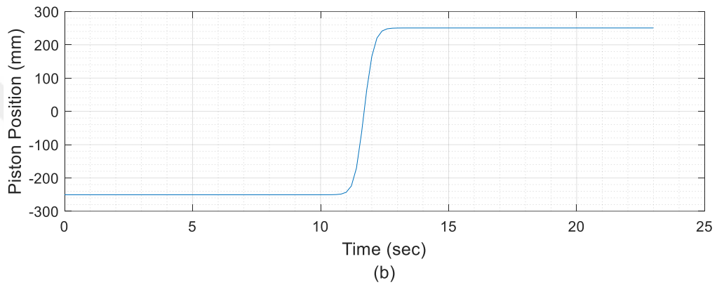
Figure 3.9: Piston Positions for Dry (a) and Half-Water (b) Conditions
