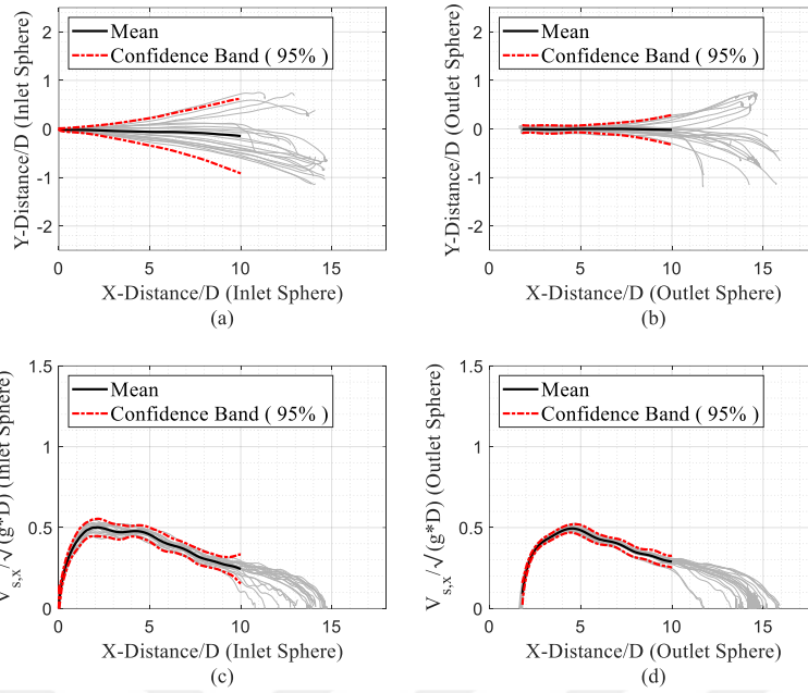
Figure 4.12: Results of Case 7 (SP7-NB-T-HI: Two Spheres under Non-Breaking Wave Attack on the Impermeable Slope and Impermeable Horizontal Area for Half-Water Condition) (a-b) Dimensionless Trajectory and (c-d) Dimensionless Velocity for Inlet and Outlet Spheres
