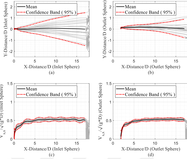
Figure 4.18: Results of Case 13 (SP13-B-T-DI: Two Spheres under Breaking Wave Attack on the Impermeable Slope and Impermeable Horizontal Area for Dry Condition) (a-b) Dimensionless Trajectory and (c-d) Dimensionless Velocity for Inlet and Outlet Spheres
