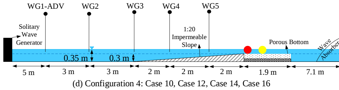
Figure 3.7: Side Views of the Experimental Setup for Different Configurations (Non-breaking Cases: a-b, Breaking Cases: c-d, Figure is not the scale!)
