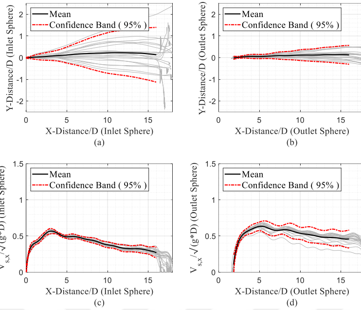
Figure 4.20: Results of Case 15 (SP15-B-T-HI: Two Spheres under Breaking Wave Attack on the Impermeable Slope and Impermeable Horizontal Area for Half-Water Condition) (a-b) Dimensionless Trajectory and (c-d) Dimensionless Velocity for Inlet and Outlet Spheres
