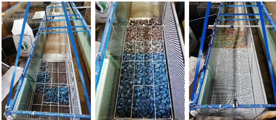
Figure 3.3: Captions for the Construction of the Porous Bottom with 1:4.5 Slope
