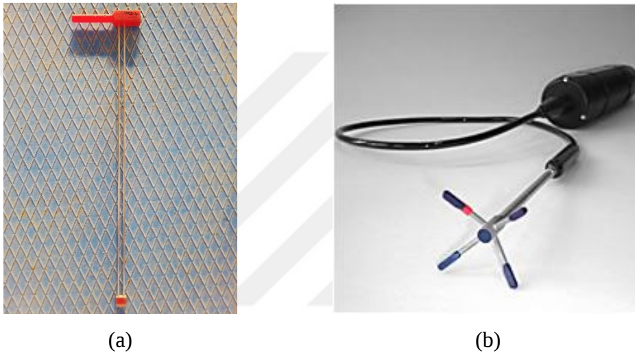
Figure 3.5: Wave Gauge (a) and Water Particle Velocity Measure Device (b)
