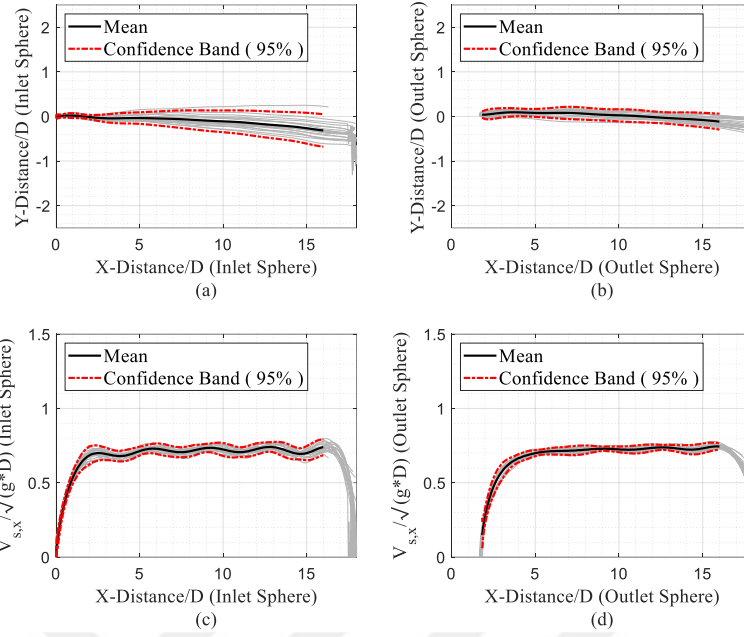
Figure 4.10: Results of Case 5 (SP5-NB-T-DI: Two Spheres under Non-Breaking Wave Attack on the Impermeable Slope and Impermeable Horizontal Area for Dry Condition) (a-b) Dimensionless Trajectory and (c-d) Dimensionless Velocity for Inlet and Outlet Spheres
