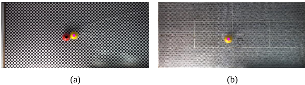
Figure 3.12: Tracked Captions of the Spheres for the Impermeable Bottom (a) and the Porous Bottom (b)
