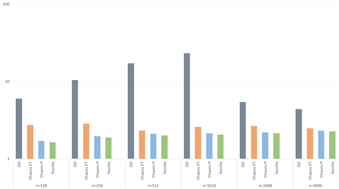
Figure 7.12 Average length of SISs generated by JUJY, with W-sets/K-sets generated by several algorithms, given in logarithmic scale, for p = 128 and q = 128
