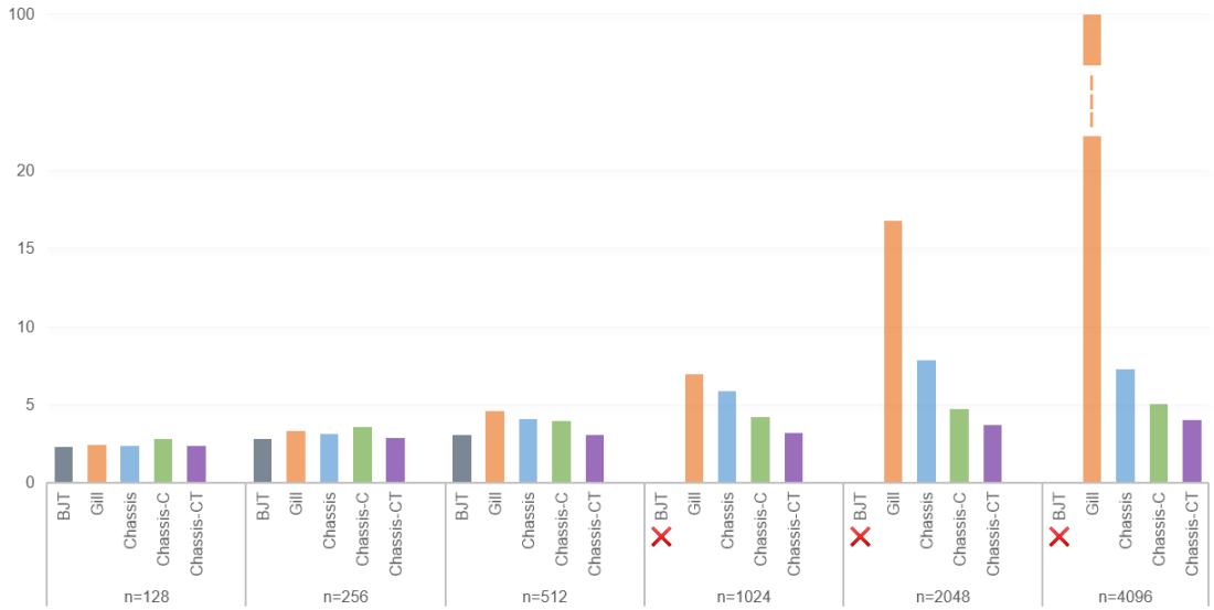
Figure 6.4 Average total number of input letters of the W -sets that each algorithm generates, for p = 128 and q = 128
