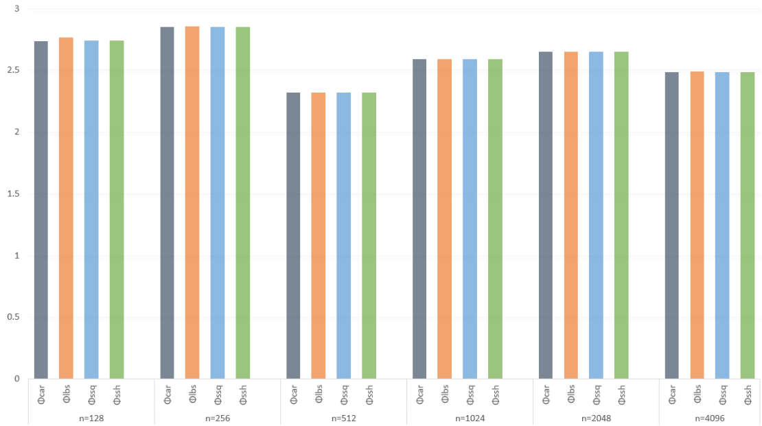
Figure 7.2 Average length of State Identification Sequences generated by each score function, for p = 128 and q = 128
