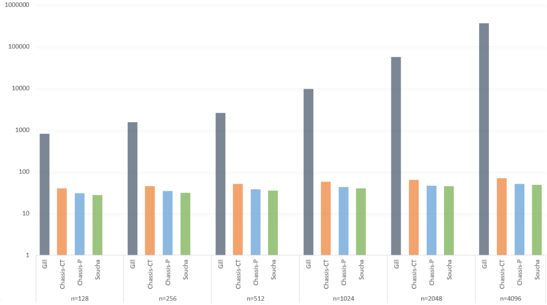
Figure 7.11 Average length of SISs generated by JUJY, with W-sets/K-sets generated by several algorithms, given in logarithmic scale, for p = 2 and q = 2
