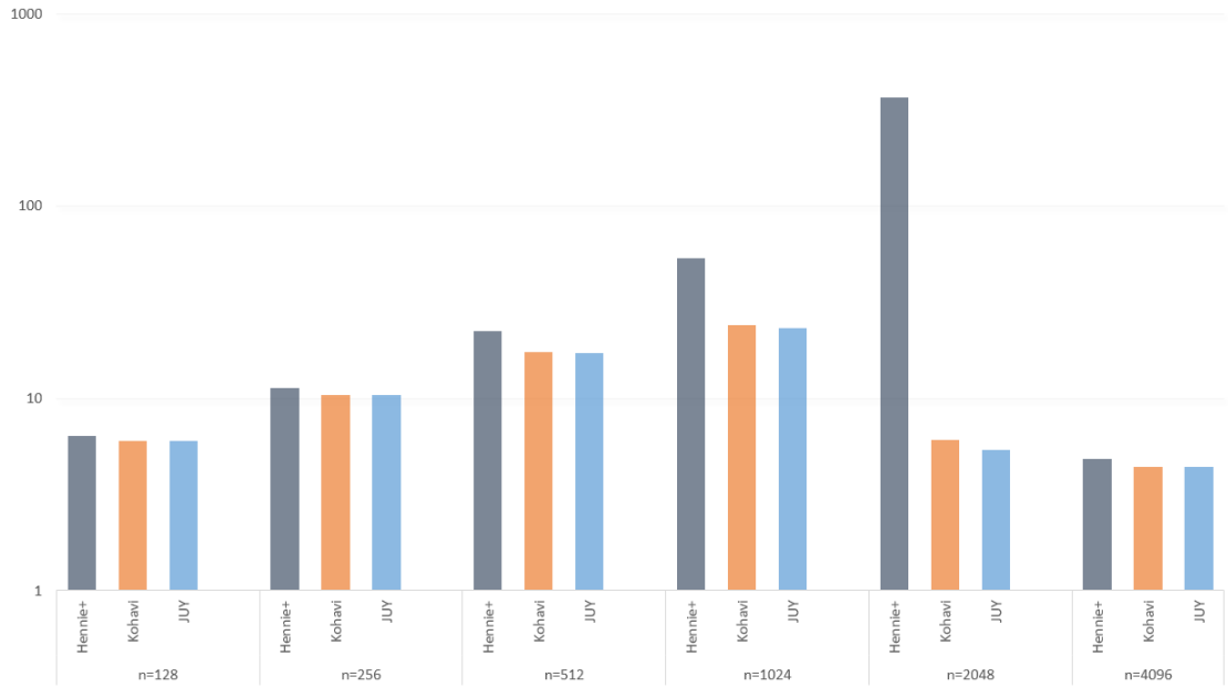
Figure 7.6 Average length of SISs generated by various techniques, with a W -set generated by GILL, given in logarithmic scale, for p = 128 and q = 128
