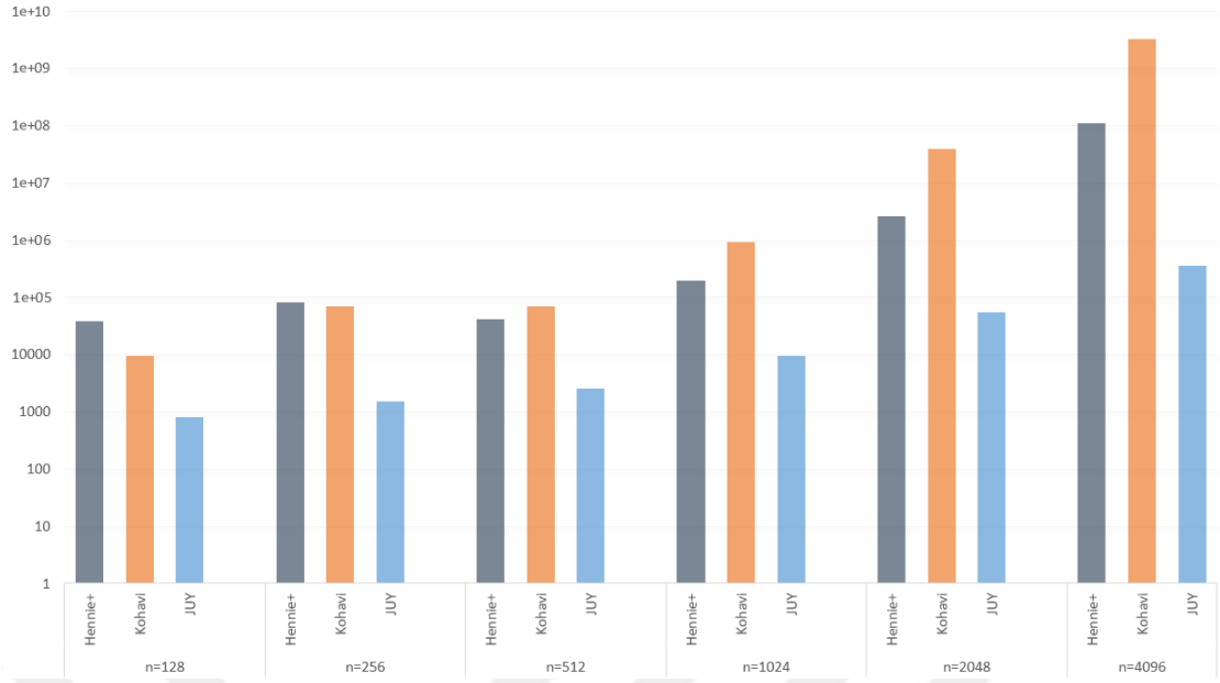
Figure 7.5 Average length of SISs generated by various techniques, with a W -set generated by GILL, given in logarithmic scale, for p = 2 and q = 2
