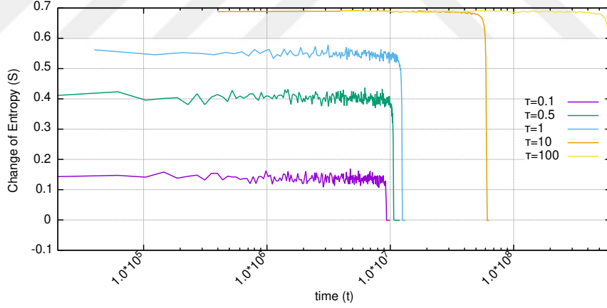
Figure 6.25: \Delta S_T graphs of simulations with bosonic heat baths for varying values of \tau
