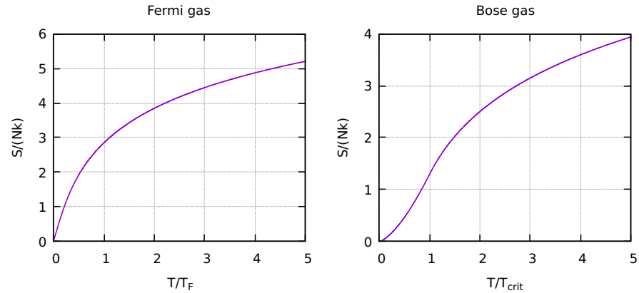
Figure 6.3: Reduced internal entropy per particle versus reduced temperature graphs
