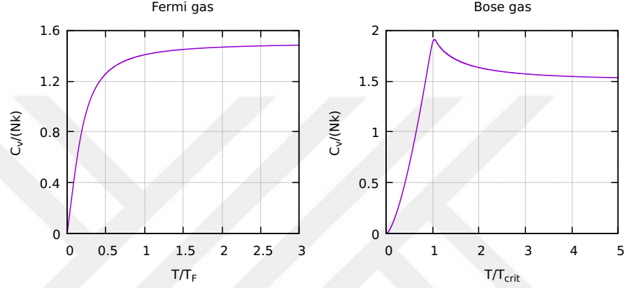
Figure 6.2: Reduced heat capacity per particle versus reduced temperature graphs
