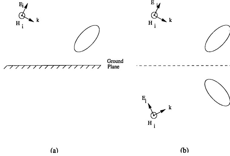
Figure 2.1: (a) A conducting body over a ground plane illuminated by an electromagnetic source. (b) The equivalent problem.
