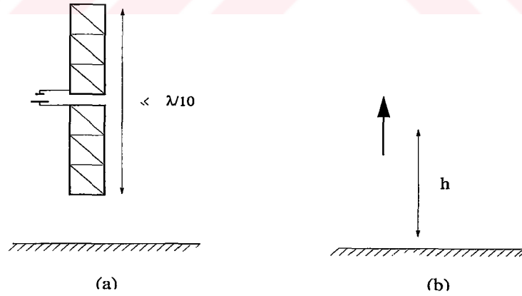
Figure 4.2: (a) A conducting strip approximating an infinitesimal dipole. (b) An infinitesimal electric dipole above the ground plane.
