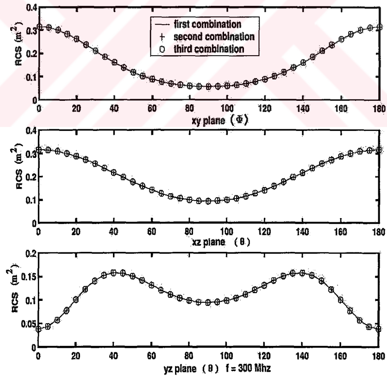
Figure 5.8: The RCS results of the geometry shown in Figure 5.7 using three different combinations from a set of 16 acceptable choices
