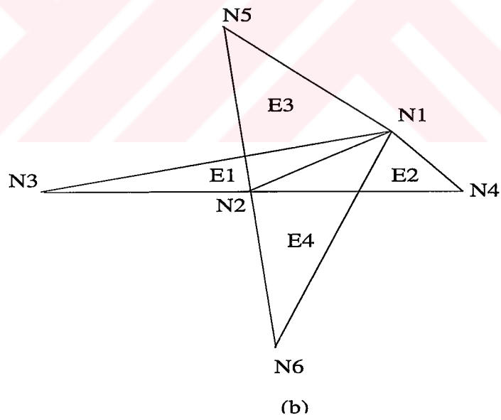
Figure 5.11: (a) A triangulated surface having only two-triangle connections. (b) A triangulated surface having four-triangle connections.
