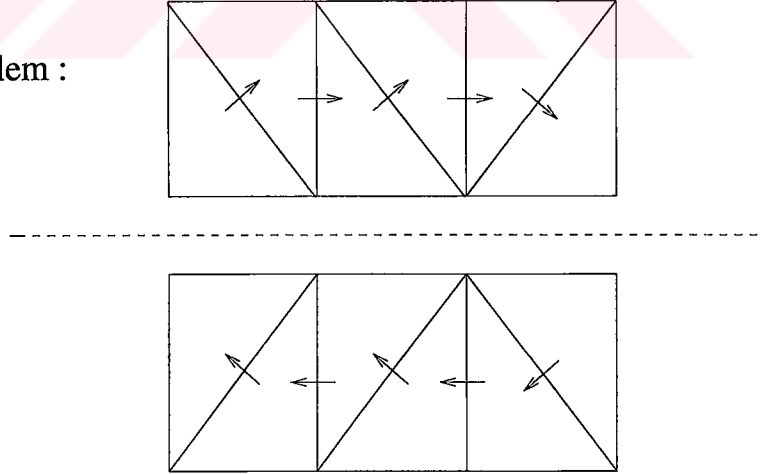
Figure 2.2: Samples of induced currents on the triangulated surface of the rectangular plate above the ground plane and the equivalent problem.
