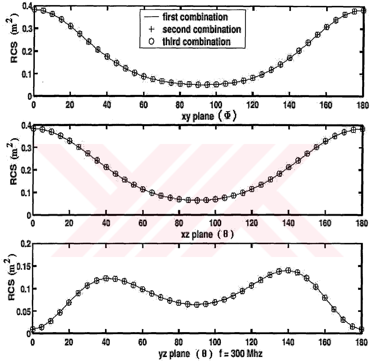
Figure 5.4: The RCS results of the geometry shown in Figure 5.3 using three different combinations of the basis functions.
