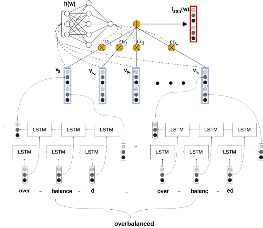
FIGURE 4.4. Architecture of morph2vec with an attention mechanism on top of bi-LSTMs. [9]
