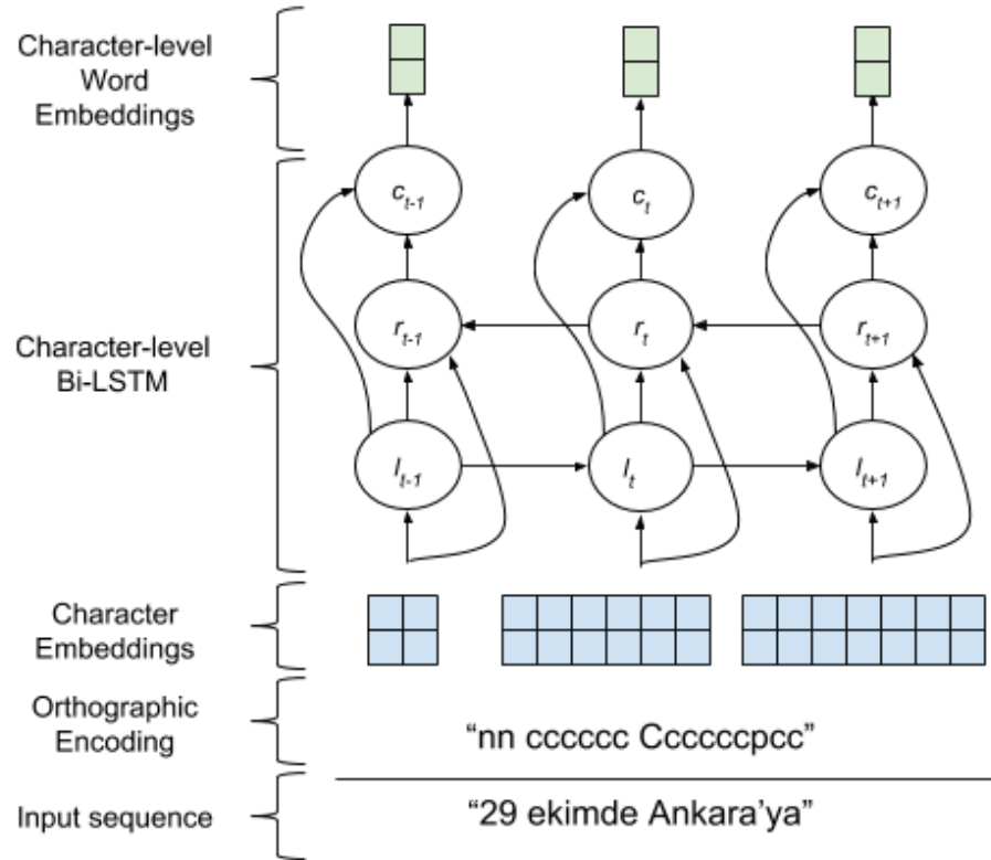
FIGURE 4.2. Character-level word embedding using a bidirectional LSTM
