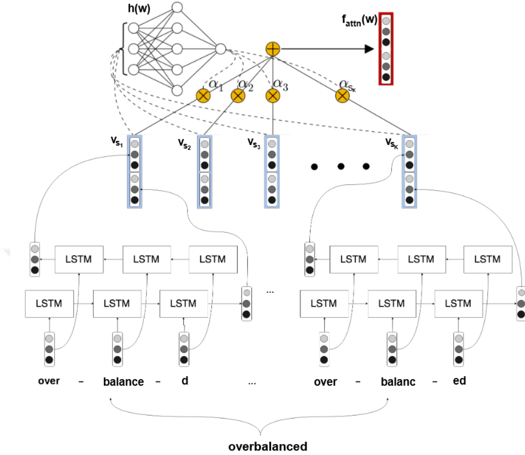
FIGURE 2.11. Architecture of morph2vec with an attention mechanism on top of bi-LSTMs. [9]
