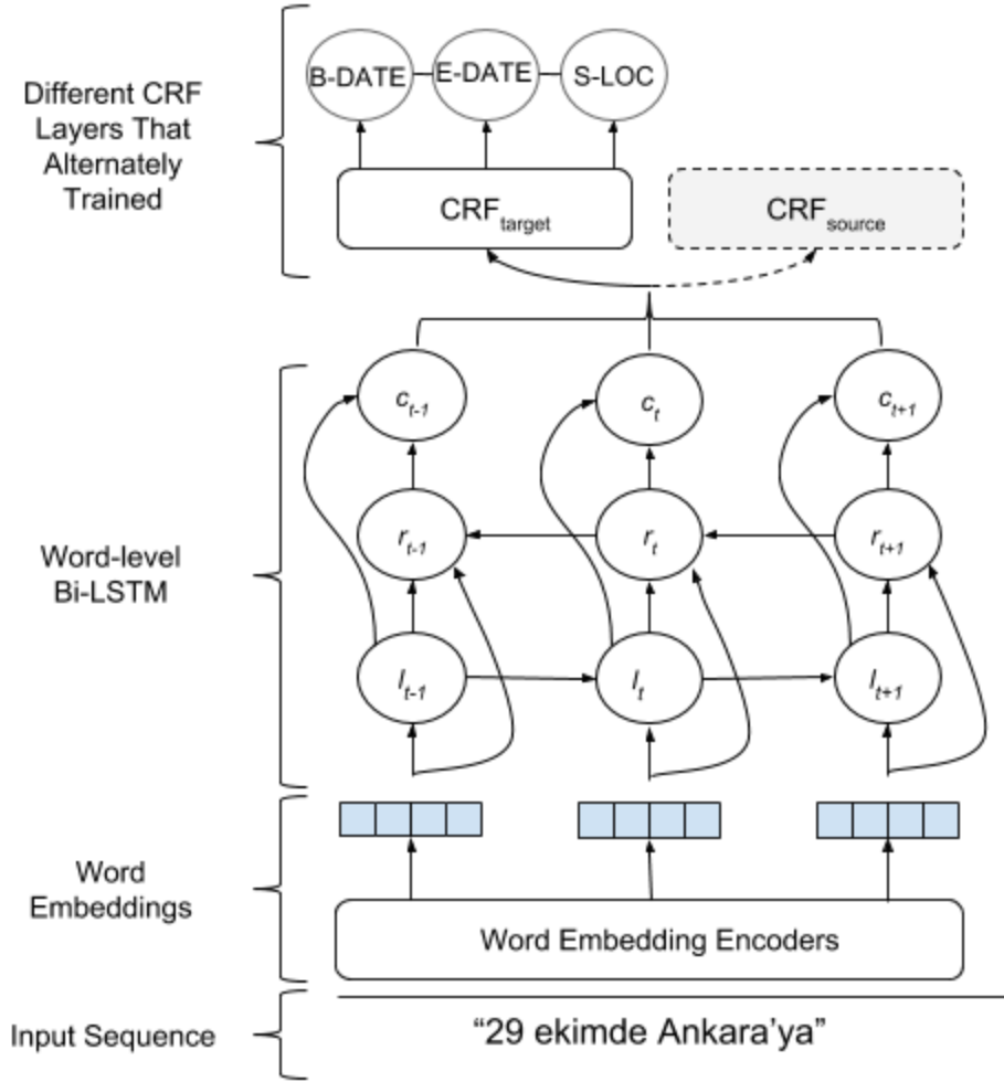
FIGURE 4.7. Overview of the initial transfer learning model which incorporates additional CRF layer. CRF layers are alternately trained on different datasets so that the shared layers learn from both datasets and, therefore, learning can be transferred from source dataset to target dataset.
