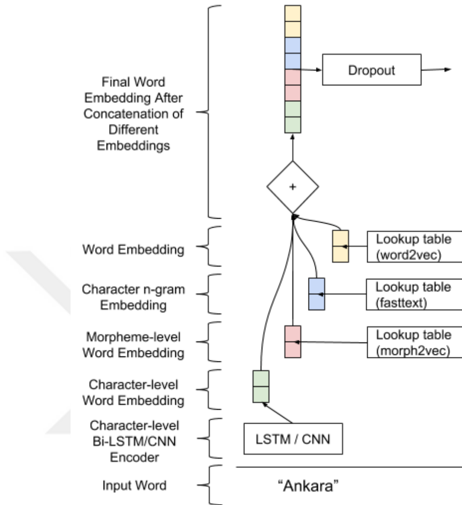
FIGURE 4.1. Overview of the final word embeddings. After concatenating embeddings obtained from fasttext , word2vec , morph2vec and orthographic character-level embeddings, we also apply dropout for better generalization and consequently, obtain the final word embedding for a word.
