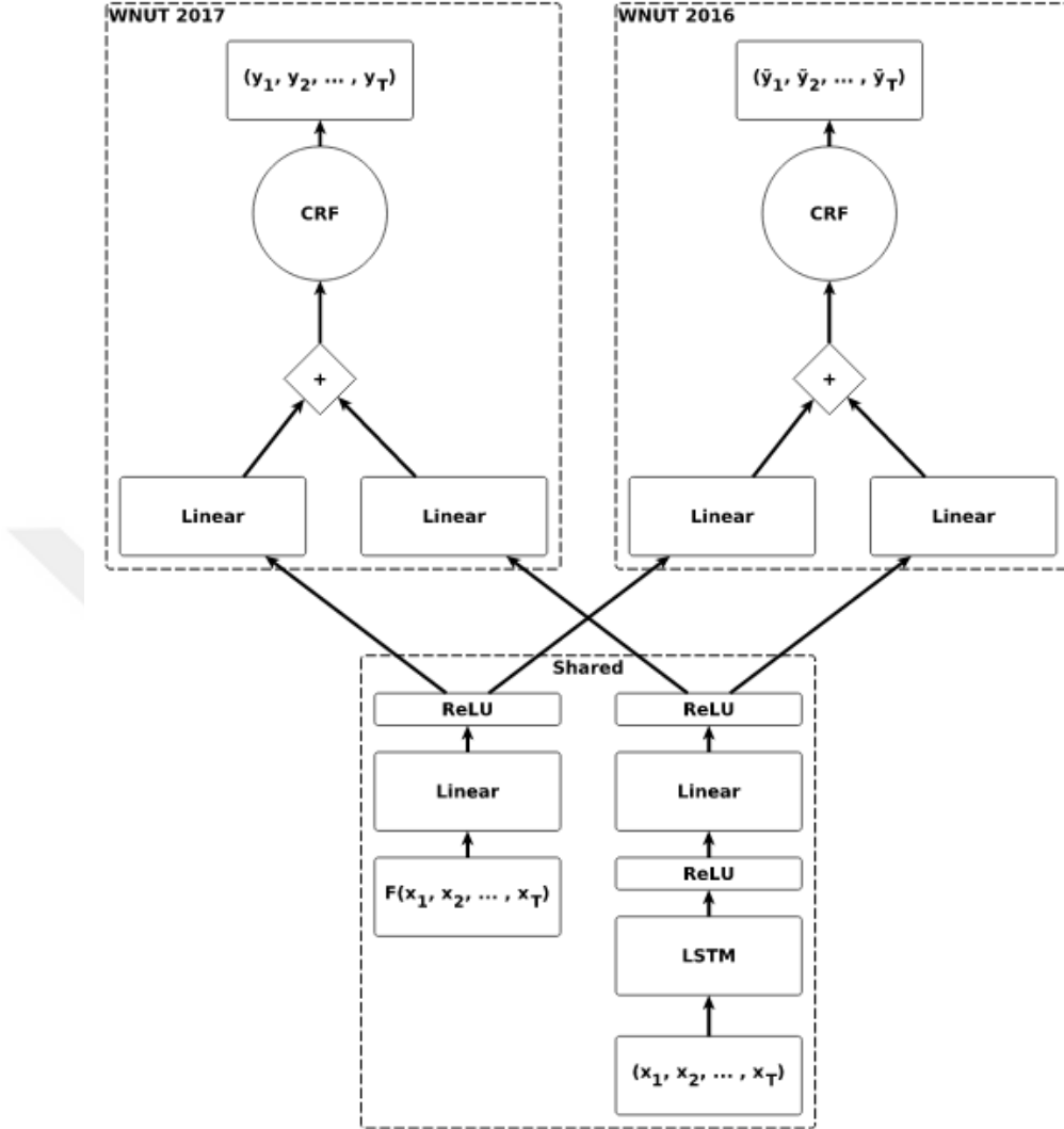
FIGURE 3.4. Architecture of Transfer Learning in a BiLSTM-CRF network [43]
