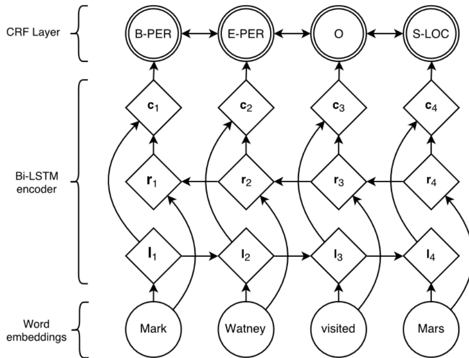
FIGURE 3.2. Overview of the BiLSTM-CRF model [4]
