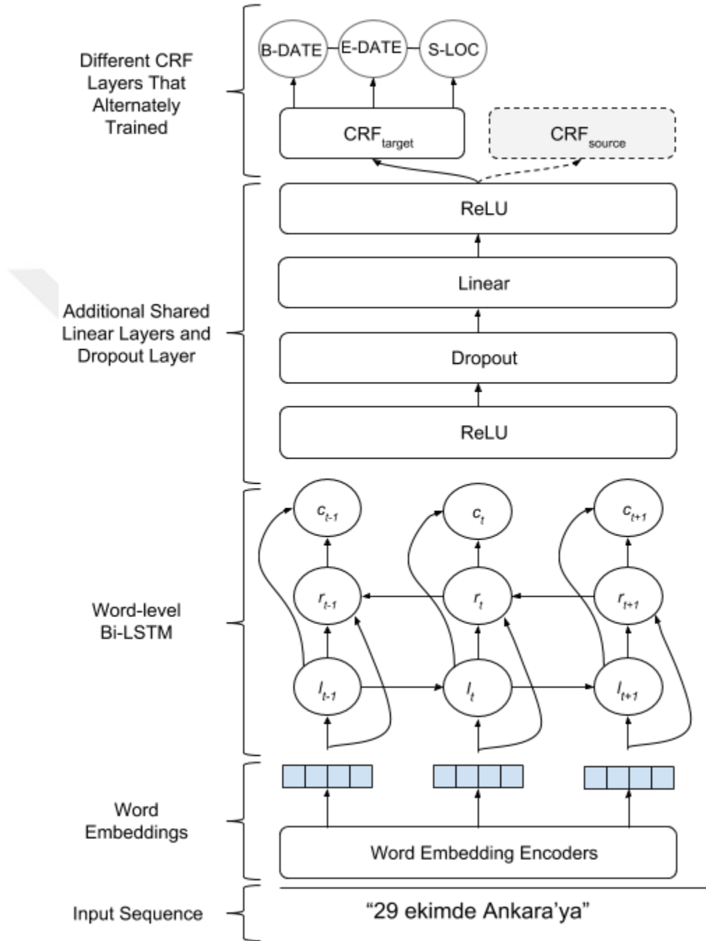
FIGURE 4.8. Overview of the final transfer learning model which incorporates additional CRF layer and additional linear and ReLU layer to further improve model performance.
