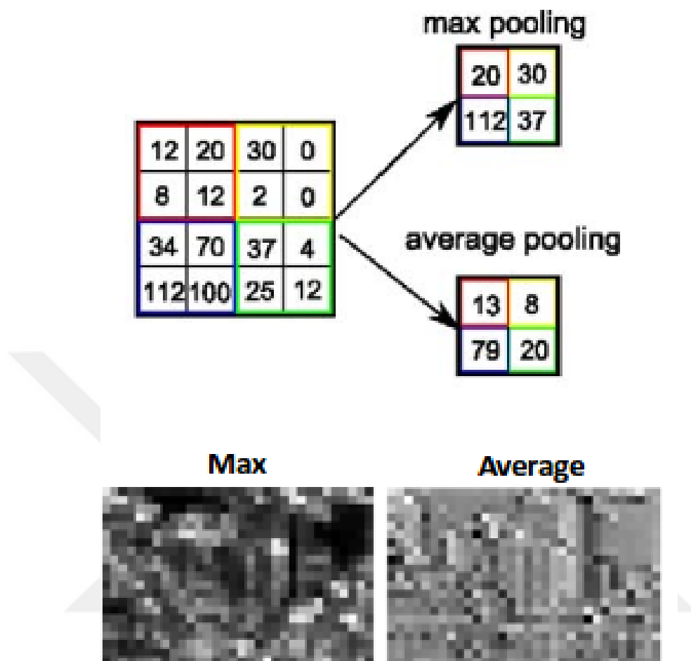
FIGURE 2.9. An example of difference between max pooling and average pooling
