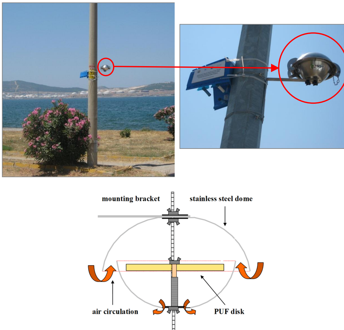
Figure 3.4 A PUF passive air sampler used in this study.
