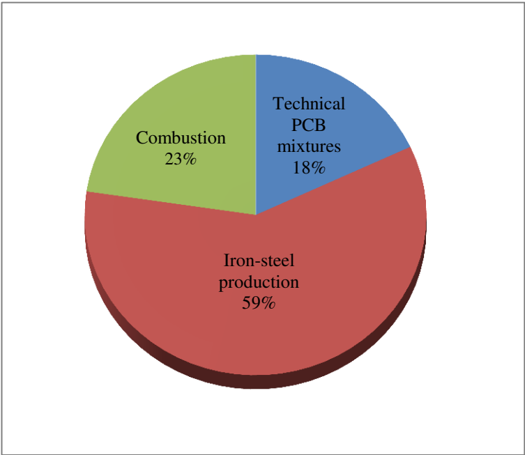
Figure 4.18 Source contributions to the total PCB concentrations.
