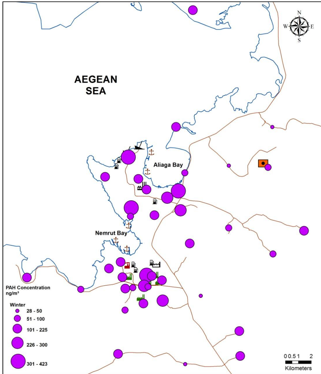
Figure 4.5 The spatial distribution of total ambient air PAH concentrations ( \text{ng m}^{-3} ) for winter.
