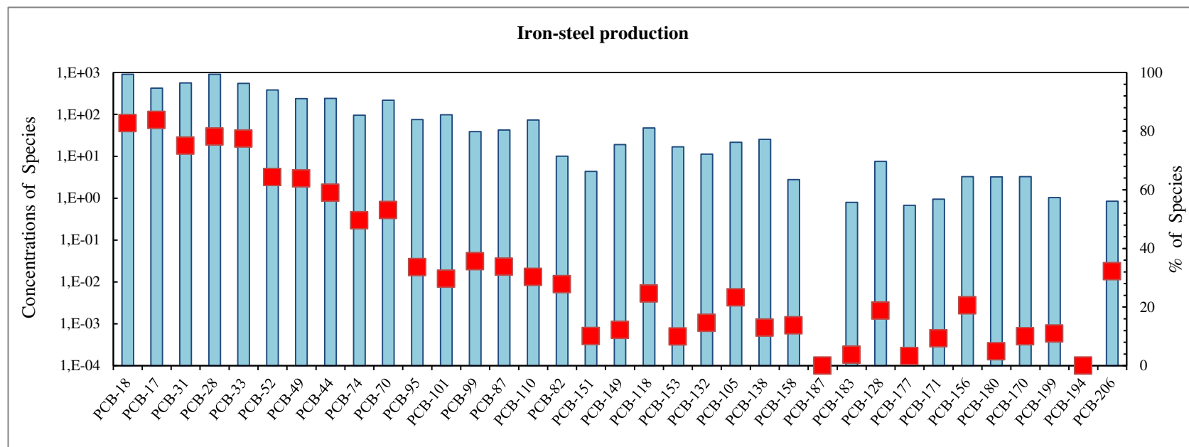
Figure 4.20 PMF profile of factor 1 for PCBs.
