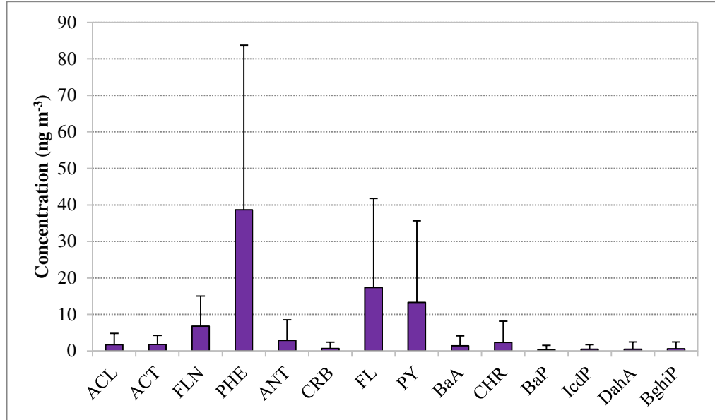
Figure 4.2 Overall average concentrations ( \text{ng m}^{-3} ) of individual PAHs including all sites and seasons. Error bars indicate 1 SD.
