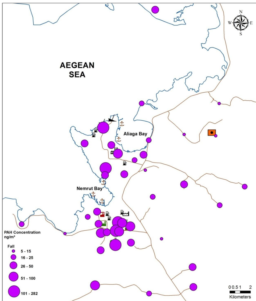
Figure 4.4 The spatial distribution of total ambient air PAH concentrations ( \text{ng m}^{-3} ) for fall.
