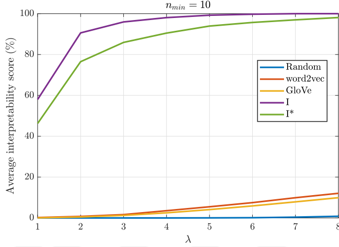
Figure 2.9: Average interpretability scores of four Turkish embedding spaces along with a random baseline for n_{min} = 10 and \lambda \in \{1, 2, \dots, 8\} .
