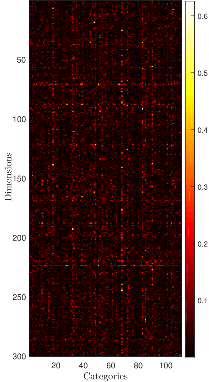
Figure 2.2: Semantic category weights ( \mathcal{W}_B_{300 \times 110} ) for 110 categories and 300 embedding dimensions obtained using Bhattacharya distance. Weights vary between 0 (represented by black) and 0.63 (represented by white). It can be noticed that some dimensions represent larger number of categories than others do and also some categories are represented strongly by more dimensions than others.
