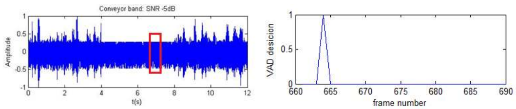
Figure 5.12 Non-speech decision of G.729 VAD with -5db SNR
