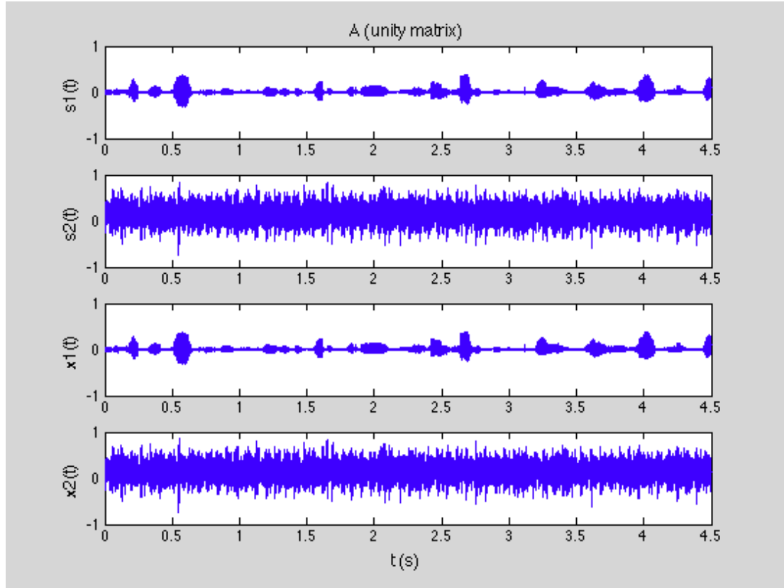
Figure 3.3 The sources and observations according to the unity matrix of A
