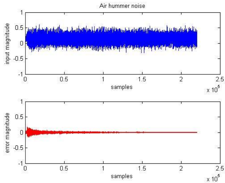
Figure 5.15 Time domain representation of input and error signal of air hammer sound with Fx-LMS algorithm
