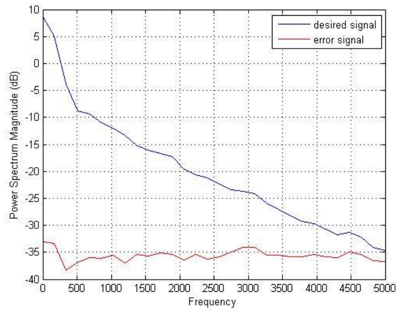
Figure 5.18 Frequency domain representation of input and error signal of ambiance sound with Fx-LMS algorithm
