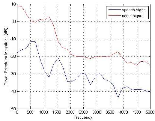
Figure 5.23 The PSD of two source signals
