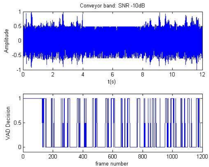
Figure 5.10 G.729 VAD with conveyor band sound examples in -10db SNR
