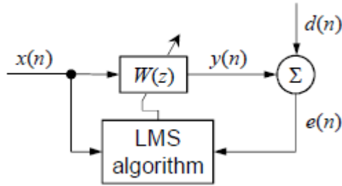
Figure 4.2 LMS algorithm block diagram (Kataja, 2012)
