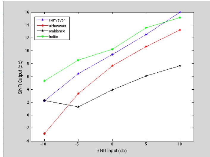
Figure 5.26 Comparison of SNR performance between input and output
