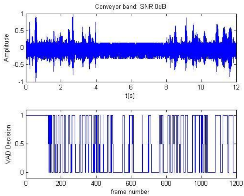
Figure 5.8 G.729 VAD with conveyor band sound examples in 0db SNR
