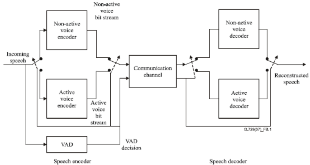
Figure 2.7 Speech coding with VAD in DTX (ITU-T Series G: Transmission Systems and Media, Digital Systems and Networks. Digital terminal equipments-Coding of voice and audio signals, 2012)
