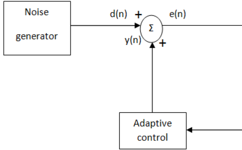
Figure 4.9 Feedback ANC block diagram
