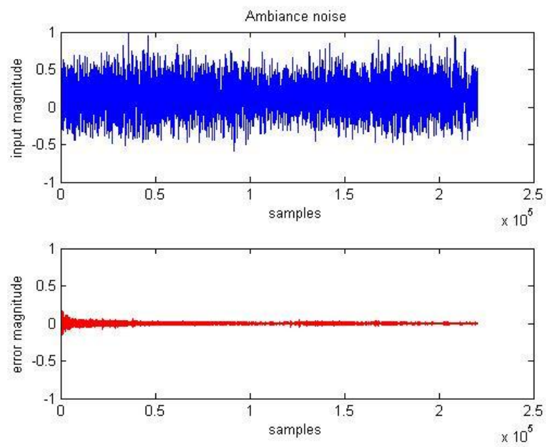
Figure 5.17 Time domain representation of input and error signal of ambiance sound with Fx-LMS algorithm
