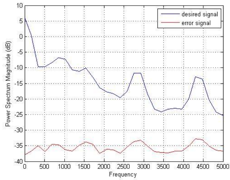
Figure 5.14 Frequency domain representation of input and error signal of conveyor band sound with Fx-LMS algorithm
