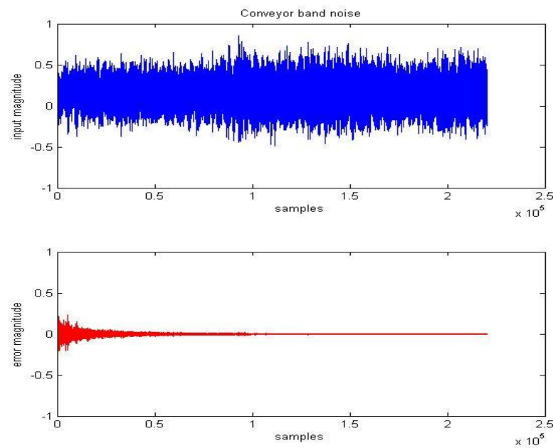
Figure 5.13 Time domain representation of input and error signal of conveyor band sound with Fx-LMS algorithm
