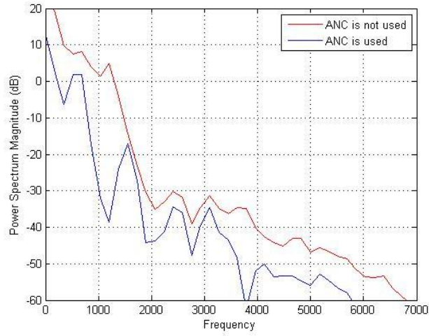
Figure 5.24 The PSD of signals at the system output when ANC is used or not.
