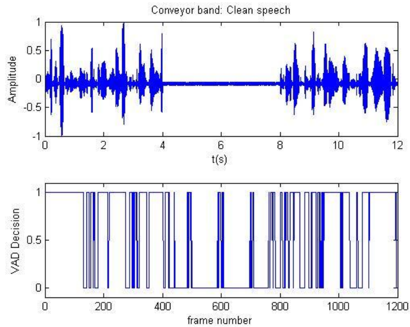
Figure 5.5 G.729 VAD with conveyor band sound examples in clean speech
