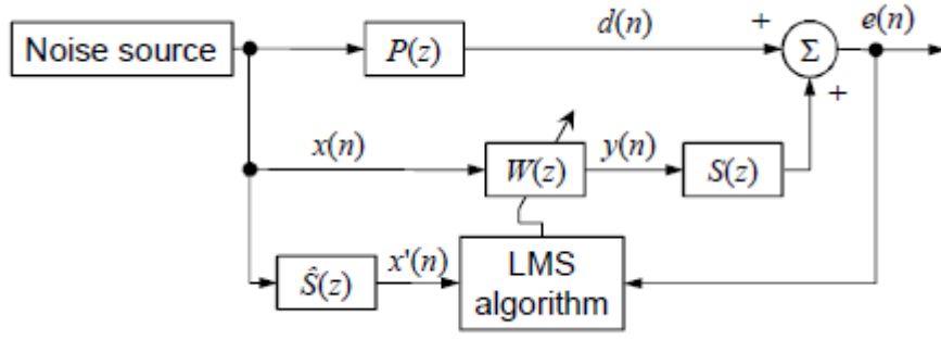
Figure 4.5 Fx-LMS algorithm block diagram (Kataja, 2012)
