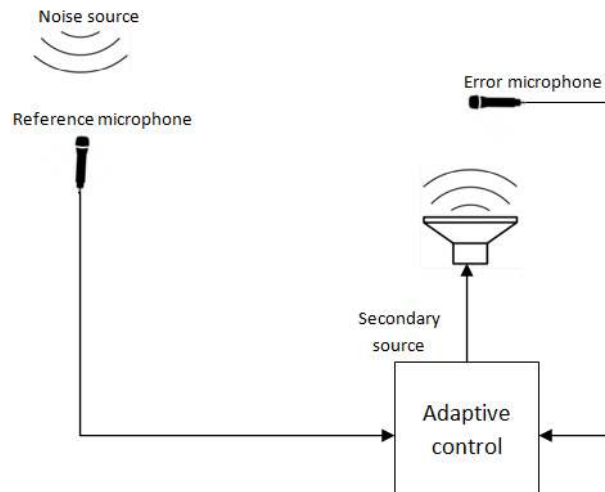
Figure 4.6 Feedforward ANC system
