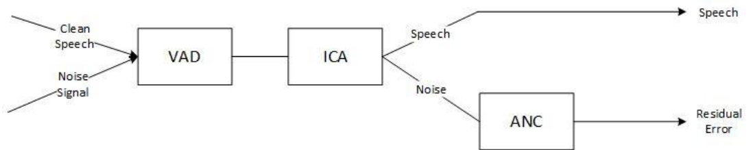
Figure 5.25 Block diagram of the proposed system
