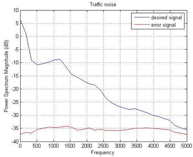
Figure 5.20 Frequency domain representation of input and error signal of traffic sound with Fx-LMS algorithm
