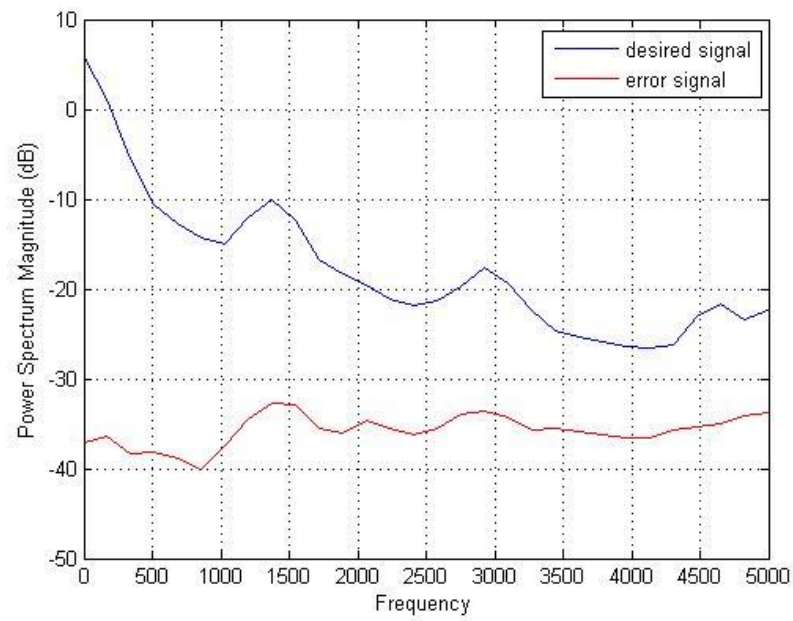
Figure 5.16 Frequency domain representation of input and error signal of air hammer sound with Fx-LMS algorithm
