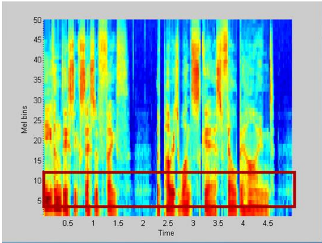
Figure 2.5 Selected bins of mel-frequency spectrogram
