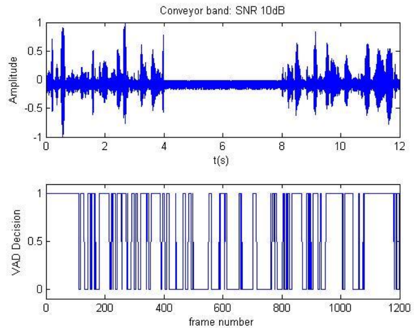
Figure 5.6 G.729 VAD with conveyor band sound examples in 10db SNR
