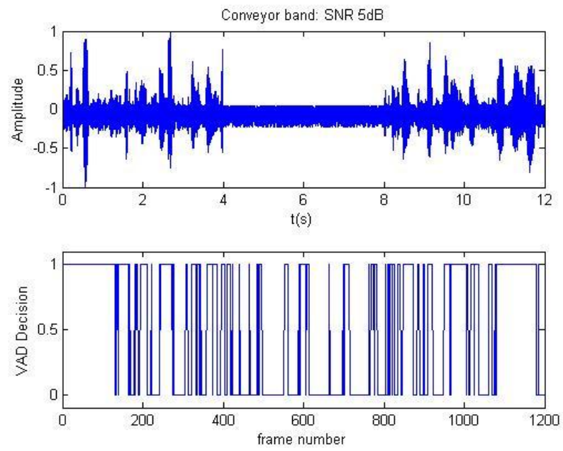
Figure 5.7 G.729 VAD with conveyor band sound examples in 5db SNR
