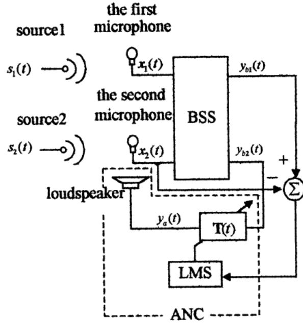
Figure 4.10 Proposed ANC system for selective attention (Sohn & Lee, 2000)
