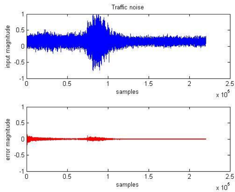
Figure 5.19 Time domain representation of input and error signal of traffic sound with Fx-LMS algorithm
