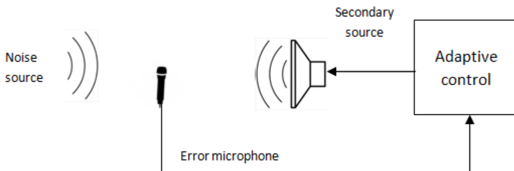
Figure 4.8 Feedback ANC system
