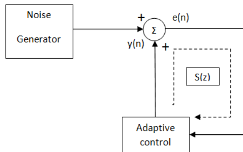
Figure 4.4 Model of transfer functions of the secondary path
