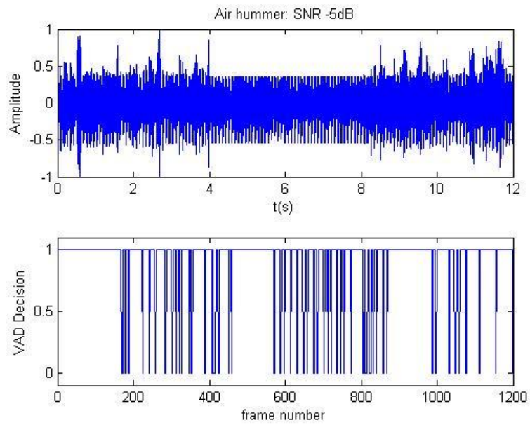
Figure 5.2 G.729 VAD with air hammer noise examples in -5db SNR
