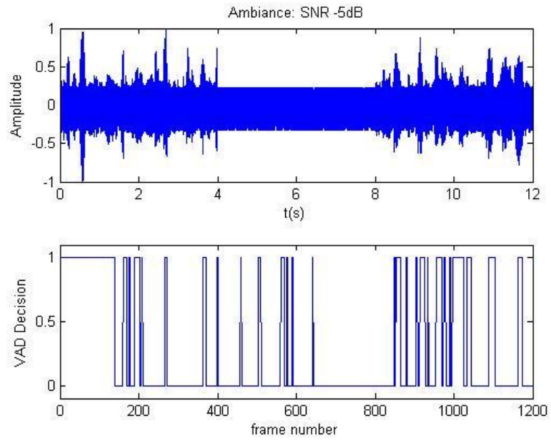
Figure 5.3 G.729 VAD with ambient noise examples in -5db SNR
