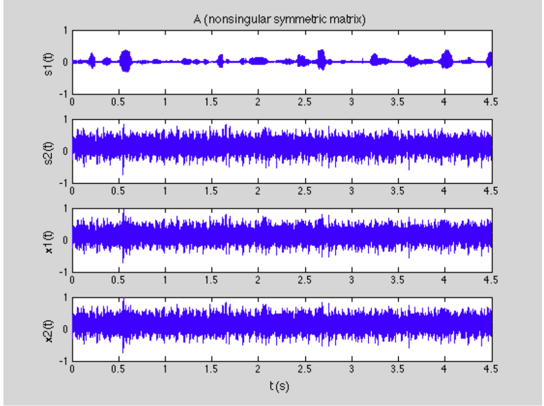
Figure 3.4 The sources and observations according to the nonsingular symmetric matrix of A
