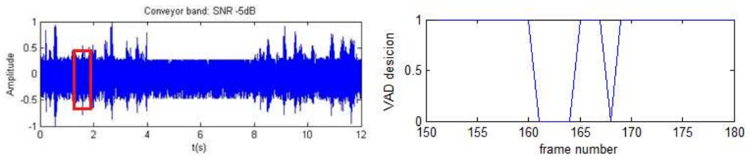
Figure 5.11 Speech decision of G.729 VAD with in -5db SNR
