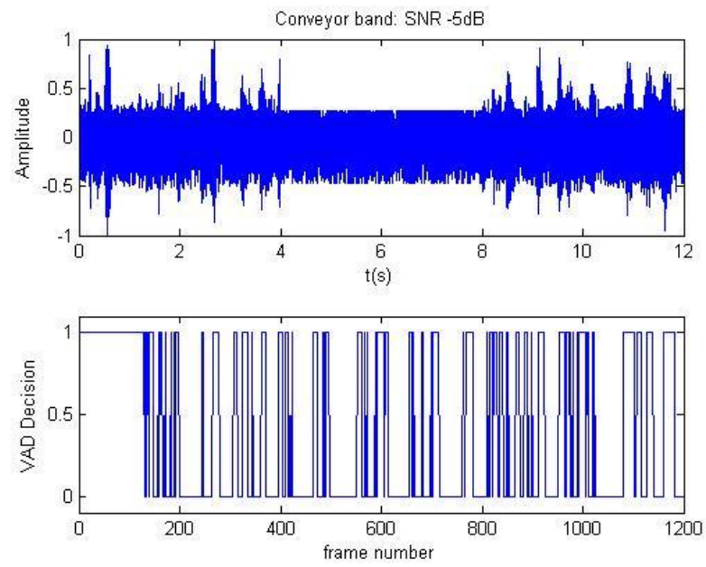
Figure 5.9 G.729 VAD with conveyor band sound examples in -5db SNR
