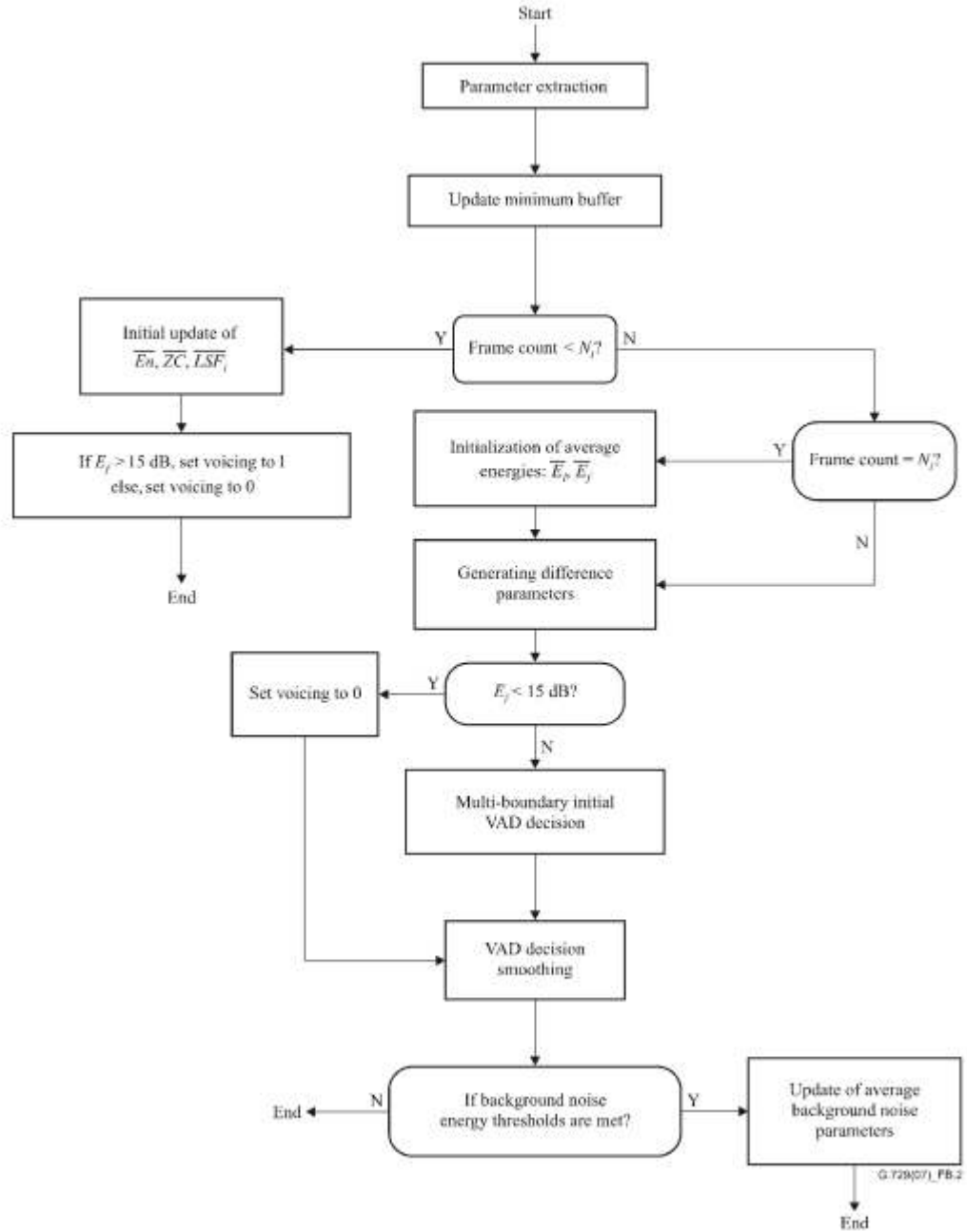
Figure 2.8 VAD flowchart (ITU-T Series G: Transmission Systems and Media, Digital Systems and Networks. Digital terminal equipments-Coding of voice and audio signals, 2012).
