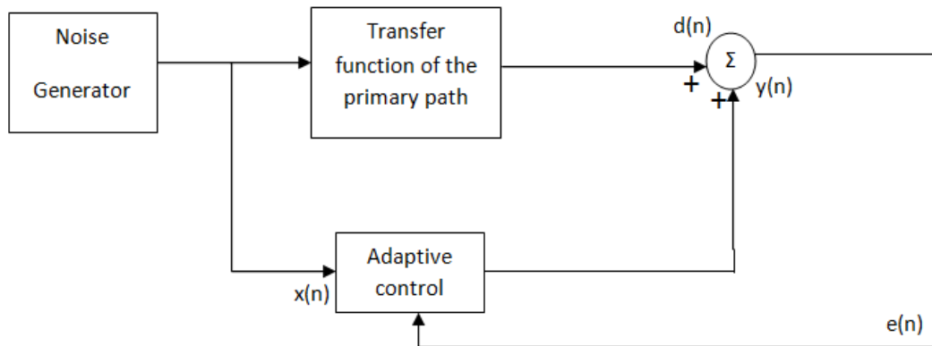
Figure 4.7 Feedforward ANC block diagram
