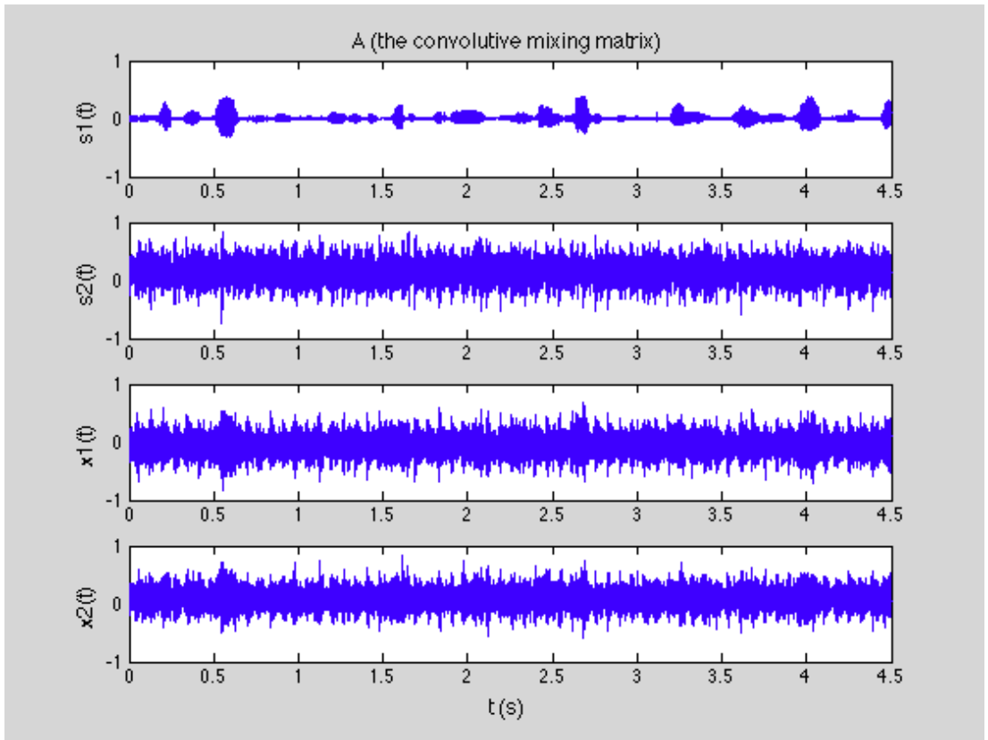
Figure 3.5 The sources and observations according to the convolutive mixing matrix of A
