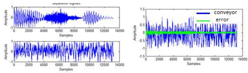
Figure 5.21 The output of blocks if the VAD returns '1'
