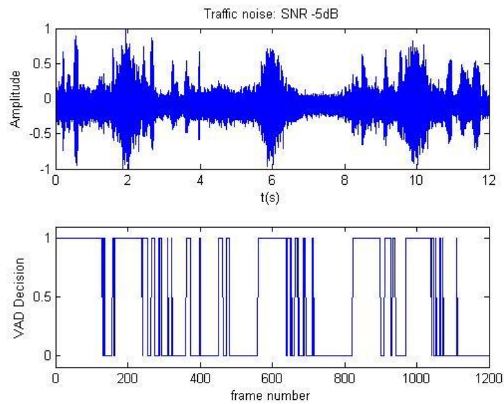
Figure 5.4 G.729 VAD with traffic noise examples in -5db SNR
