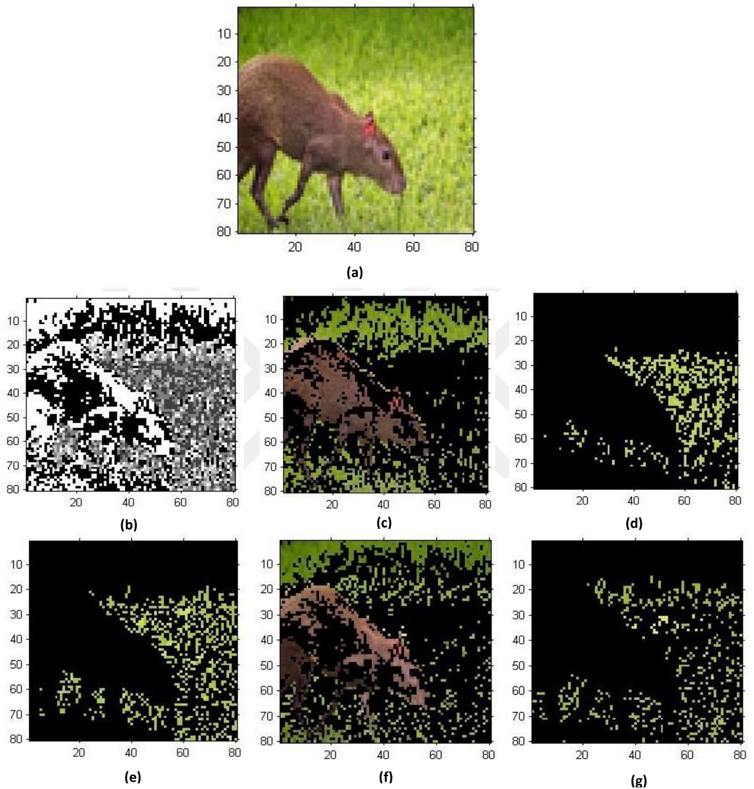
Figure 13. (a) Original Image (b) labeled image Using cluster index (c) Segmented Image (d) Segmented Image (e) segmented Image (f) Segmented Image (g) Segmented Image. The spectral clustering algorithm has been applied to the color image (RGB) without changing to any other space and these results at kmean=5 .
