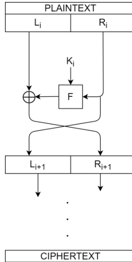
Figure 1.2: Feistel Network
