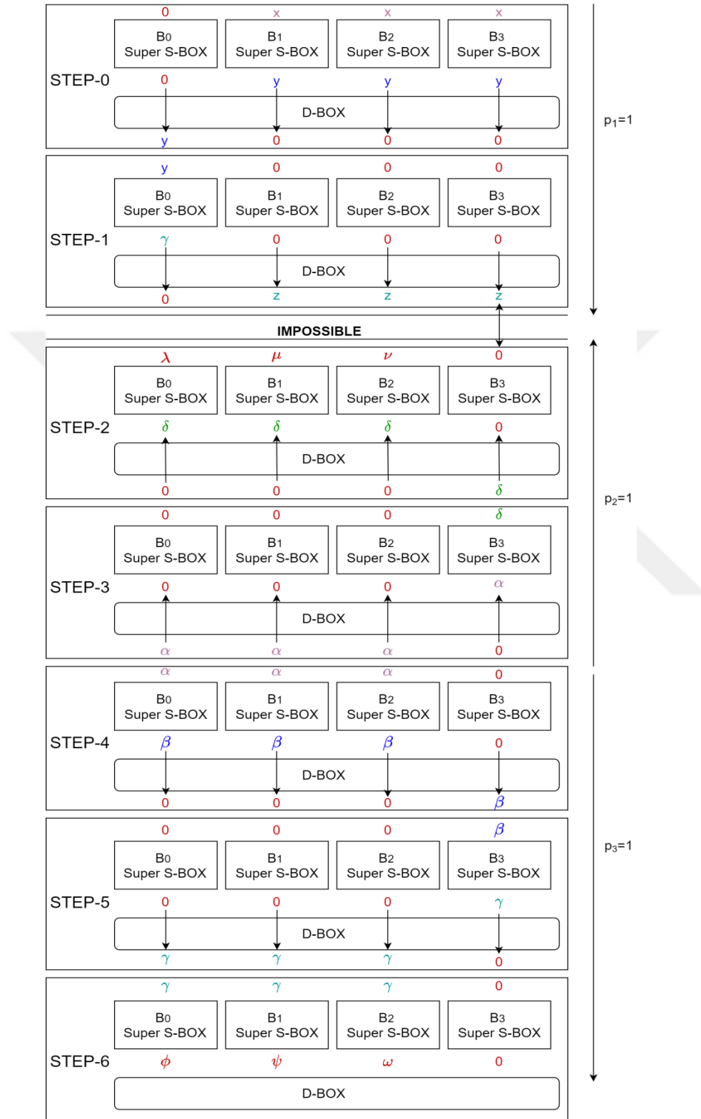
Figure 4.3: 7-Step Impossible Differential Distinguisher of Shadow-512
