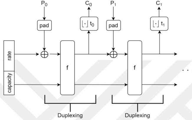
Figure 1.3: Duplex Construction
