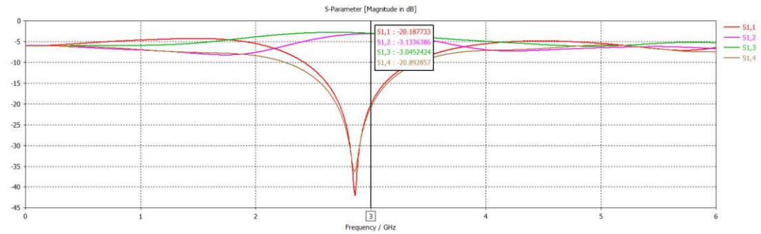
Figure 5.5: Magnitude of the first row of the scattering matrix at the operational frequency for the strip line hybrid
