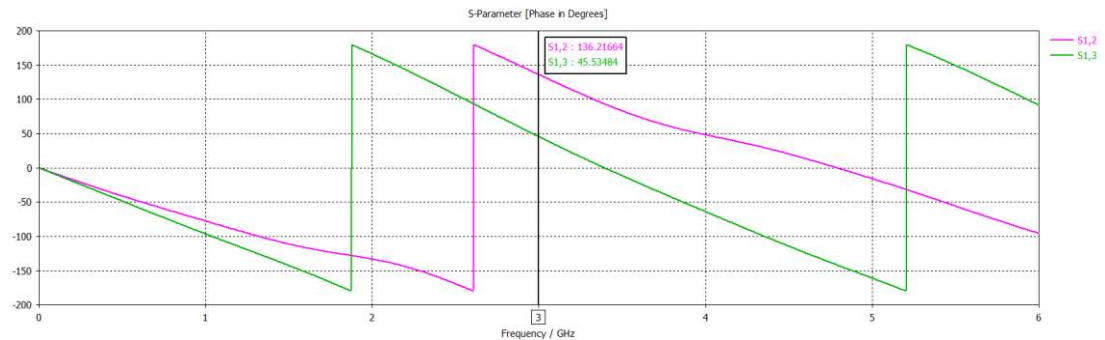
Figure 5.6: Phase shift between S_{12} and S_{13} at the operating frequency for the strip line hybrid
