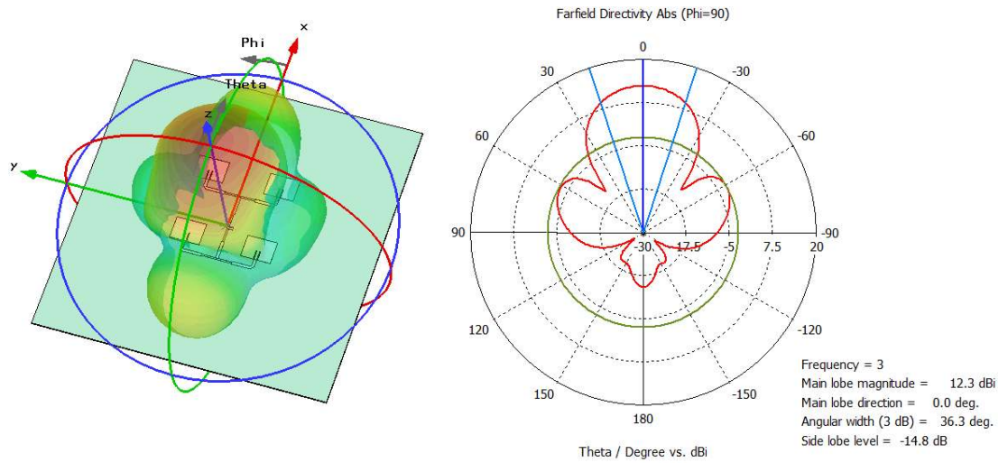
Figure 4.17: Radiation pattern for the 2 by 2 conventional array
