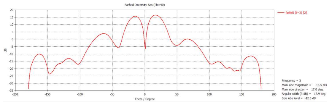
Figure 5.15: 2-D difference pattern in \phi=90^\circ plane
