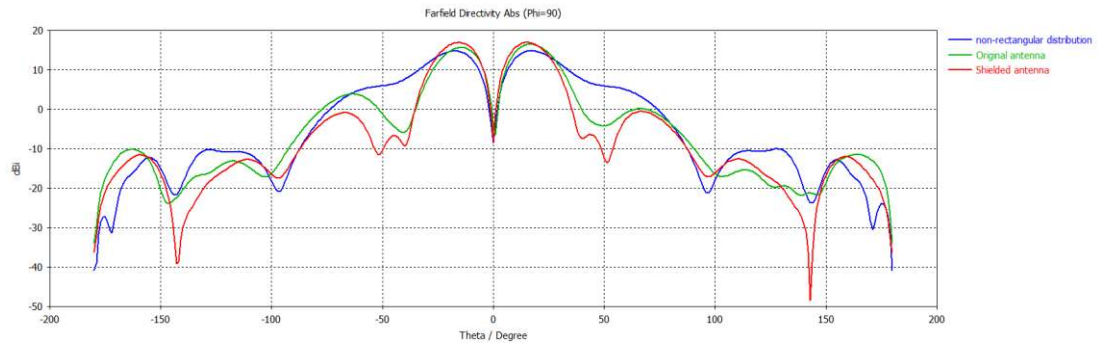
Figure 5.31: 2-D difference pattern in \phi=90^\circ plane for the non-rectangular shielded antenna
