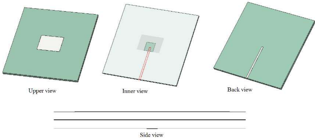
Figure 3.6: Aperture coupling
