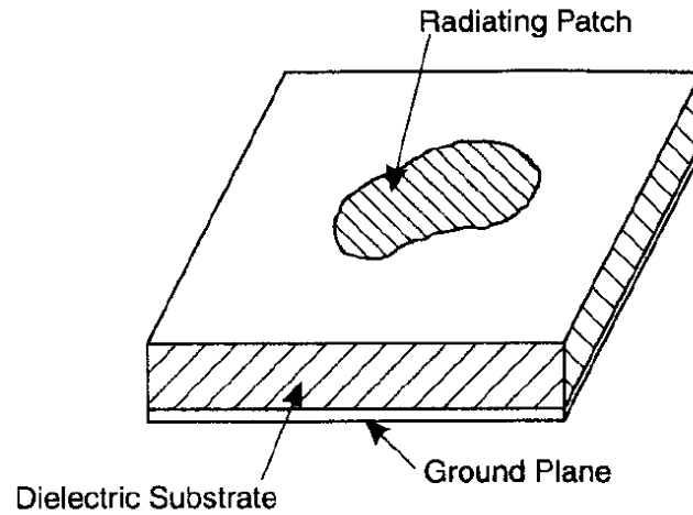
Figure 3.1: Microstrip antenna basic structure [21]
