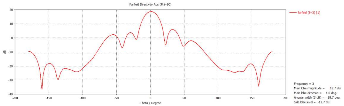
Figure 5.13: 2-D sum pattern in \phi=90^0 plane
