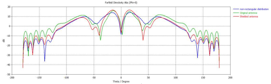
Figure 5.30: 2-D difference pattern in \phi=0^\circ plane for the non-rectangular shielded antenna
