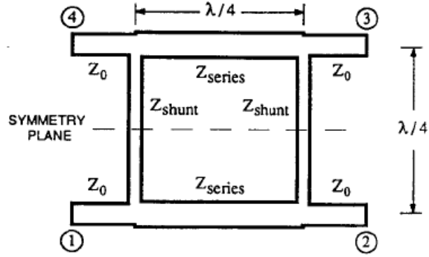
Figure 3.19: 90° Hybrid microstrip coupler [25]
