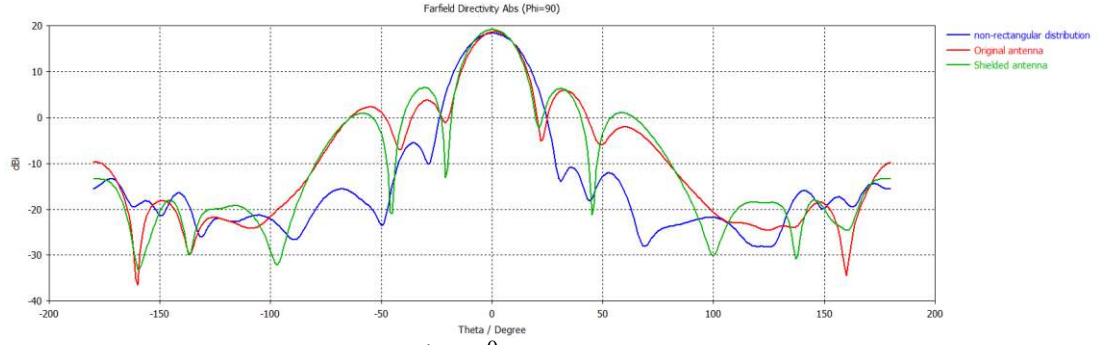
Figure 5.29: 2-D sum pattern in \phi=90^\circ plane for the non-rectangular shielded antenna
