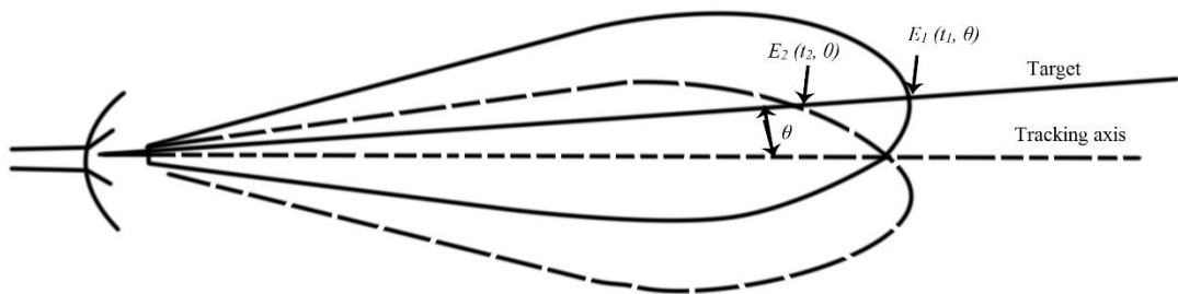
Figure 2.1: Sequential lobing
