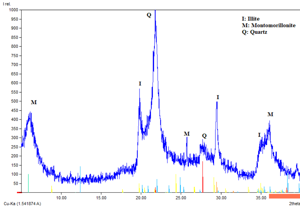
Figure 2.4. X-ray analysis of soil
