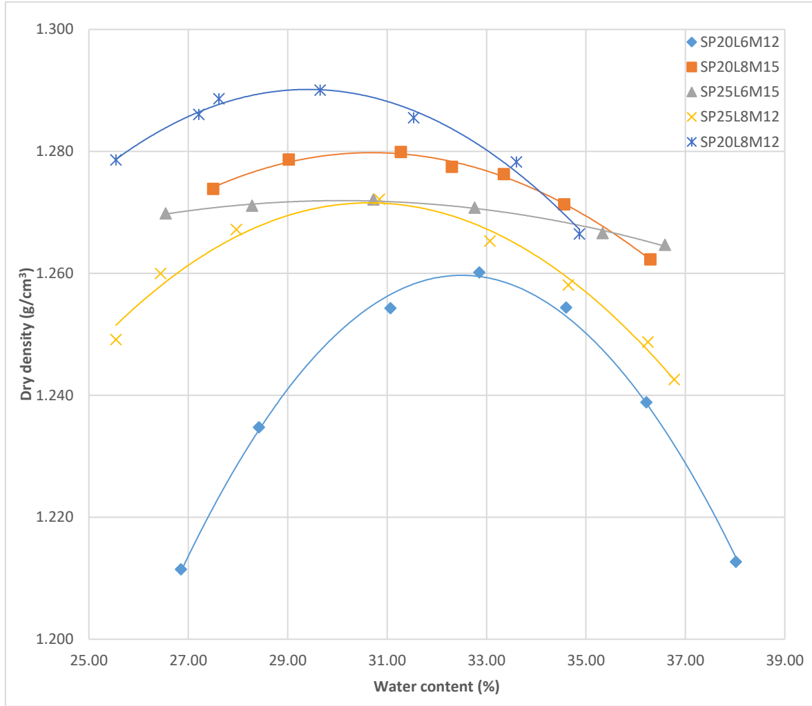
Figure 3.15. Compaction curves for mixtures
