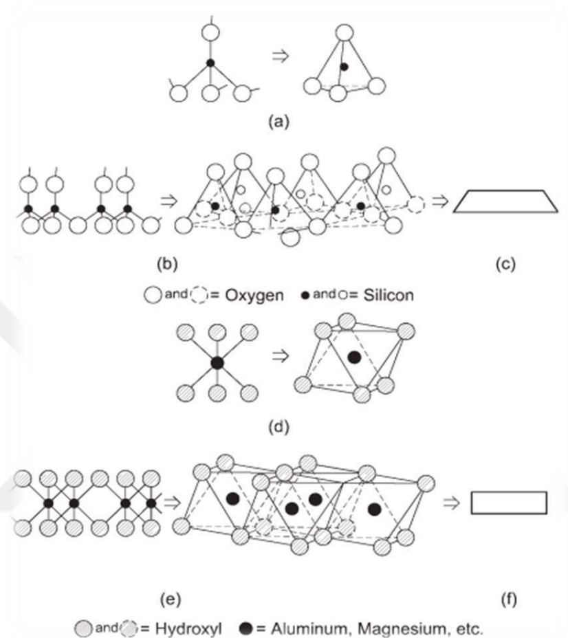
Figure 1.1. Atomic structure of silicon tetrahedra and aluminomagnesium octahedra: (a) silicon tetrahedron; (b) silica sheet; (c) symbolic structure for silica sheet; (d) aluminomagnesium octahedron; (e) octahedral sheet; (f) symbolic structure for octahedral sheet (after Lambe and Whitman, 1969).
