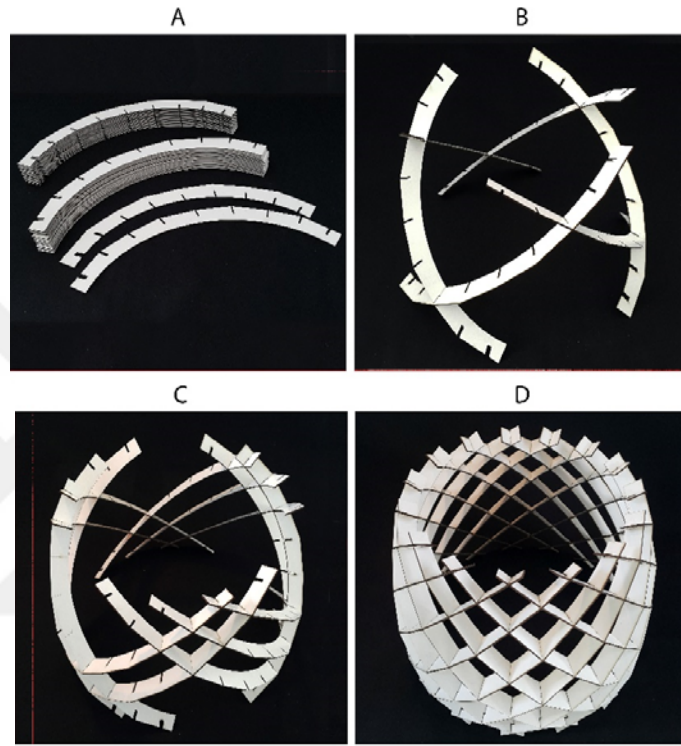
Figure 61. Assembly process (Image created by the author).
