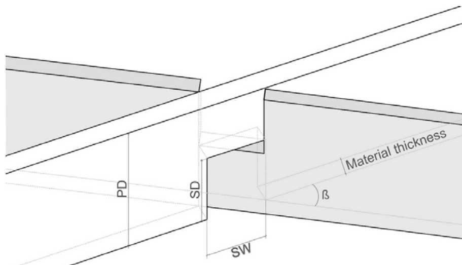
Figure 60. Slit formation detail (Image created by the author).
