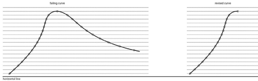
Figure 59. Horizontal Line Test (Image created by the author).
