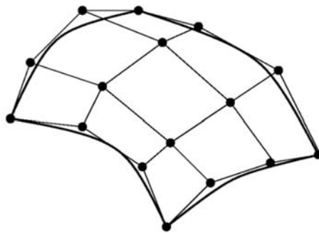
Figure 21. An example of a 2 nd -degree Bezier surface with control points (Segarsa, Mahesh, Beck, Frey, & Tsui, 2008, p. 3802).
