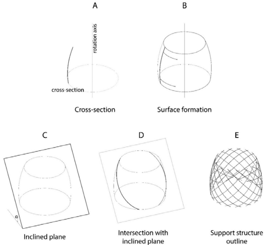
Figure 58. Formation process (Image created by the author).
