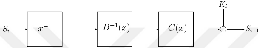
Figure 4.1: One round of the JARVIS block cipher
