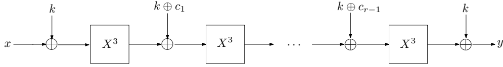
Figure 5.1: r rounds of the MiMC- n/n block cipher
