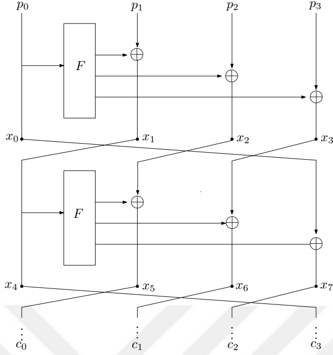
Figure 6.2: Introducing new intermediate variables x_{4(i-1)}, x_{4(i-1)+1}, x_{4(i-1)+2}, x_{4(i-1)+3} for r rounds of GMiMC erf where 1 \leq i \leq r with branch number t = 4 .
