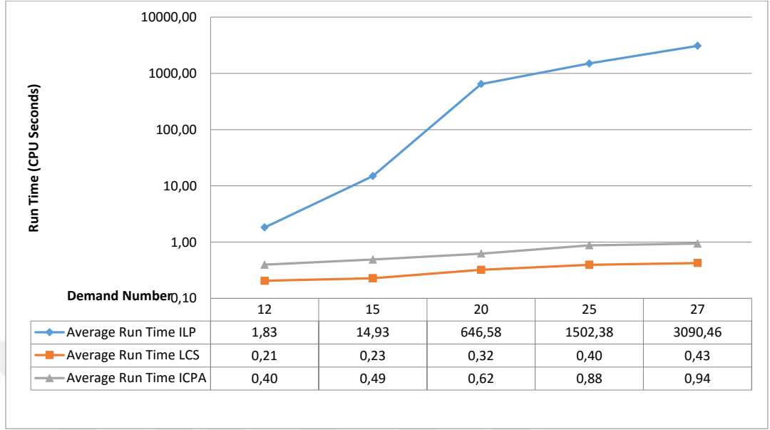
Figure 5.10: Average run time of ILP Formulation and Heuristic Algorithms for traffic loads of 12, 15, 20, 25 and 27 commodities.
