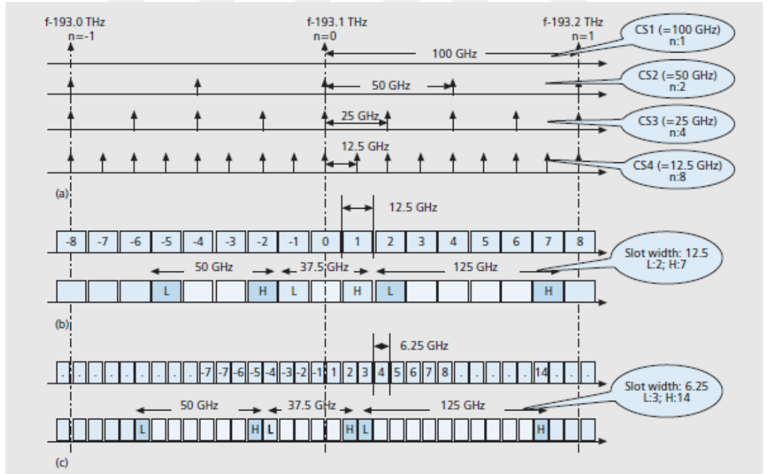
Figure 1.4: Comparison of frequency grid slot divisions. a) Current ITU-T DWDM frequency grid. b) single slot approach. c) double-sided half slot approach.[4]
