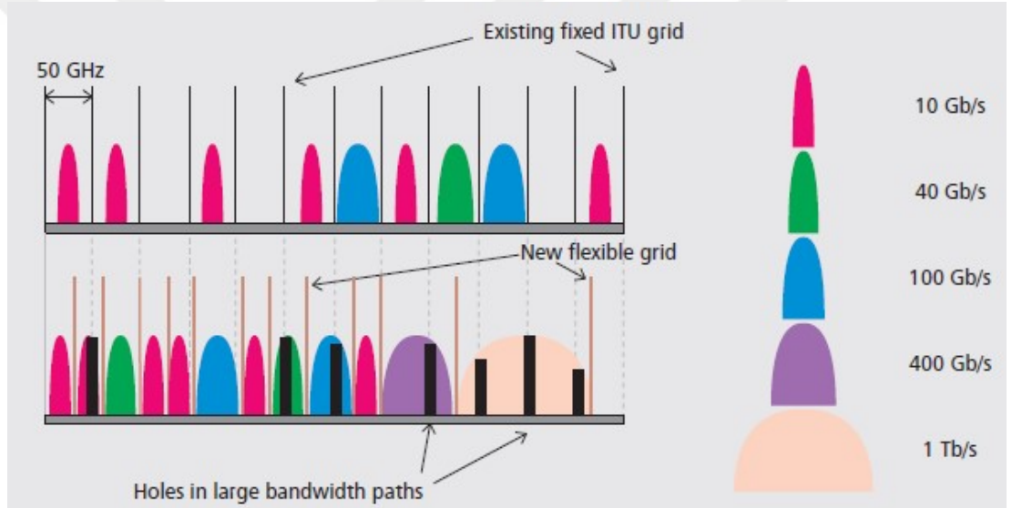
Figure 1.3: Bandwidth allocation in existing fixed ITU grid versus in flexible grid.[3]
