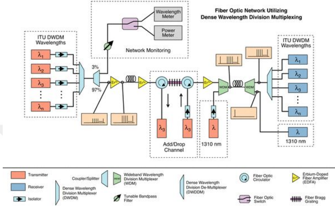
Figure 1.2: Components of a fiber optic network.[2]
