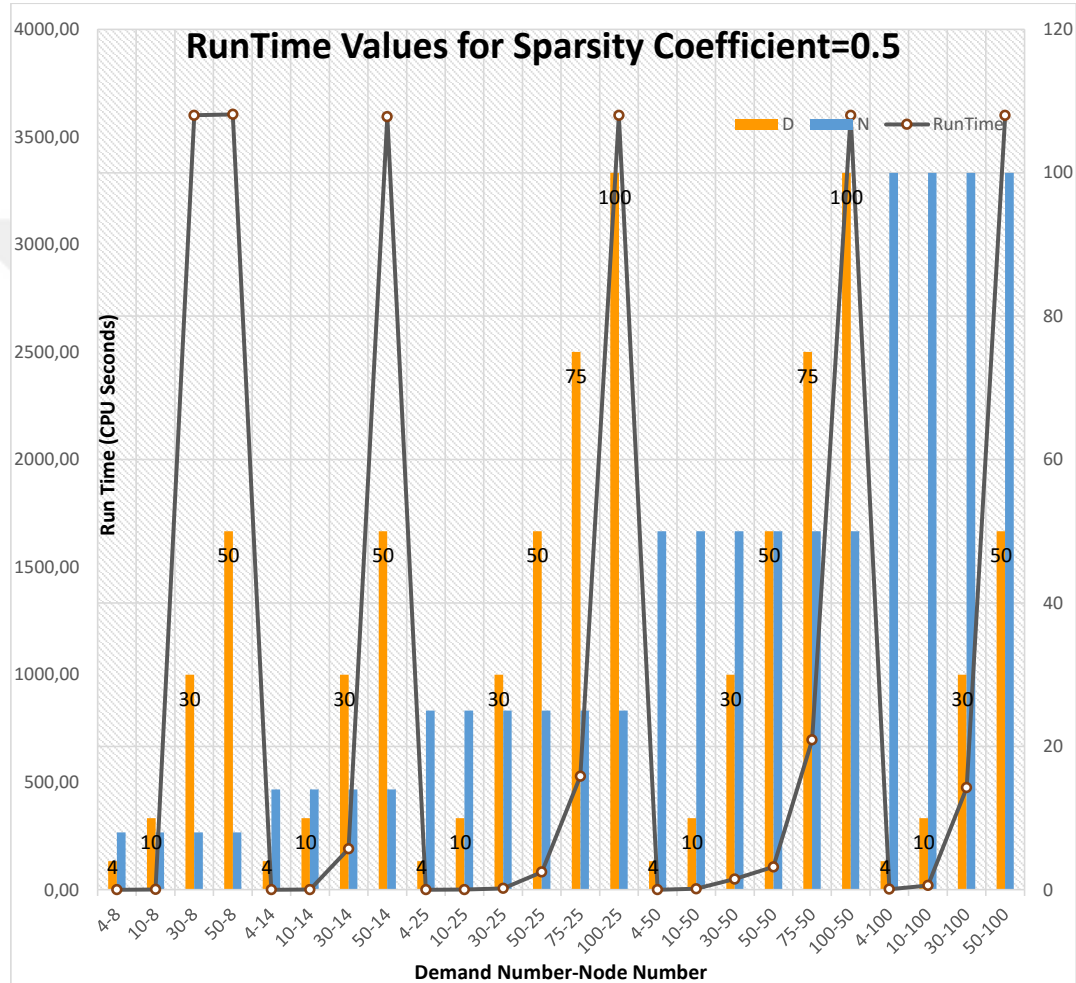
Figure 5.7: Effects of increasing connection requests on run time values at various network topologies for sparsity coefficient of 0.5
