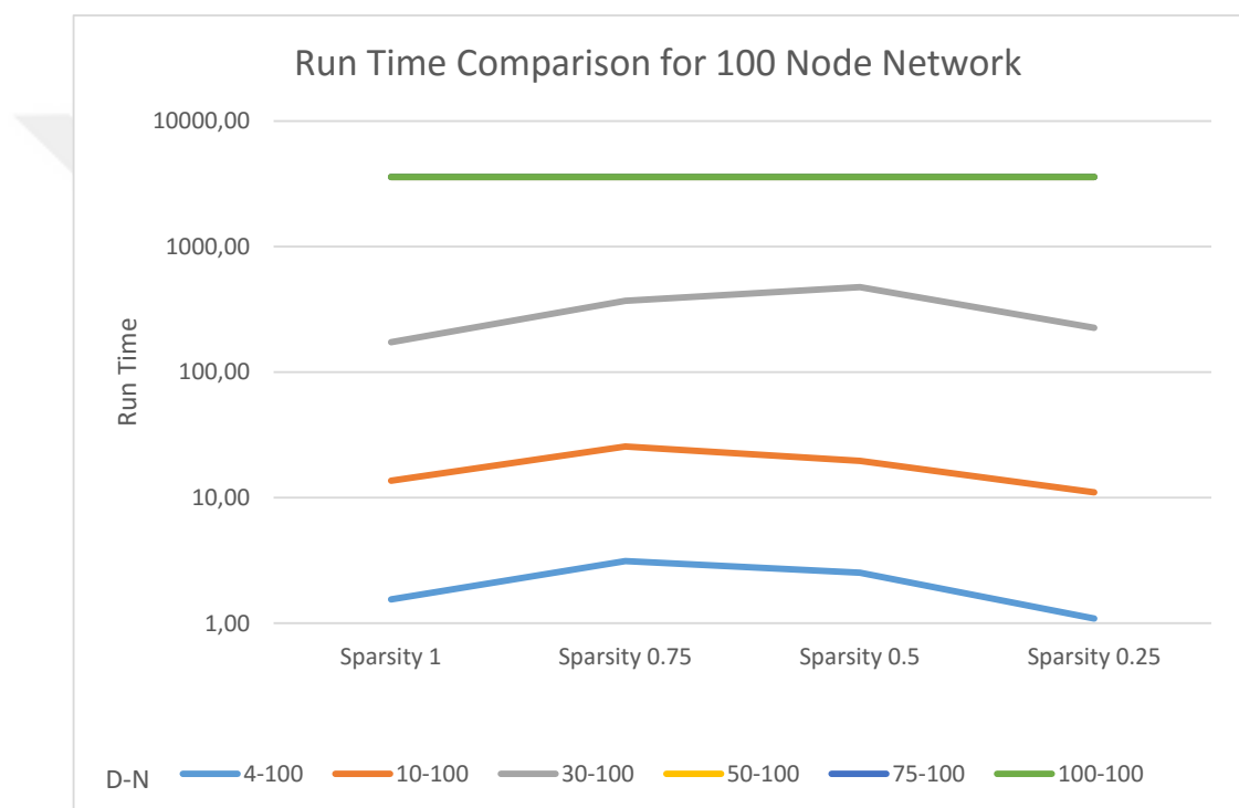
Figure 5.4: Run Time Comparison of Different Sparsity Coefficients for Large Networks Consisting of 100 Nodes
