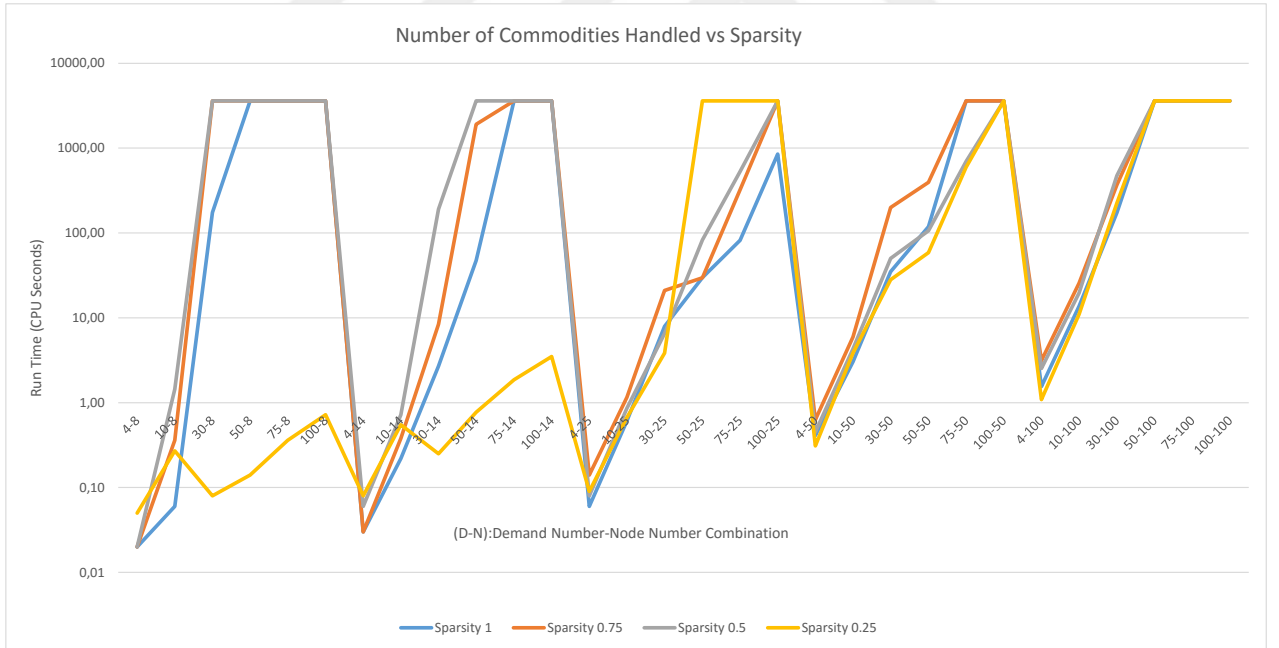
Figure 5.1: Trend of Run Time Values for Demand Number-Node Number vs Sparsity Combinations
