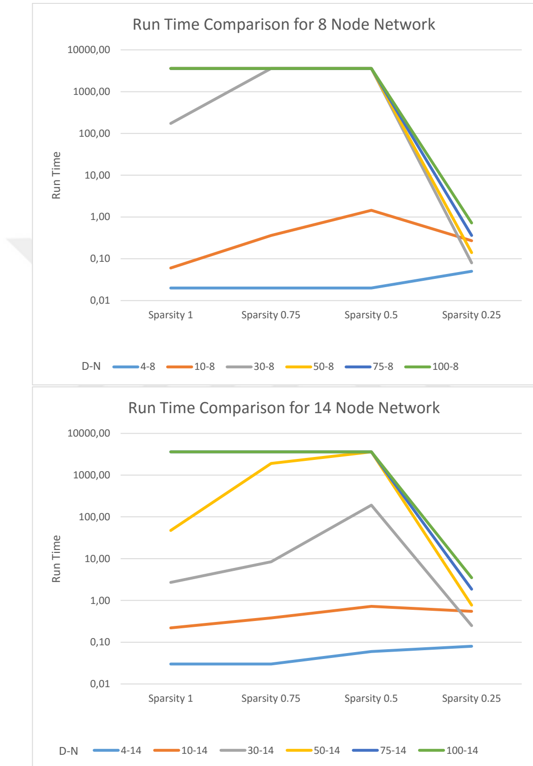
Figure 5.2: Run Time Comparison of Different Sparsity Coefficients for Small Networks Consisting of 8 and 14 Nodes 49
