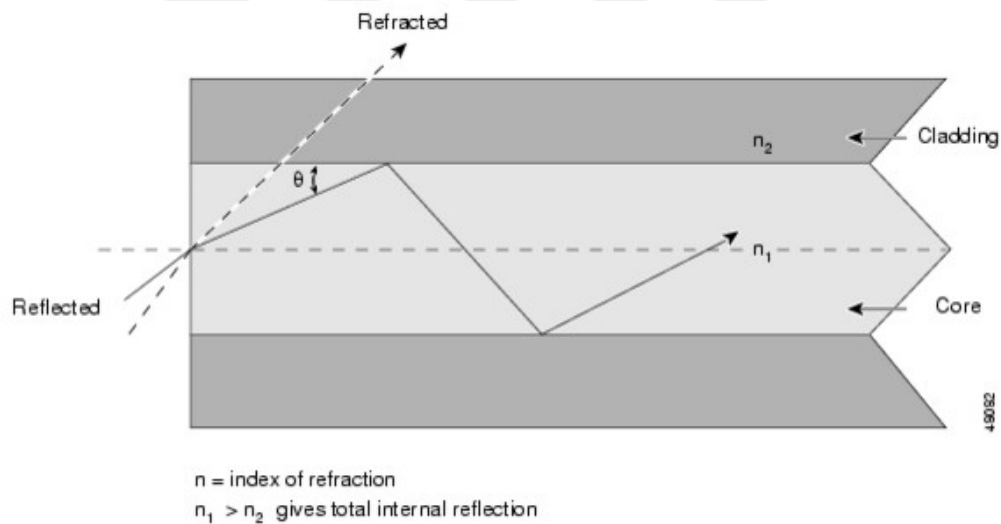
Figure 1.1: Principle of total internal reflection.[1]
