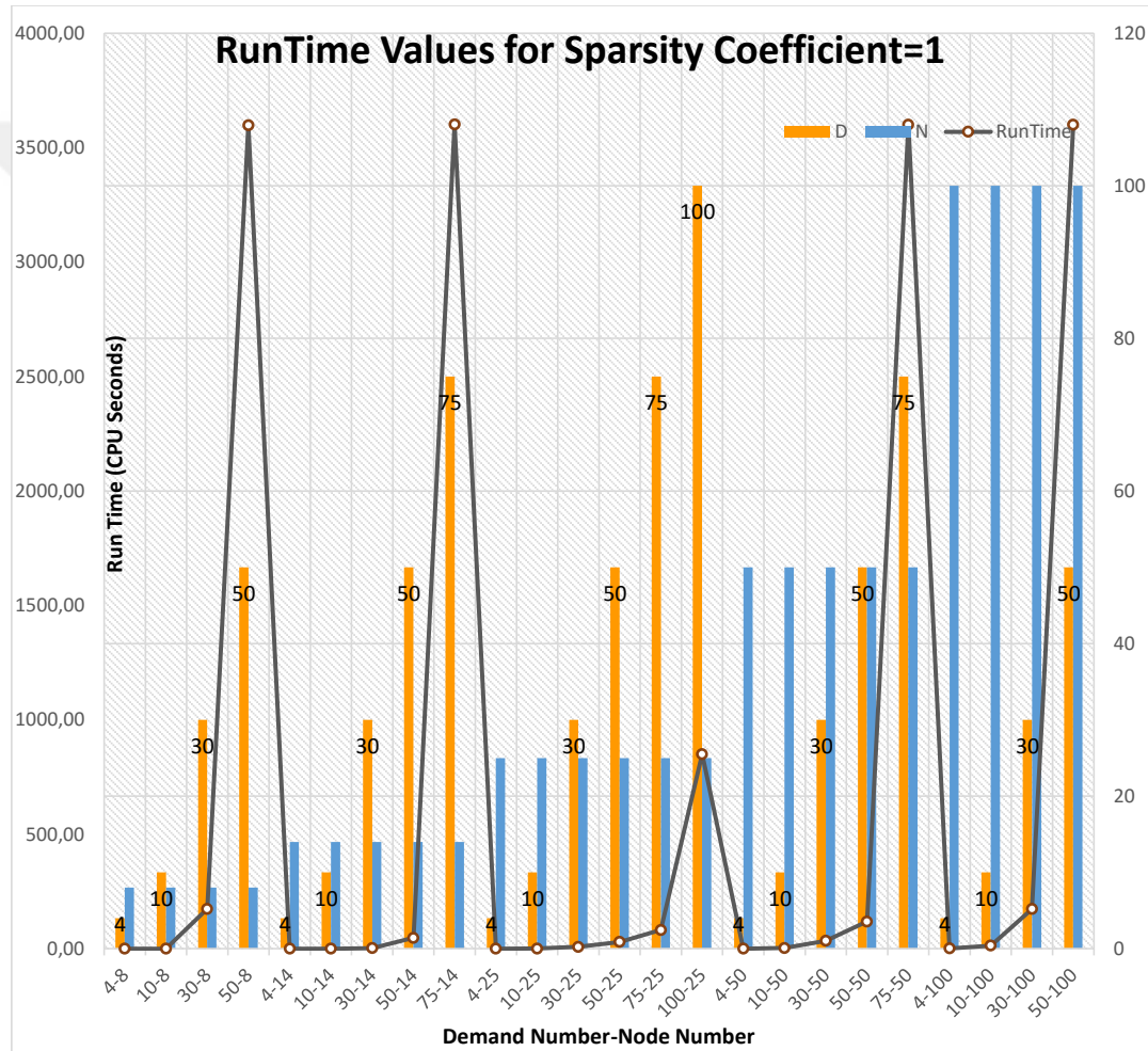
Figure 5.5: Effects of increasing connection requests on run time values at various network topologies for fully connected networks
