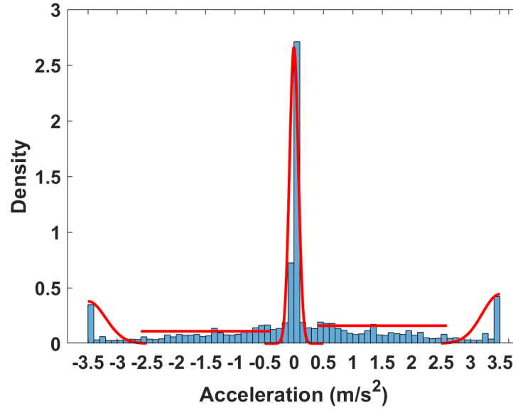
Figure 2.7: Acceleration distribution is approximated with five different distributions: a normal distribution with 0 mean and 0.075 standard deviation, a uniform distribution between 0.5 m/s and 2.5 m/s, a uniform distribution between -0.5 m/s and -2.5 m/s, a half normal distribution with 3.5 mean and 0.3 standard deviation and a half normal distribution with -3.5 mean and 0.3 standard deviation. x-axis shows the accelerations in \text{m/s}^2 and y-axis presents the values of the probability density function.
