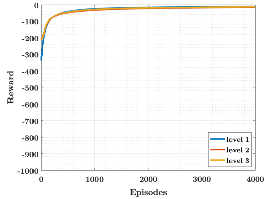
Figure 2.9: Average rewards during level-1, level-2 and level-3 policy training for continuous Deep Q-Learning.
