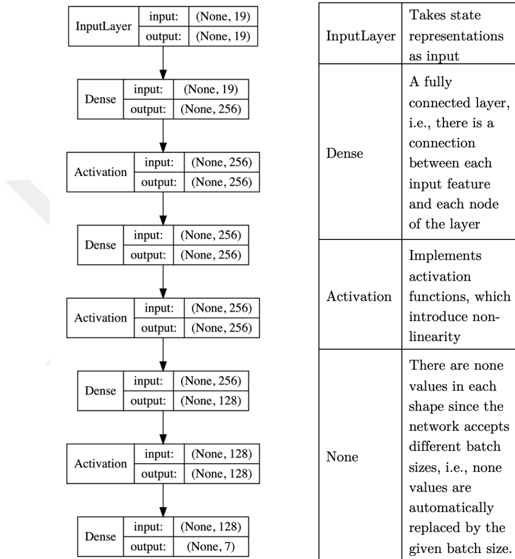
Figure 2.3: A deep neural network consisting of 4 layers is utilized to approximate the Q-function.
