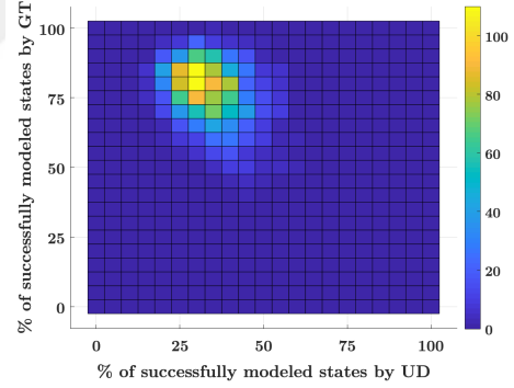
(d) Color map showing the number of drivers whose x\% of the visited states are successfully modeled by the UD policy and y\% by the c-DQN-based GT policy. x and y percentages are given in the horizontal and vertical axes, respectively.
