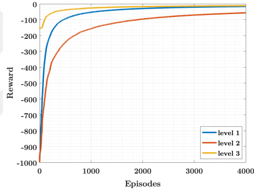
Figure 2.8: Average rewards during level-1, level-2 and level-3 policy training for Deep Q-Learning.
