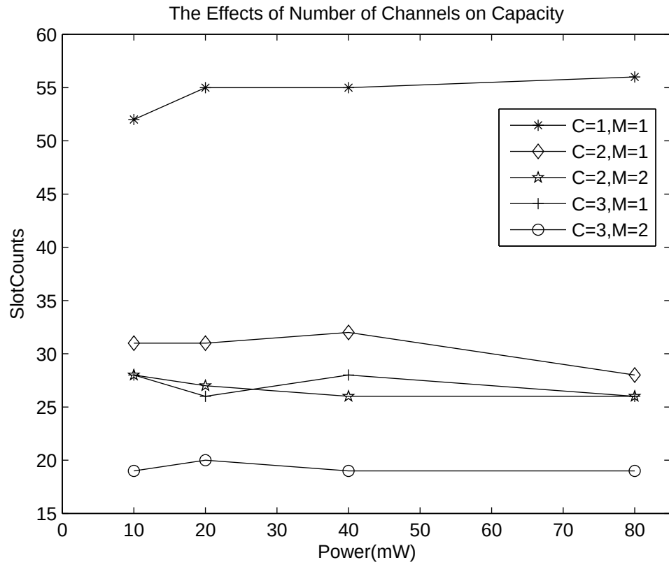
Figure 4.3: The effects of number of channels and radios on the capacity-(Joint transmit and receive beamforming, K = 3 )
