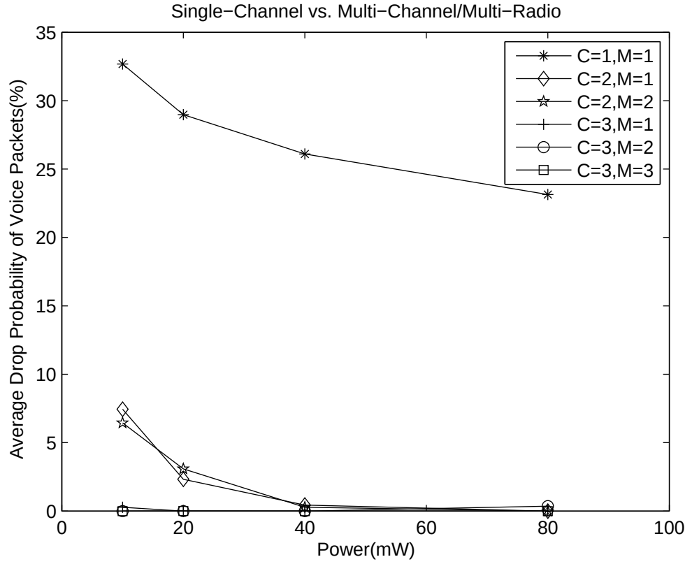
(a) Average drop probability of voice packets
