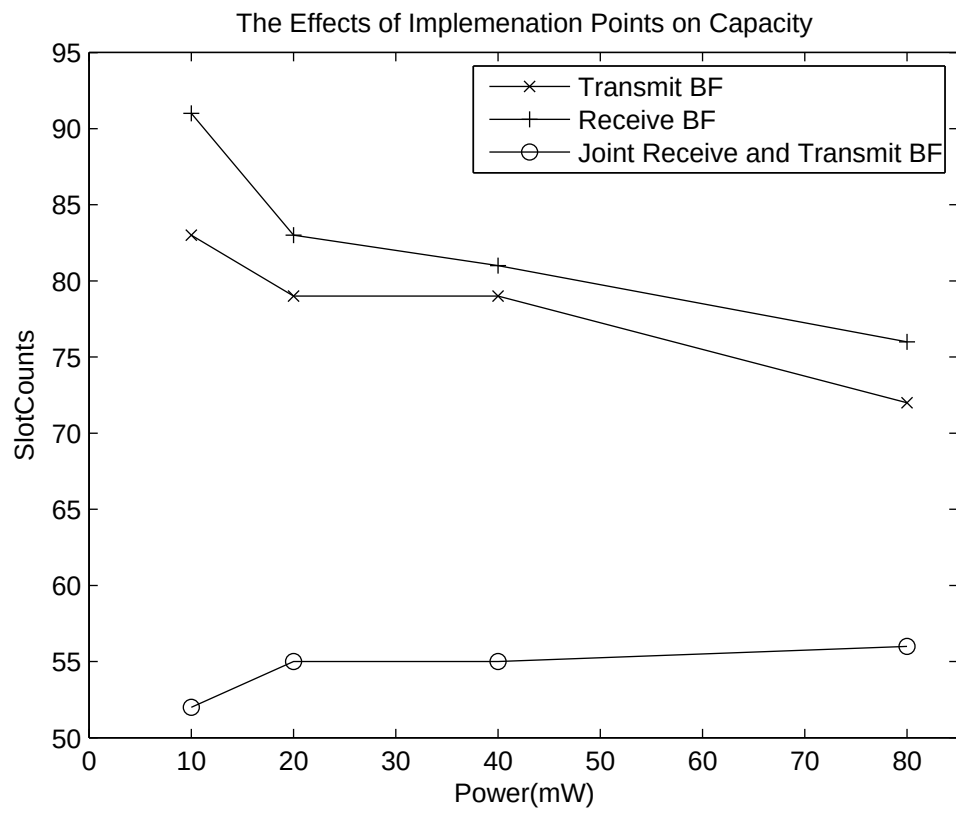
Figure 4.4: The effects of implementation points- ( C = 1 , M = 1 , K = 3 )
