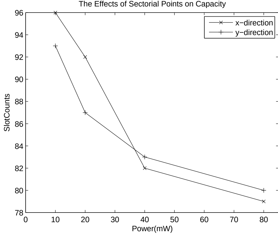
Figure 4.2: The effects of sectorial points on capacity- ( C = 1 , M = 1 , K = 2 , Transmit Beamforming)
