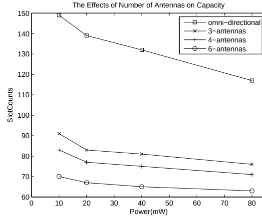
(b) Receive Beamforming
