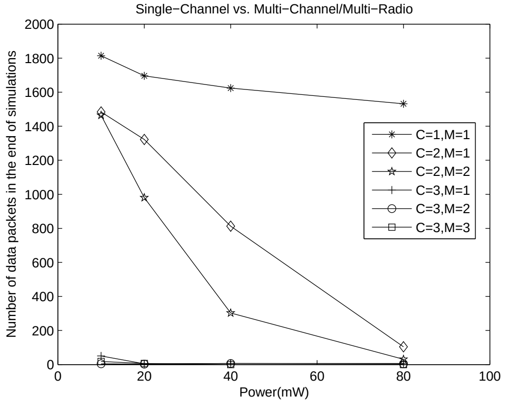
(b) The number of remaining data packets in the end of simulation
