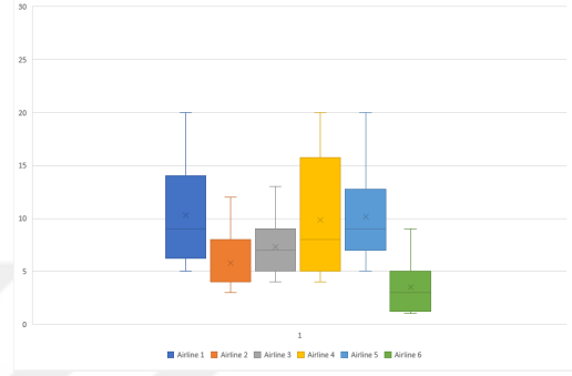
(b) CVaR with \alpha = 0.95, \beta = 20 (Approximate Solution)
