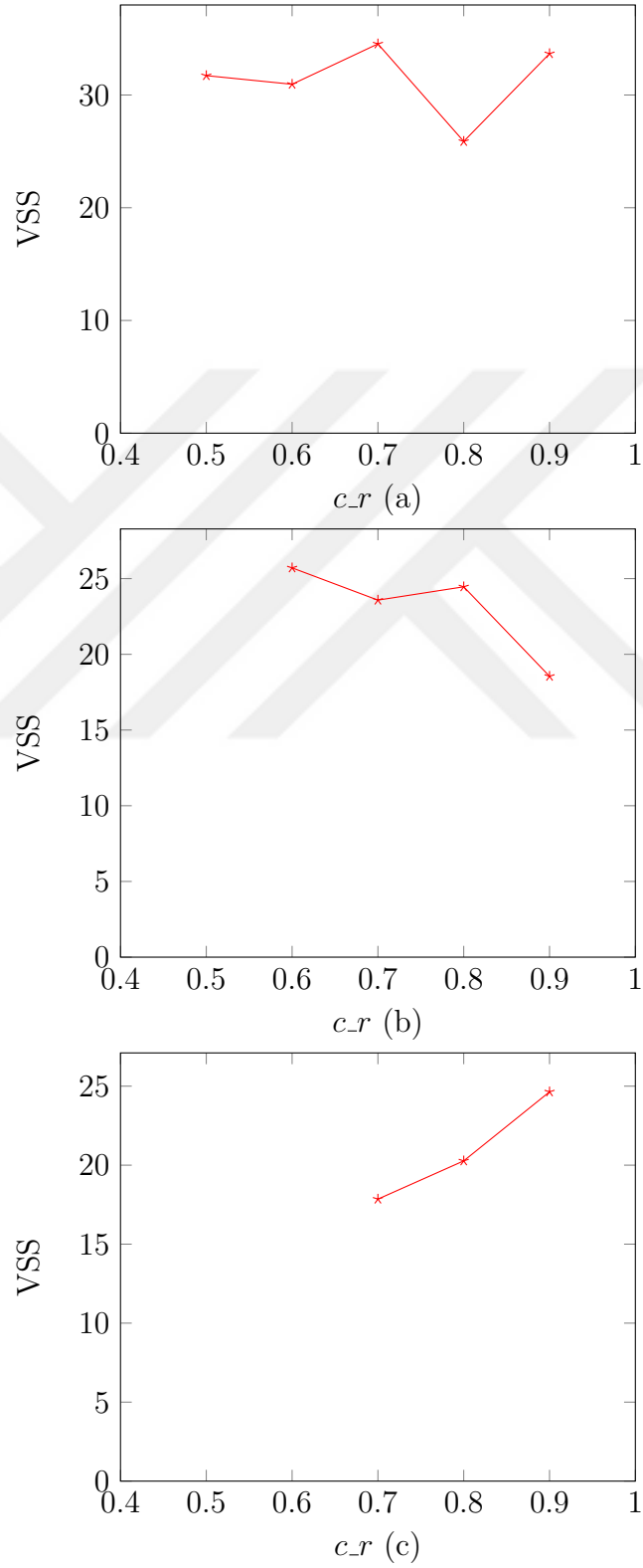
Figure 6.3: VSS for different values ( c_r ). (a) 100 flights and more capacity, (b) 200 flights and more capacity, (c) 200 flights and less capacity
