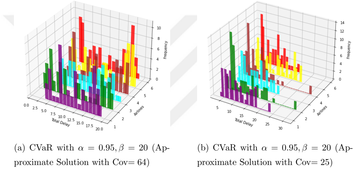
Figure 6.19: Comparison of Approximate CVaR solutions for 600 flights with full and partial coverage of scenarios ( \beta = 20 )
