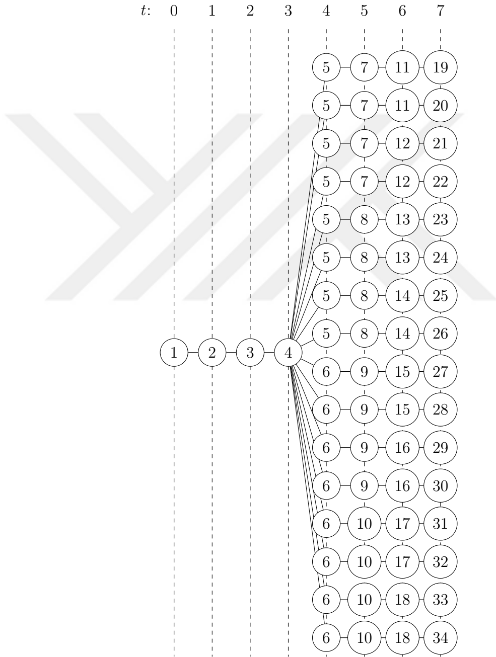
Figure 3.4: Two-stage relaxation of the scenario tree example given in Figure 3.3
