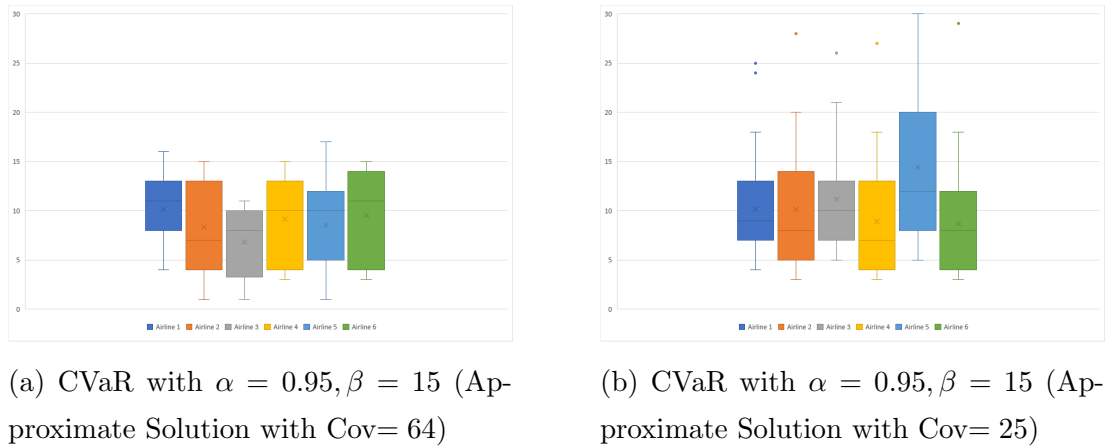
Figure 6.18: Comparison of Approximate CVaR solutions for 600 flights with full and partial coverage of scenarios ( \beta = 15 )
