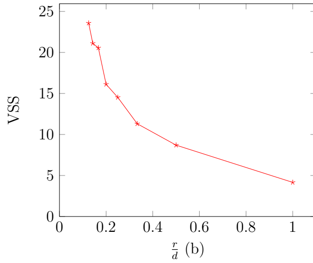
Figure 6.1: VSS for different values of route cost ( r ) to delay cost ( d ) ratio (more capacity). (a) 100 flights, (b) 200 flights
