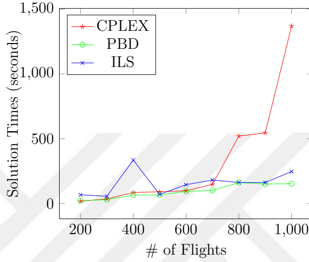
Figure 6.4: Solution times of problems with different number of flights in the setting of Table 6.1
