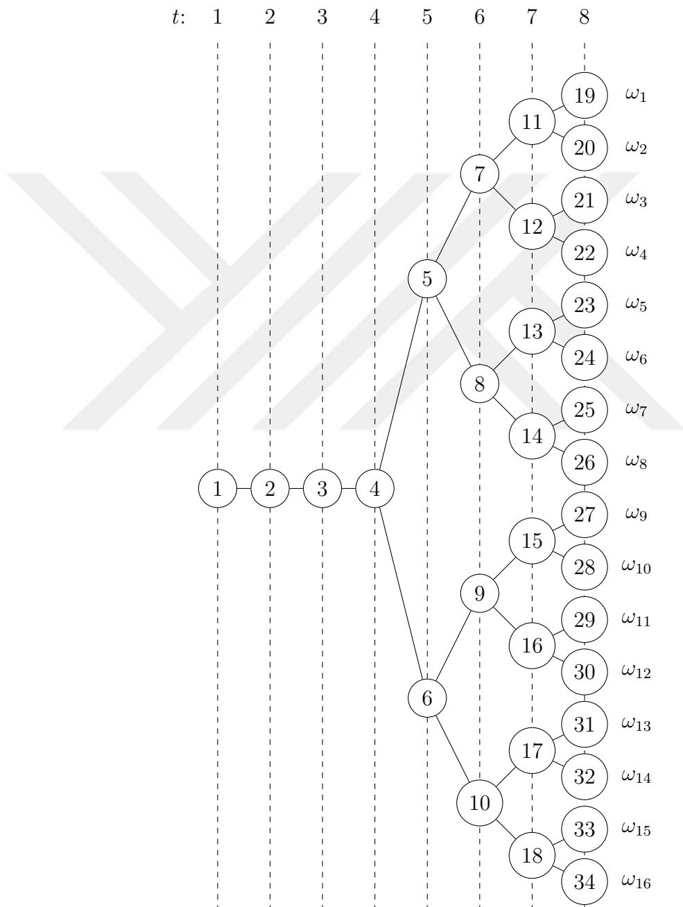
Figure 3.3: Example of a multistage scenario tree considering 8 time periods and 16 scenarios
