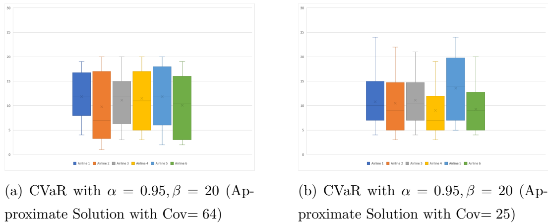
Figure 6.20: Comparison of Approximate CVaR solutions for 600 flights with full and partial coverage of scenarios ( \beta = 20 )
