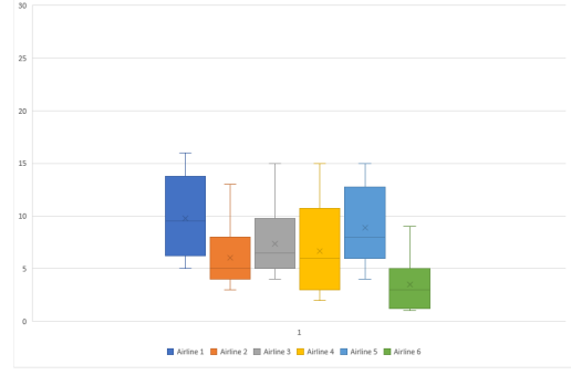
(b) CVaR with \alpha = 0.95, \beta = 15 (Approximate Solution)
