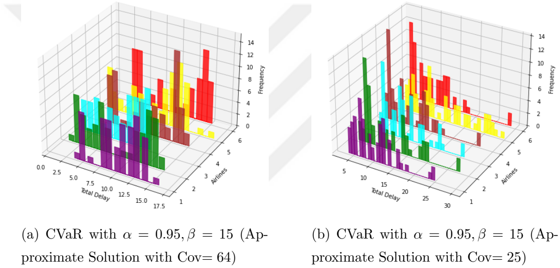
Figure 6.17: Comparison of Approximate CVaR solutions for 600 flights with full and partial coverage of scenarios ( \beta = 15 )
