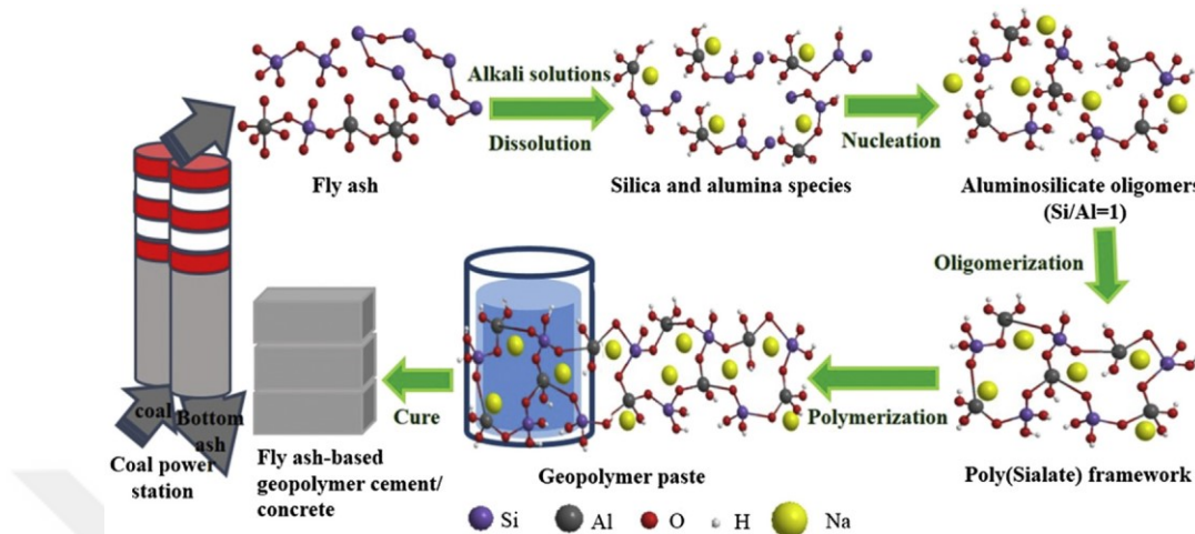
Figure 2.4 Geopolymerisation process (Zhuang et al. 2016)
