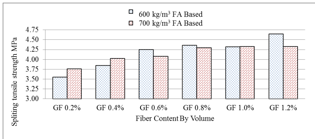
Figure 4.5 Splitting tensile strength
