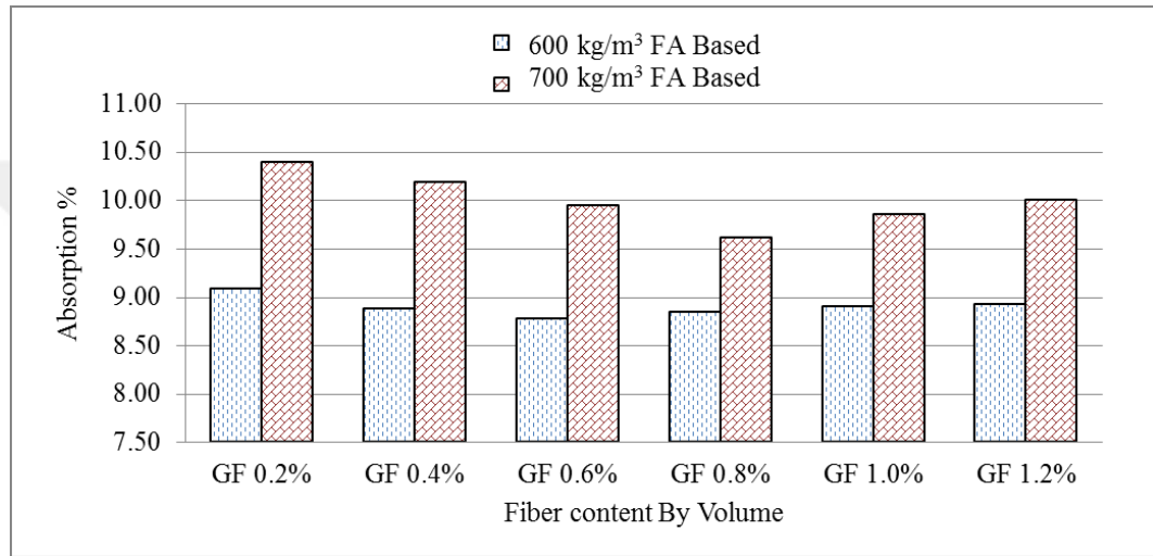
Figure 4.7 Water absorption
