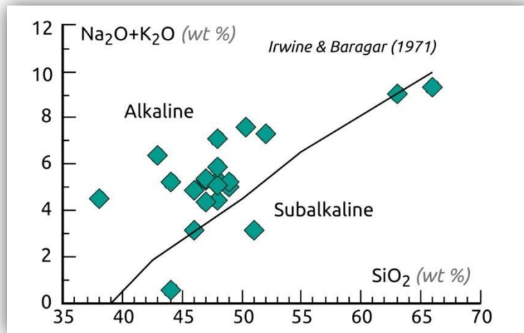
Figure 3.5 Diagram of total alkalis vs \text{SiO}_2 showing character of the mafic volcanic rocks from the Bornova melange in the Akhisar region. Three samples plot on the subalkaline field and the other nineteen samples locate on the alkaline field in the diagram of Irvine & Baragar (1971).
