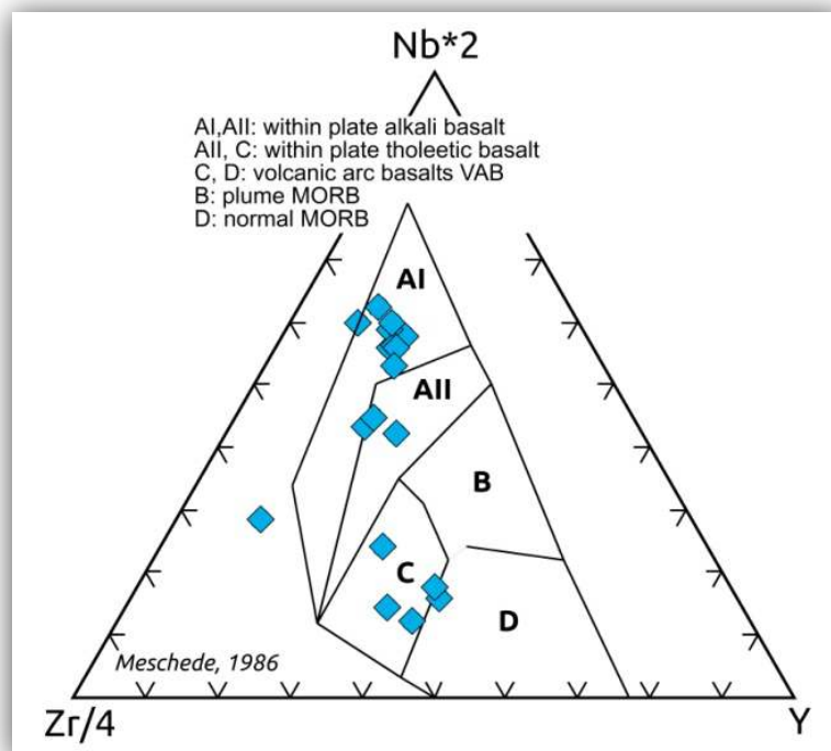
Figure 3.11 Ternary diagram combined by 2Nb-Zr/4-Y of Meschede (1986) showing tectonic setting of the basalts of Bornova melange.
