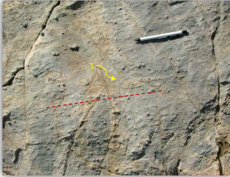
Figure 4.2 Stretching lineation along the foliation planes of the recrystallized limestones of the Kayaaltı formation that represents the structurally upper part of the Menderes massif. Red dashed line is parallel to the stretching lineation diagnosed by stretched dolomite clast (yellow arrow 1). Pencil is 13 centimeters.
