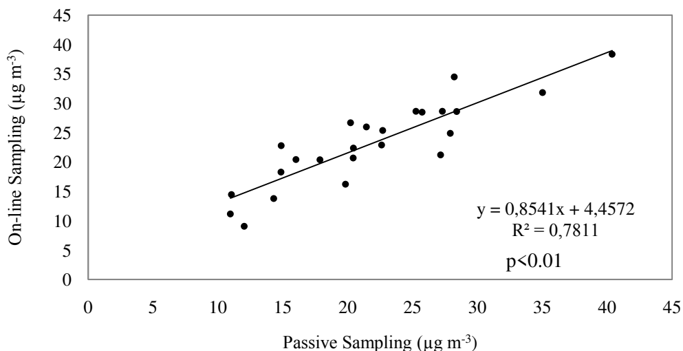
Figure 3.6 Diffusive sampling and on-line sampling comparison for NO_2 , S-5.
