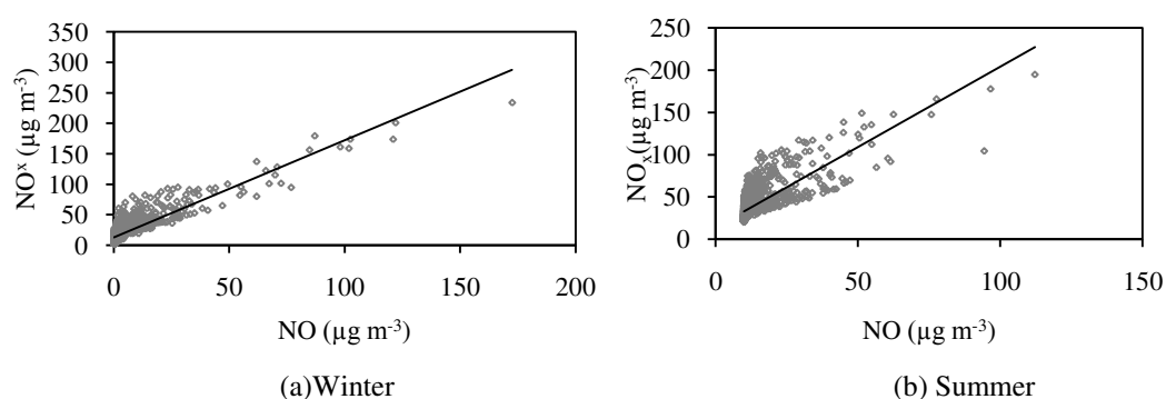
Figure 4.10 Relationship between NO_x and NO levels in (a) winter and (b) summer.
