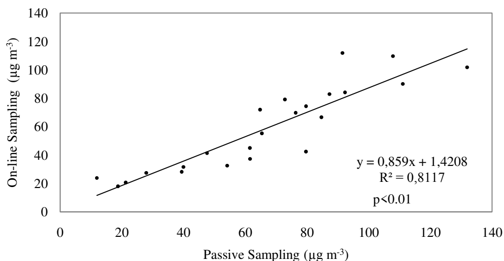
Figure 3.5 Diffusive sampling and on-line sampling comparison for O_3 , S-5.
