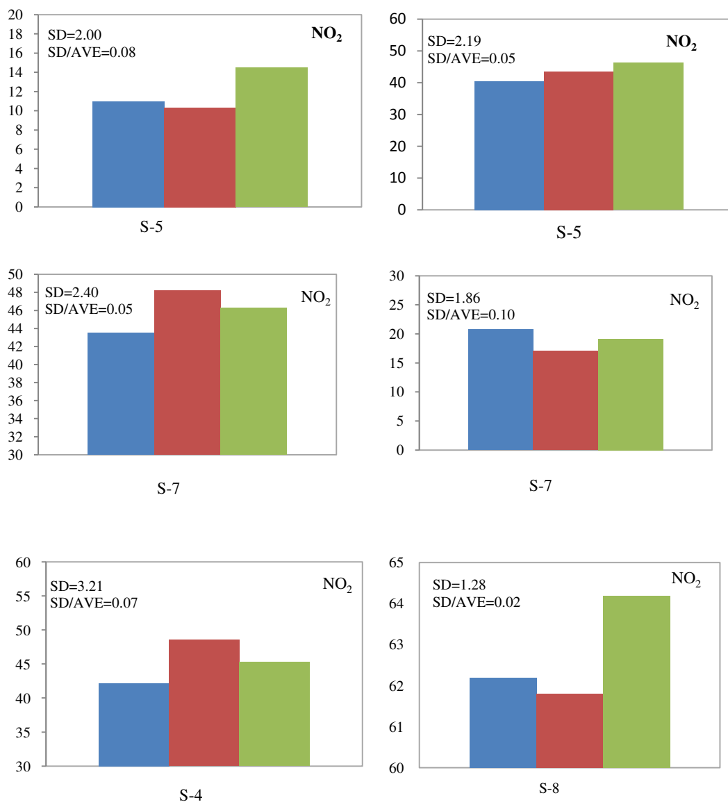
Figure 3.8 Repeatability of results of \text{NO}_2 measurement with diffusive sampling.
