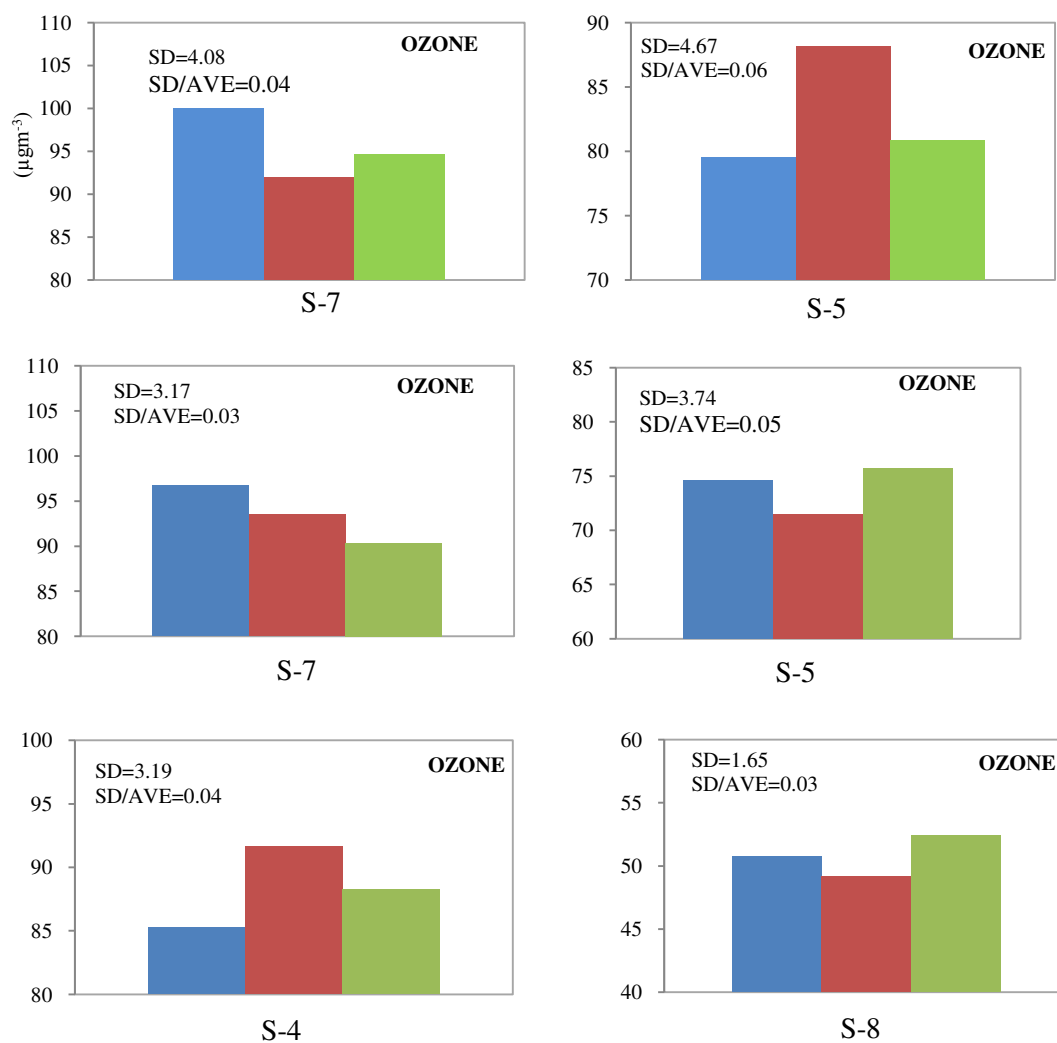
Figure 3.7 Repeatability of results of O 3 measurement with diffusive sampling.
