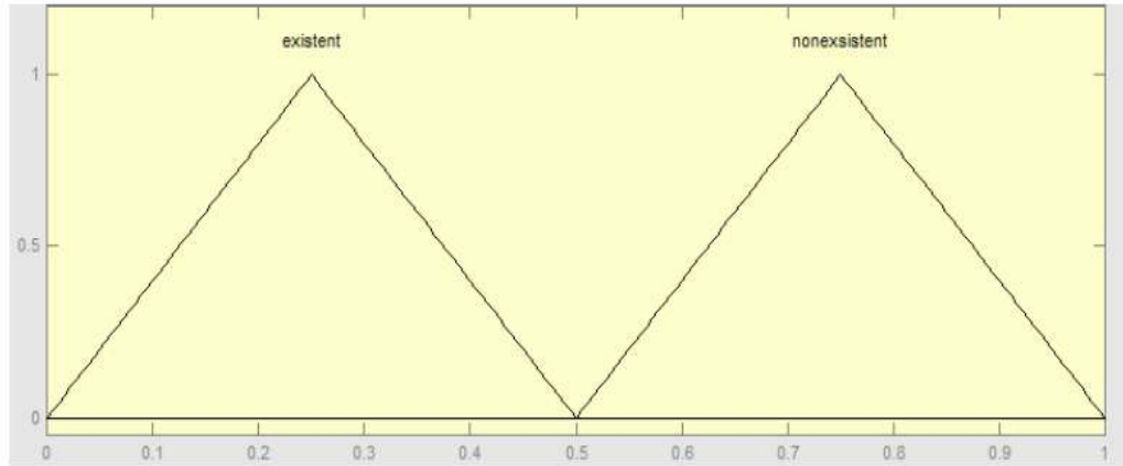
Figure 2.15 Fuzzy input membership functions used for flay ash.
