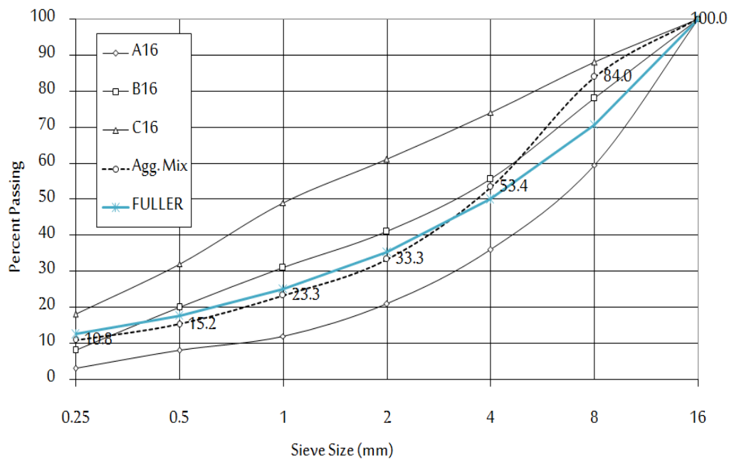
Figure 4.3 Grading of aggregate mix and reference curves.
