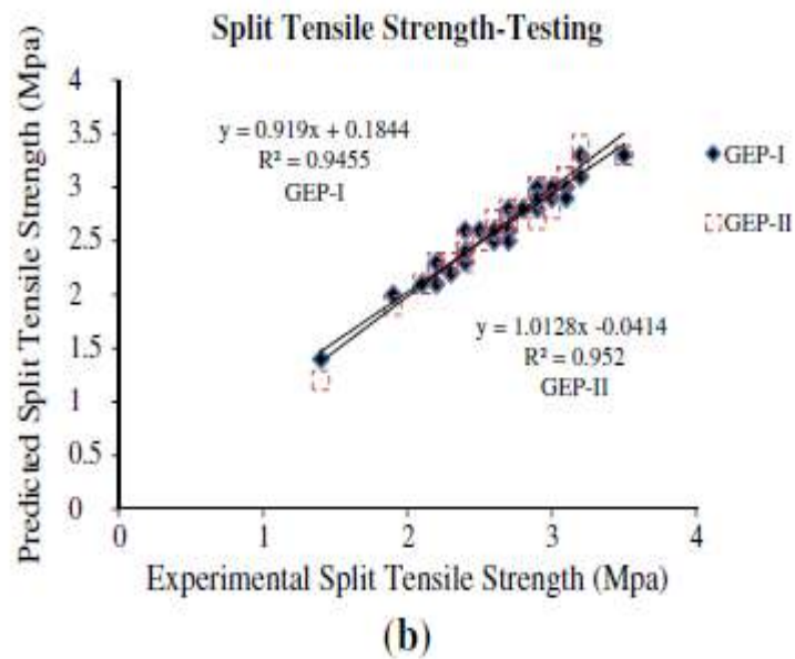
Figure 2.8 The correlation of the measured and predicted split tensile strengths in (a) Training and (b) testing phase for GEP models.( Nazari and Riahi , 2011)
