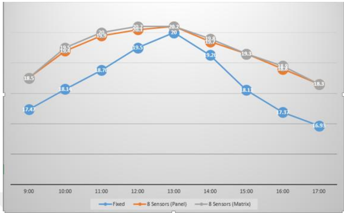
Figure 4.22 PV panel voltage generation difference with time between solar panel with 8 LDR on panel tracker and 8 matrix LDR tracker from Gaziantep city in 30 October
