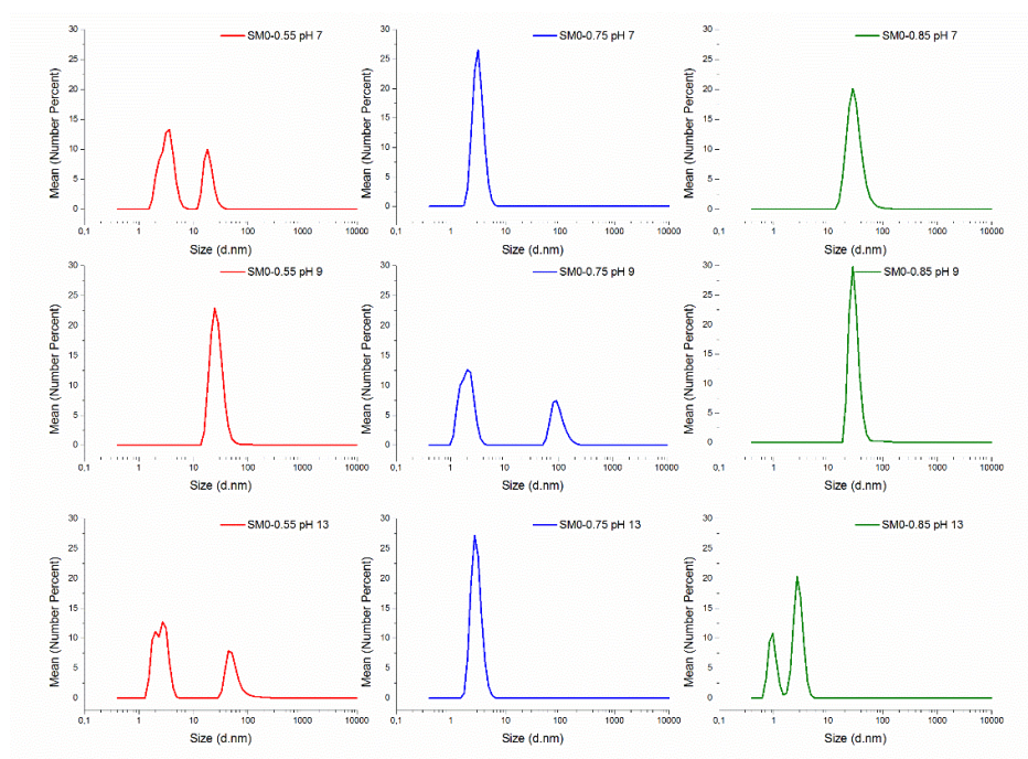
Figure 81 DLS spectra of SM0-based SHBPAES samples; SM0-0.55, SM0-0.75, and SM0-0.85 of A 2 :B 3 ratio at pH 7, 9, and 13
