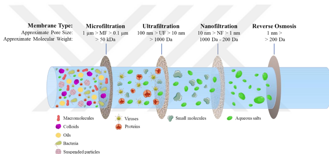
Figure 9 Required filter media according to the separation power used in industrial wastewater recovery
