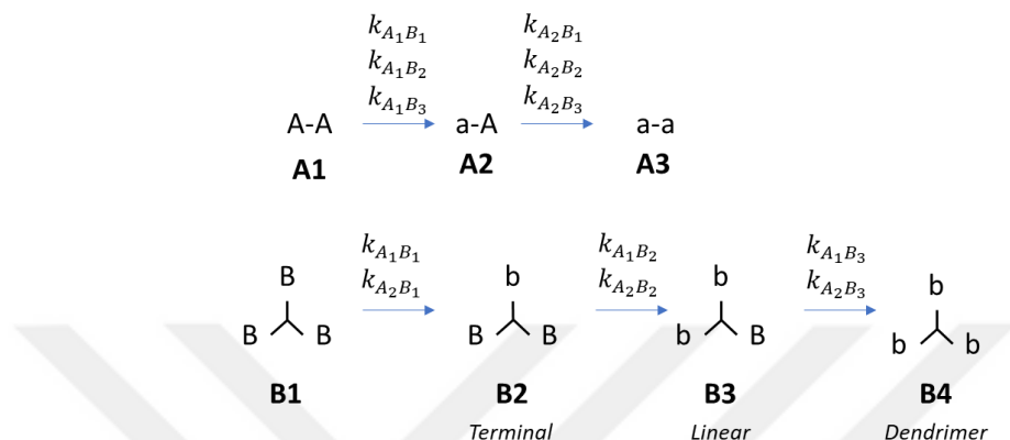
Figure 21 A_2+B_3 reaction pathways and notation of structural units [173]
