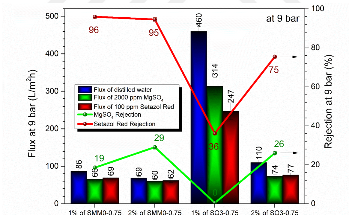
Figure 84 The comparison of the filtration performance of TFC membranes fabricated from 0.1% of TMC in hexane with 1 wt% and 2wt% aqueous solution of two different SHBPAES reagents, SMM0-0.75 and O3-0.75.
