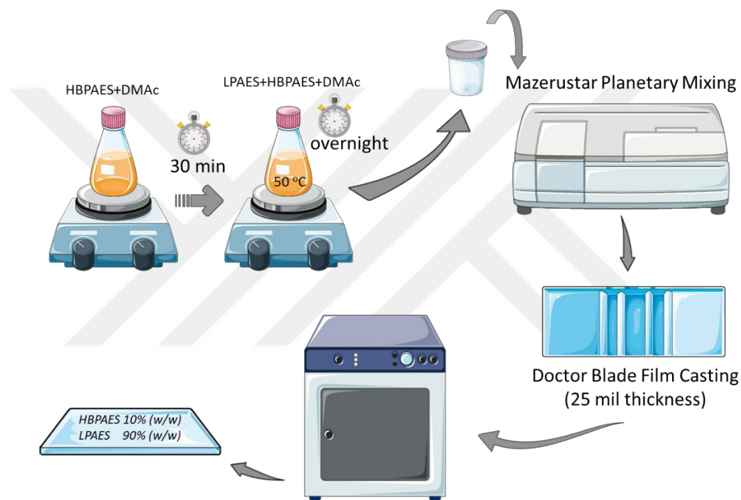
Figure 29 Schematic representation of the steps of blend film preparation
