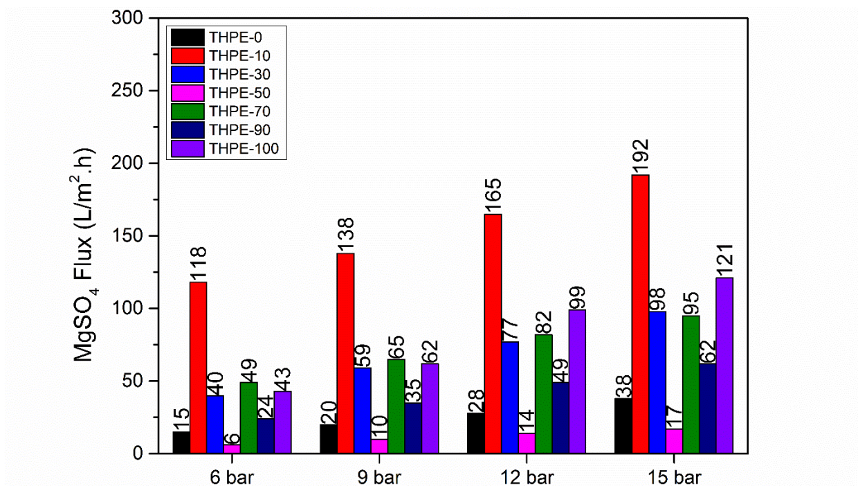
Figure 70 Results of 2000 ppm \text{MgSO}_4 aqueous solution flux of TFC membranes: THPE-0, 30, 50, 70, 90, and 100.
