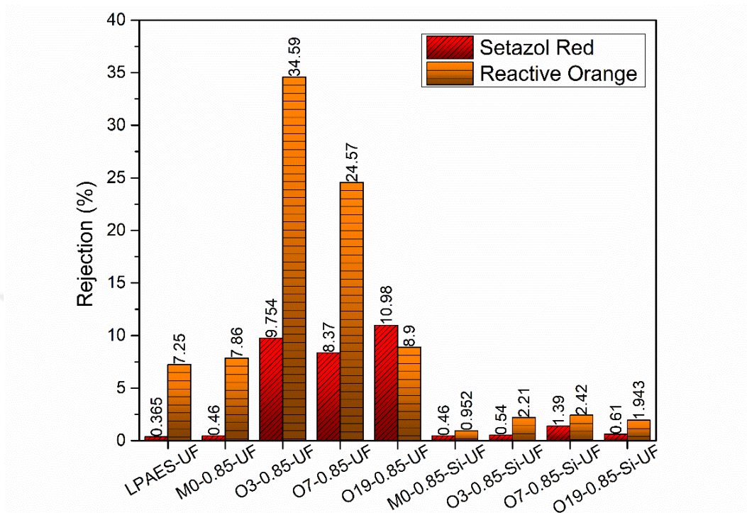
Figure 63 Setazol Red and Reactive Orange 16 dye rejections of the control and blend UF membranes at 2 bars
