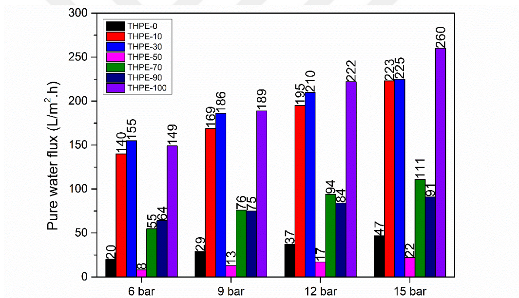
Figure 69 Results of pure water flux of TFC membranes: THPE-0, 30, 50, 70, 90, and 100.
