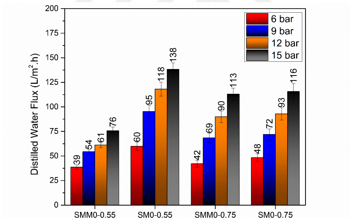
Figure 85 Distilled water fluxes of TFC membranes fabricated by the interfacial polymerization reaction of TMC with SMM0-0.55, SM0-0.55, SMM0-0.75, and SM0-0.75
