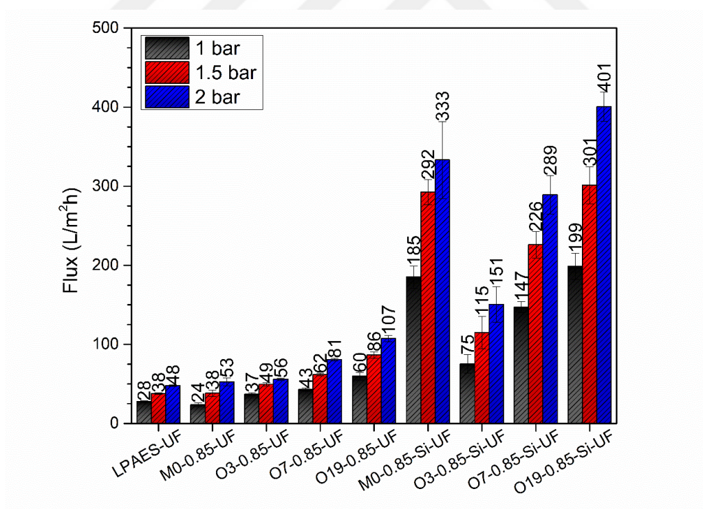
Figure 59 Distilled water fluxes of the control and blend UF membranes under 1.0, 1.5 and 2.0 bars
