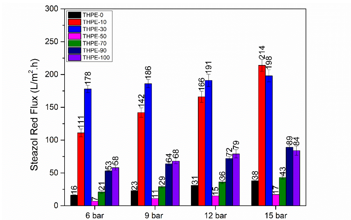
Figure 74 Results of 100 ppm Setazol Red aqueous solution flux of TFC membranes: THPE-0, 30, 50, 70, 90, and 100.
