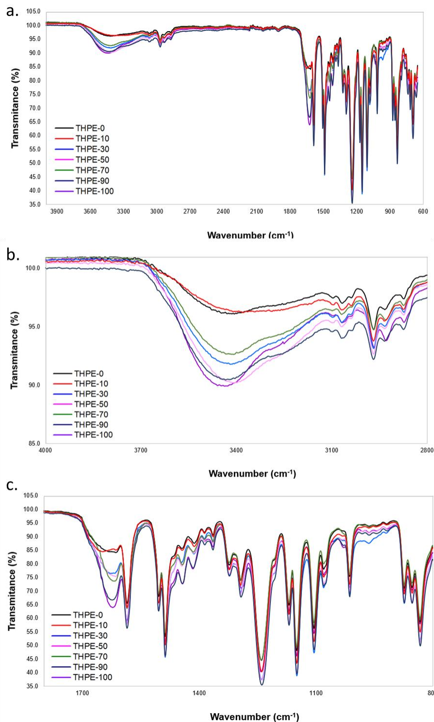
Figure 68 FT-IR transmittance spectra of the active layers of TFC membranes: THPE-0, 30, 50, 70, 90, and 100; a. between 4000 and 600 cm -1 , b. between 4000 and 2800 cm -1 , c. between 1800 and 800 cm -1
