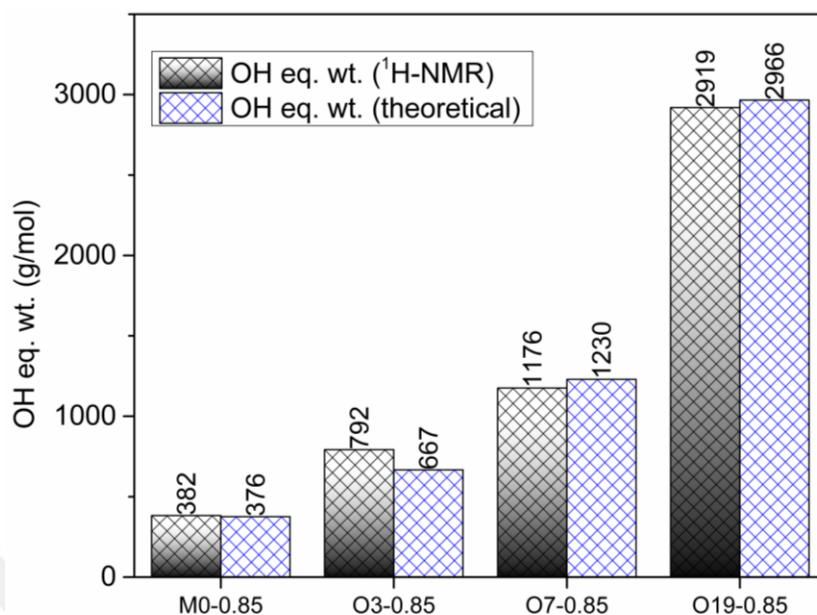
Figure 41 A comparison of theoretical results of OH equivalent weights of HBPAESs with those obtained from ^1\text{H-NMR} spectra
