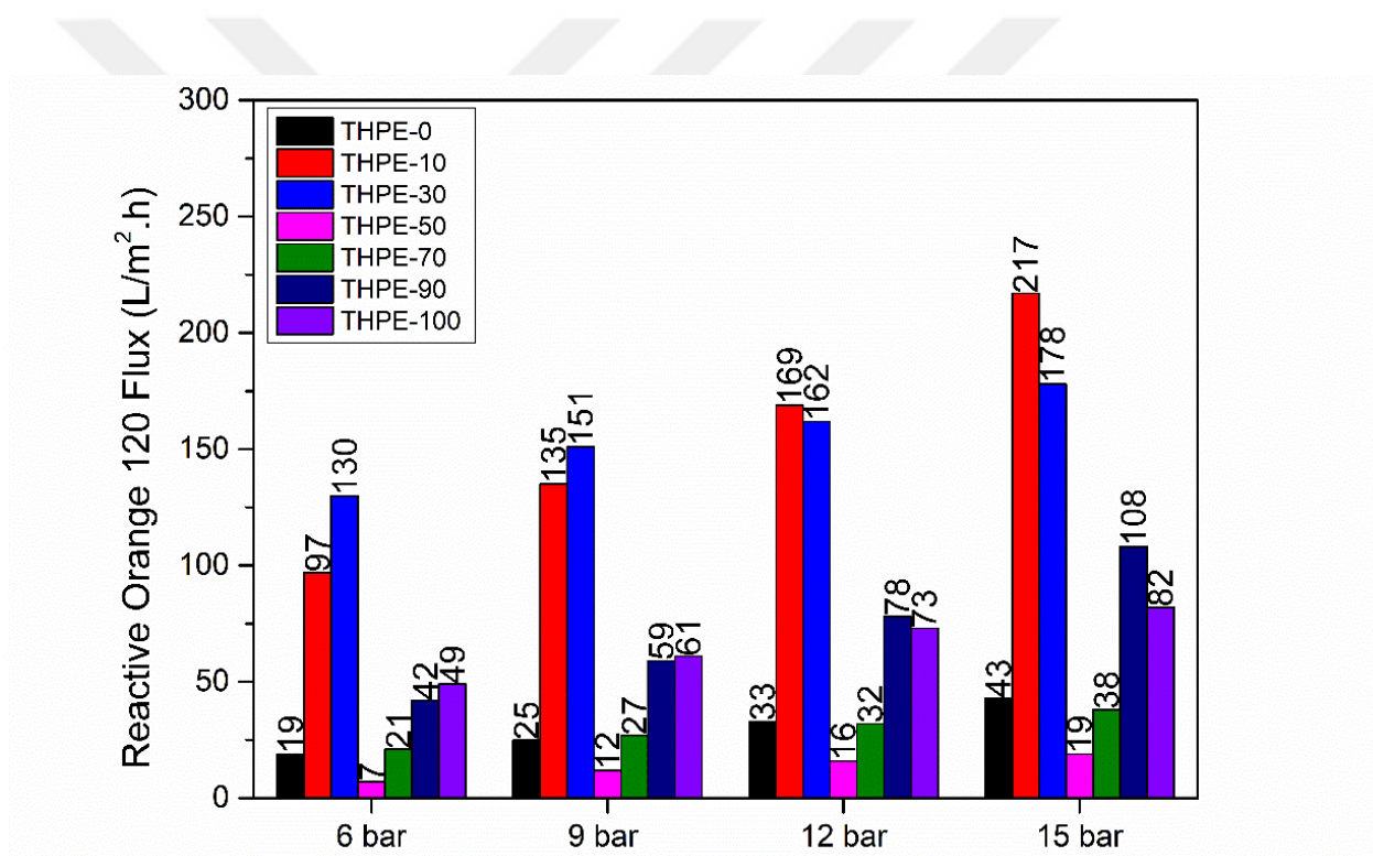
Figure 76 Results of 100 ppm Reactive Orange 120 aqueous solution flux of TFC membranes: THPE-0, 30, 50, 70, 90, and 100.
