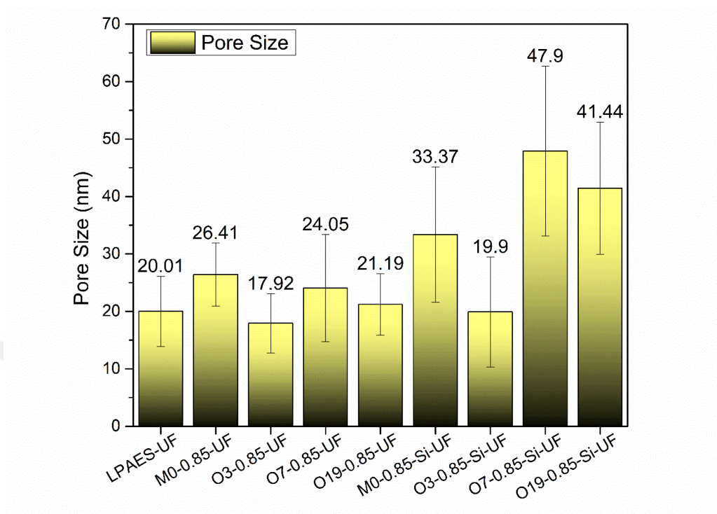
Figure 57 Pore sizes of the control and blend UF membranes determined from SEM images
