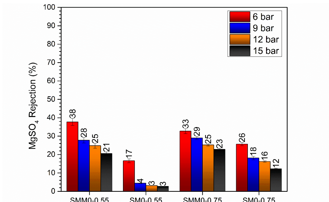
Figure 87 \text{MgSO}_4 rejections of TFC membranes made by the interfacial reaction of TMC with SMM0-0.55, SM0-0.55, SMM0-0.75, and SM0-0.75
