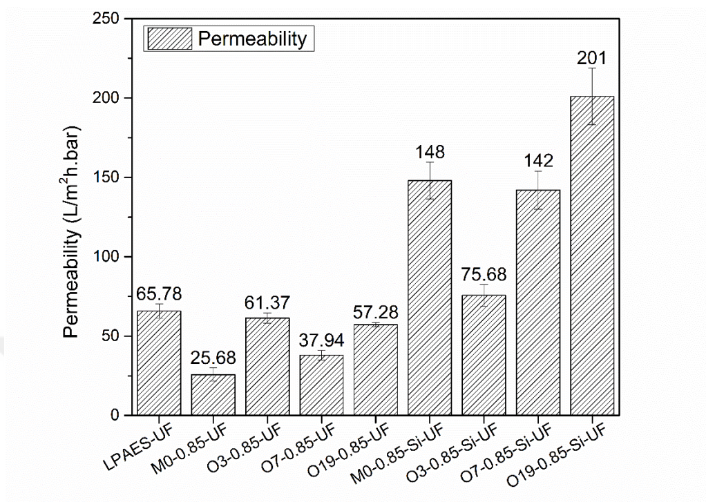
Figure 60 Distilled water permeability of the control and blend UF membranes
