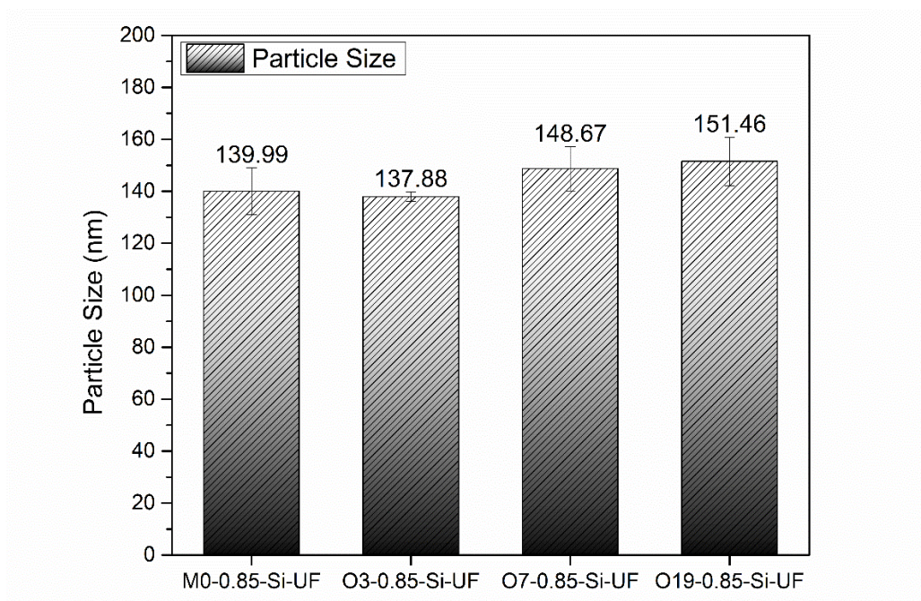
Figure 58 Size distribution of spherical particles on the HBPAES-Si containing blend UF membrane surfaces
