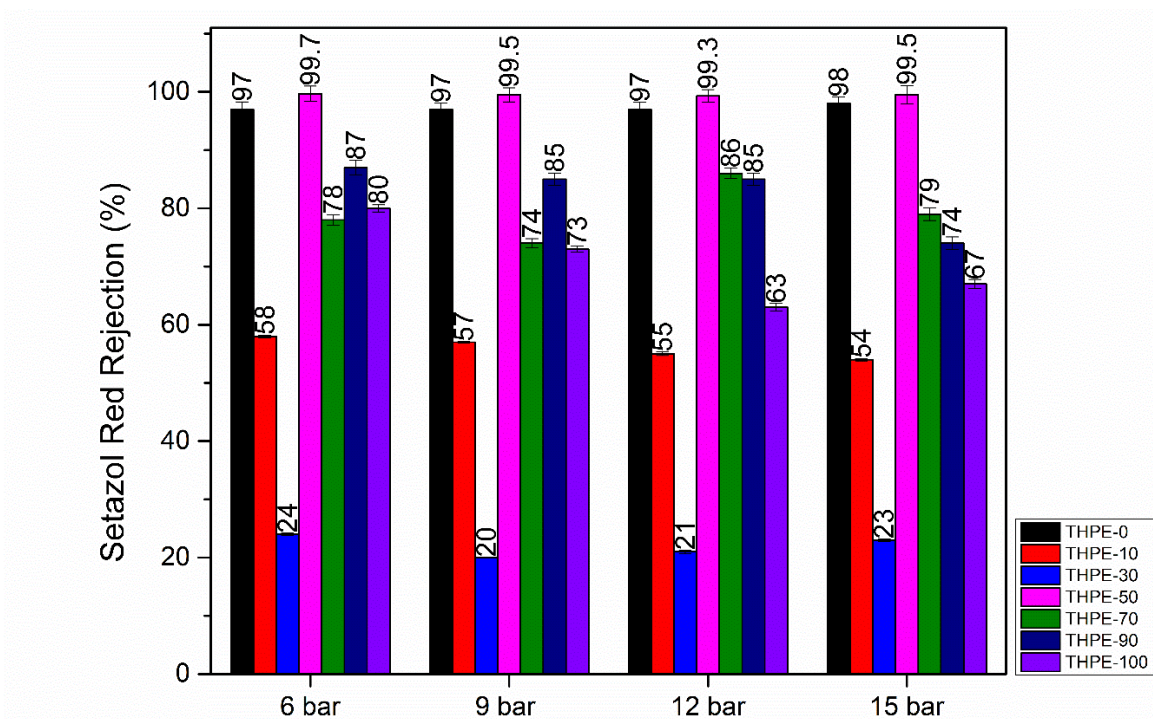
Figure 75 Setazol Red rejection results of TFC membranes: THPE-0, 30, 50, 70, 90, and 100.
