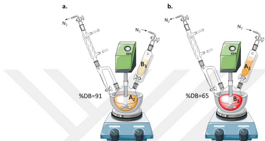
Figure 23 The reaction set-ups in accordance with monomer addition methods, which can directly influence the degree of branching of final products
