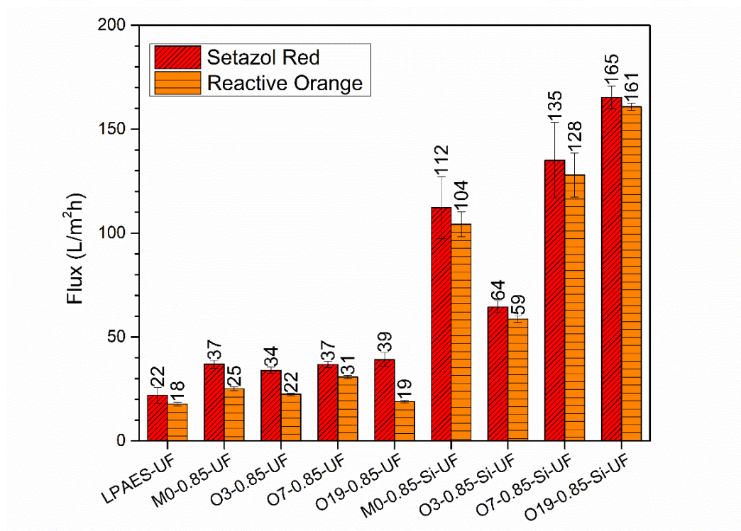
Figure 62 Setazol Red and Reactive Orange 16 flux values of the control and blend UF membranes at 2 bars
