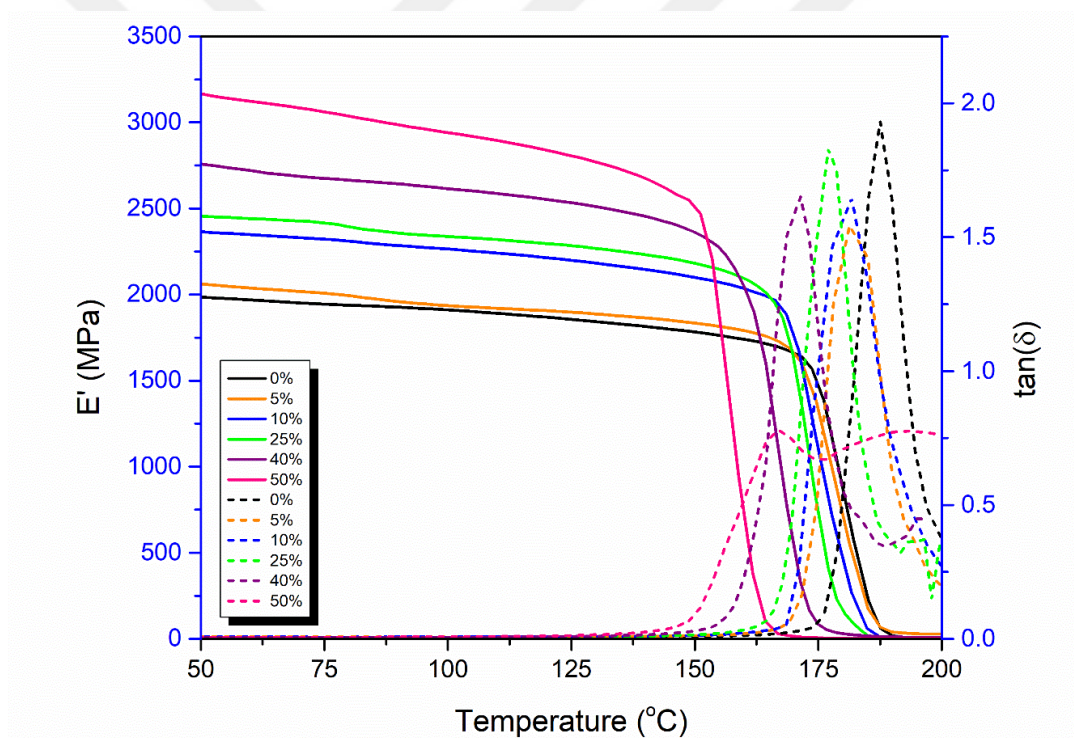
Figure 48 DMA curves of blend films containing various fractions of HBPAES O3-0.85 in LPAES [180]
