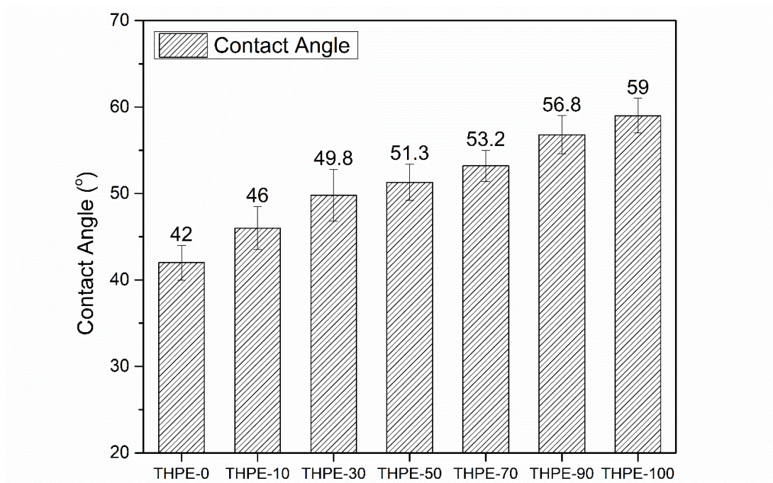
Figure 67 Contact angle measurements of TFC membranes: THPE-0, 30, 50, 70, 90, and 100.
