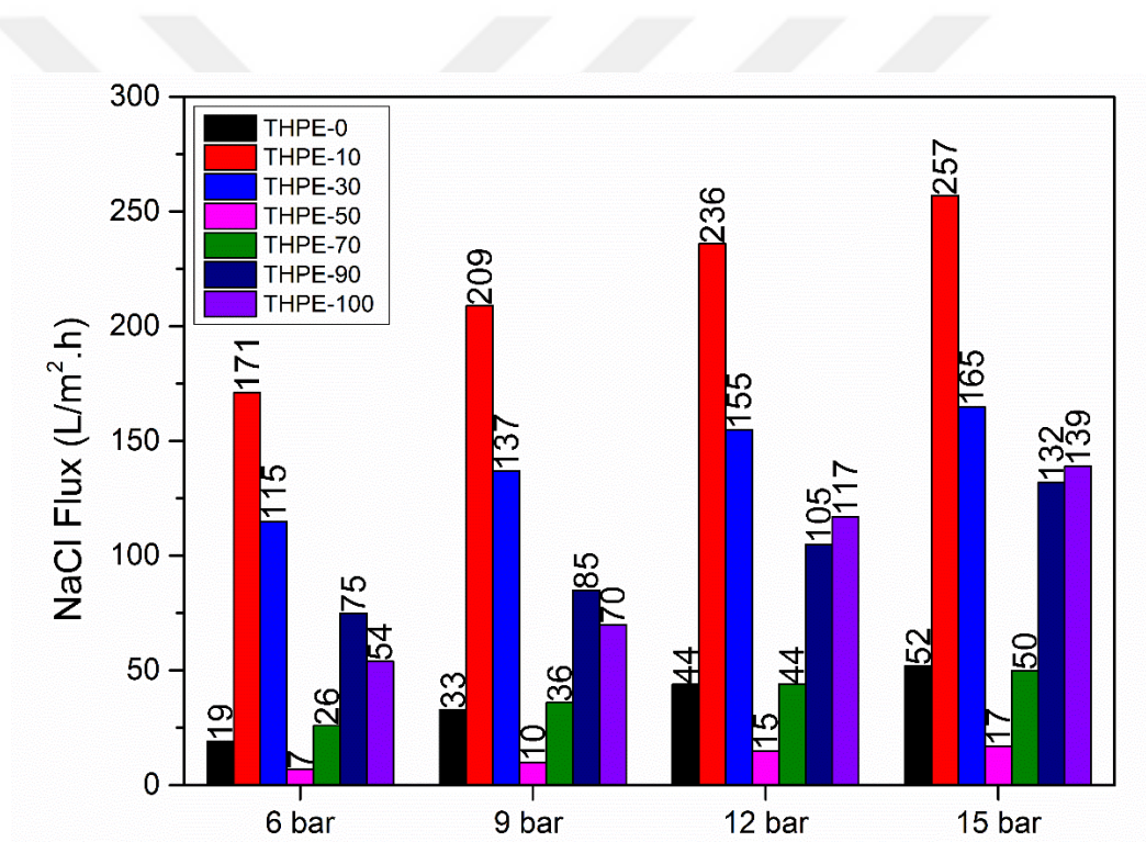
Figure 72 Results of 2000 ppm NaCl aqueous solution flux of TFC membranes: THPE-0, 30, 50, 70, 90, and 100.
