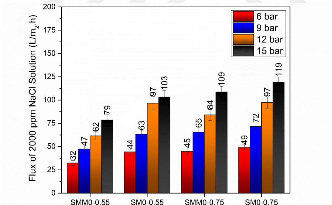
Figure 88 2000 ppm NaCl solution fluxes of TFC membranes made by the interfacial reaction of TMC with SMM0-0.55, SM0-0.55, SMM0-0.75, and SM0-0.75
