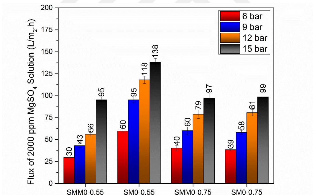
Figure 86 2000 ppm \text{MgSO}_4 solution fluxes of TFC membranes made by the interfacial reaction of TMC with SMM0-0.55, SM0-0.55, SMM0-0.75, and SM0-0.75
