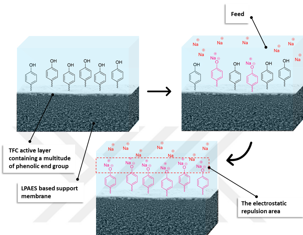
Figure 90 A proposed \text{Na}^+ rejection mechanism for TFC active layers containing a multitude of phenolic end groups
