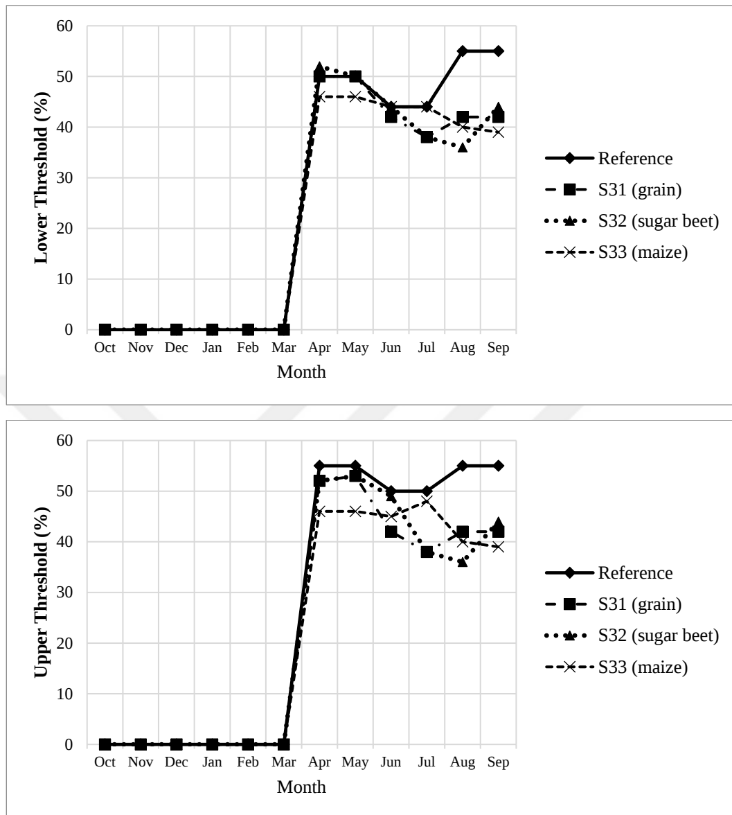
Figure 3.23. Monthly lower and upper threshold values modified for deficit irrigation application
