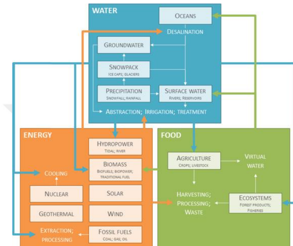
Figure 1.1. Water, energy and food nexus schematic (Biggs et al., 2015)
