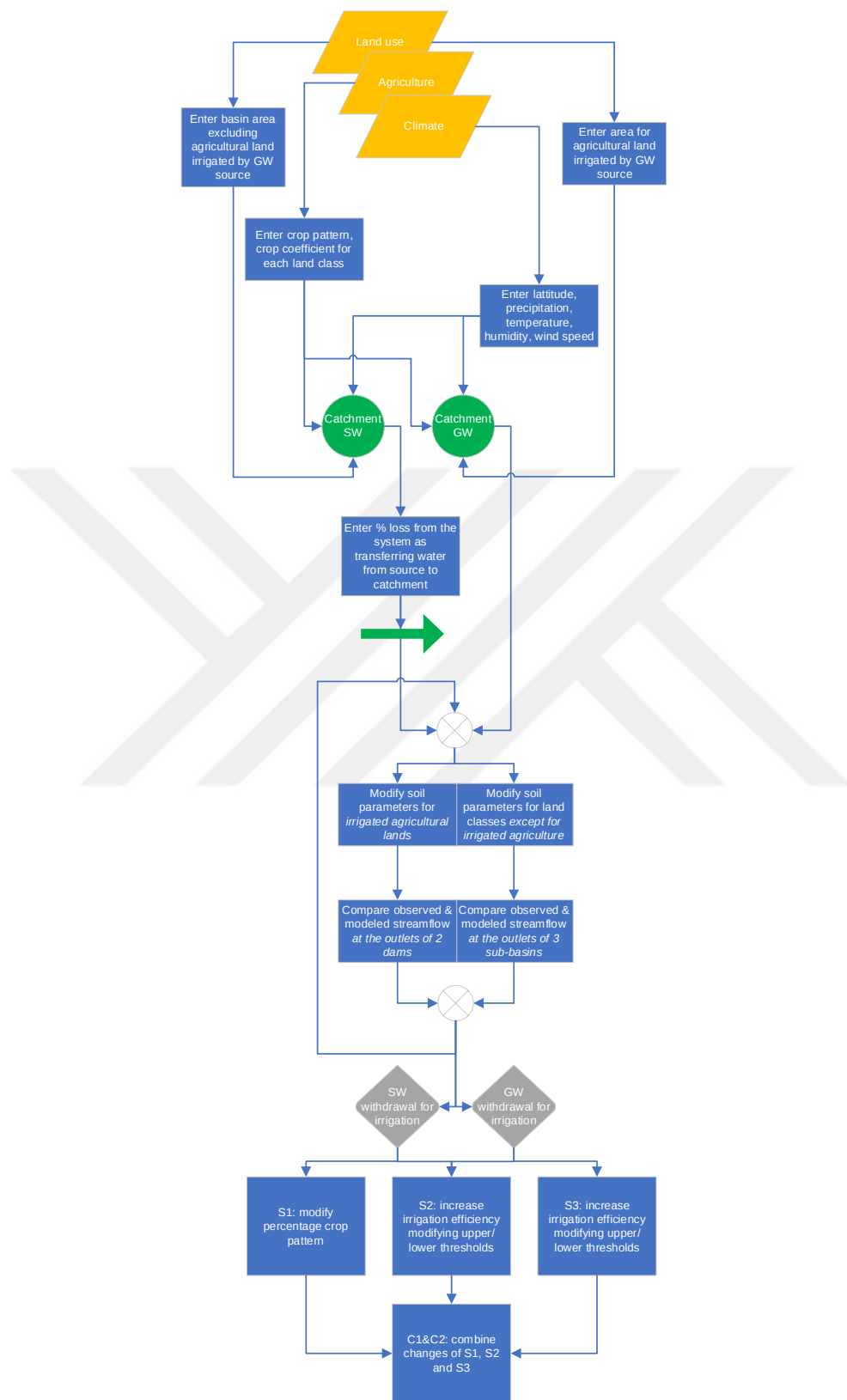
Figure 3.6. The conceptual model for simulation of catchment
