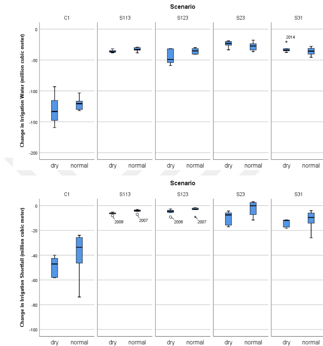
Figure 4.4. Box and whisker plots by the most effective scenarios (2005-2016)
