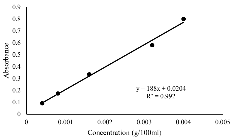
Figure A.2. Calibration curve for OPA method prepared by glycine for free amino group determination
