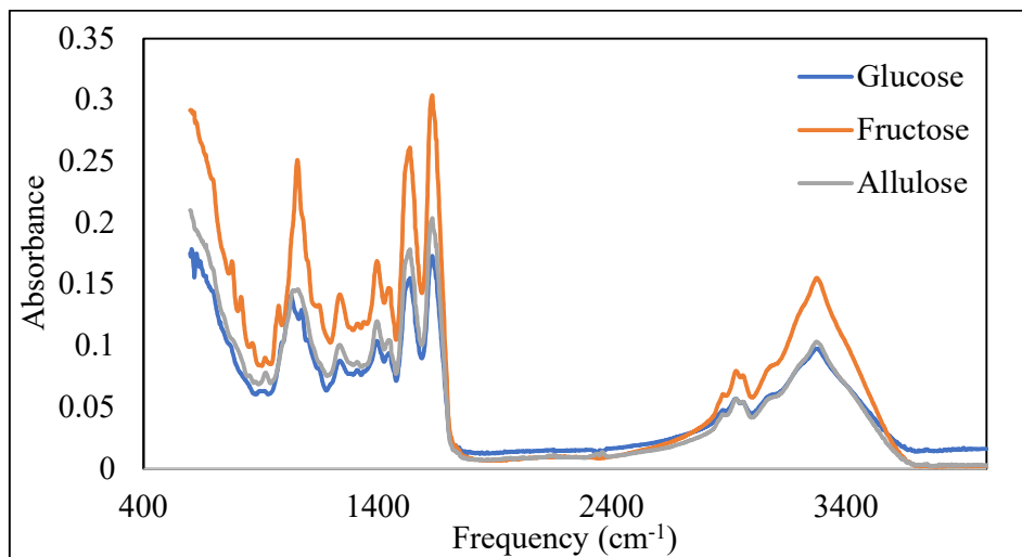
Figure B.2. FT-IR spectra of proteins glycated with glucose, fructose and allulose at a protein-water ratio of 1:1 (w/w) at 100°C
