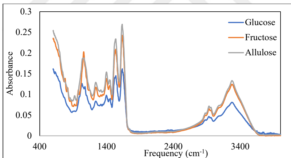
Figure B.4. FT-IR spectra of proteins glycated with glucose, fructose and allulose at a protein-water ratio of 1:1 (w/w) at 130°C
