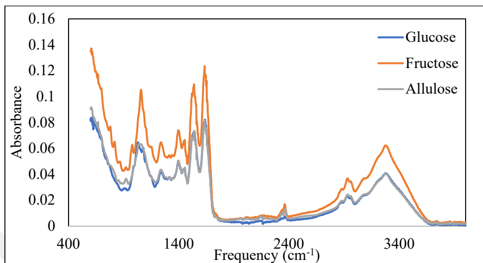
Figure B.3. FT-IR spectra of proteins glycated with glucose, fructose and allulose at a protein-water ratio of 1:2 (w/w) at 100°C
