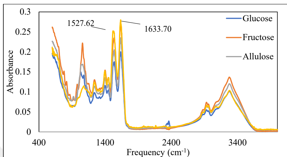
Figure 3.9. FT-IR spectra of native SPI and proteins glycated with glucose, fructose and allulose at a protein-water ratio of 1:2 (w/w) under incubation conditions
