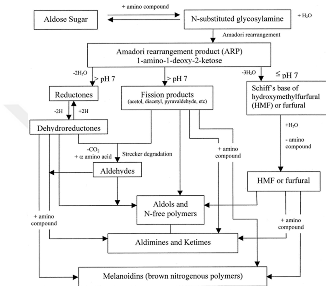
Figure 1.1. Hodge's Maillard Scheme (Hodge, 1953)
