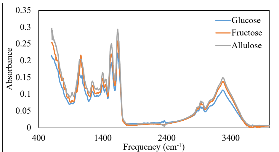
Figure B.1. FT-IR spectra of proteins glycated with glucose, fructose and allulose at a protein-water ratio of 1:1 (w/w) under incubation conditions
