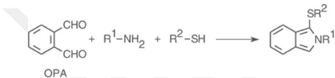
Figure 1.2. Reaction of O-phthalaldehyde with SH-group containing compound and free amino groups on proteins (de Oliveira et al., 2016)
