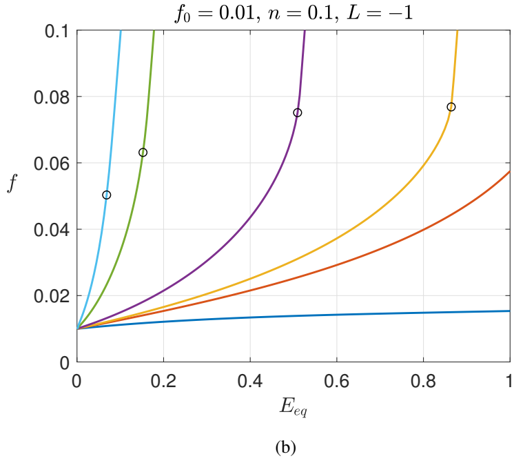
Figure 4.5: Results from the RVE simulations for f_0 = 0.01, n = 0.1 and L = -1 . (a) Normalized equivalent stress strain relation, (b) void volume fraction, f , vs equivalent strain. The onset of uniaxial straining mode is marked by \circ .
