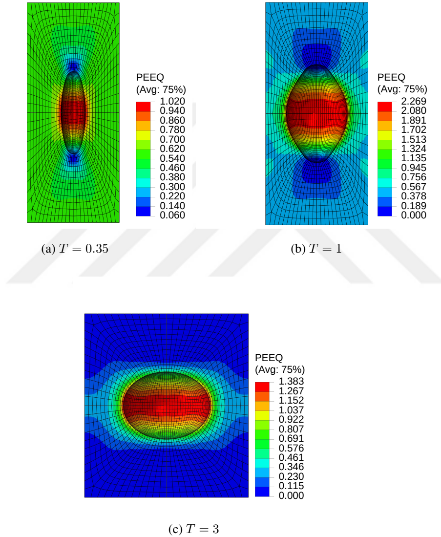
Figure 4.9: Equivalent plastic strain distribution and deformed shapes of the RVE's for f_0 = 0.01 at the onset of void coalescence for (b)(c) and at an arbitrary point for (a).
