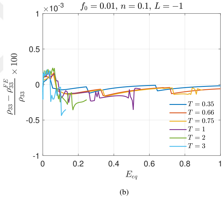
Figure 4.4: The percent error in stress ratios (a) \rho_{11} and (b) \rho_{33} vs equivalent strain for f_0 = 0.01 , n = 0.1 and L = -1 .
