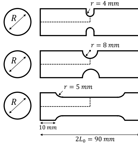
Figure 4.19: Smooth and notched tensile test specimen geometry. Notch radius r = 4 and 8 mm, specimen diameter R = 40 \text{ mm} , length 2L_0 = 90 \text{ mm} , and smooth specimen fillet radius r = 5 \text{ mm} .
