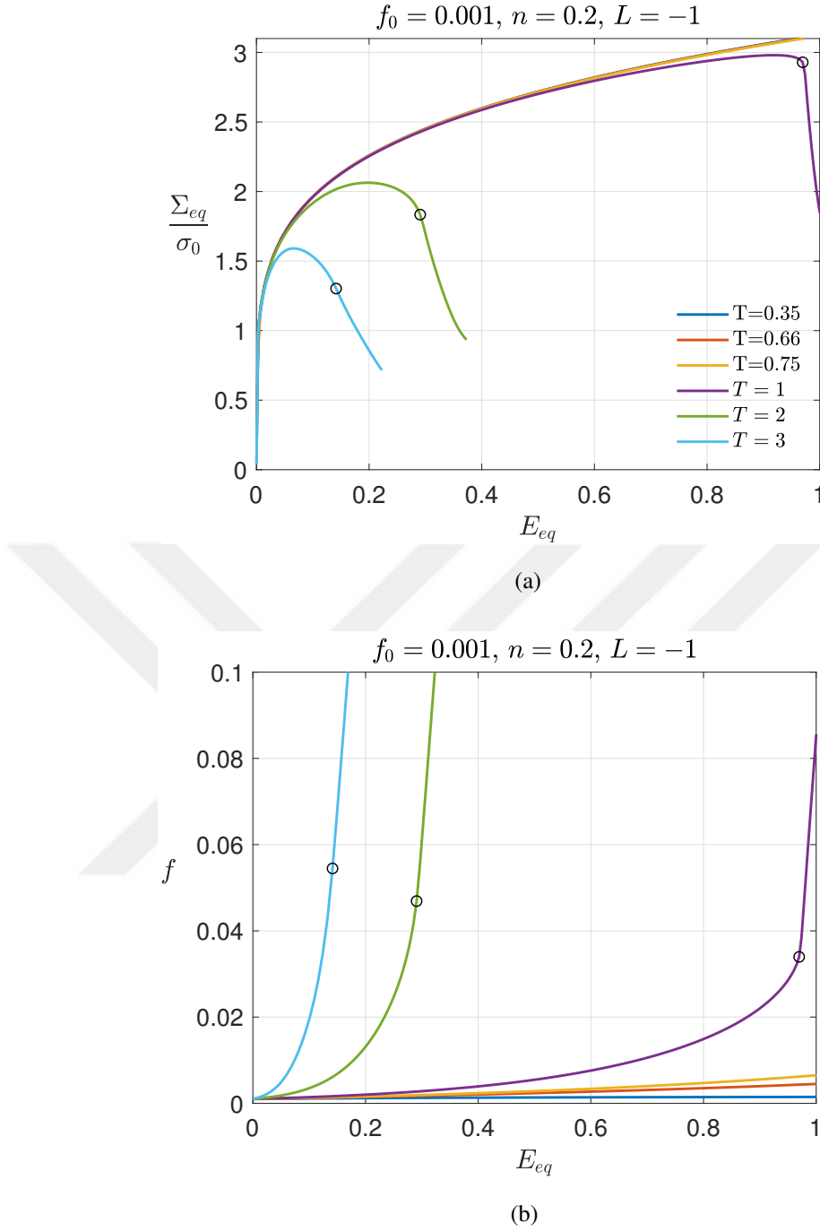
Figure 4.8: Results from the RVE simulations for f_0 = 0.001 , n = 0.2 and L = -1 . (a) Normalized equivalent stress strain relation, (b) void volume fraction, f , vs equivalent strain. The onset of uniaxial straining mode is marked by \circ .
