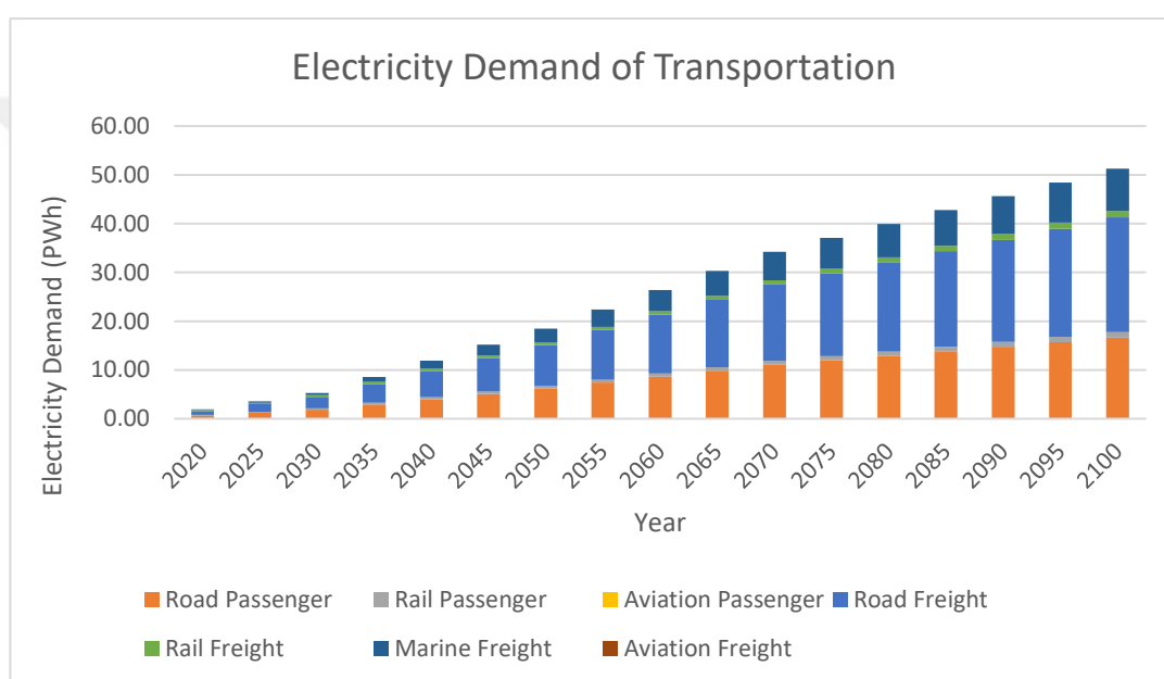
Figure 6-4 Electricity Demand of Transportation
