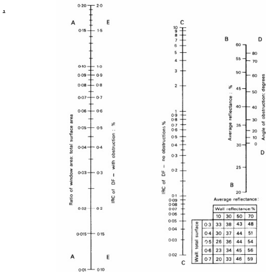
Figure 4.23 Nomogram (Szokolay,1980)
