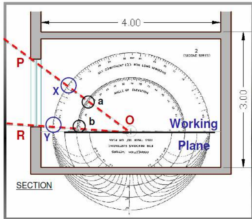
Figure 4.21 Usage of protractor (Szokolay,1980)
