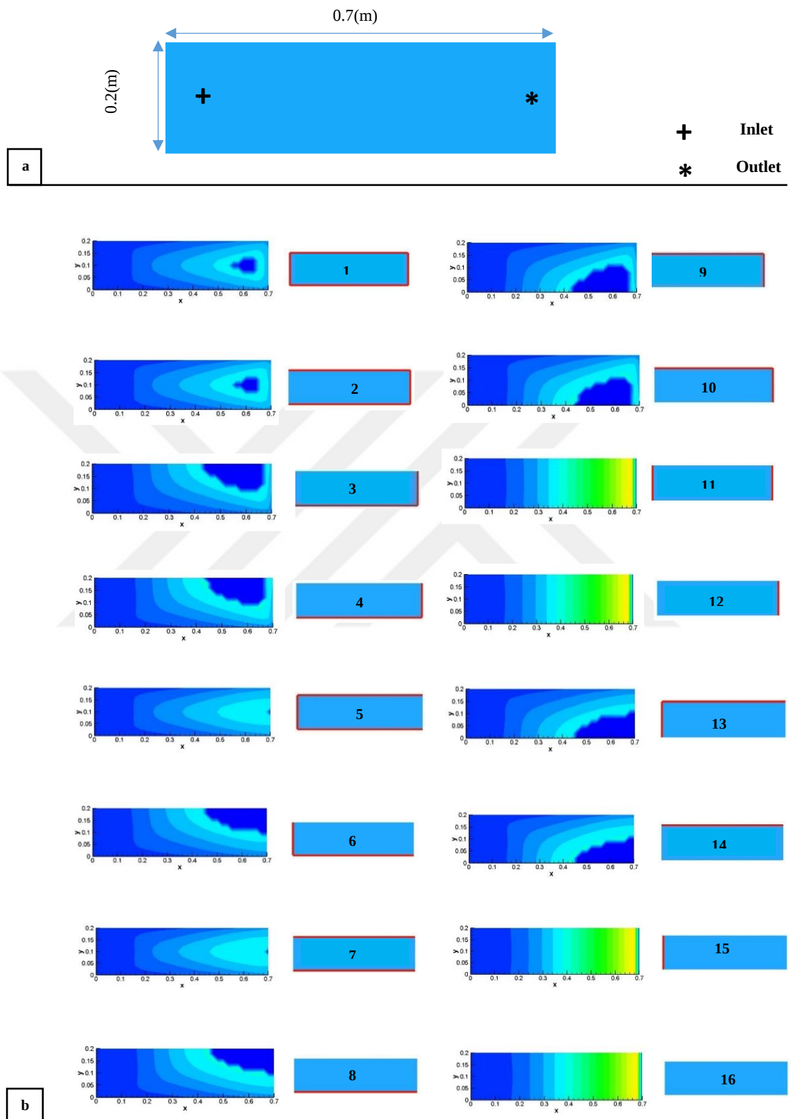
Figure 3.2. (a). Inlet and outlet locations in the given mold (b)flow distribution for different race tracking scenarios
