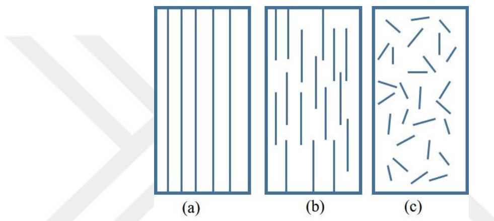
Figure 1.2. Classification of fiber reinforced composites according to the fiber orientation: (a) continuous and aligned fibers (b) discontinuous and aligned fibers (c) discontinuous and randomly oriented fibers
