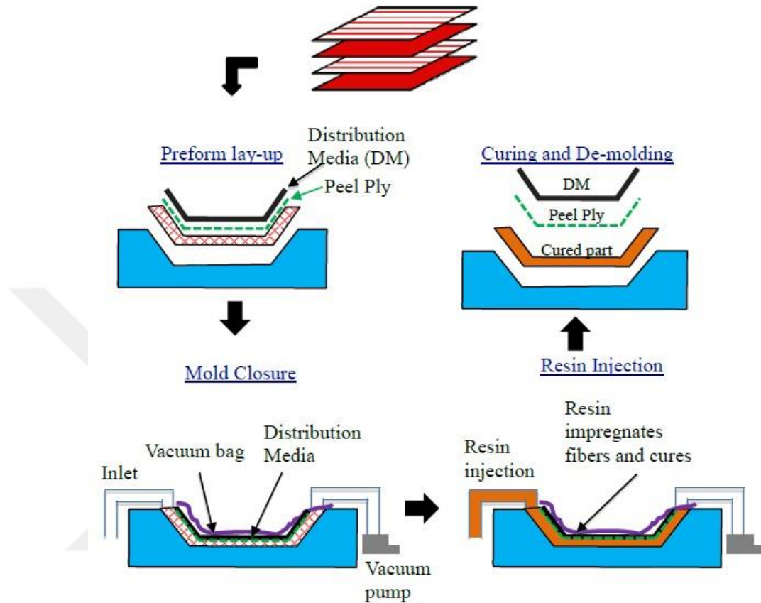
Figure 1.5. Illustration of Seeman Corporation resin infusion molding process (SCRIMP)
