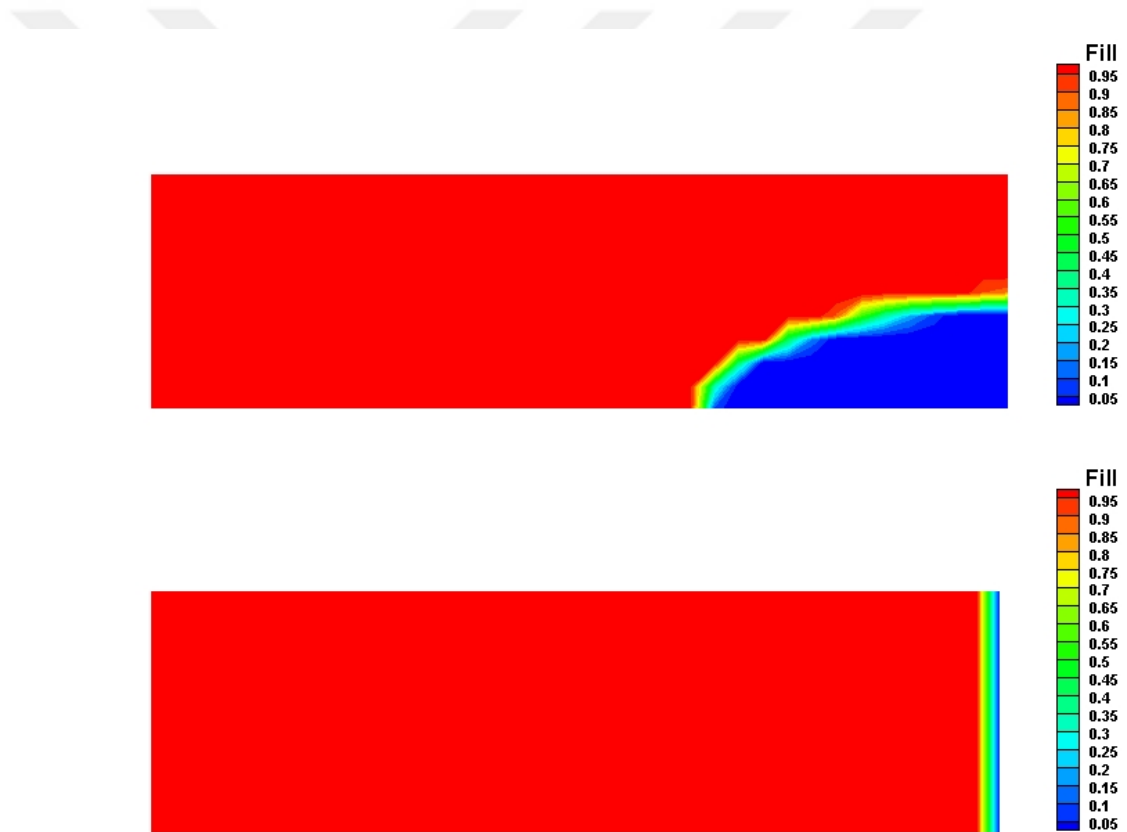
Figure 3.4. Comparison of case 13 (top) and case 16 (bottom) fill factor distribution at the instant where the resin reaches the exit for the first time
