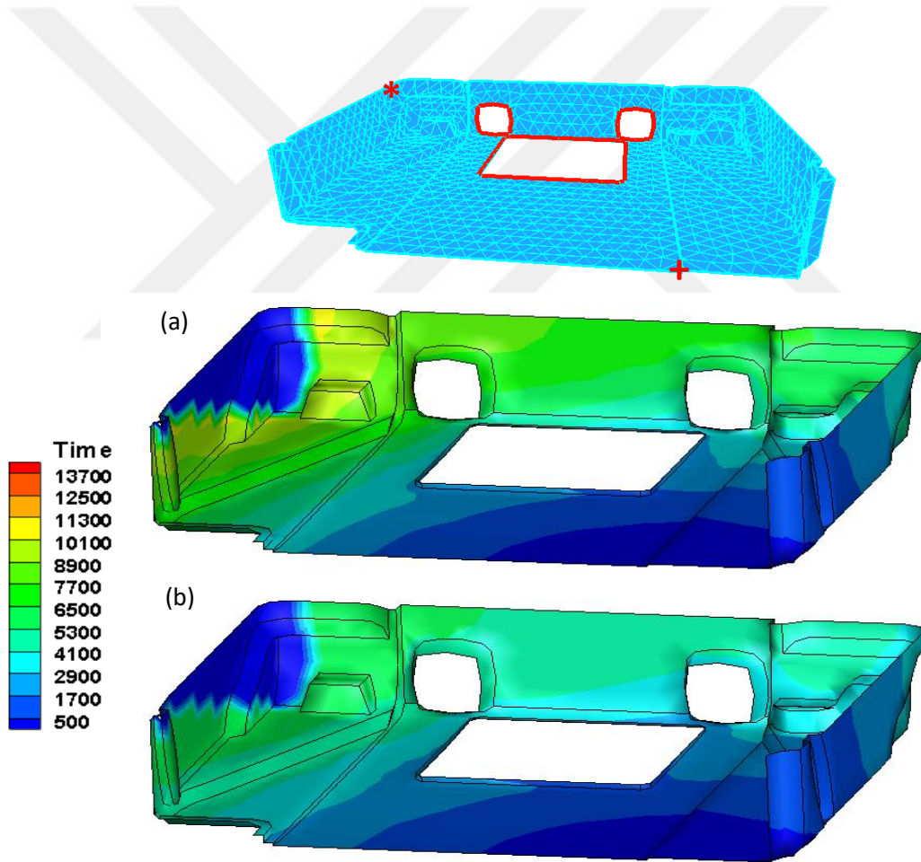
Figure 3.8. Flow distribution with time for (a) \mu=0.0259+0.00004xt Pa.s (b) \mu=0.0259 Pa.s
