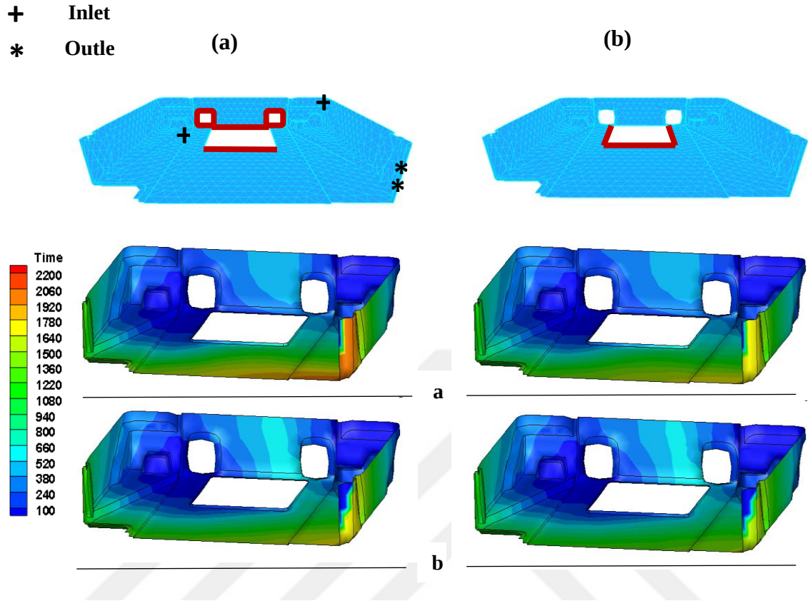
Figure 3.9 Flow distribution with time for two type of viscosity adaptation, \mu=0.0259 Pa.s (right side) and \mu=0.0259+0.00004xt Pa.s (left side)
