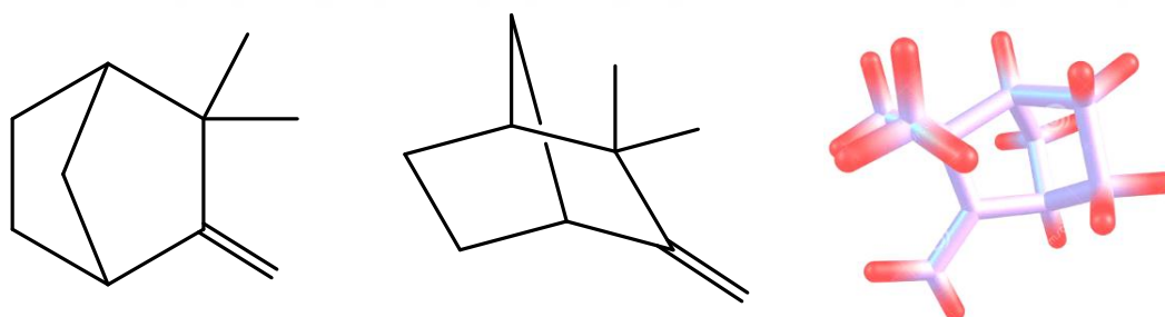
Figure 2.3. (±)-Camphene structure.
