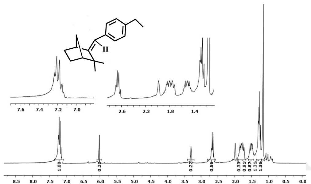
Figure 4.21. ^1\text{H} NMR of (1 S ,4 R )-3-(4-ethylphenyl)-2,2-dimethyl[2.2.1]heptane.
