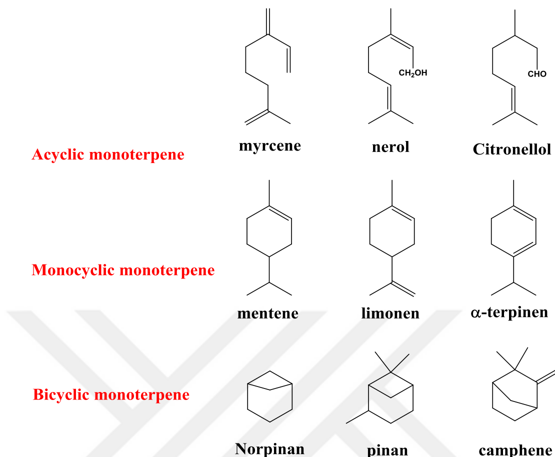
Figure 2.2. Acyclic, monocyclic, and bicyclic monoterpenes.
