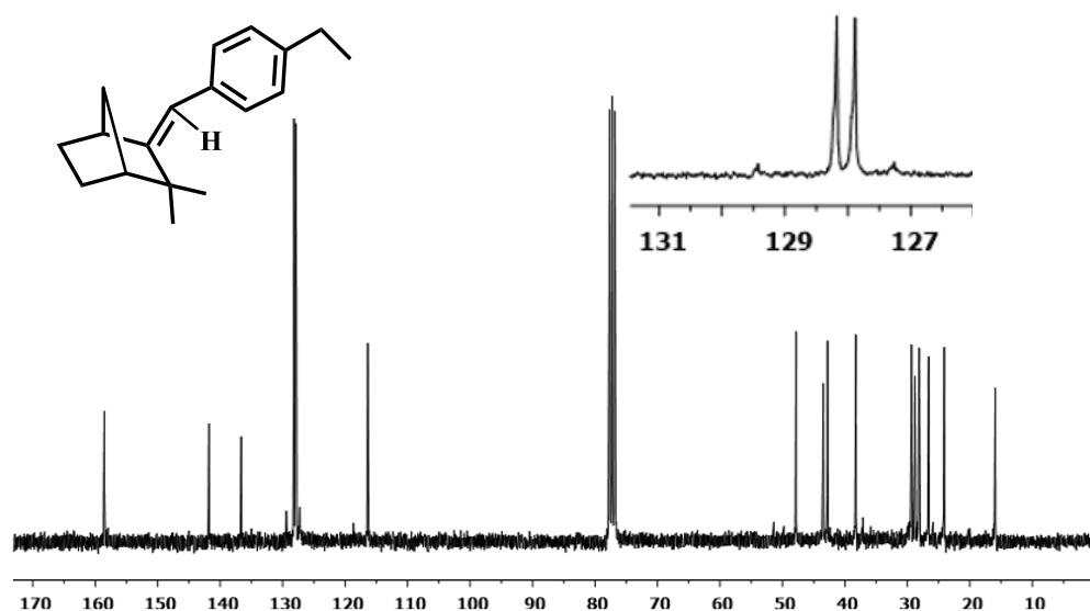
Figure 4.22. ^{13}\text{C} NMR of (1 S ,4 R )-3-(4-ethylphenyl)-2,2-dimethyl[2.2.1]heptane.
