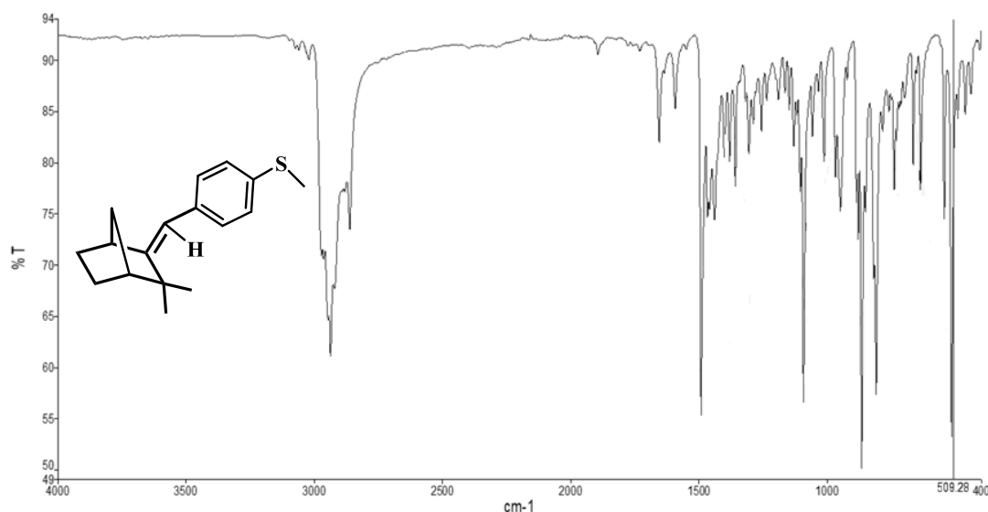
Figure 4.19. FTIR of (1 S ,4 R )-3-(4-thiomethylphenyl)-2,2-dimethyl[2.2.1]heptane.
