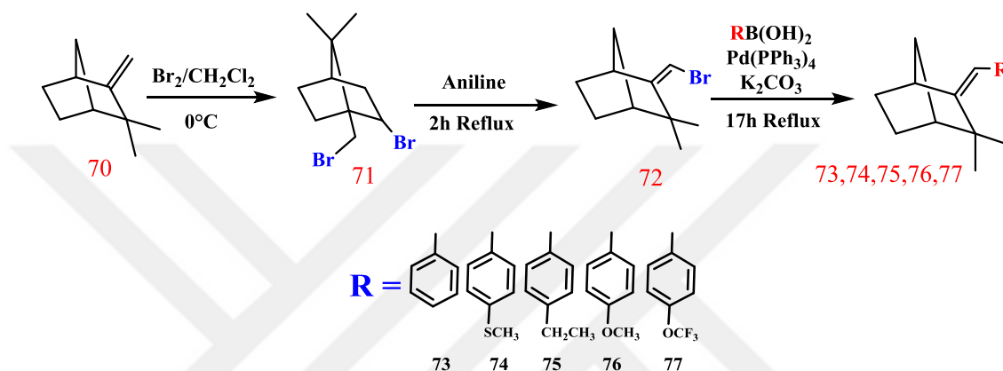
Figure 5.1. New (-)-camphene derivatives reactions.
