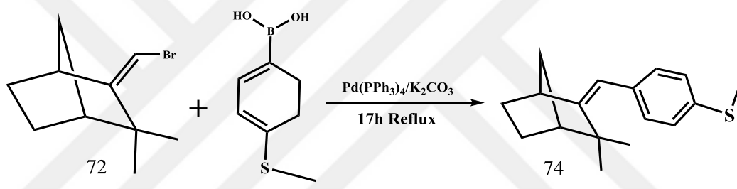
Figure 4.16. (1 S ,4 R )-3-(4-Thiomethylphenyl)-2,2-dimethyl[2.2.1]heptane reaction.
