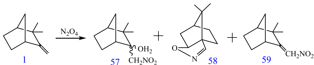
Figure 2.21. ( \pm )-Camphene interaction with N_2O_4 and HNO_3 .
