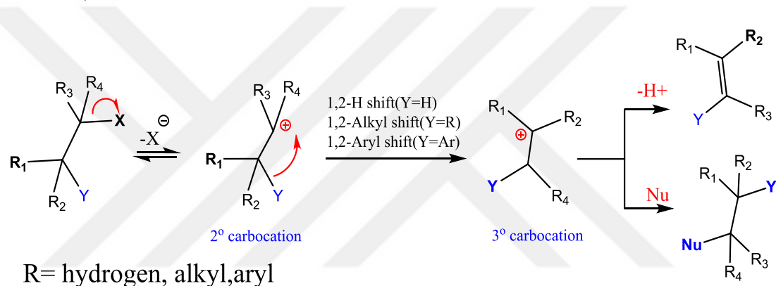
Figure 2.5. Wagner-Meerwein rearrangement mechanisms reaction.
