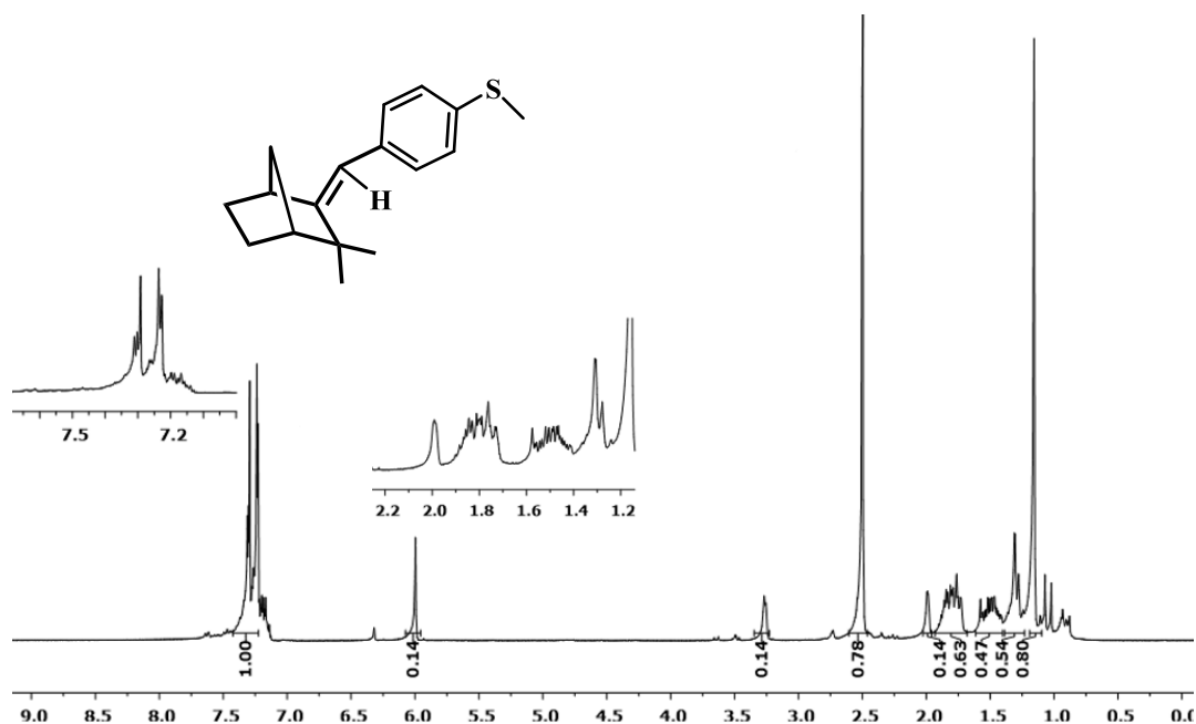
Figure 4.17. ^1\text{H} NMR of (1 S ,4 R )-3-(4-thiomethylphenyl)-2,2-dimethyl[2.2.1]heptane.
