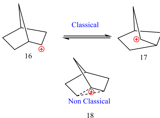
Figure 2.10. Classic and nonclassical carbocation.
