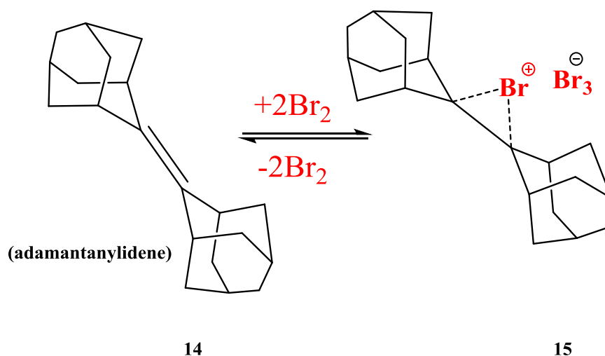
Figure 2.9. Adamantanylidene bromination reaction.
