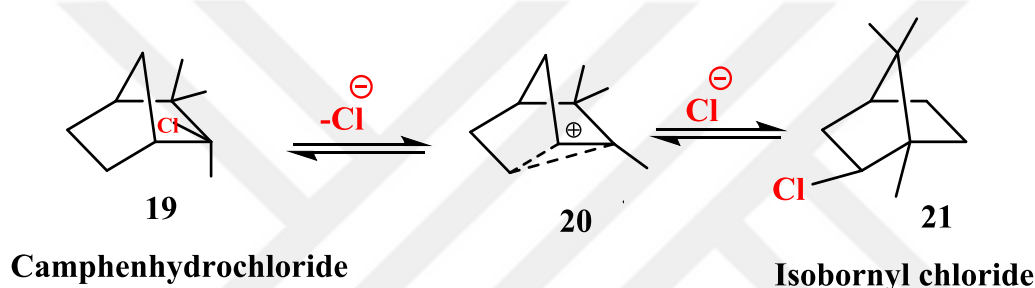
Figure 2.11. Adding chlorine to (±)-camphene.
