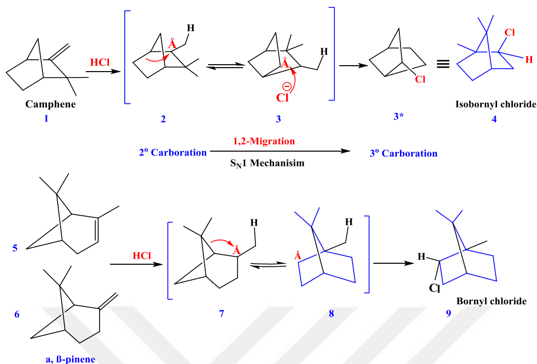
Figure 2.6. ( \pm )-Camphene is transformed into isobornyl.
