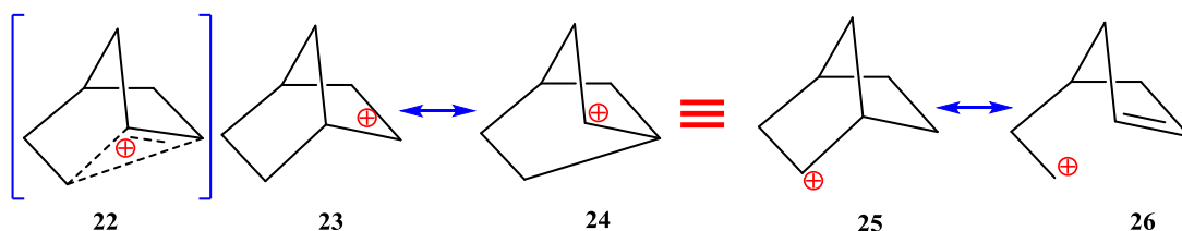
Figure 2.12. Mechanism of adding chlorine to norbornyl.
