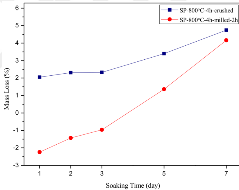
Figure 7.17. Mass loss (%) values of wafers with respect to soaking time
