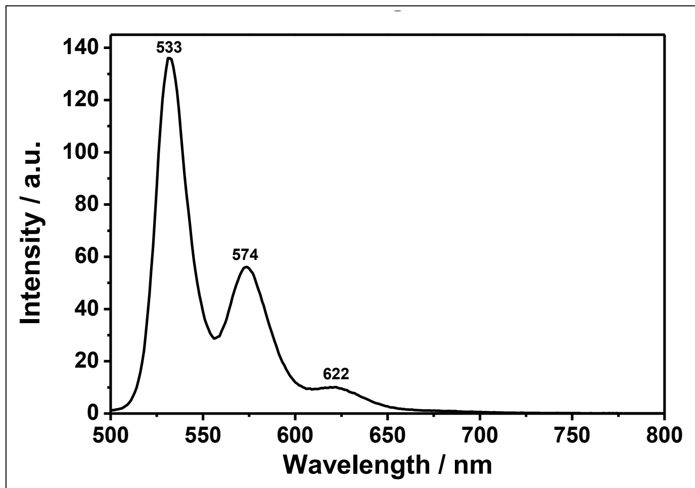
Figure 4.8: Emission spectrum ( \lambda_{\text{exc}} = 485 \text{ nm} ) of HE-PDI in CHL
