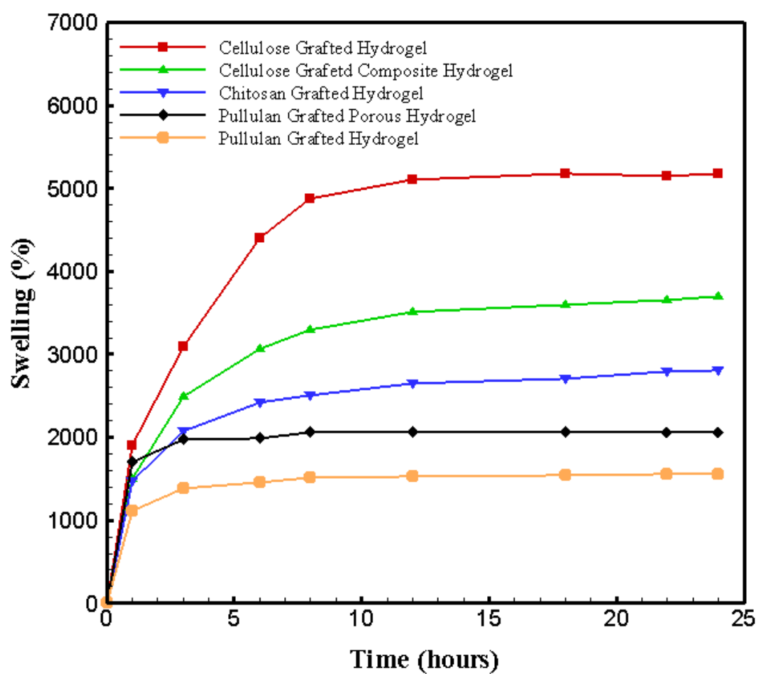
Figure 12. Effect of time on swelling behavior of cellulose, chitosan, and pullulan grafted hydrogels and porous and composite hydrogels
