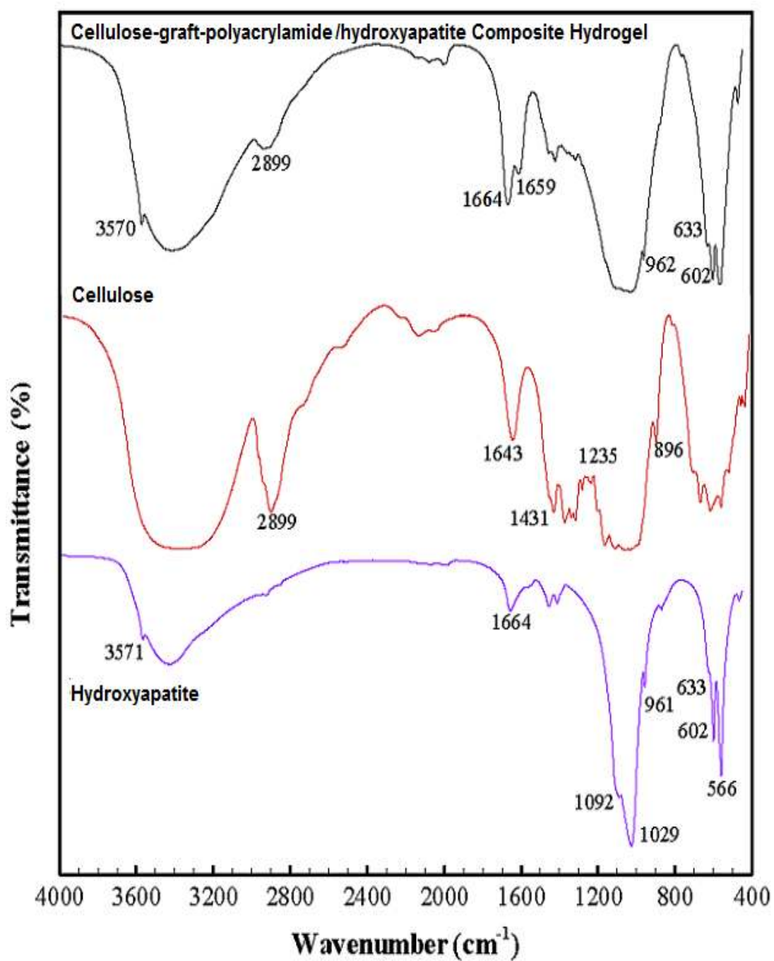
Figure 7. FTIR spectra of cellulose, hydroxyapatite and its grafted polyacrylamide composite hydrogel in the range 500–4000 cm -1
