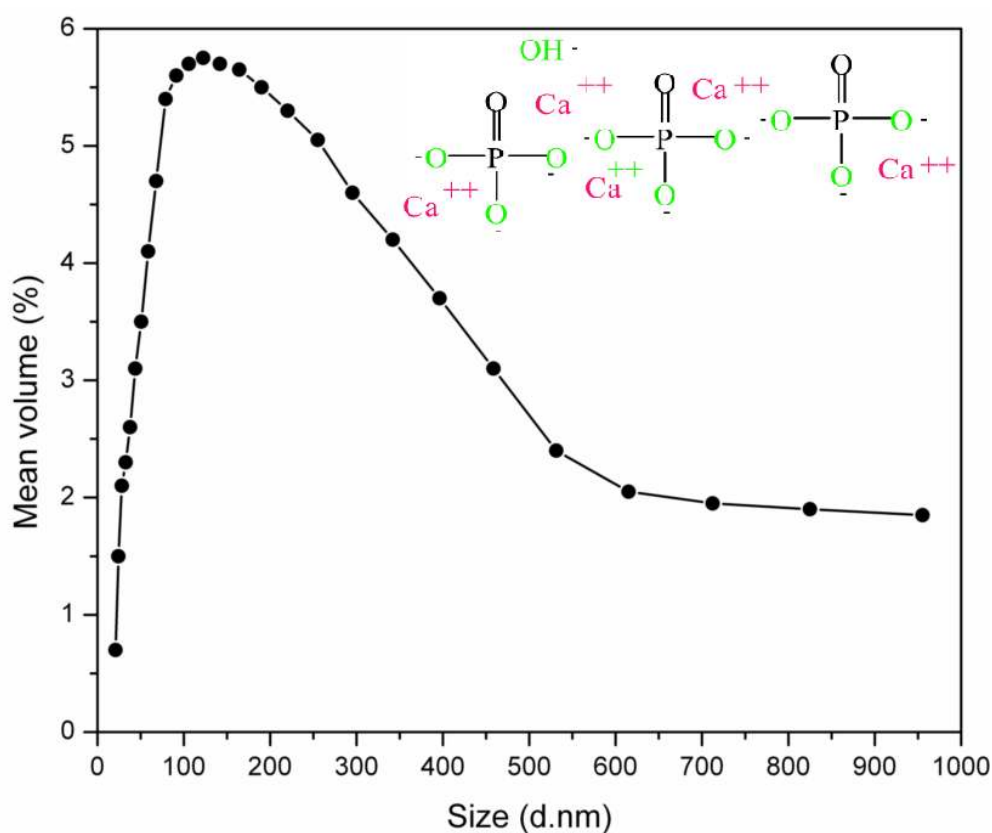
Figure 5. Size distribution curve of synthesized nano-hydroxyapatite, inset shows the nano-hydroxyapatite structure
