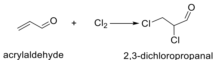
Figure 6.3. Reaction mechanism for synthesized 2,3-dichloropropanal
