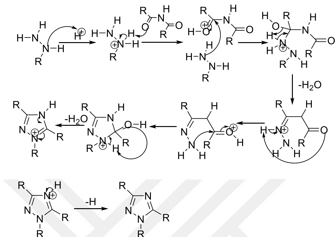
Figure 2.5. Einhorn-Brunner reaction mechanism
