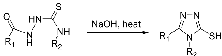
Figure 2.11. 1,2,4-Triazole-5-thions derivatives
