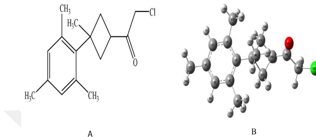
Figure 7.18. Structure of the compound (5) A) Drawing by ChemBioDraw Ultra B) Gaussian Optimized by B3LYP/cc-pVDZ
