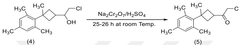
Figure 6.7. Reaction for synthesis 2-chloro-1-(3-methyl-3-mesityl-cyclobutyl)-ethanone (5)
