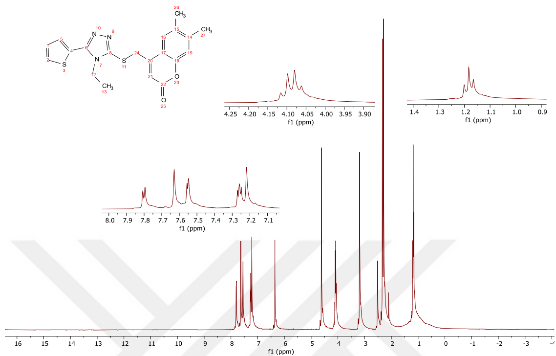
Figure 7.53. Experimental ^1\text{H} -NMR spectrum for compound (9) in DMSO- d_6
