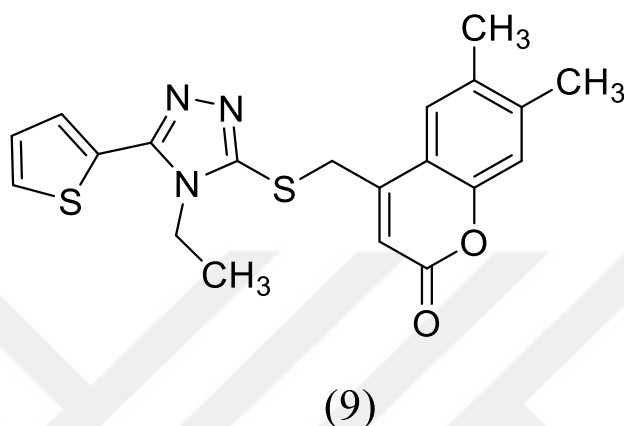
Figure 7.49. 4-(((4-ethyl-5-(thiophen-2-yl)-4H-1,2,4-triazol-3-yl)thio)methyl)-6,7-dimethyl-2H-chromen-2-one
