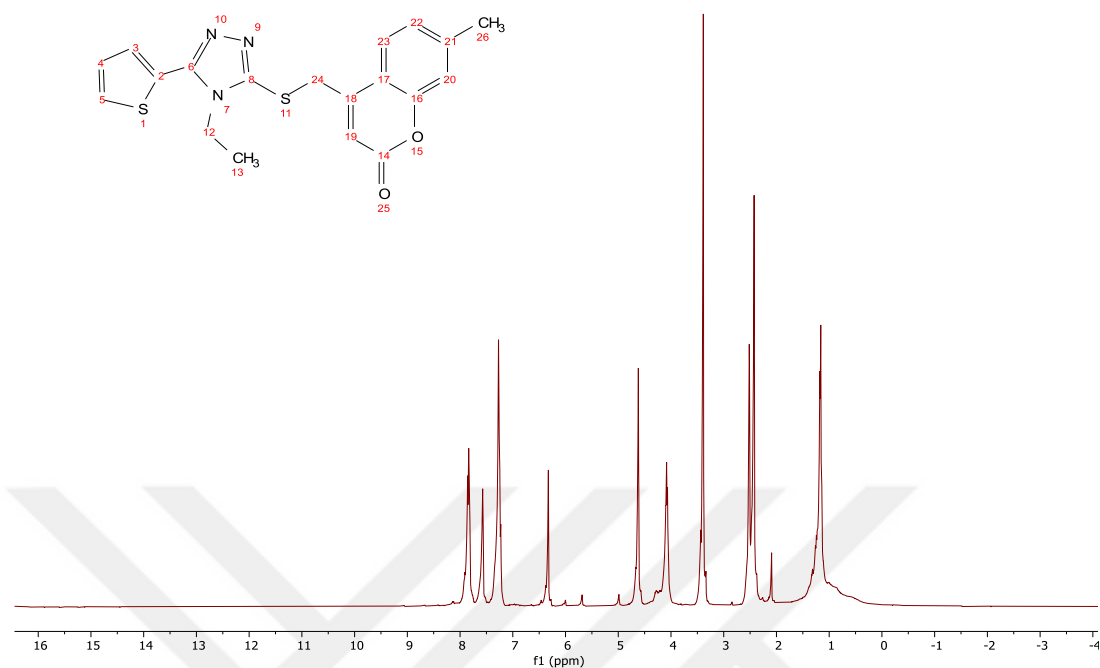
Figure 7.37. Experimental ^1\text{H} -NMR spectrum for compound (7) in DMSO- d_6
