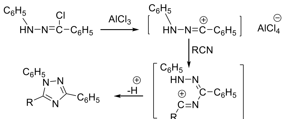
Figure 2.6. Hand reaction of 1,3-diphenyl-5-alkyl-1H-1,2,4-triazole.
