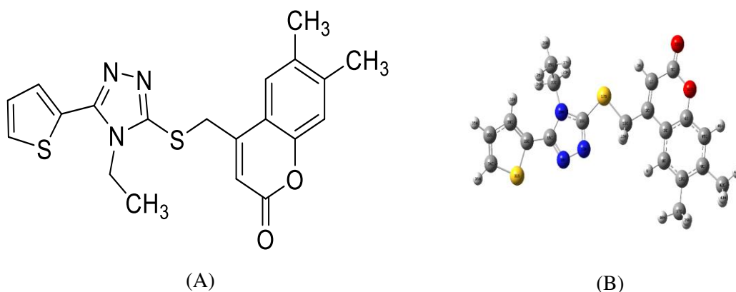
Figure 7.50. Structure of the compound (9) A) Drawing by ChemBioDraw Ultra B) Gaussian Optimized by B3LYP/cc-pVDZ
