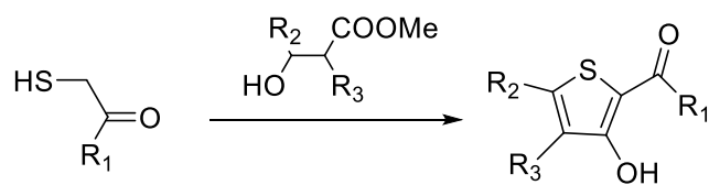
Figure 3.6. Fieser synthesis
