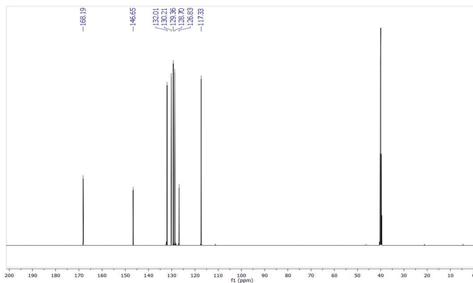
Figure 7.6. The experimental ^{13}\text{C} -NMR spectrum for compound (1) in DMSO- \text{d}_6
