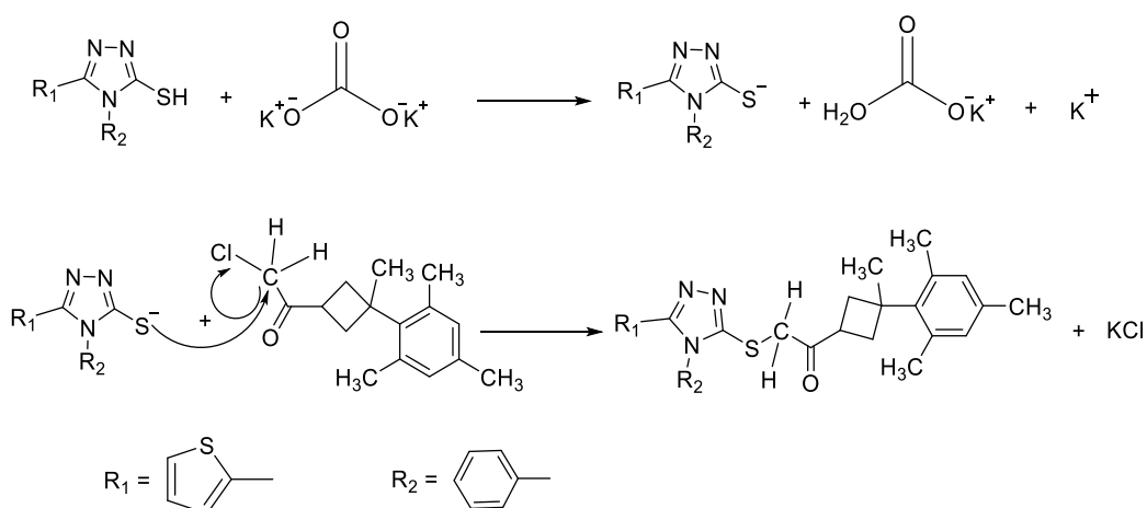
Figure 8.4. Reaction mechanism for the formation of sulfanyl compounds containing triazole and cyclobutane ring.
