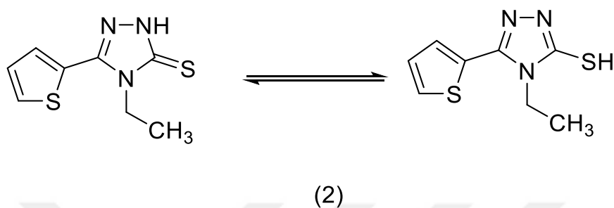
Figure 7.9. 4-Ethyl-5-(thiophene-2-yl)-4H-1,2,4-triazole-3-thiol
