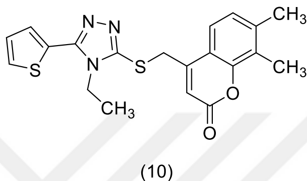
Figure 7.57. 4-(((4-ethyl-5-(thiophen-2-yl)-4H-1,2,4-triazol-3-yl)thio)methyl)-7,8-dimethyl-2H-chromen-2-one
