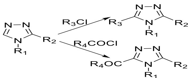
Figure 2.18. 3,4,5-Trisubstituted-1,2,4-triazoles
