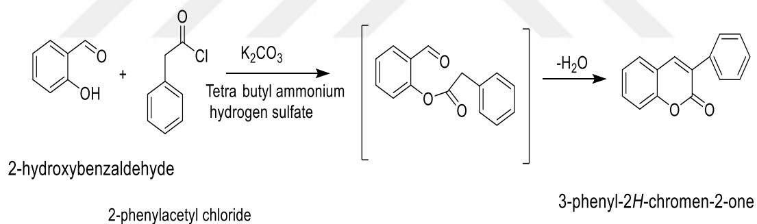
Figure 5.6. Synthesis phenyl coumarin
