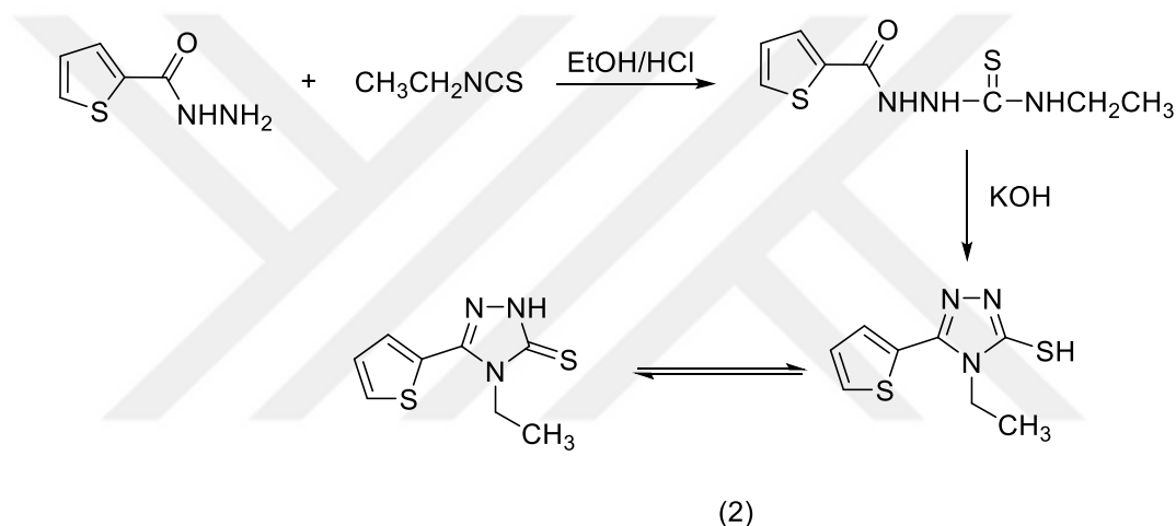
Figure 6.2. Reaction for synthesis 4-ethyl-5-(thiophen-2-yl)-4H-1,2,4-triazole-3-thiol (2)
