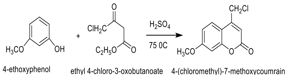
Figure 5.2. Synthesized 4-(Chloromethyl)-7-methylcoumarin
