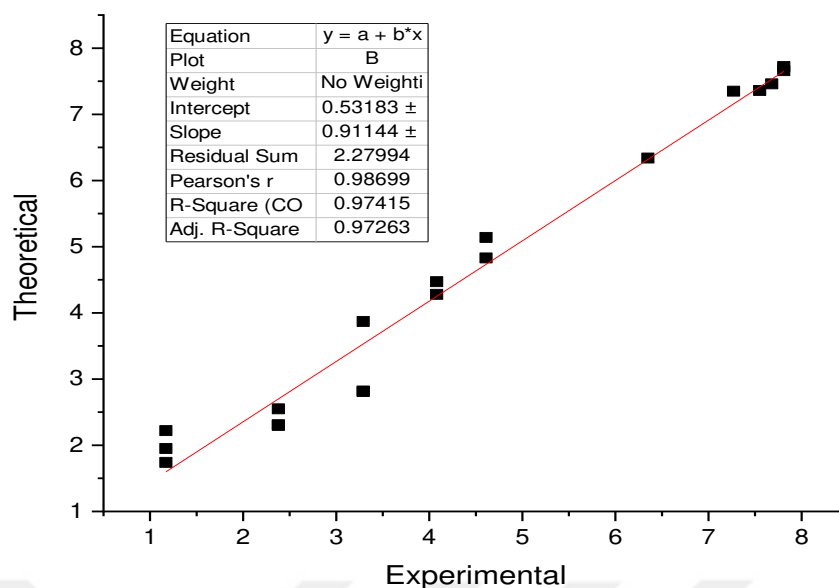
Figure 8.19. The ^1\text{H} -NMR correlation between experimental and theoretical calculation for 4-(((4-ethyl-5-(thiophen-2-yl)-4H-1,2,4-triazol-3-yl)thio)methyl)-7,8-dimethyl-2H-chromen-2-one
