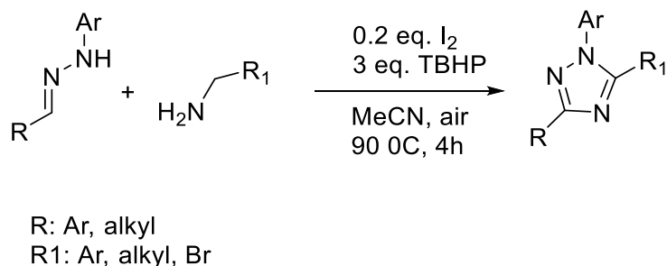
Figure 2.7. Formation recreation of 1,3,5-trisubstituted 1,2,4-triazole compounds as a result of the reaction of hydrazone and aliphatic amines.
