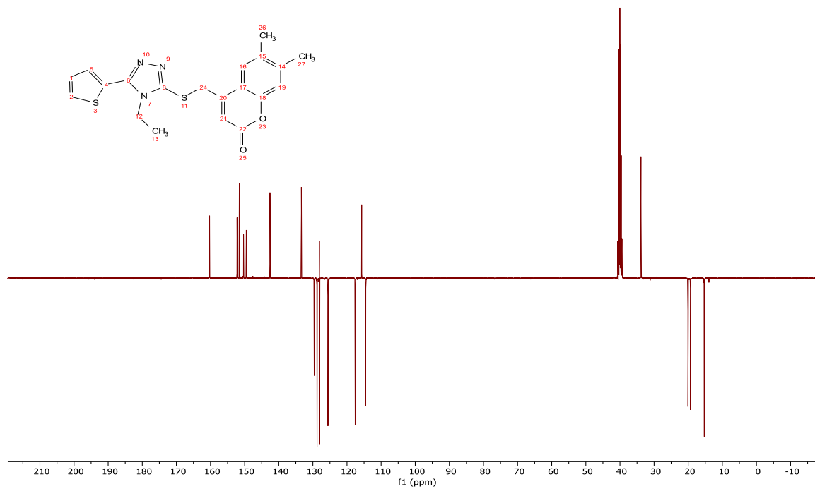
Figure 7.54. The experimental ^{13}\text{C} -NMR spectrum for compound (9) in DMSO- d_6
