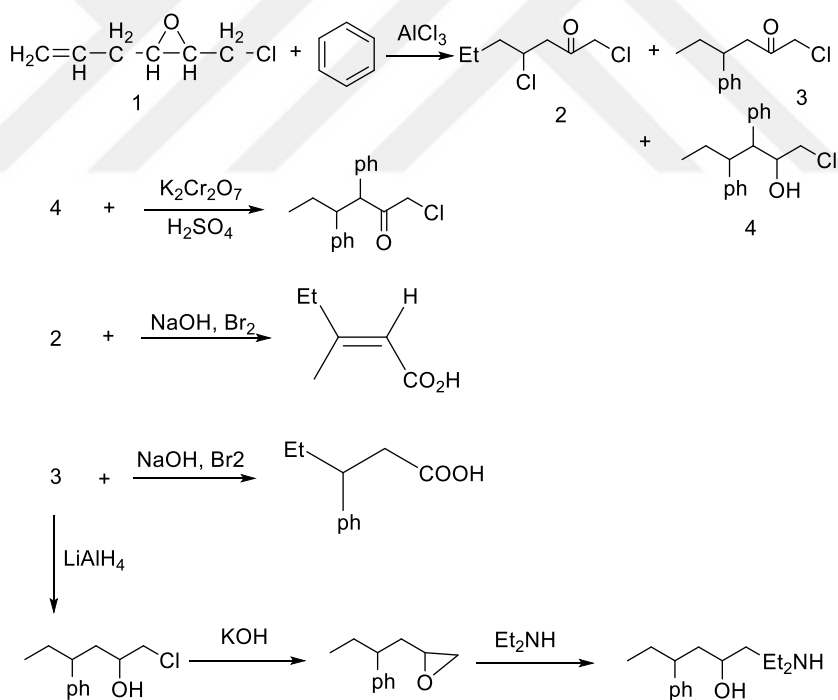
Figure 4.8. Synthesis of oxirane compounds
