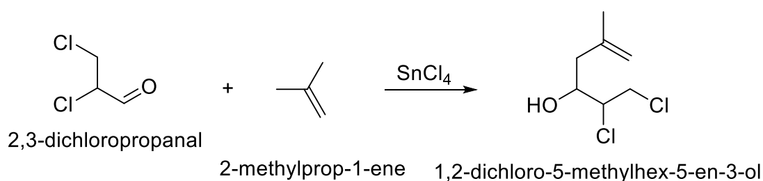
Figure 6.4. Reaction mechanism for synthesized 1,2-dichloro-5-methylhex-5-en-3-ol
