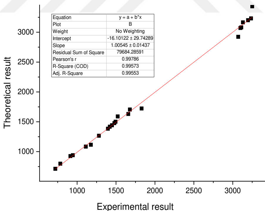
Figure 7.44. Relationship graphics for compound (8), between theoretical and experimental frequencies
