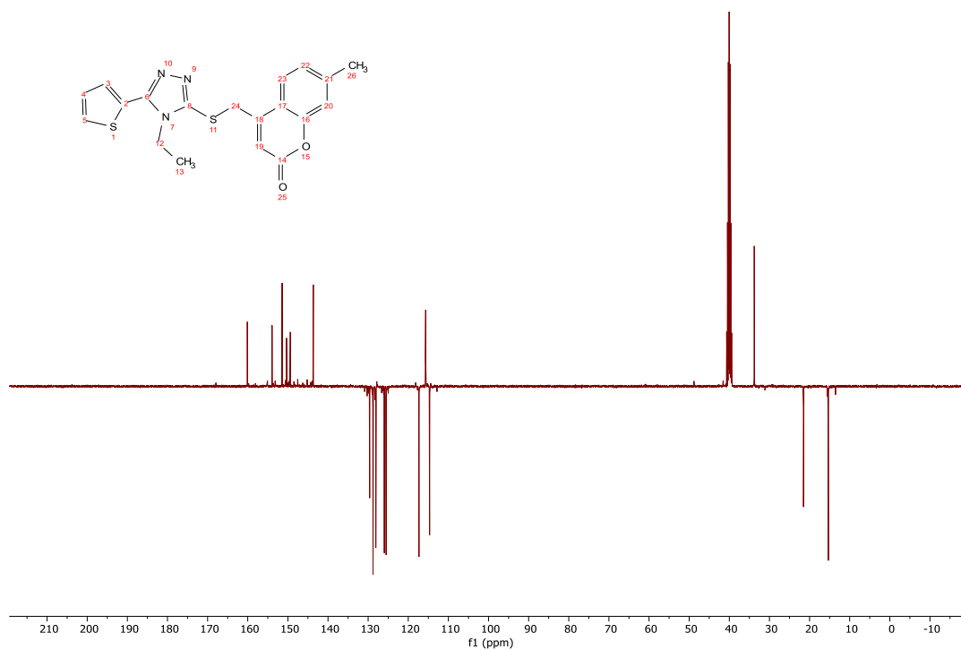
Figure 7.38. The experimental ^{13}\text{C} -NMR spectrum for compound (7) in DMSO- d_6
