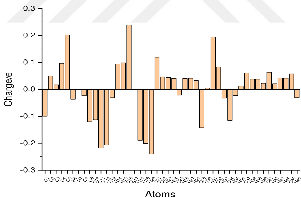
Figure 7.56. Millikan charge distribution on the compound (9)
