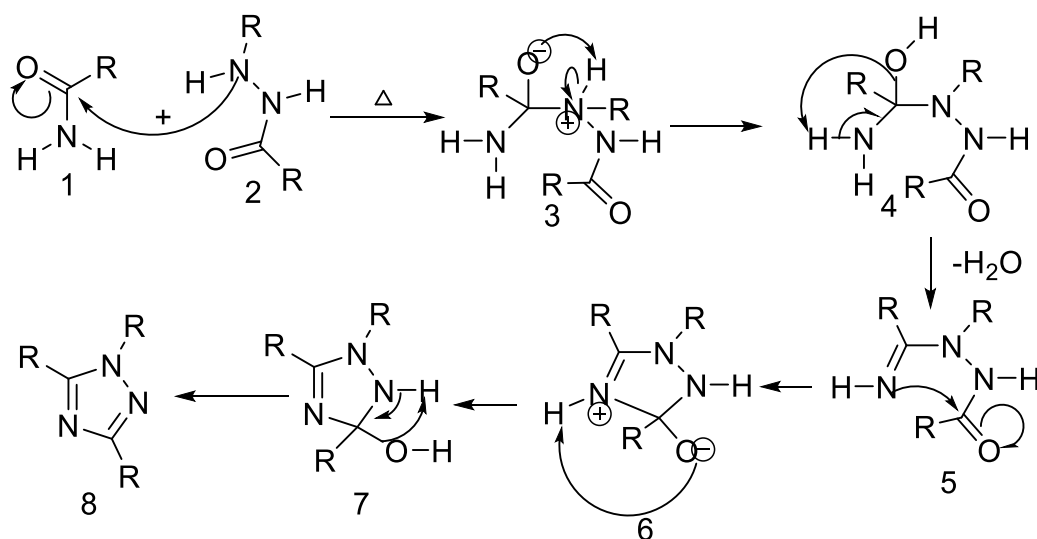
Figure 2.3. Mechanism of pellizzari reaction.
