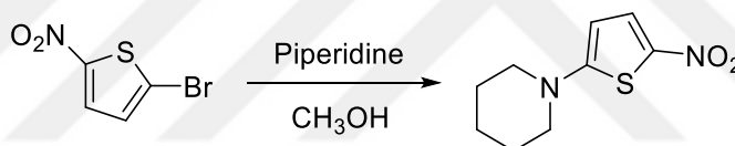
Figure 3.12. Nucleophilic reaction of thiophene
