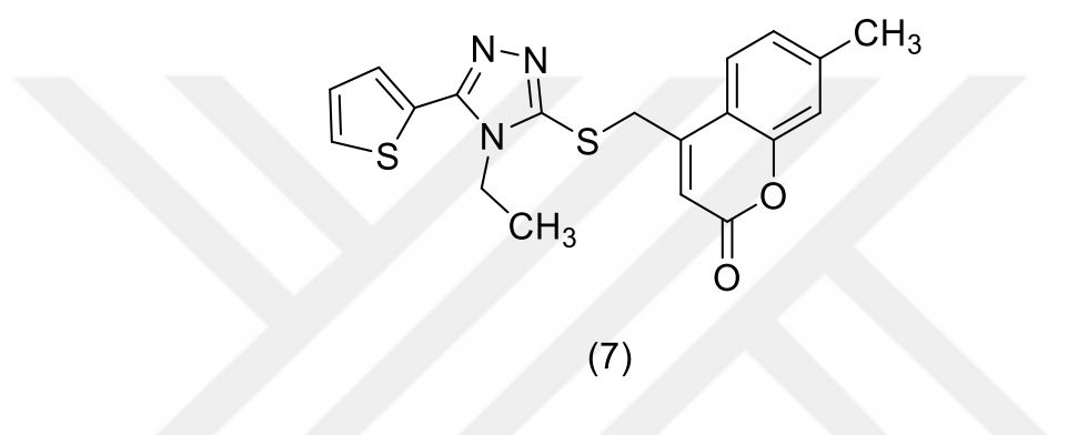
Figure 7.33. 4-(((4-ethyl-5-(thiophen-2-yl)-4H-1,2,4-triazol-3-yl)thio)methyl)-7-methyl-2H-chromen-2-one
