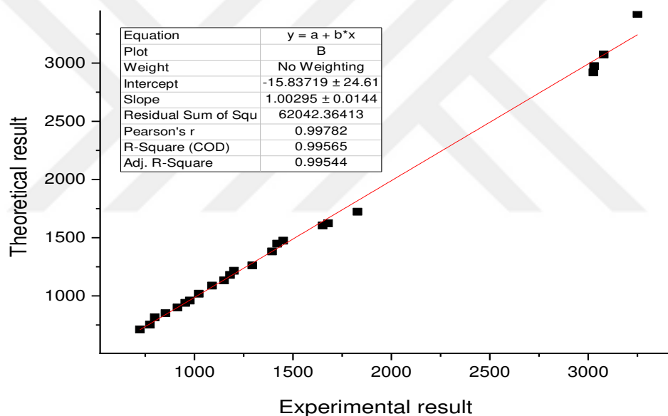
Figure 7.60. Relationship graphics for compound (10), between theoretical and experimental frequencies
