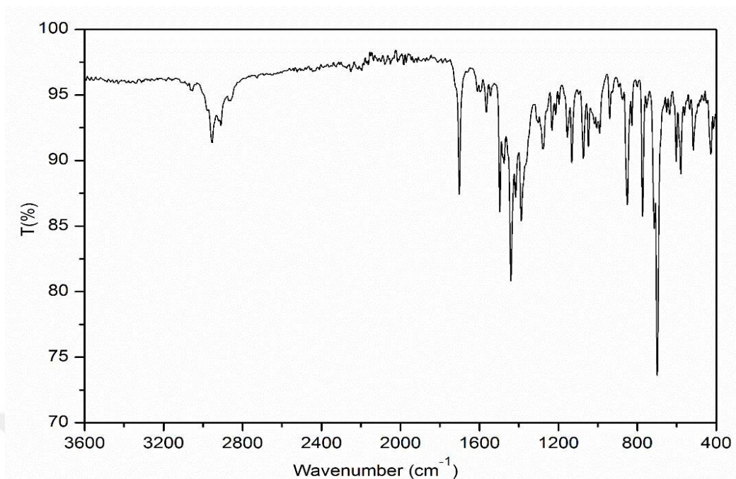
Figure 8.9. Representation of structure-specific characteristic peaks in the FTIR spectrum belonging to 1-(3-methyl-3-mesityl)-cyclobutyl-2-[[5-(thiophen-2-yl)-4-phenyl-4H-1,2,4 triazol-3-yl] sulfanyl]-ethanone
