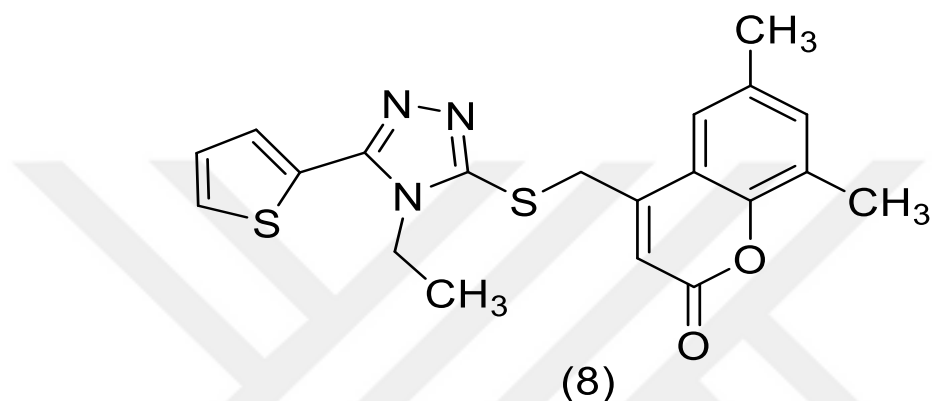
Figure 7.41. 4-(((4-ethyl-5-(thiophen-2-yl)-4H-1,2,4-triazol-3-yl)thio)methyl)-6,8-dimethyl-2H-chromen-2-one
