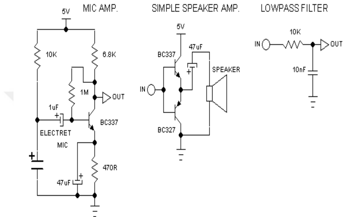
Figure 3.10 audio ampliphicator, low pass circuit, triggering circuit and audio transmitter module
