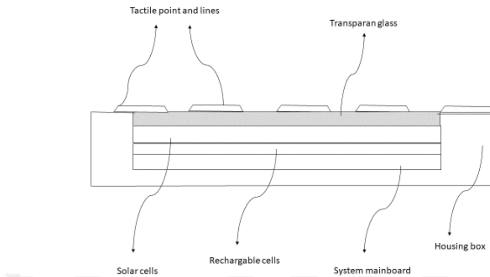
Figure 1.6- View of the designed embedded Audio knowledge transmitter unit
