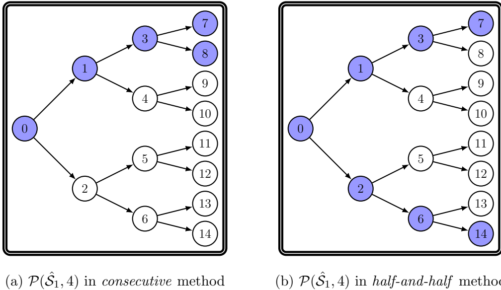
Figure 5.2: Problems solved to compute an upper bound in different selection strategies
