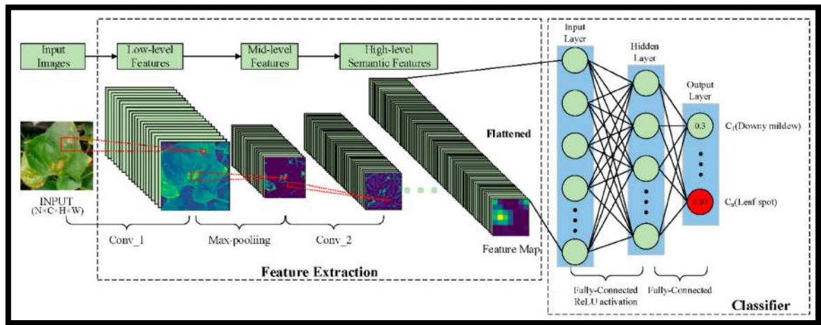
Figure 3.4: Full Convolutional Neural Networks For Detection And Classification Of Agricultural Pest And Vermin's.
