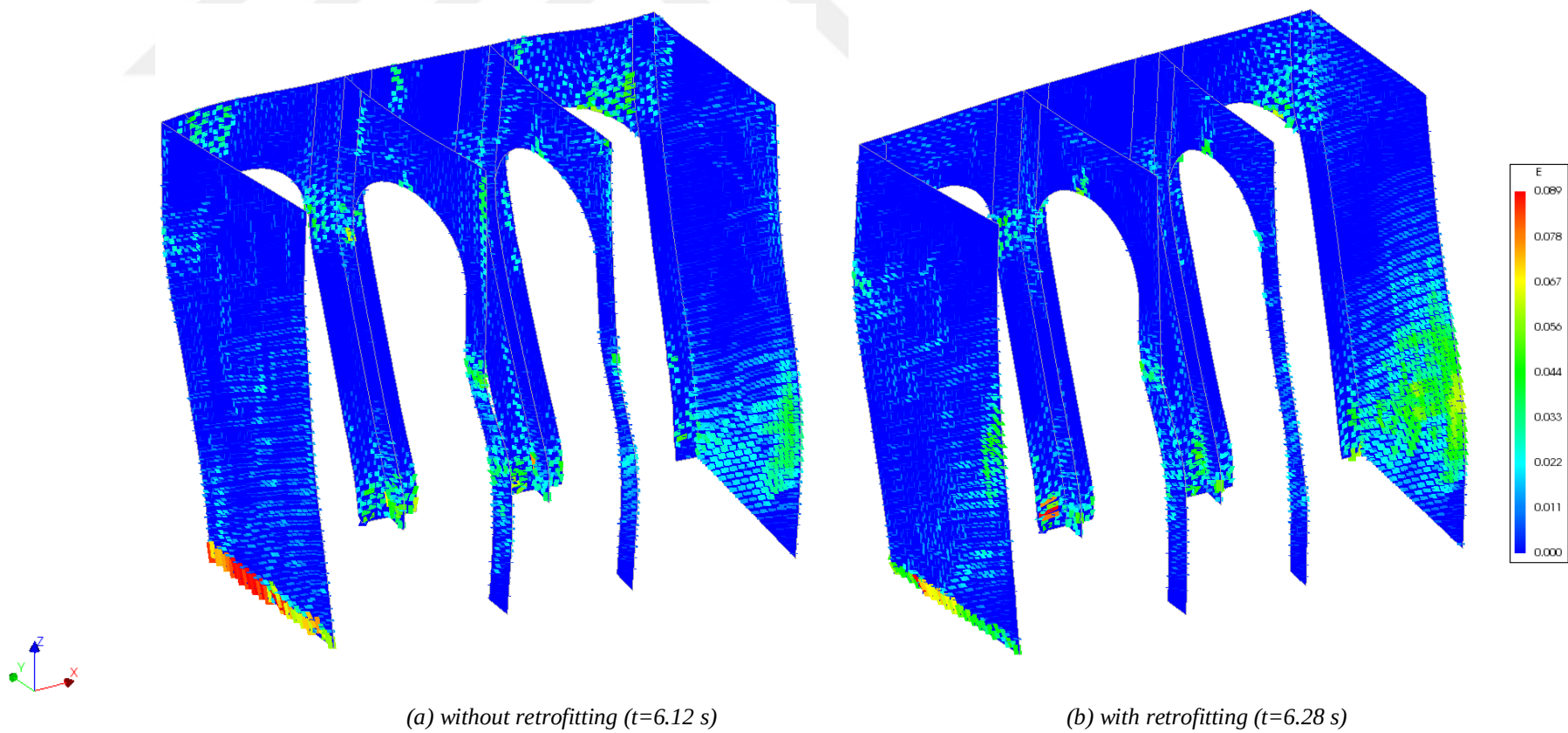
Figure A2. 11. Principal tensile strains of portico, deformed shape scale factor:5, the Bolu Earthquake
