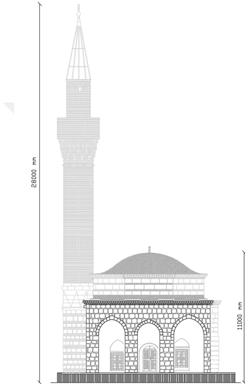
Figure A1. 1. North façade
