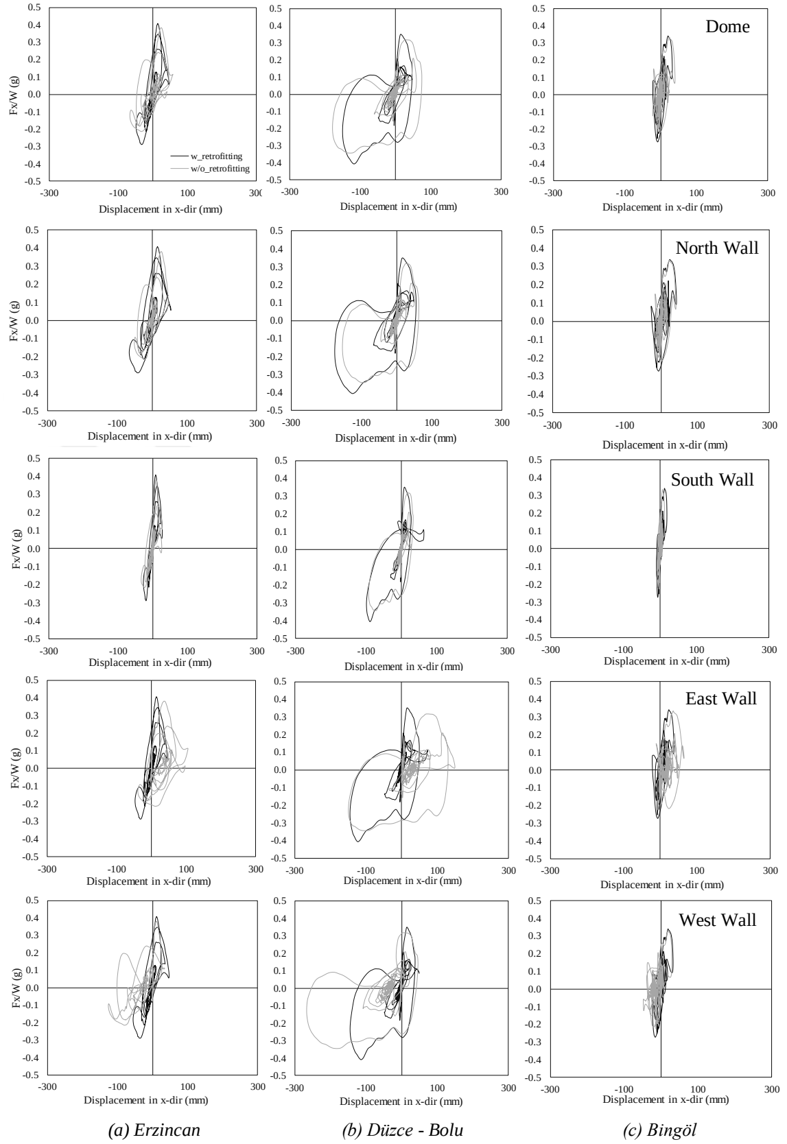
Figure 6.28. Change in the hysteretic response in the transversal direction
