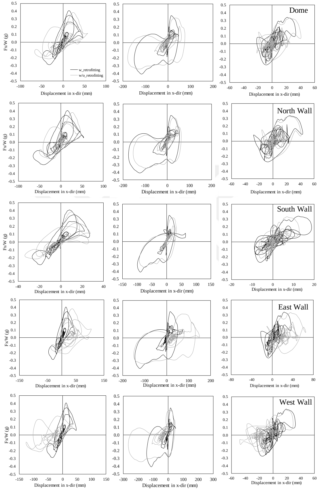
(a) Erzincan (b) Düzce - Bolu (c) Bingöl Figure 6.30. Change in the hysteretic response in the X direction, detailed
