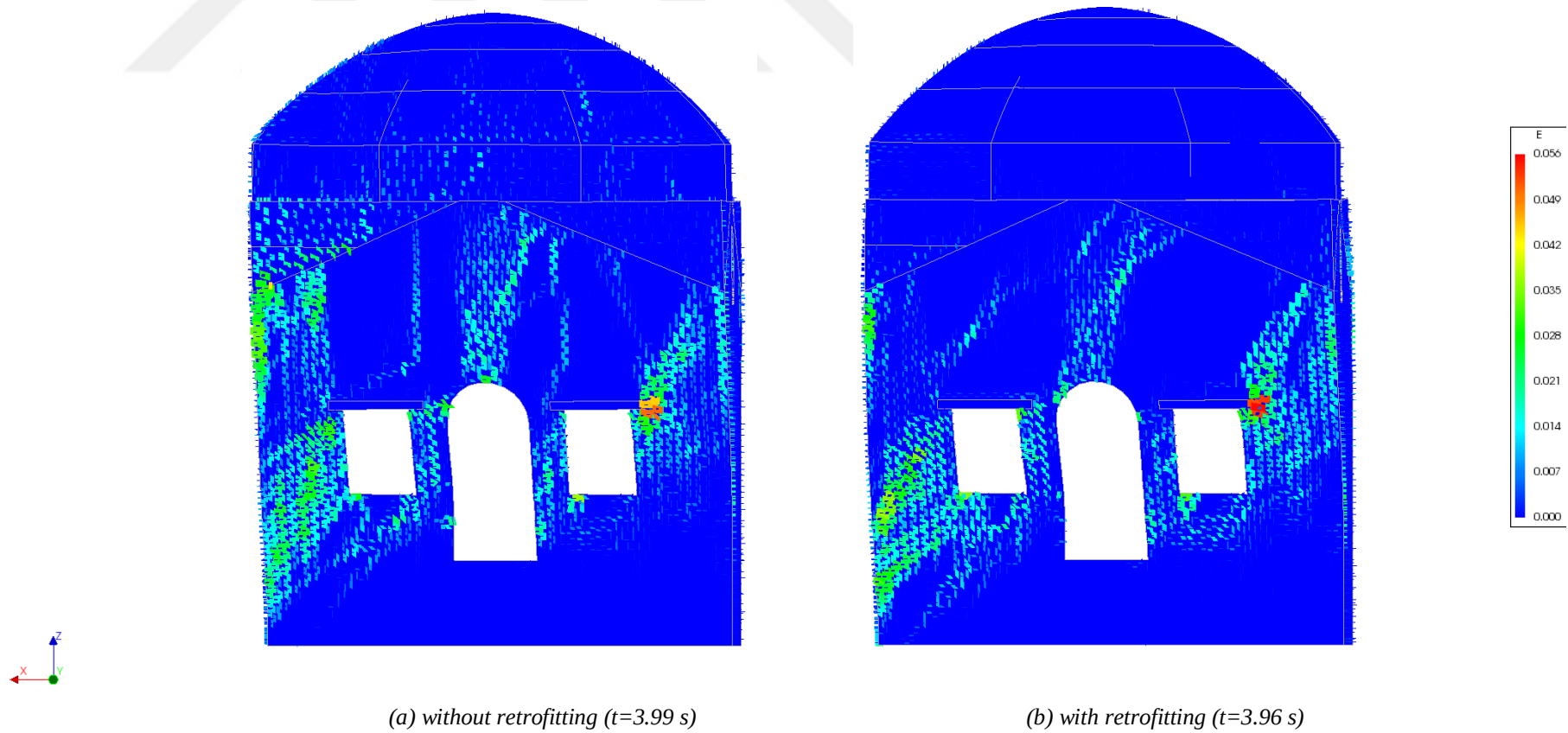
Figure A2. 14. Principal tensile strains of North Wall without portico, deformed shape scale factor:5, the Bingöl Earthquake
