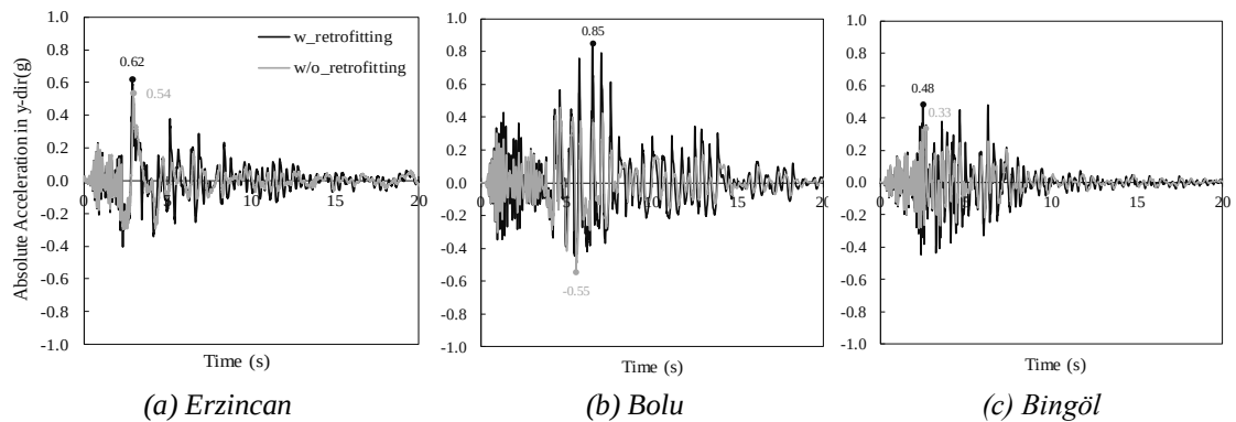
Figure 6.25. Change in absolute acceleration demand in longitudinal direction
