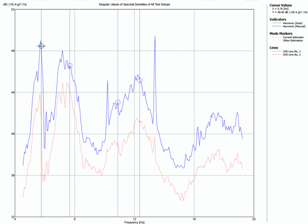
Figure 4.4. Singular values of spectral densities of all setups, EFDD method
