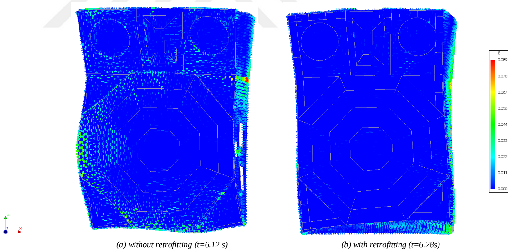
Figure A2. 10. Principal tensile strains of dome, deformed shape scale factor:5, the Bolu Earthquake
