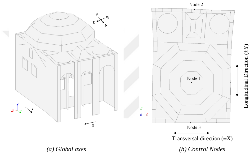
Figure 5.1. Global coordinate system and defined control nodes
