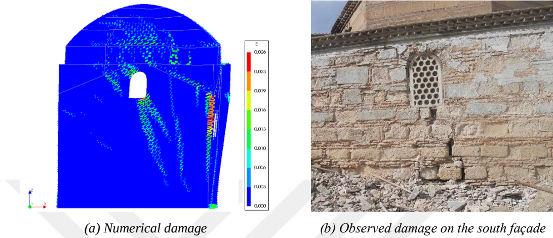
Figure 5.3. The non-retrofitted numerical and real damage on the south wall, maximum principal strain distribution at load factor 0.27g in +X direction
