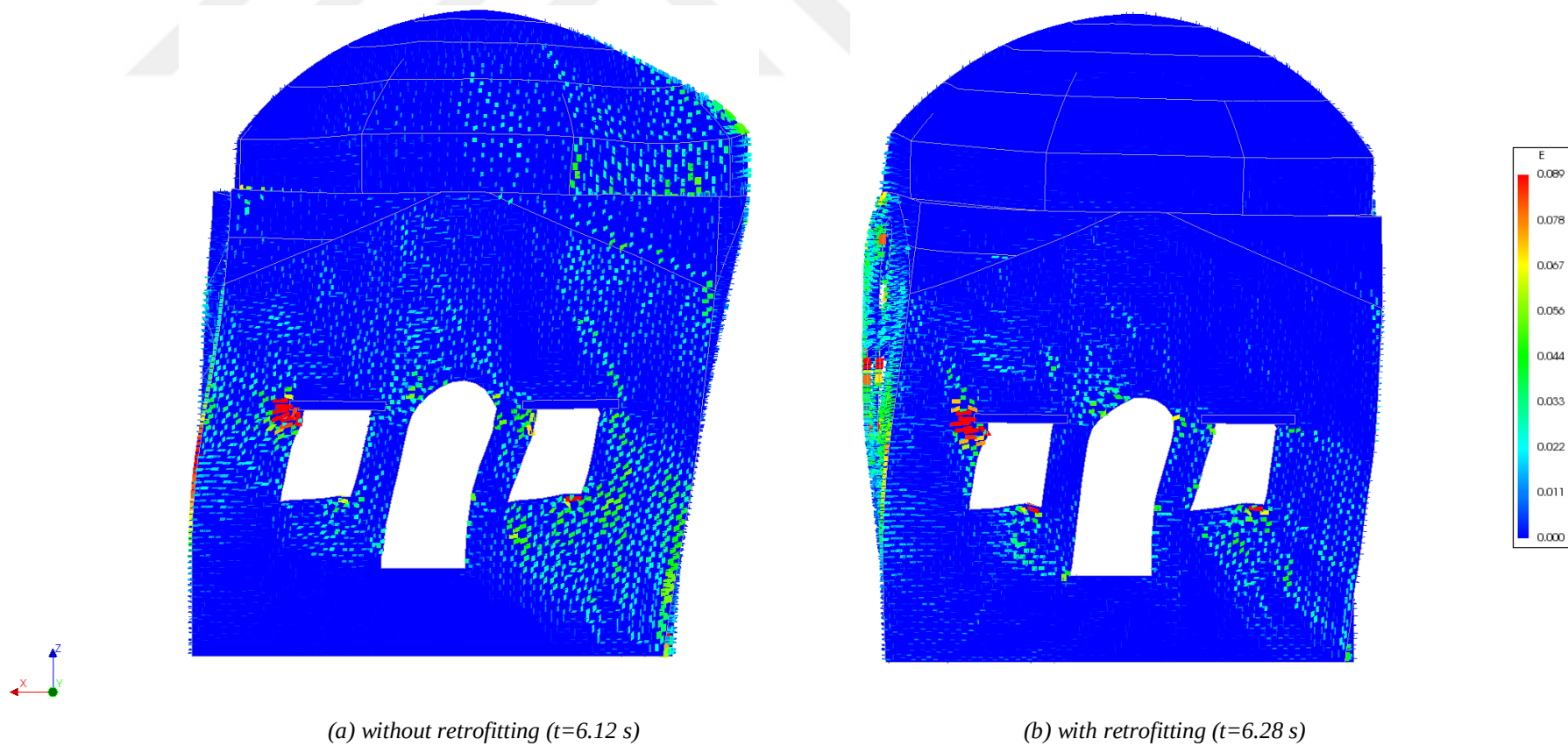
Figure A2. 9. Principal tensile strains of North Wall without portico, deformed shape scale factor:5, the Bolu Earthquake
