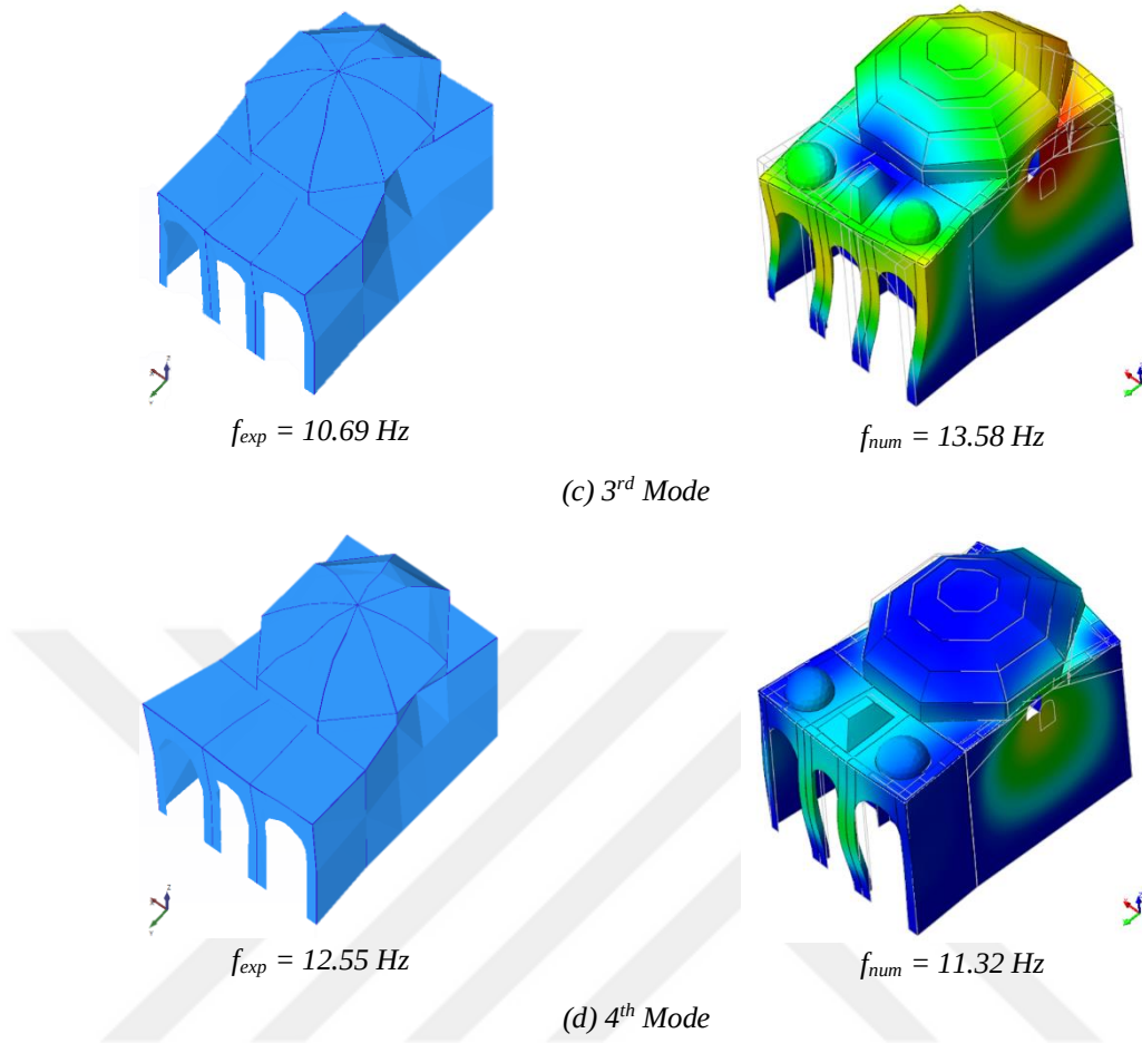
Figure 4.7. (continued) Experimental and calibrated numerical modes of vibrations
