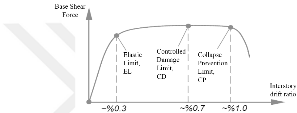
Figure 6.7. Pushover curve, inter-story drift ratio limits suggested by the Turkish guideline for historical structures (TYDRYK, 2017)
