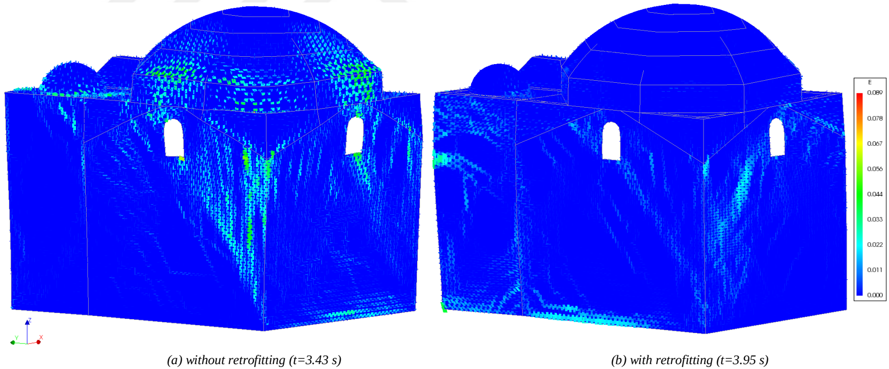
Figure A2. 2. Principal tensile strains of the South-West façade, deformed shape scale factor:5, the Erzincan Earthquake
