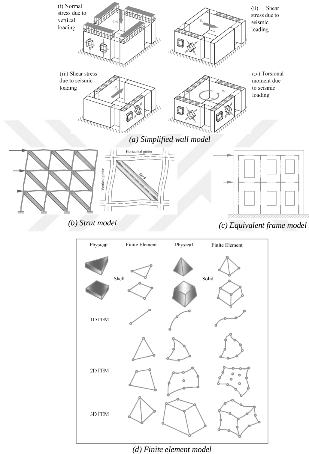
Figure 3.1. Modeling techniques defined in (TYDRYK, 2017)
