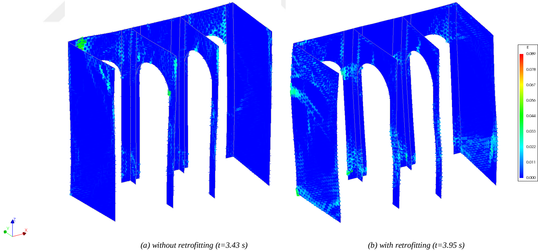
Figure A2. 6. Principal tensile strains of portico, deformed shape scale factor:5, the Erzincan Earthquake
