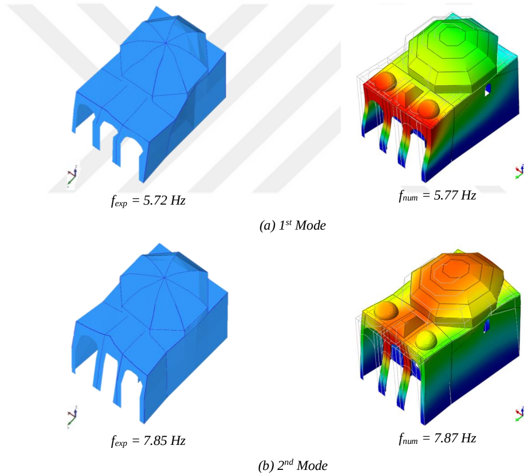
Figure 4.7. Experimental and calibrated numerical modes of vibrations
