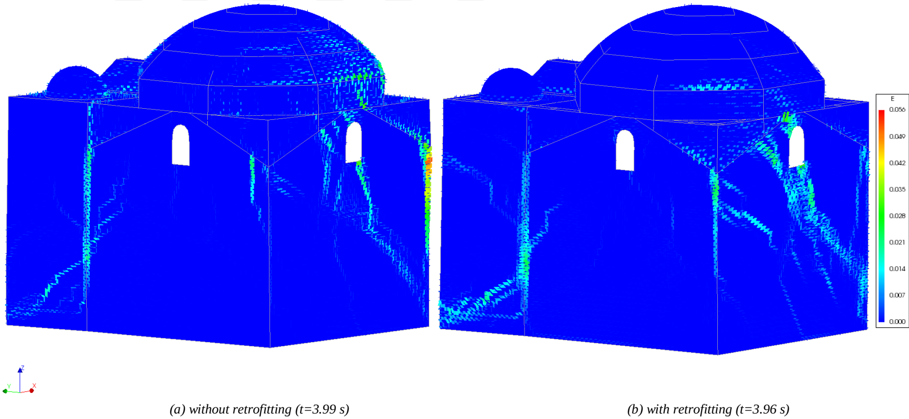
Figure A2. 12. Principal tensile strains of South-West façade, deformed shape scale factor:5, the Bingöl Earthquake
