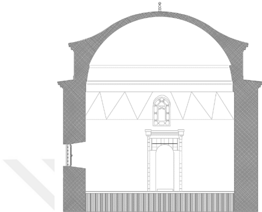
Figure A1. 5. Section A-A
