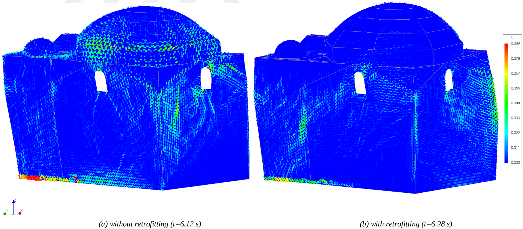
Figure A2. 7. Principal tensile strains of South-West façade, deformed shape scale factor:5, the Bolu Earthquake
