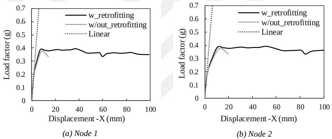
Figure 5.7. The pushover curves in the negative transversal direction
