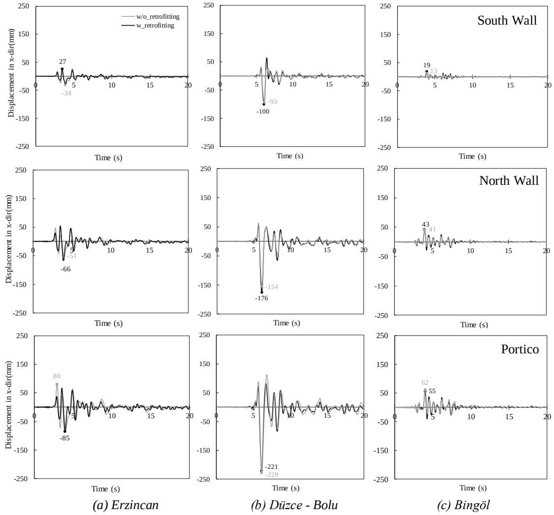
Figure 6.23. Change in response of control points on South Wall, North Wall and Portico due to retrofitting in terms of in-plane displacement
