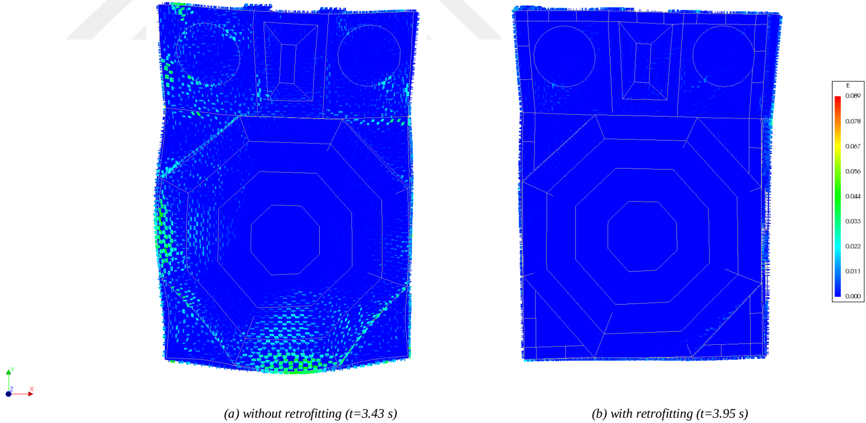
Figure A2. 5. Principal tensile strains of dome, deformed shape scale factor:5, the Erzincan Earthquake
