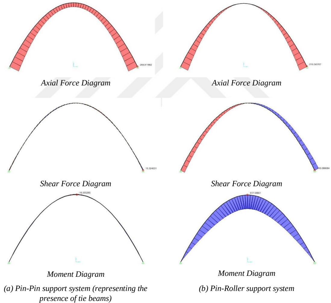
Figure 2.7. Arch response on the different arch systems
