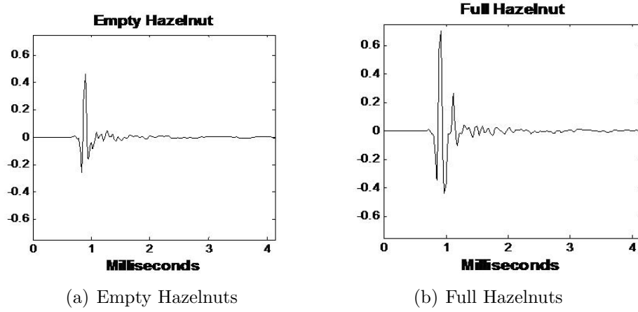
Figure 5.1: Typical impact sound signals from an empty hazelnut and a full hazelnut. The extremum of a full hazelnut is usually higher than an empty hazelnut.
