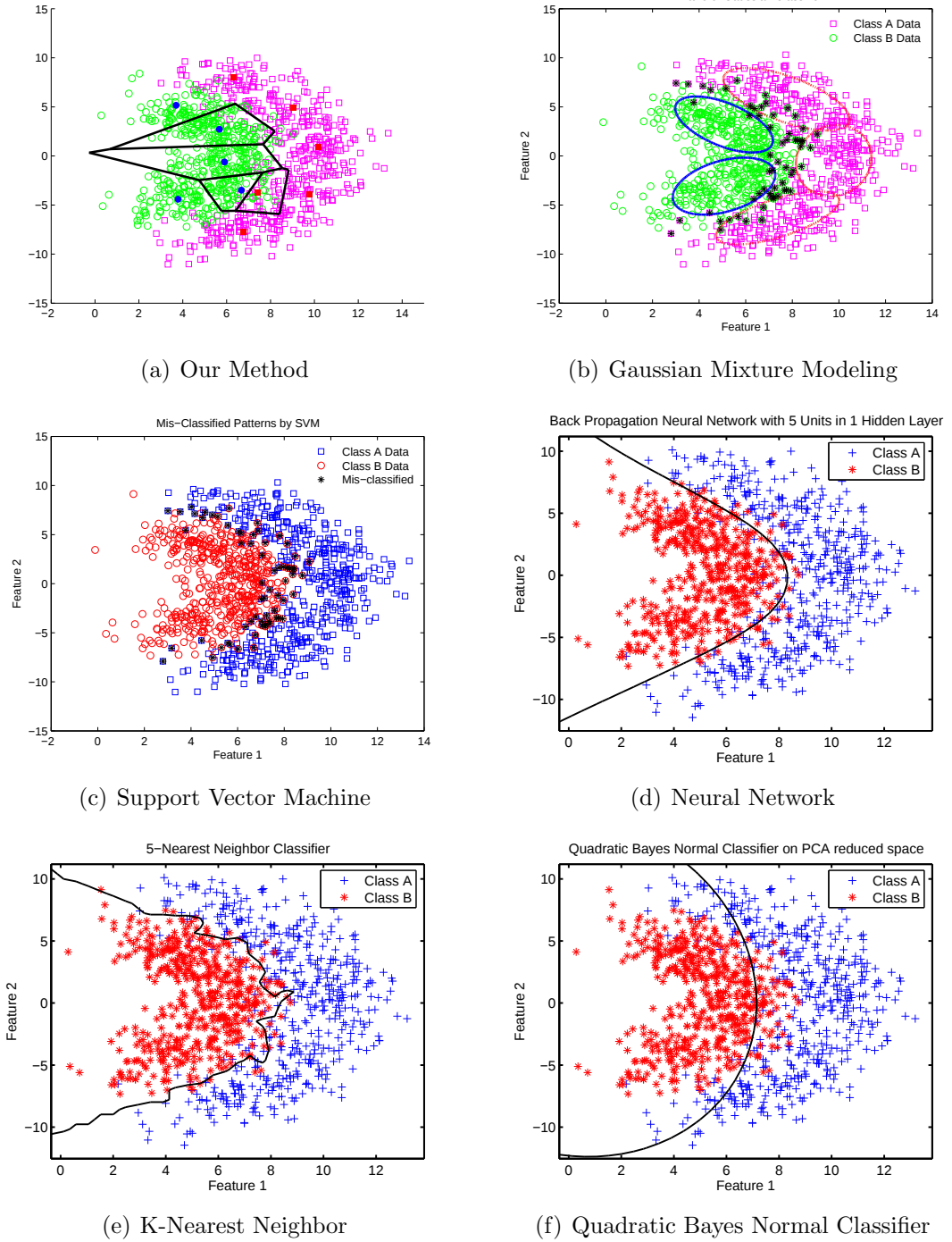
Figure 2.6: Performance comparison of our modified k -means algorithm with some state-of-the-art classifiers on Lithuanian dataset with 2 classes: (a) Our method ( k = 10 , T_1 = 0.5 , T_2 = 20 ), (b) Gaussian Mixture Models using arbitrary covariance matrices, (c) SVM using radial basis function, (d) Back-propagation Neural Network with 5 units using 1 hidden layer, (e) K-Nearest Neighbors ( k = 5 ), and (f) Quadratic Bayes Normal Classifier on PCA reduced space.
