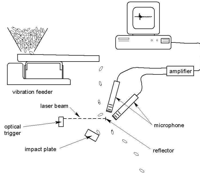
Figure 1.2: Schematic of experimental apparatus for collecting acoustic emissions from hazelnuts
