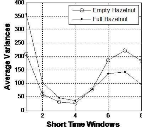
Figure 5.2: Average variances from short time windows of time domain signals
