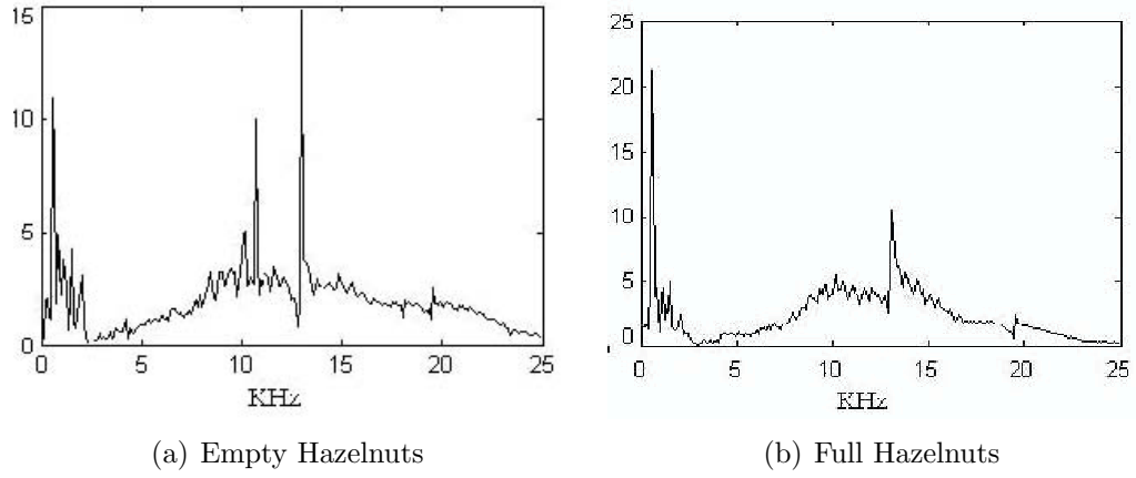
Figure 5.3: Example frequency spectra magnitudes for empty and full hazelnuts
