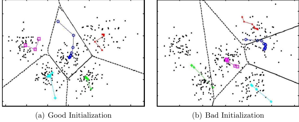
Figure 2.1: Effect of initial point selection on the performance of k -means algorithm. Here the same dataset is partitioned into five clusters; (a) yields the desired clustering while (b) gets trapped in a local minimum.
