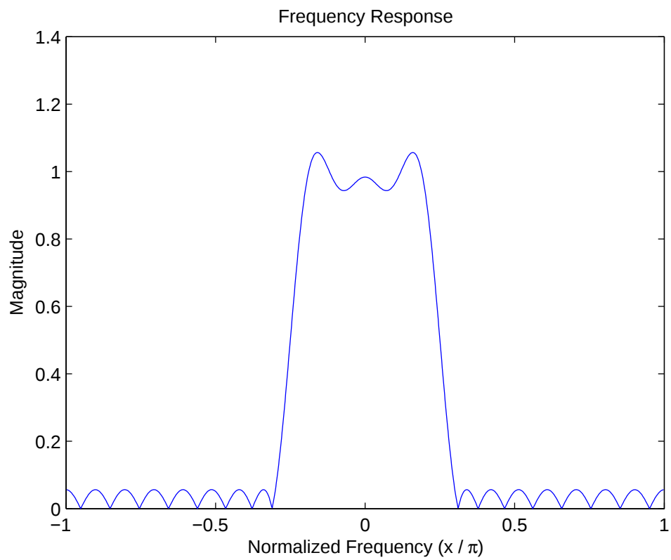
Figure 4.2: Frequency response of the low-pass filter used in pre-processing
