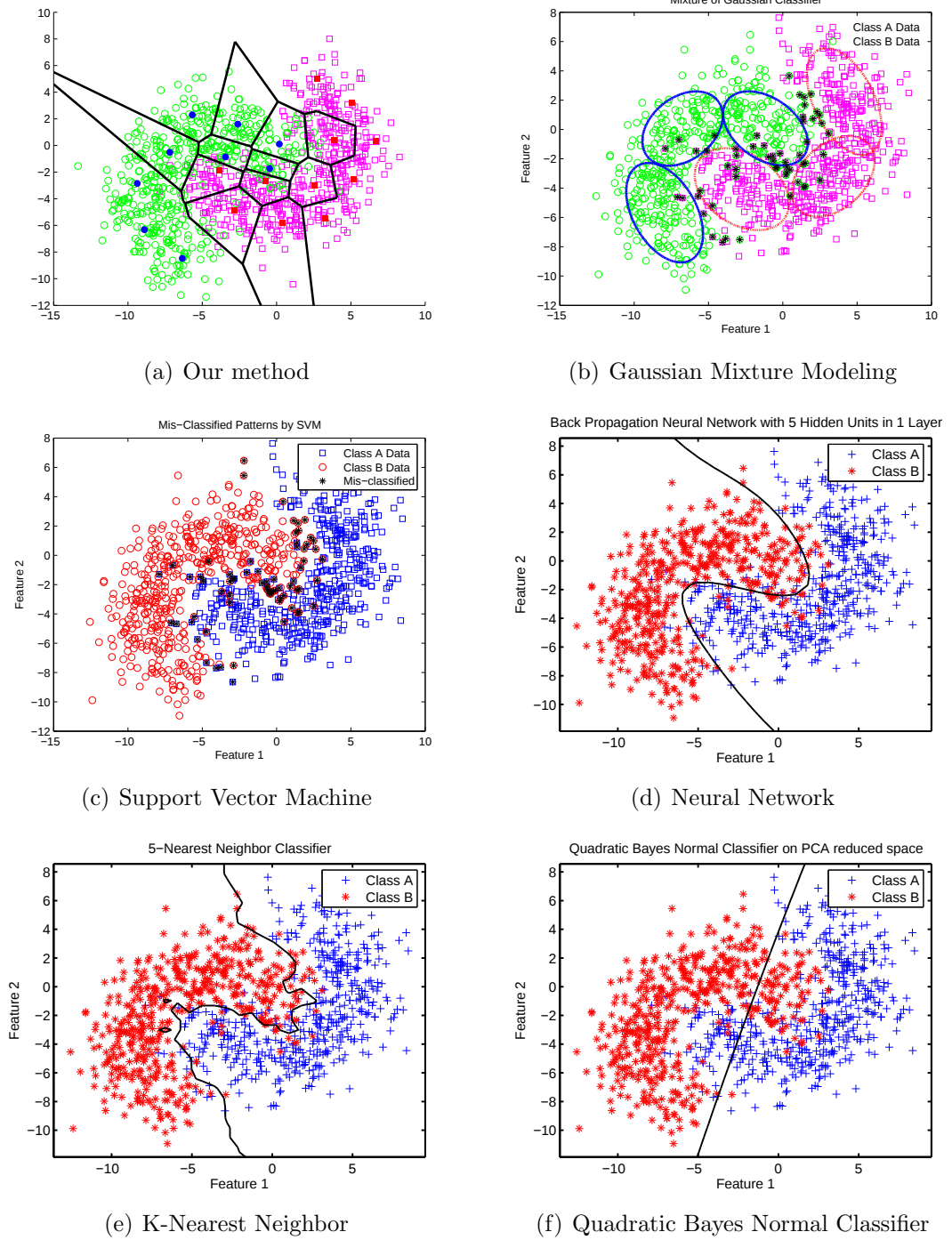
Figure 2.8: Performance comparison of our modified k -means algorithm with some state-of-the-art classifiers on banana-shaped dataset with 2 classes ( randomnessfactor = 1.5 ): (a) Our method with minimum distance based brute forcing ( k = 20 , T_1 = 0.8 , T_2 = 30 ), (b) Gaussian Mixture Models using arbitrary covariance matrices, (c) SVM using radial basis function, (d) Back-propagation Neural Network with 5 units using 1 hidden layer, (e) K-Nearest Neighbors ( k = 5 ), and (f) Quadratic Bayes Normal Classifier on PCA reduced space.
