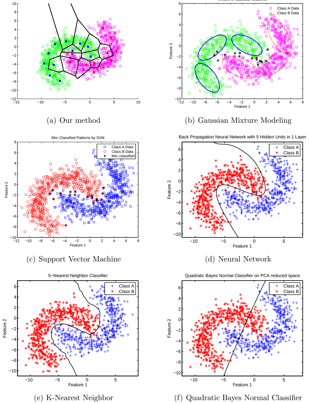
Figure 2.7: Performance comparison of our modified k -means algorithm with some state-of-the-art classifiers on banana-shaped dataset with 2 classes ( randomnessfactor = 1 ): (a) Our method with minimum distance based brute forcing ( k = 25 , T_1 = 0.6 , T_2 = 30 ), (b) Gaussian Mixture Models using arbitrary covariance matrices, (c) SVM using radial basis function, (d) Back-propagation Neural Network with 5 units using 1 hidden layer, (e) K-Nearest Neighbors ( k = 5 ), and (f) Quadratic Bayes Normal Classifier on PCA reduced space.
