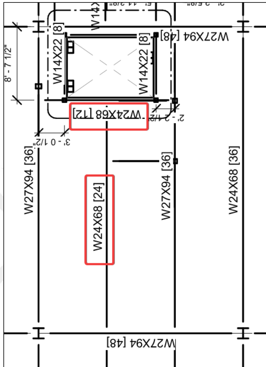
Figure 5.16 Framing Configuration in 95% Design Drawings
