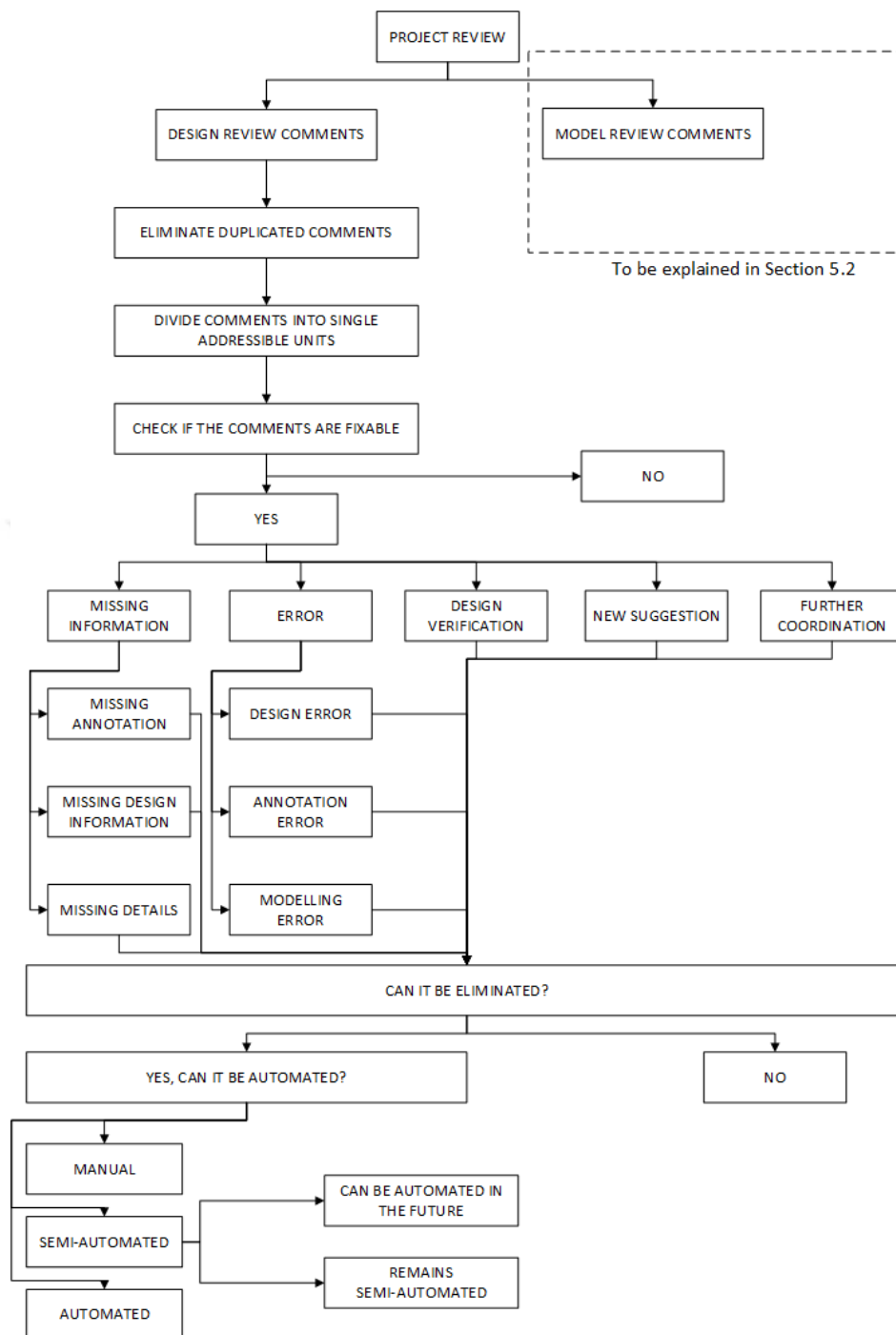
Figure 5.1 Design Review Comment Classification Process
