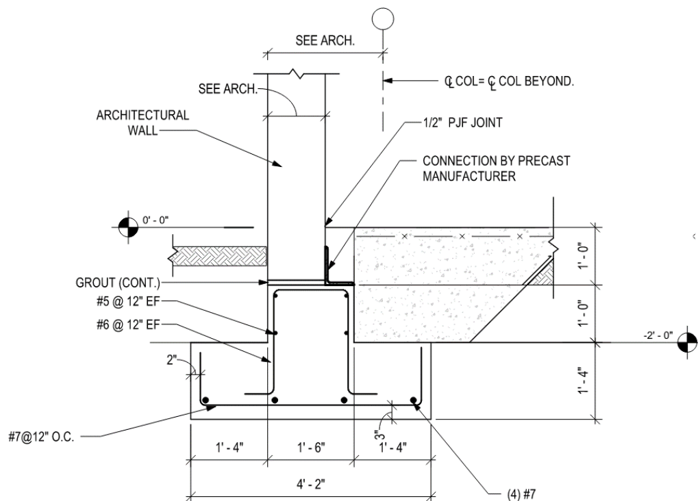
Figure 5.9 Precast Wall Support Detail – 65% Design Drawings
