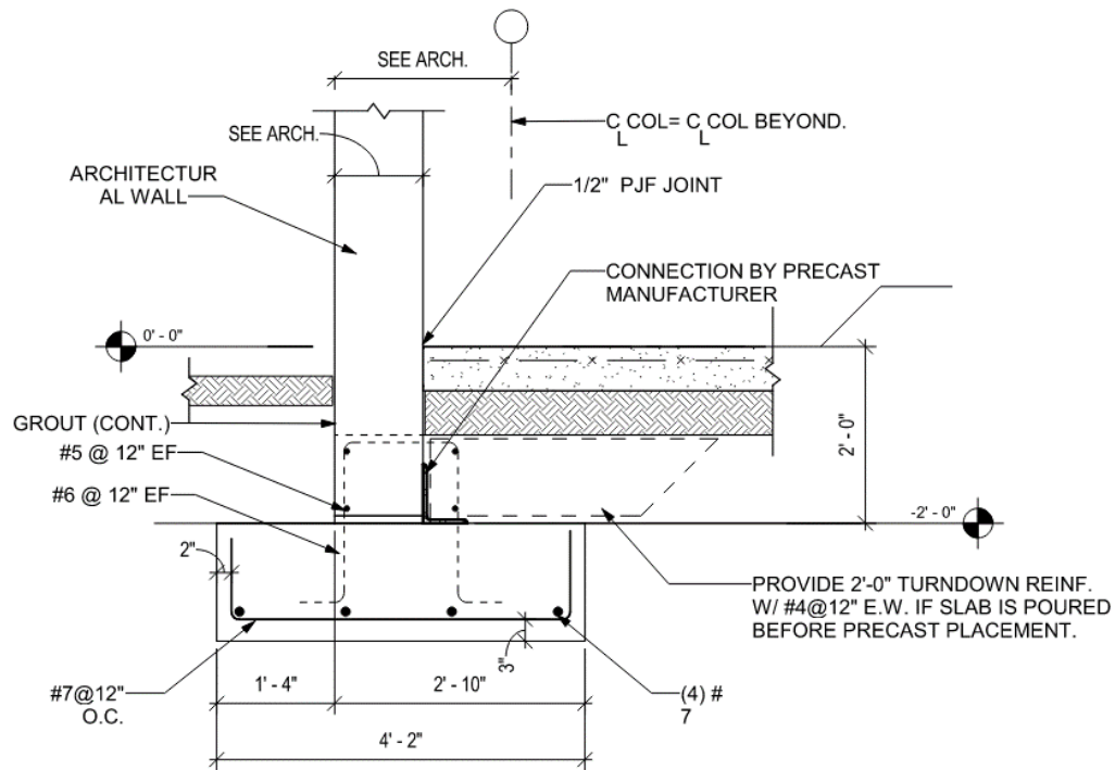
Figure 5.10 Precast Wall Support Detail – 95% Design Drawings
