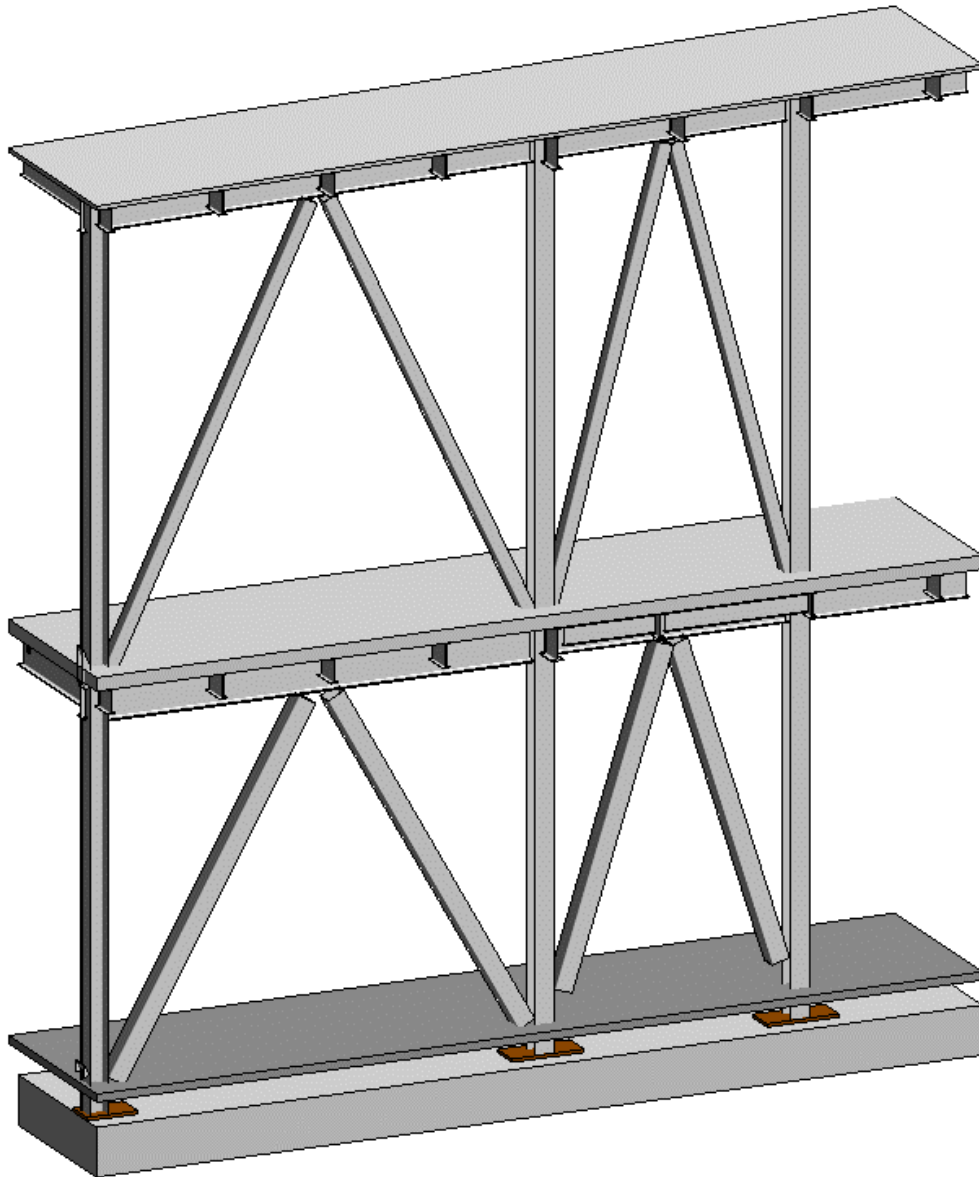
Figure 5.12 Isometric View of Brace Line
