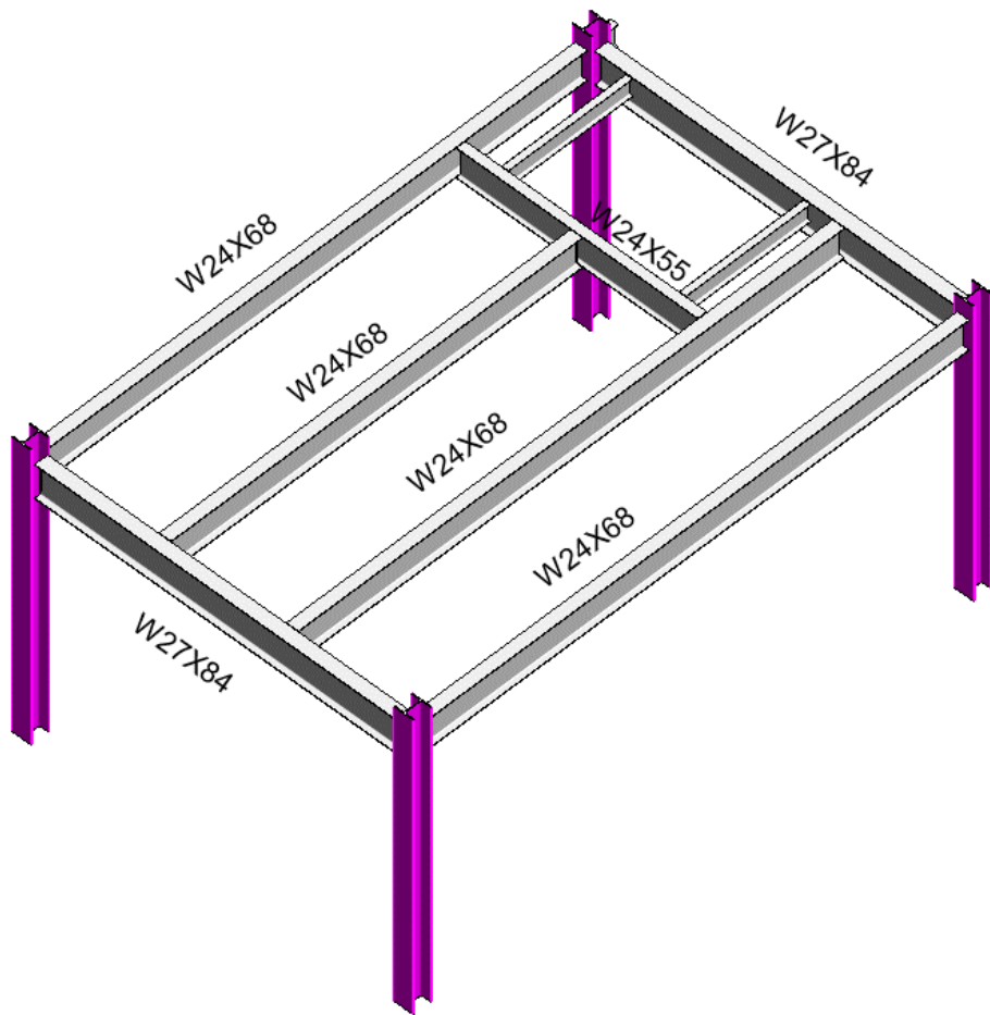
Figure 5.15 Framing Configuration Isometric View – 65% Design Drawings
