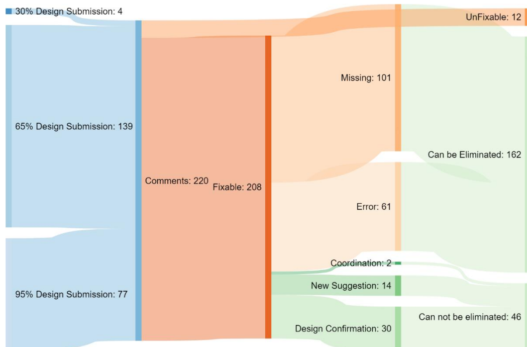
Figure 5.4 Comment Distribution
