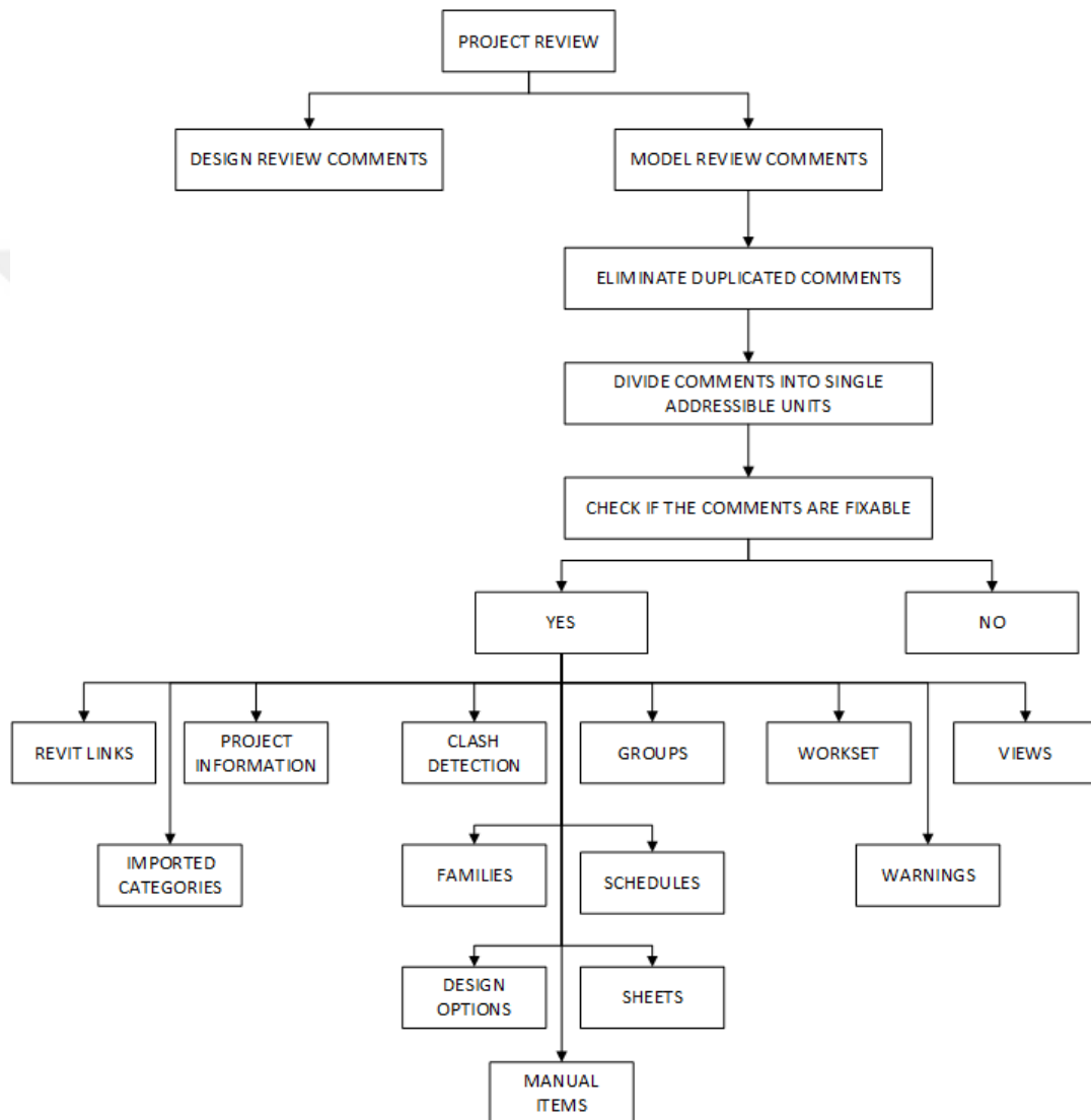
Figure 5.2 Model Review Comment Classification Procedure
