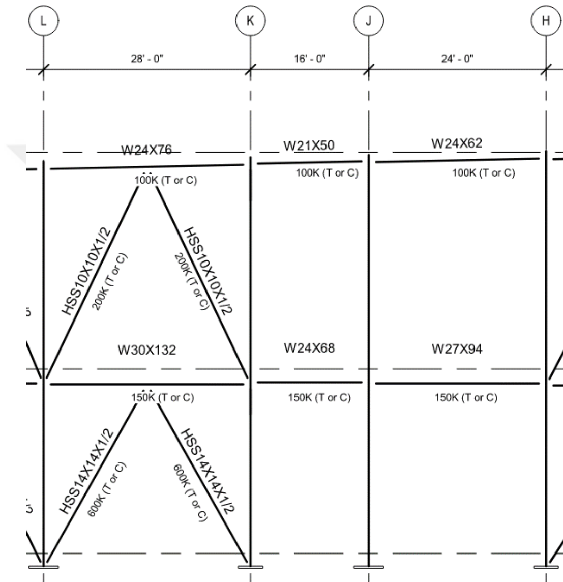
Figure 5.13 Brace Effectiveness Check – 95% Design Drawings
