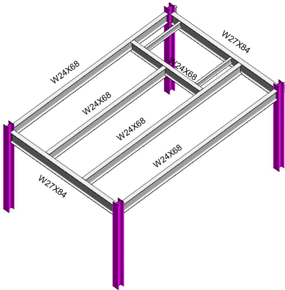
Figure 5.17 Framing Configuration Isometric View – 95% Design Drawings
