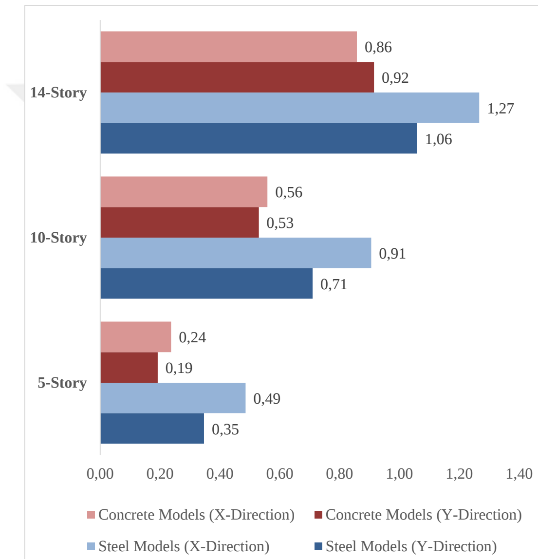
Figure 4.4. Fundamental Periods in Both Principle Directions
