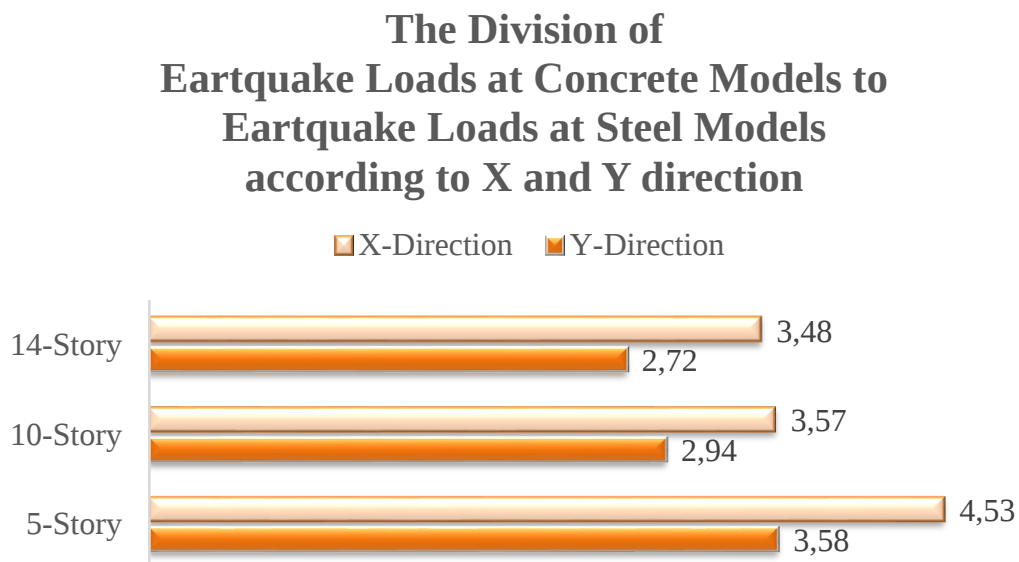
Figure 4.8. Earthquake Loads Ratio between Reinforced Concrete and Steel Models
