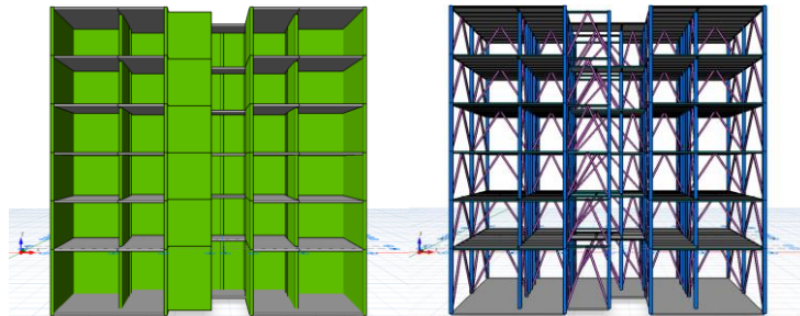
Figure 4.1. 5-Story Reinforced Concrete Model (left) and 5-Story Steel Model (right)
