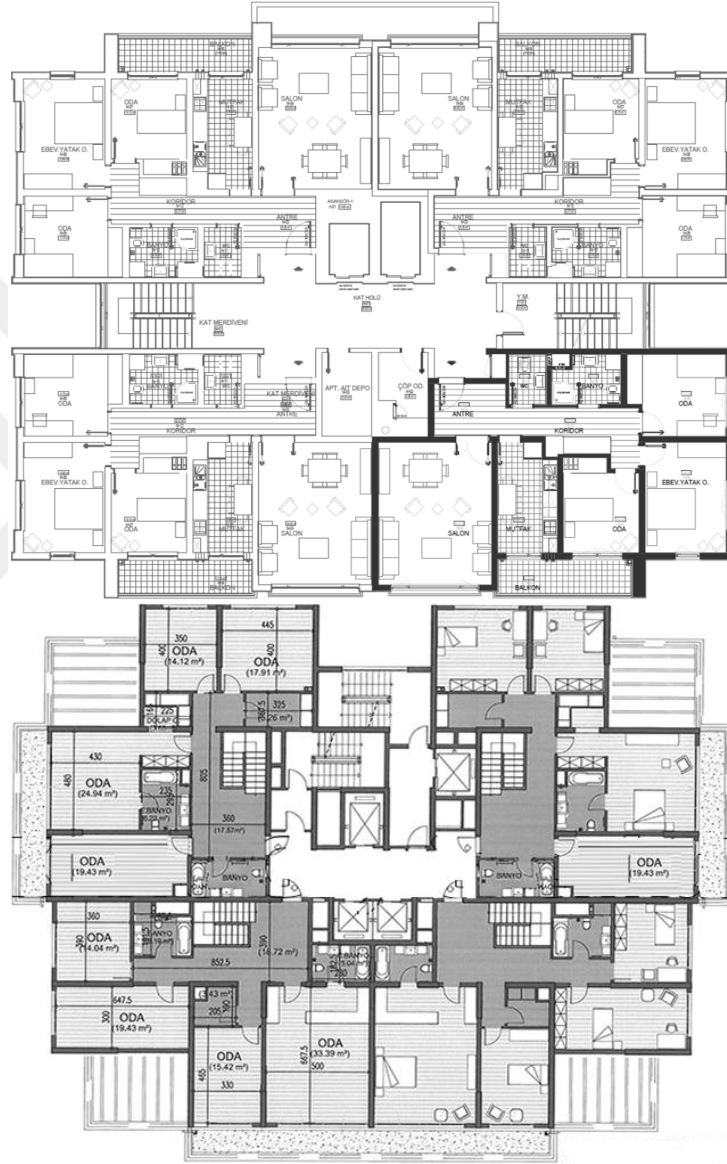
Figure 2.23. F4 Scheme with 6-7-8 floors (above) and 25 floors (below)
