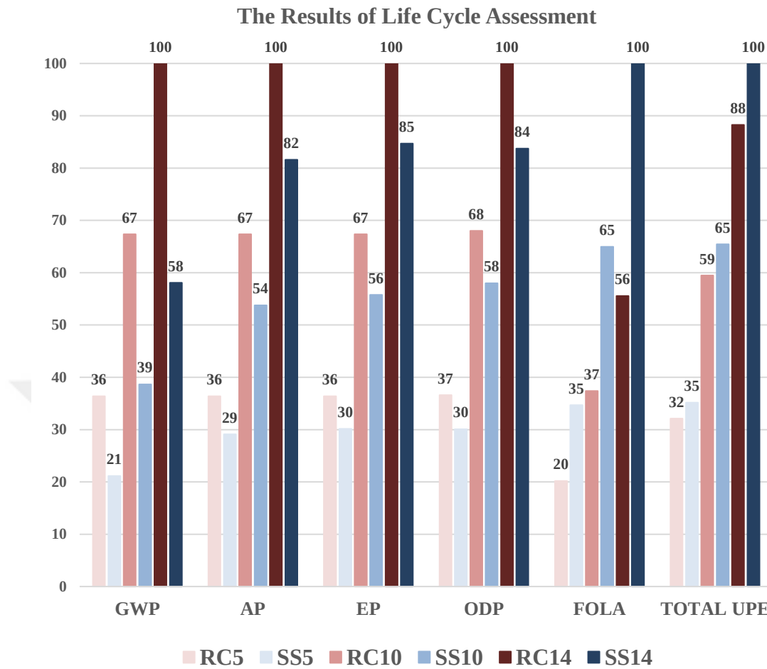
Figure 4.15. The Results of Life Cycle Assessment for All Impact Categories
