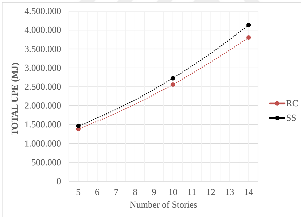
Figure 4.14. The Results of Total Use of Primary Energy
