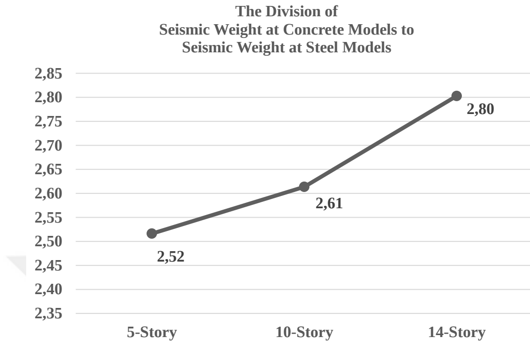
Figure 4.6. The Floor Weight Ratio between Reinforced Concrete and Steel Models
