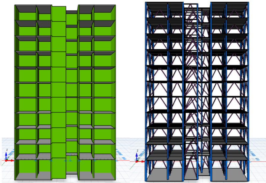
Figure 4.2. 10-Story Reinforced Concrete Model (left) and 10-Story Steel Model (right)
