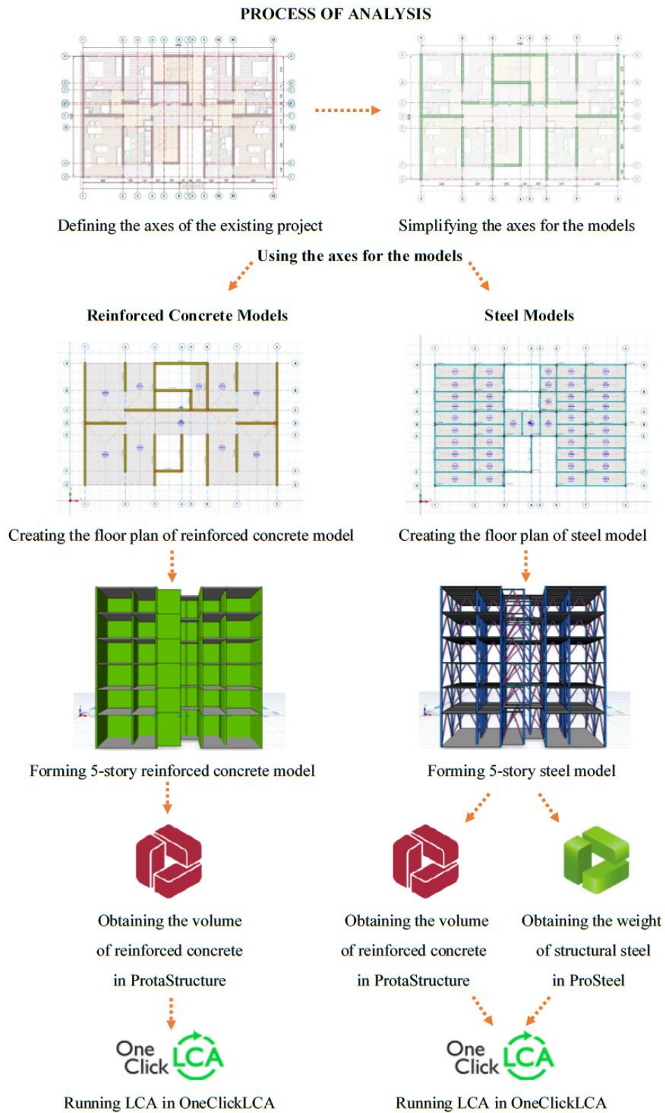
Figure 3.30. The Process of Analysis
