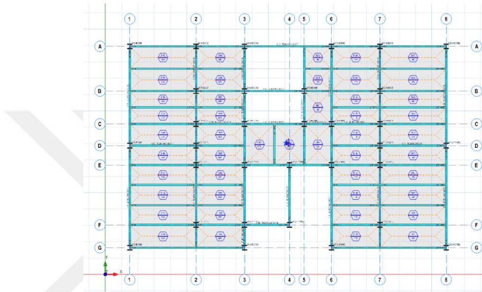
Figure 3.12. Floor Plan of SS10 Model in ProtaStructure
