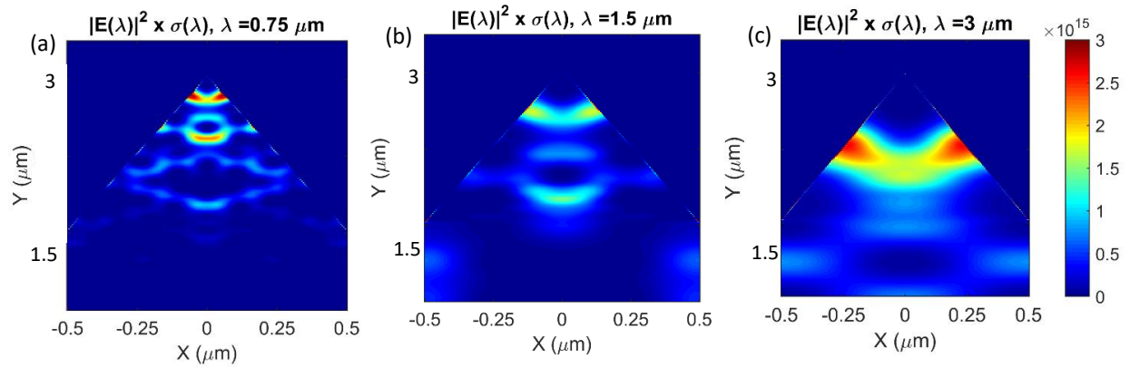
Fig. 4.11. a-b-c) |E(\lambda)|^2 \times \sigma(\lambda) at wavelengths of 0.75, 1.5 and 3 \mu\text{m} for the triangle dimensions of p = 1 \mu\text{m} , h = 3 \mu\text{m} and carrier concentration of 10^{14} \text{ cm}^{-3} .
