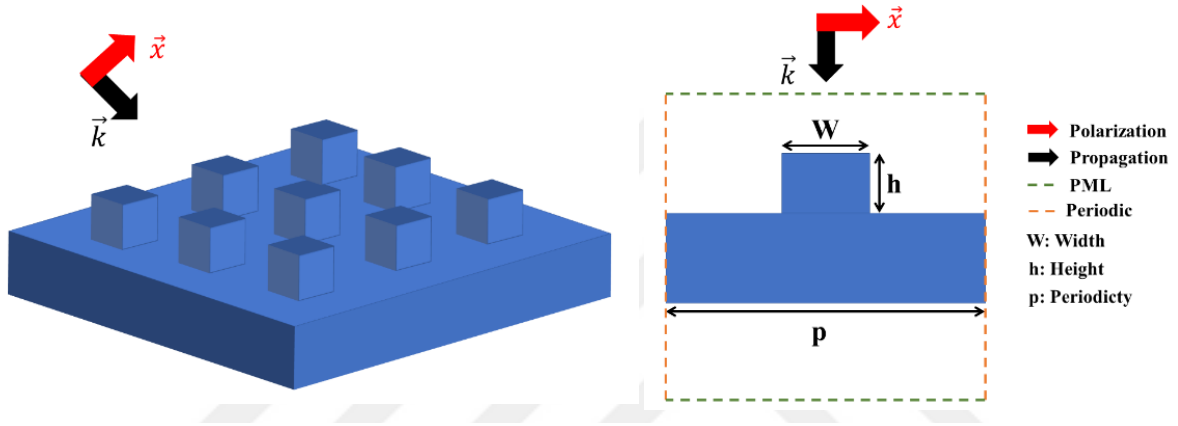
Fig. 5.1. a) 3D visualization of rectangular gratings. b) 2D scheme of geometrical dimensions and simulation physics.
