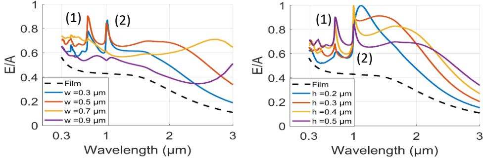
Fig. 5.4. a) \varepsilon(\lambda)/\alpha(\lambda) intensities for h=0.5 \mu\text{m} and p=1 \mu\text{m} and varying widths. b) \varepsilon(\lambda)/\alpha(\lambda) intensities for w=0.5 \mu\text{m} and p=1 \mu\text{m} .
