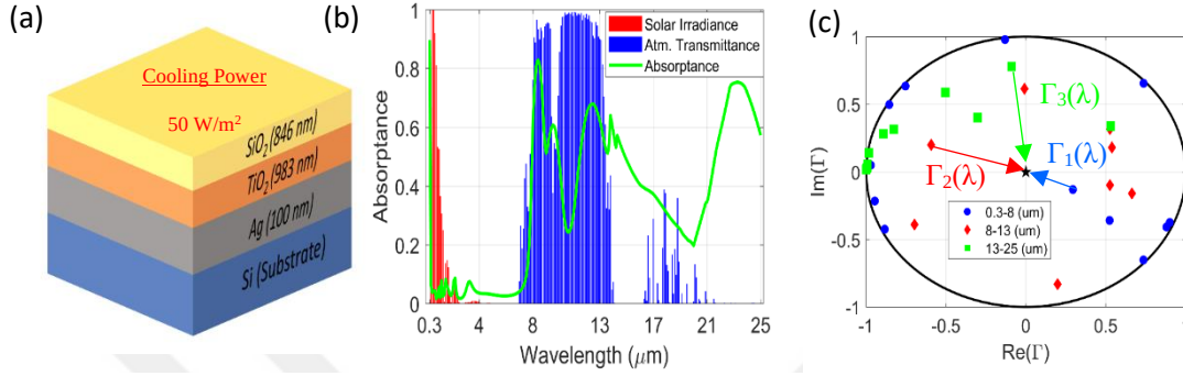
Fig. 2.5. a) Structure with 3 layers designed by the impedance formulation which has cooling power of 50 \text{ W/m}^2 at 300 \text{ K} . b) Spectral absorptance of the structure depicted in (a) at perpendicular angle of incidence, plotted with solar irradiance in 0.3 - 4 \mu\text{m} and atmospheric transmittance in 8 - 25 \mu\text{m} spectrum interval. c) Spectral distribution of reflectance coefficients of the structure depicted in (a).
