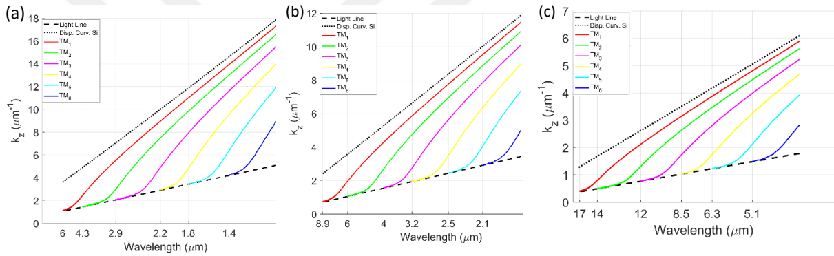
Fig. 4.16. a-b-c) Dispersion diagrams for d=0.7, 1 and 2\text{ }\mu\text{m} and supported \text{TM} modes with cut-off wavelengths labeled.
