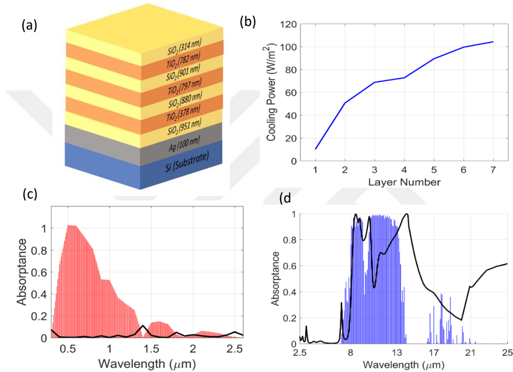
Fig. 2.7. a) Final structure with 7 layers. b) Cooling power at 300 K and T_{\text{Amb}} = 297 \text{ K} . c) Absorptance of the structure depicted in (a) in spectrum interval 0.3\text{--}2.5 \text{ }\mu\text{m} plotted on solar irradiance in this interval at perpendicular angle of incidence. d) Absorptance of the structure depicted in (a) in spectrum interval 2.5\text{--}25 \text{ }\mu\text{m} at perpendicular angle of incidence, plotted on atmospheric transmittance in this interval.
