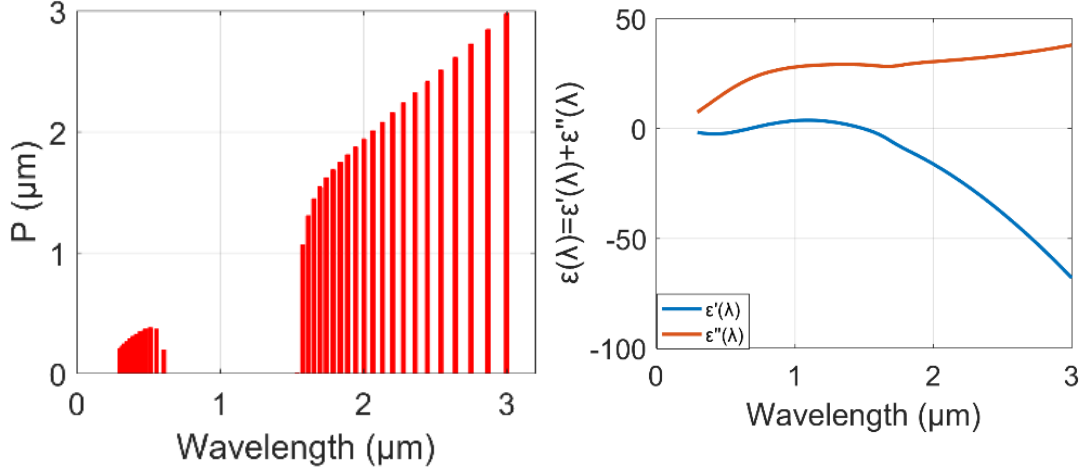
Figure 5.6. a) Required periodicities for allowed plasmonic modes. b) Permittivity of \text{ZrB}_2 retrieved from [179].
