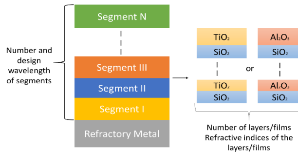
Fig. 3.6. Schematic for the proposed structures which are composed of several periodic high-low index segments. Possible design parameters that influence the performance of the structure, number of segments, central wavelength of the segments, number of layers in the segments and materials, are also demonstrated.
