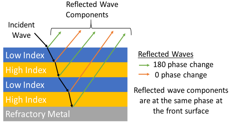
Fig. 3.3. Schematic of the high-low index periodic structures on which reflected wave components that either experiences 180^\circ (green) or 0^\circ (orange) phase change are visualized.
