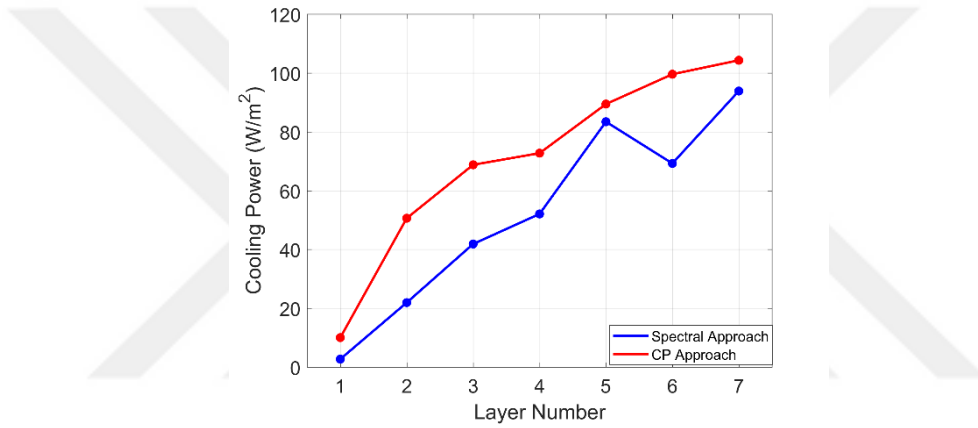
Fig. 2.9. Cooling power comparison of the structures designed by spectral and cooling power approach with layer numbers of 1 to 7.
