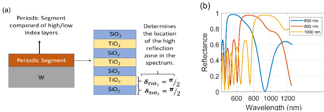
Fig. 3.4. a) A schematic representation for the simulated structure in which periodic high-low index layers are coated on tungsten on top of W. Coating materials are selected as \text{TiO}_2 as high index and \text{SiO}_2 as low index. Optical thicknesses of the layers are set to \pi/2 and central wavelengths are selected as 600, 800 and 1000 nm. b) Reflectance of the structure for which scheme is given in Fig. 3.4(a) at the specified central wavelengths. High reflectance zones are achieved around wavelengths which are slightly shifted from central wavelengths due to interference with W at the bottom.
