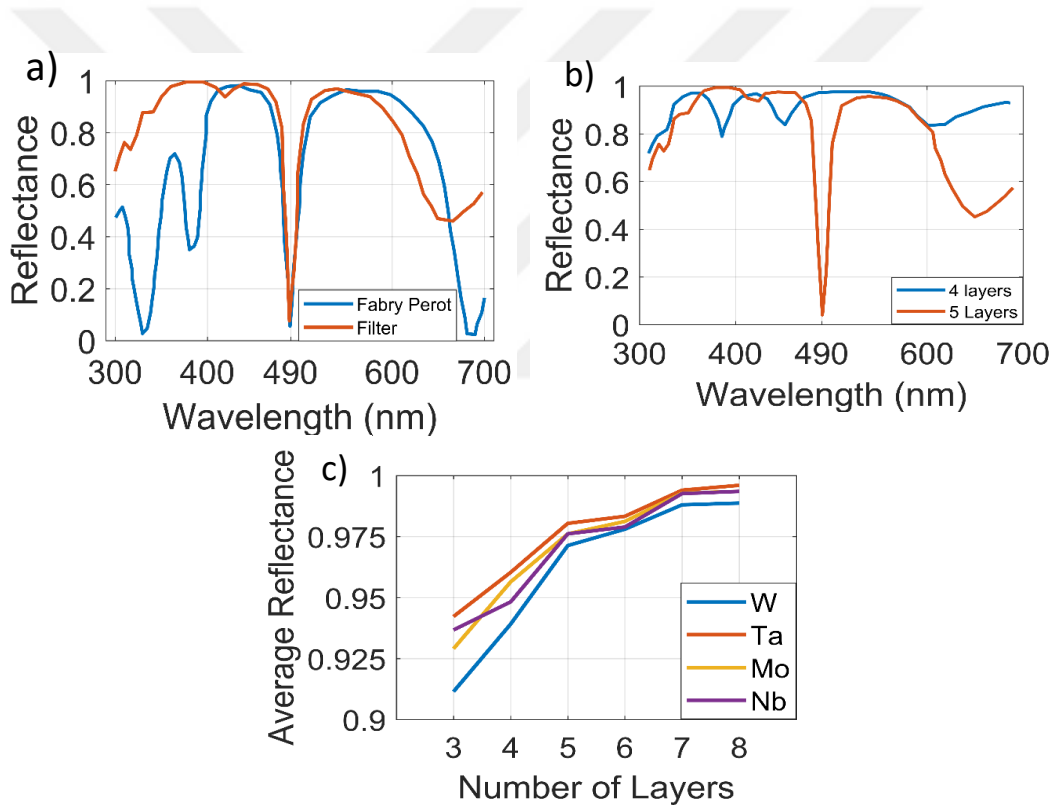
Fig. 3.9. a) Spectral reflectance of Fabry Perot filter designed at 490 nm and optical filter composed of two periodic segments with central wavelengths of 400 and 600 nm wavelengths on top of 500 nm thick tungsten. Similar spectral reflectance behaviors are observed. b) Spectral reflectances of the filters with periodic segments designed at 400 and 600 nm wavelengths on top of 500 nm thick tungsten. When layer number in the segments are 5, optical thicknesses of \text{TiO}_2 layers add up to \pi and form a half wavelength thick medium, whereas when number of layers are 4 half wavelength thick medium is not formed. c) Average reflectance of the filters for which average reflectances are reported in Fig. 7(d) when top layers of the segments are \text{TiO}_2 which creates approximate Fabry Perot effects due to \text{TiO}_2 - \text{TiO}_2 interfaces. When top layers are changed to \text{SiO}_2 increasing average reflectance with increasing number of layers shows that effect of reflectance dips in the presence of \text{SiO}_2 - \text{SiO}_2 interfaces on average reflectance are decreased.
