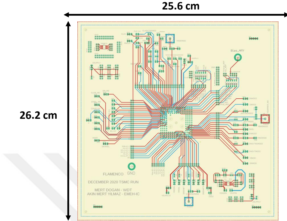
Figure 4.24. Non-Coherent WDT system circuit test PCB layout
