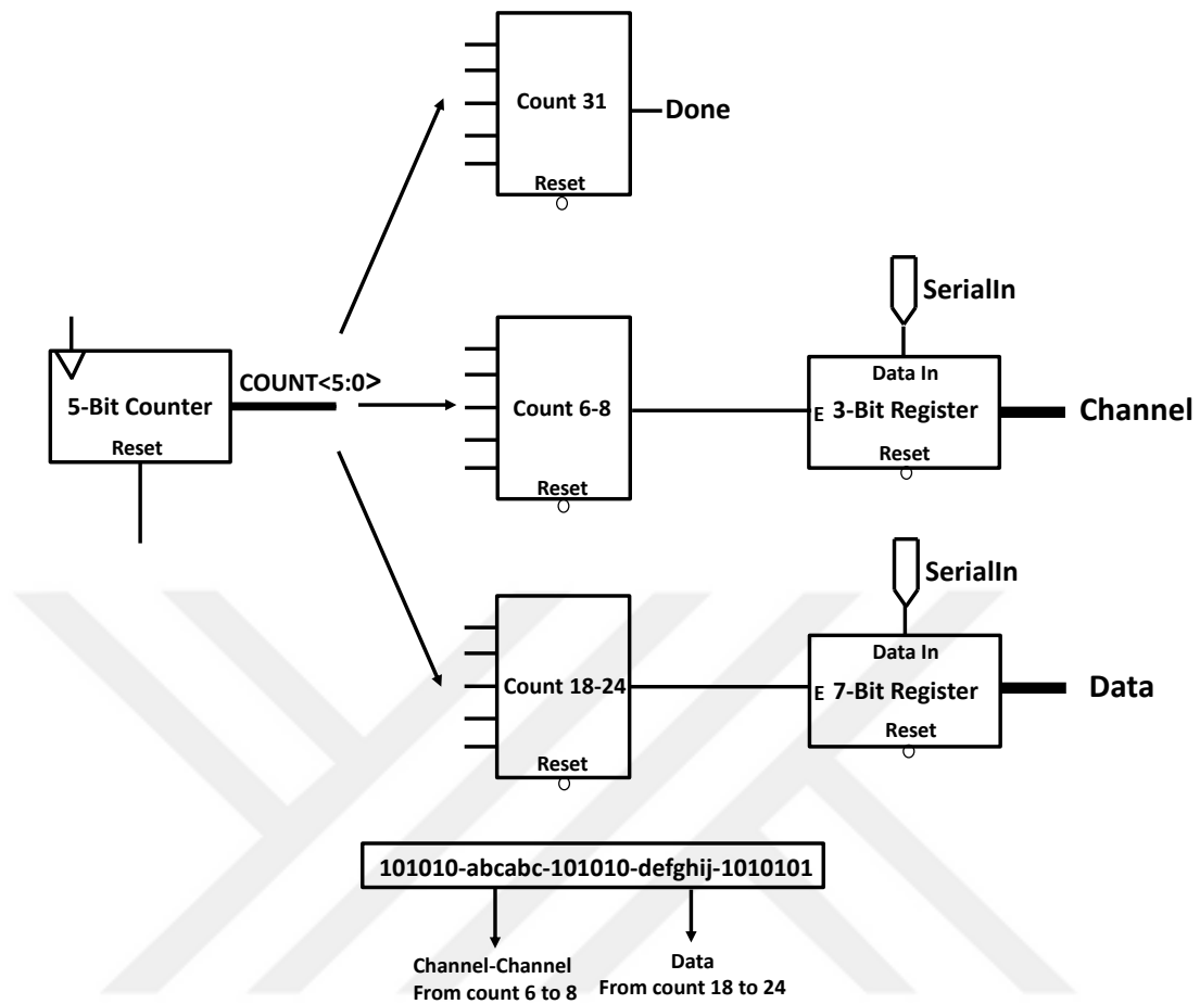
Figure 3.25. Recovered serial data input to parallel data extractor diagram
