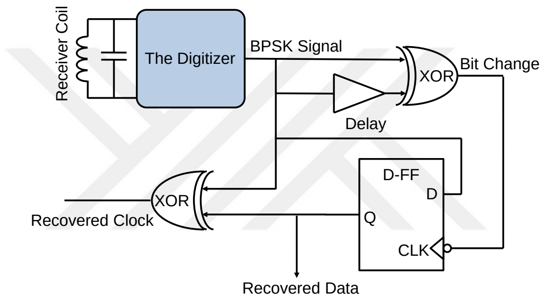
Figure 4.8. Fully digital non coherent demodulator v1
