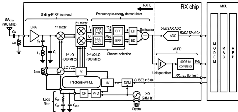
Figure 1.8. Block diagram of FSK receiver [40]
