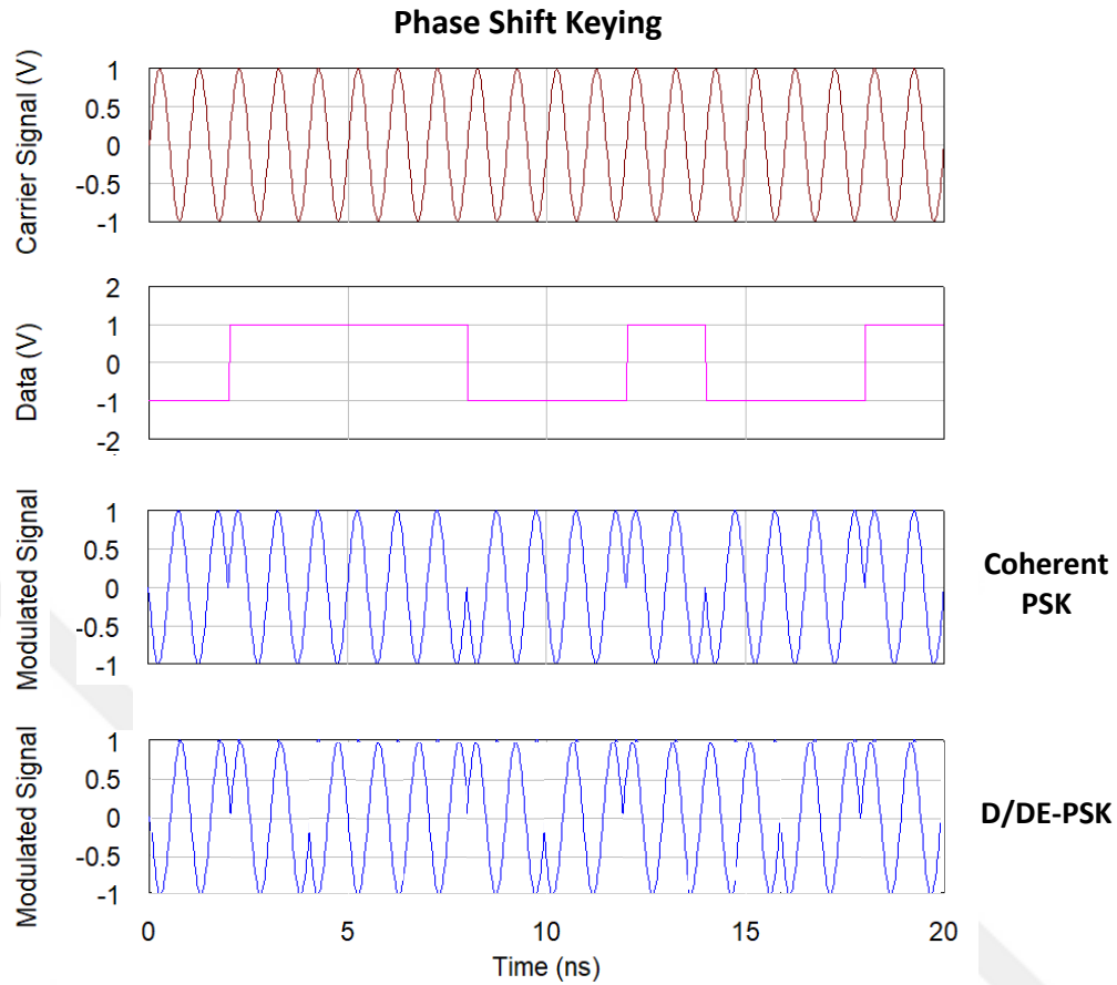
Figure 2.10. BPSK modulated signal waveforms with carrier and data inputs
