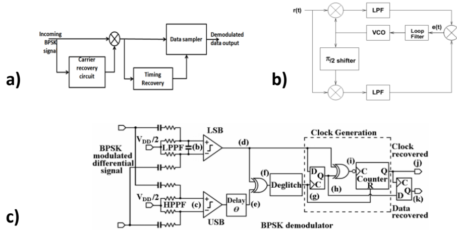
Figure 1.12. a) Coherent detection diagram of BPSK [44], b) Costas Loop [45], c) non-coherent detection overall diagram of BPSK [45]
