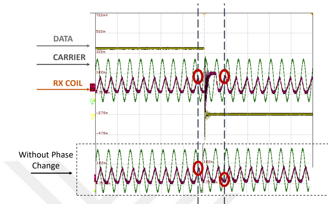
Figure 4.26. Symbol 1 to 0 transition modulated waveform received at the receiver coil with no modulation comparison
