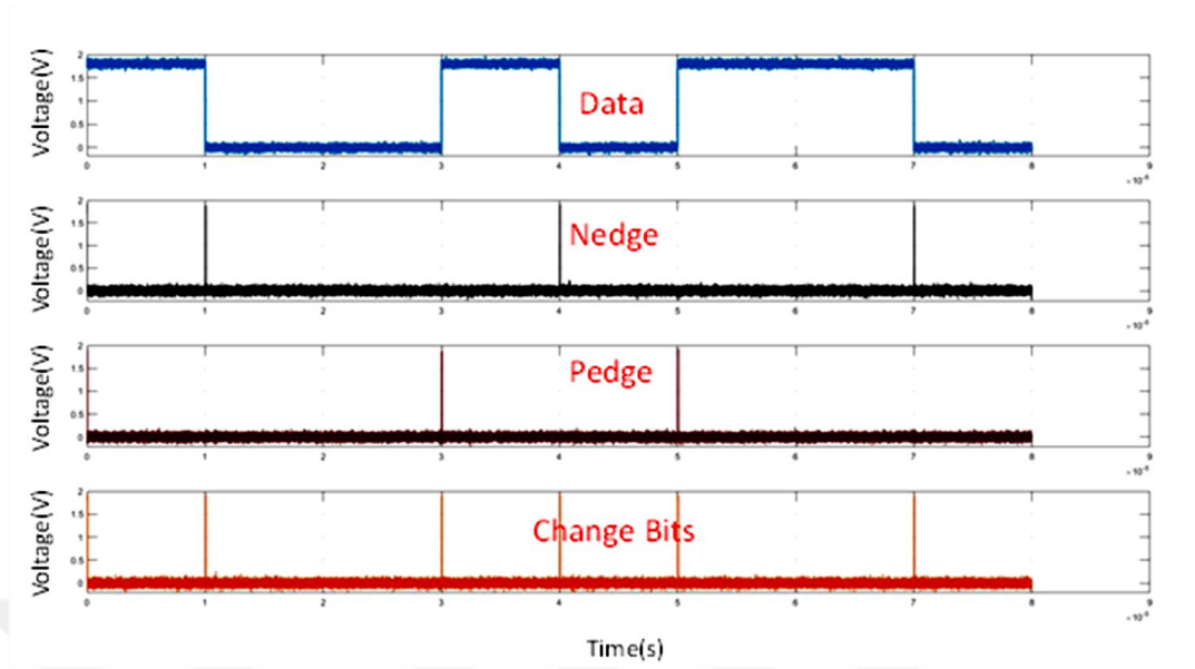
Figure 4.29. Control signals and recovered data waveform
