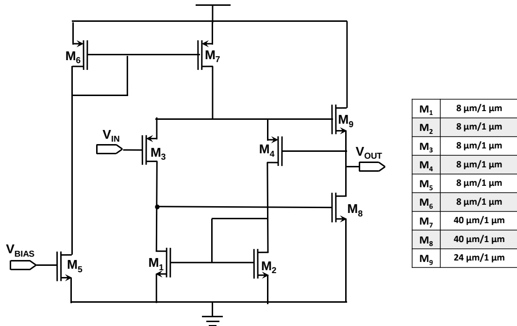
Figure 4.5. Voltage buffer schematics
