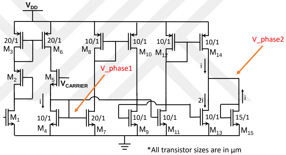
Figure 4.1. Inverse carrier generator block
