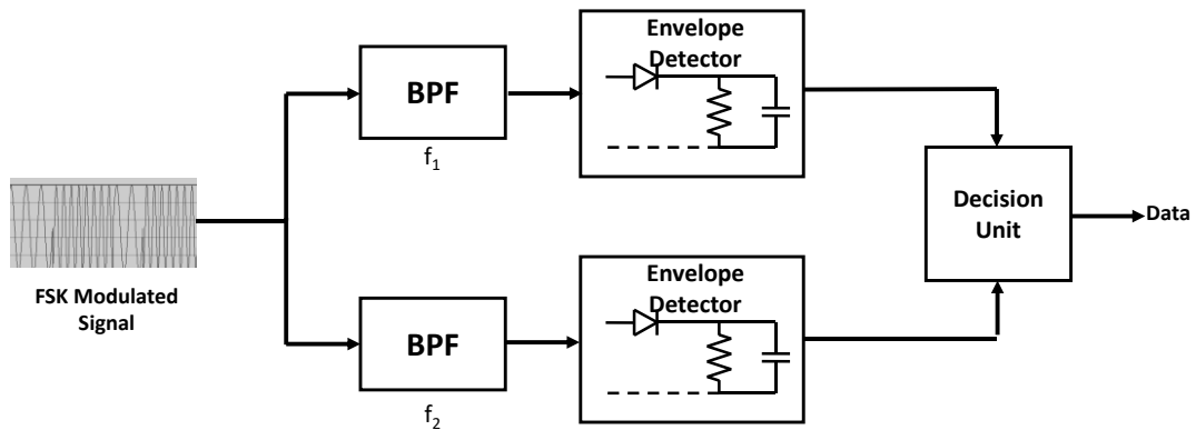
Figure 2.8. Non-coherent FSK demodulation diagram
