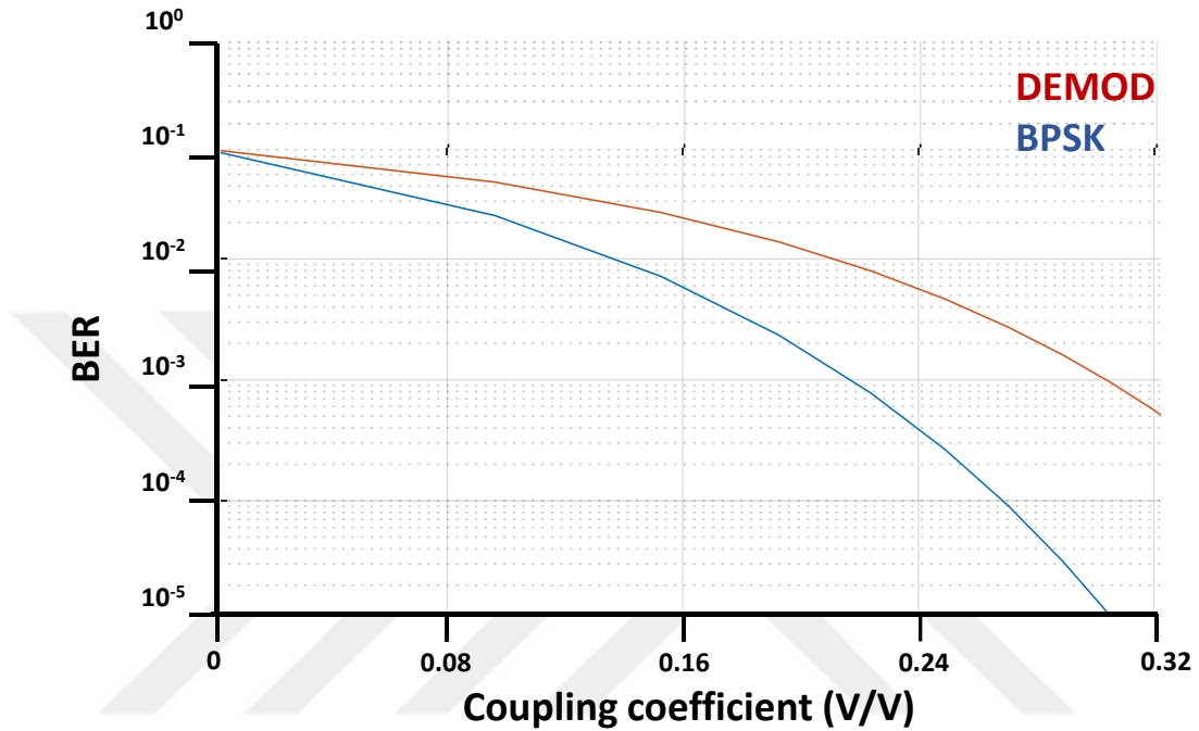
Figure 3.22. Demodulator and coherent BPSK BER vs coupling coefficients
