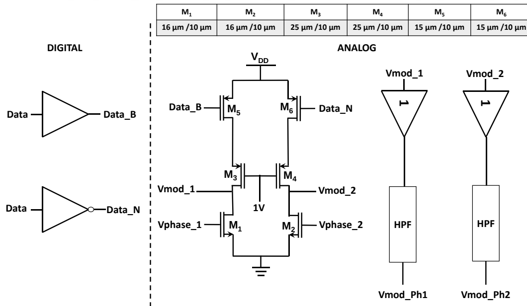
Figure 4.3. Phase modulator block diagram with amplifier circuit
