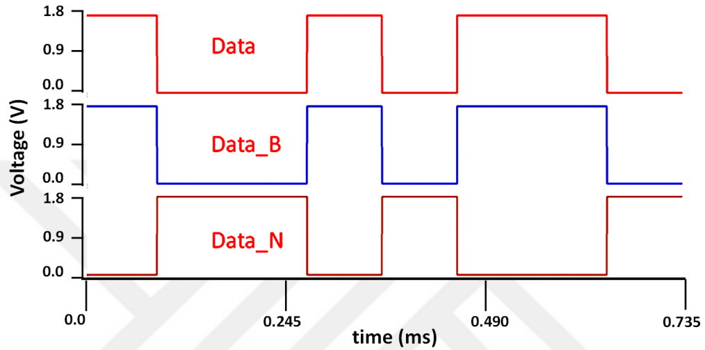
Figure 4.4. Data, buffered and inverted control voltage waveforms
