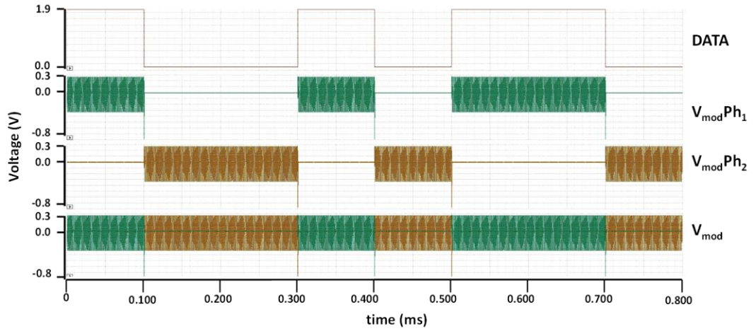
Figure 4.6. Demodulator output waveforms, separate phases, and overall modulated signal
