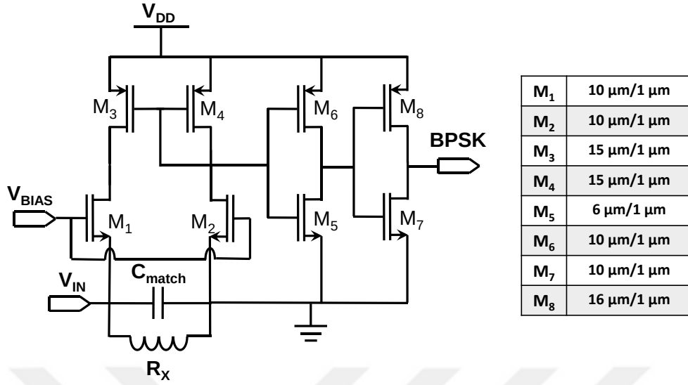
Figure 4.9. 1-Bit Digitizer Block
