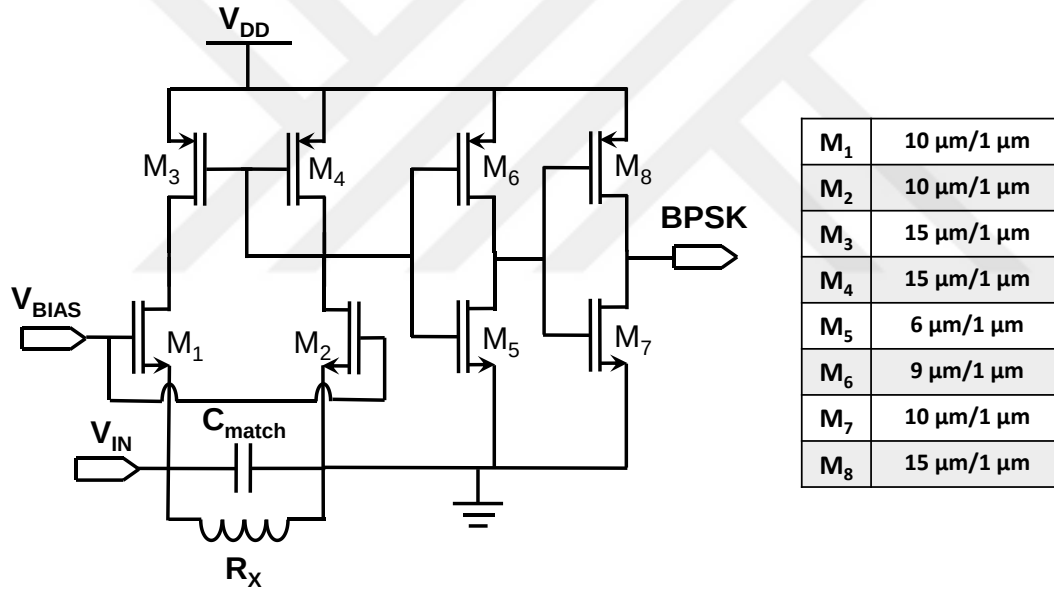
Figure 3.15. 1-Bit Digitizer with delay buffer
