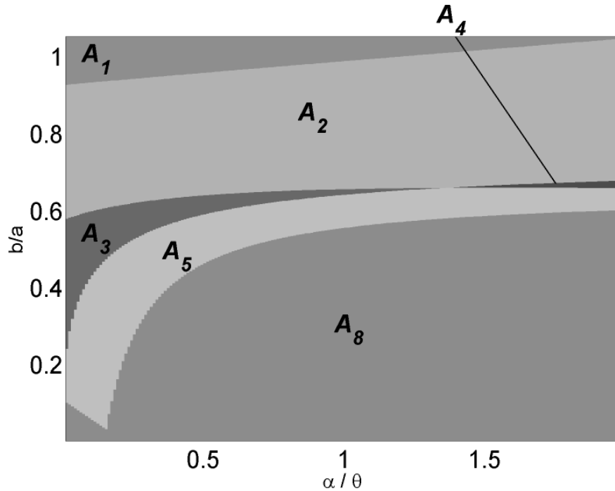
Figure 5.8: The Profit Change Regions when F = 250 (a = 100, \theta = 0.5, \text{ and } k = 0.1)
