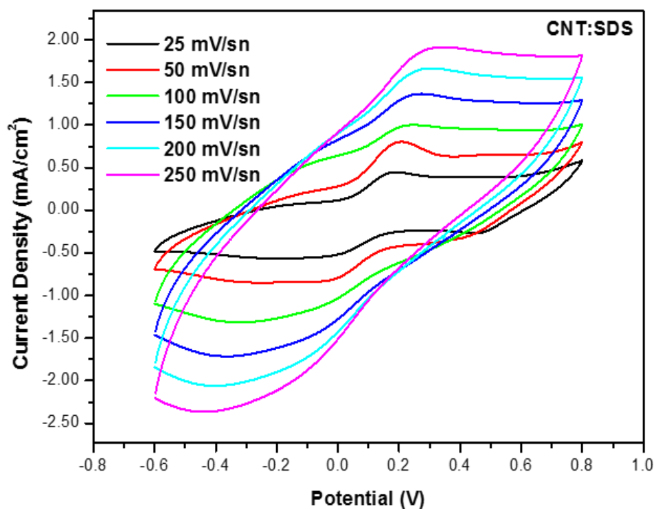
Figure 5.24 : CV curves of 5 mM \text{K}_3\text{Fe}(\text{CN})_6 and 0.1 M KCl solution for SWNT/SDS electrode
