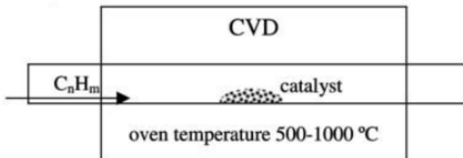
Figure 2.6: Schematic of CVD operated as floating catalyst or substrate catalyst.
