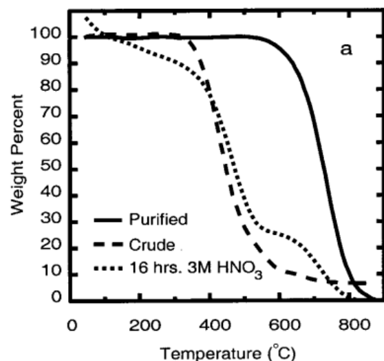
Figure 3.6: Thermogravimetric analysis
