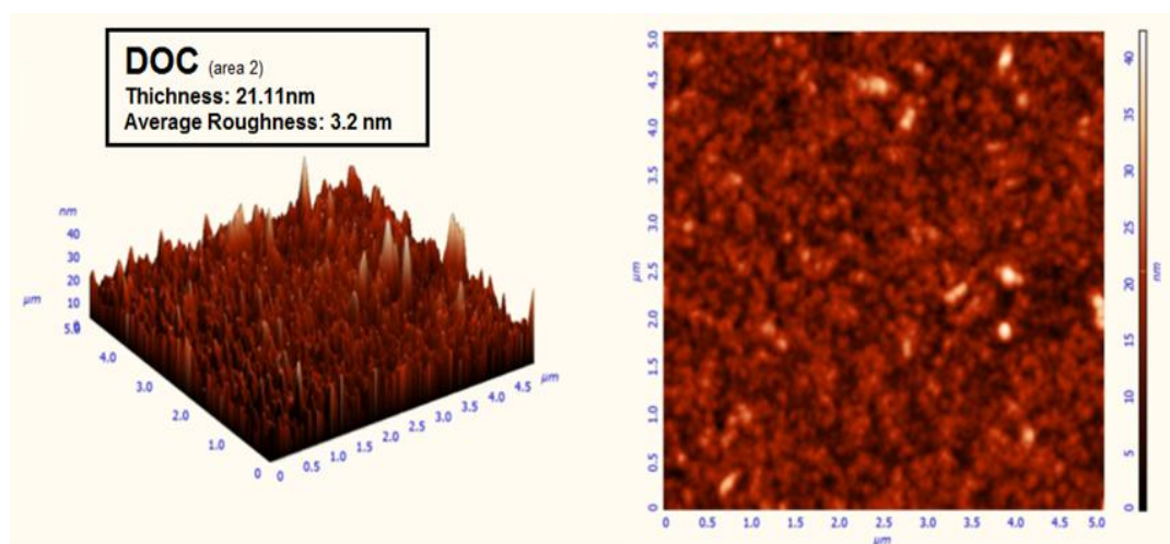
Figure 5.15 : The second AFM image of PEDOT:PSS coated glass, then spin casted for 5 times with WCNT and DOC mixture and has annealed at 110 °C
