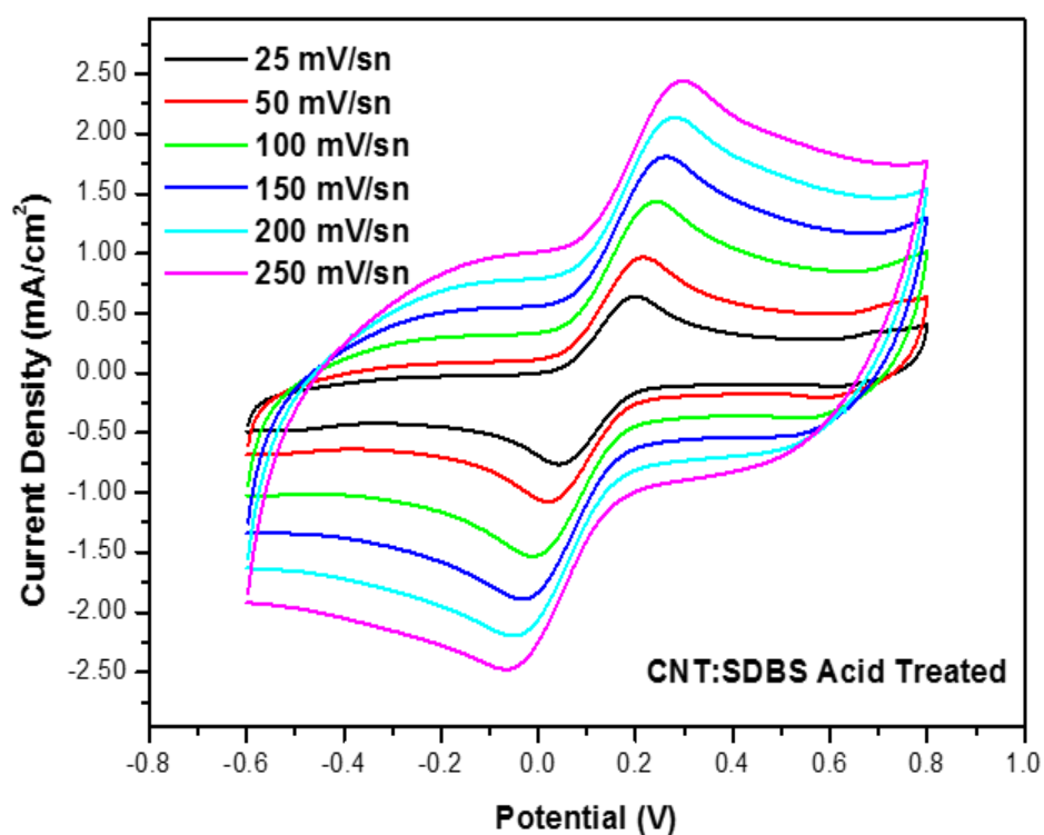
Figure 5.27 : CV curves of 5 mM K_3Fe(CN)_6 and 0.1 M KCl solution for SWNT/SDBS electrode after acid treatment.
