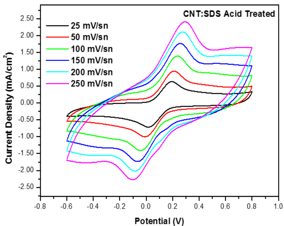
Figure 5.25: CV curves of 5 mM \text{K}_3\text{Fe}(\text{CN})_6 and 0.1 M KCl solution for SWNT/SDS electrode after acid treatment.
