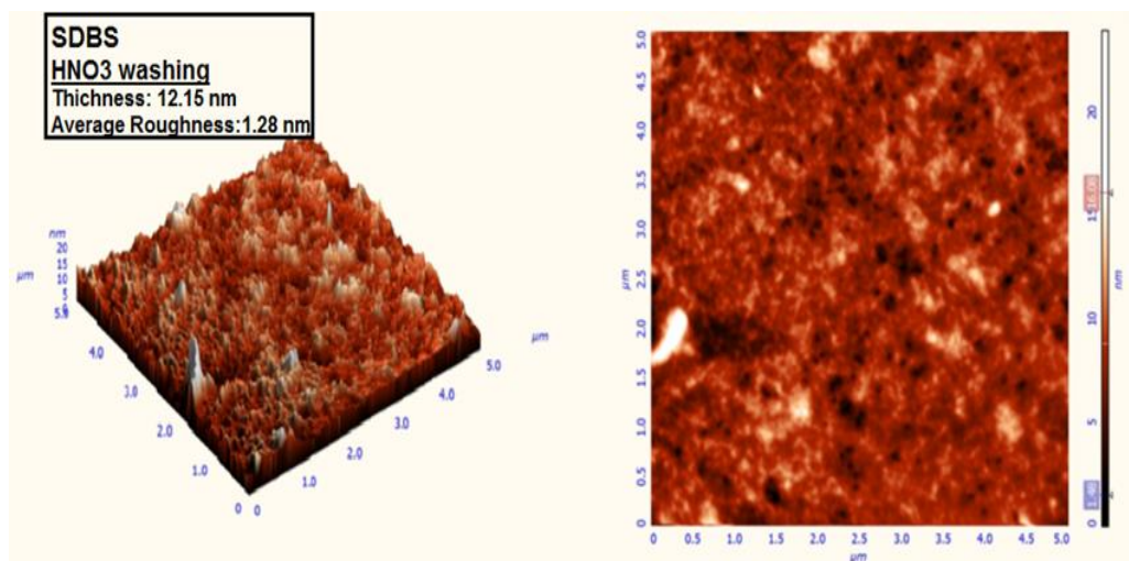
Figure 5.18: The morphology of CNT/SDBS films washed with \text{HNO}_3
