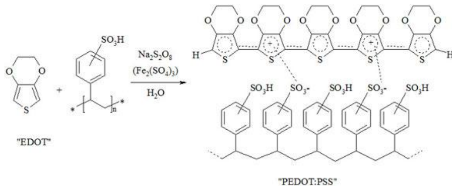
Figure 1.14 : Poly (3,4-ethylenedioxythiophene) PEDOT doped with poly(styrene 3sulfonate) chemical formula
