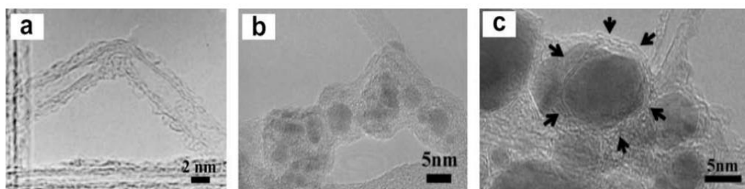
Figure 2.9: TEM images of (a) amorphous carbon and fullerene molecules on the surface of CNTs; (b) metal nanoparticles covered by amorphous carbon layer, (c) metal nanoparticles covered by graphitic carbon multi-layer[40]
