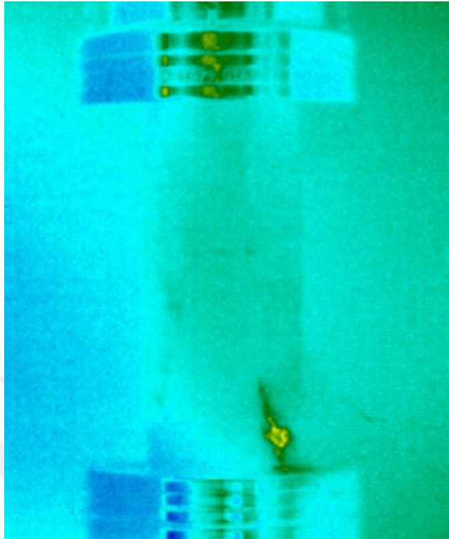
Figure B.23. Failure plane detection of the NLUCS-47 sample by the thermal camera
