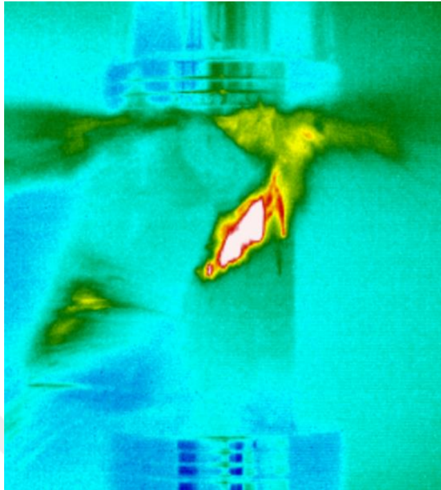
Figure B.21. Failure plane detection of the NLUCS-40 sample by the thermal camera
