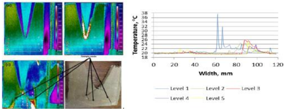
Figure 2.2. Loading of multiple crack initiation of the chevron sample with a notch angle of 45° and temperature profile (Antony et al.2017)
