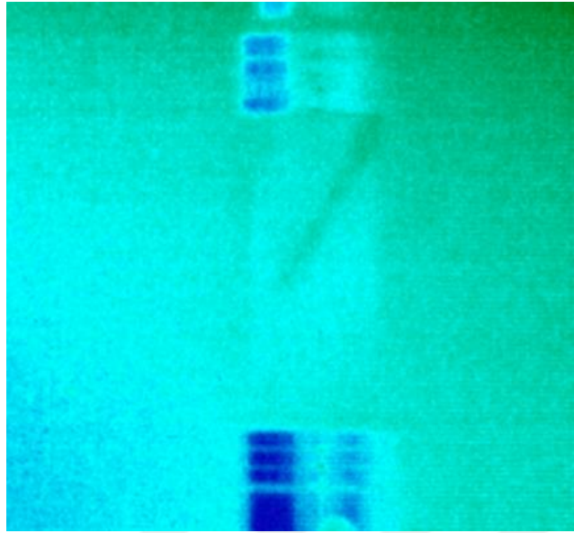
Figure B.13. Failure plane detection of the 42A-2 sample by the thermal camera
