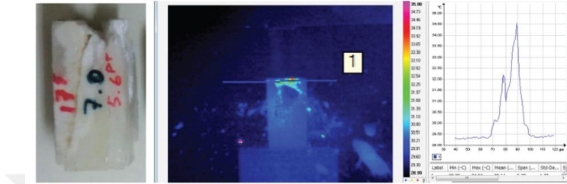
Figure 2.20. Visual and thermal image of Kuşini marble and temperature change along the selected line (Aydan et al., 2014)
