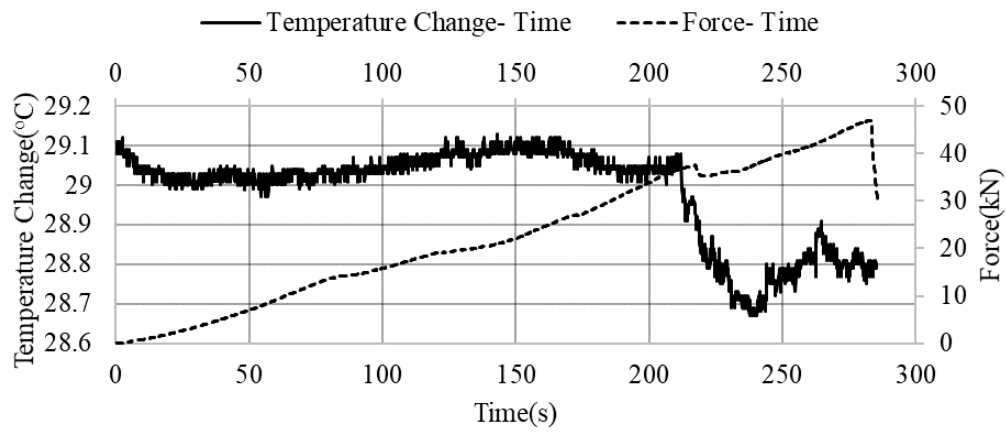
Figure C.19. Temperature change- Force- Time graph of the 42M-5 sample
