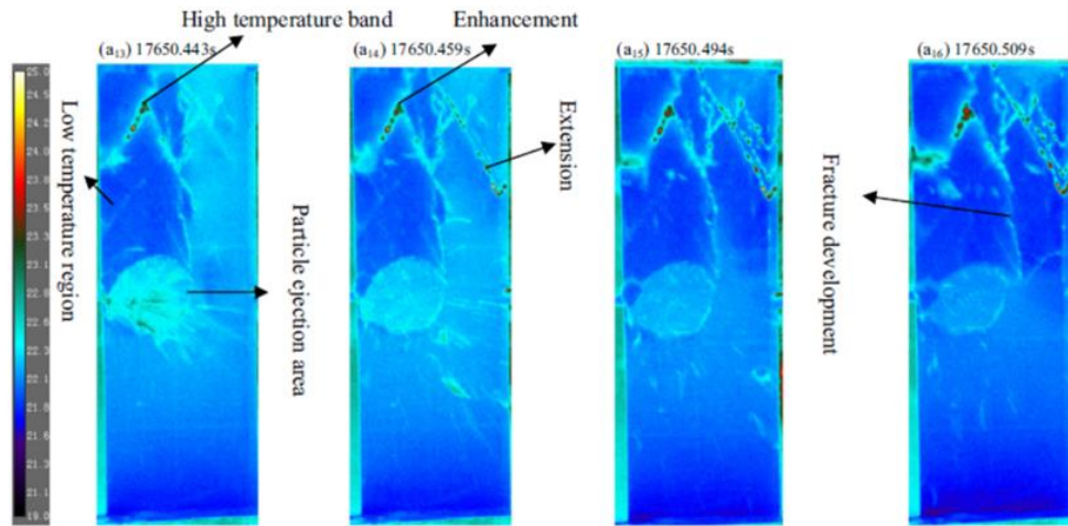
Figure 2.39. Time-dependent development of the particle removal phase (Sun et al., 2017)
