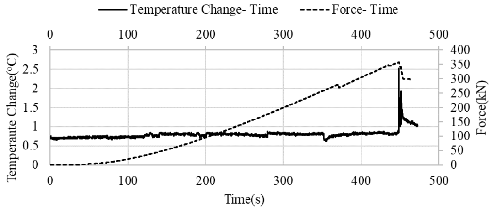
Figure C.28. Temperature change- Force- Time graph of the NLUCS-47 sample
