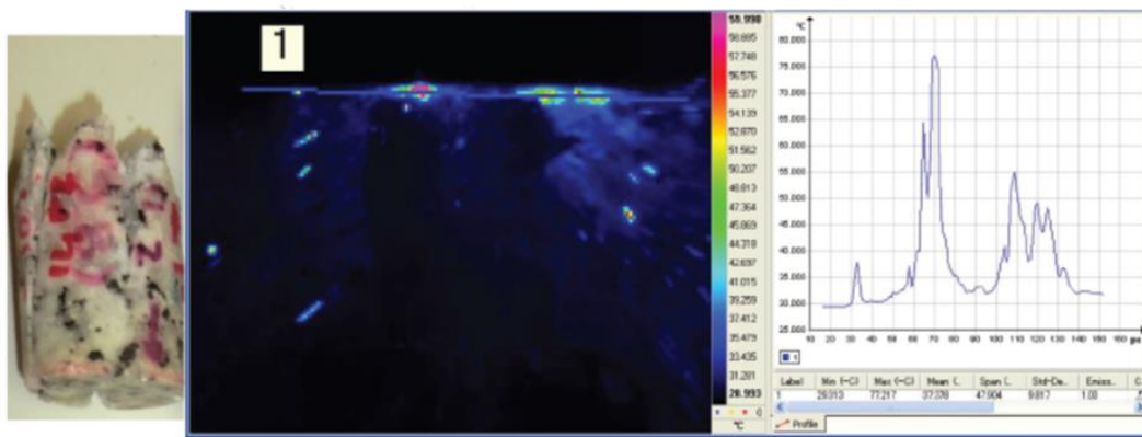
Figure 2.23. Visual and thermal image of Ehime granite and temperature change along the selected line (Aydan et al., 2014)
