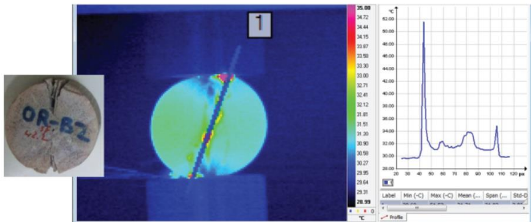
Figure 2.25. Investigation of indirect tensile strength test results of Kaore rhyolite by thermal camera and graph of temperature change along the selected line (Aydan et al., 2014)
