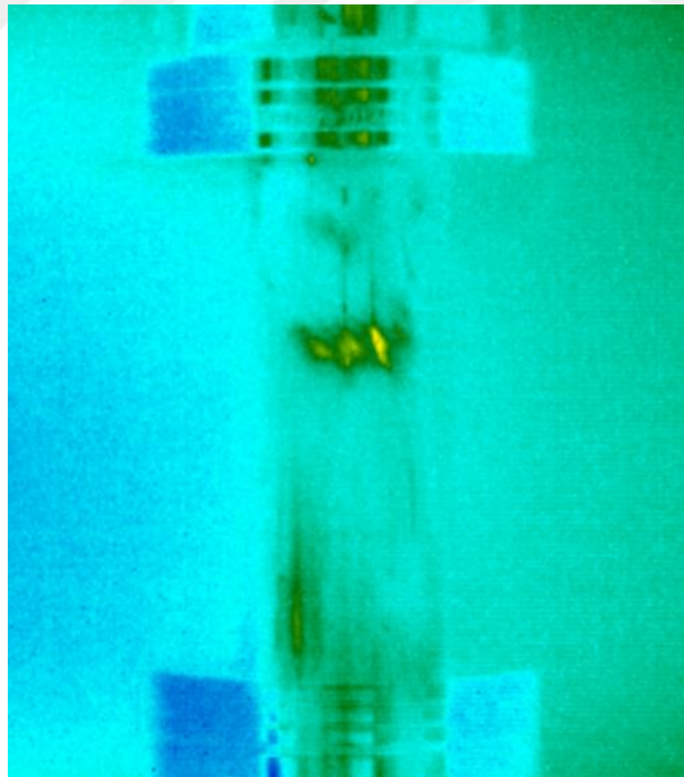
Figure B.24. Failure plane detection of the NLUCS-48 sample by the thermal camera
