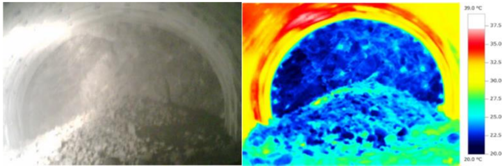
Figure 2.15. Visual and thermal image of the tunnel immediately after the blasting (Aydan et al., 2017)
