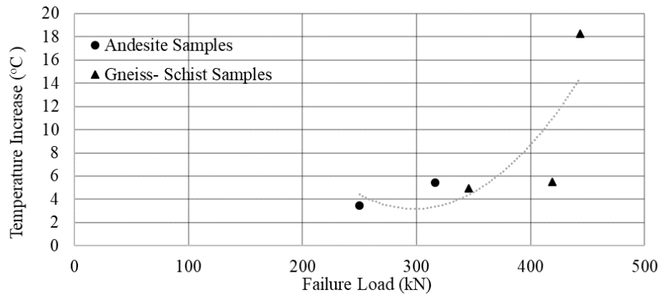
Figure 4.20. Temperature Increase- Failure Load graph of Andesite and Gneiss- Schist Samples with high temperature increase
