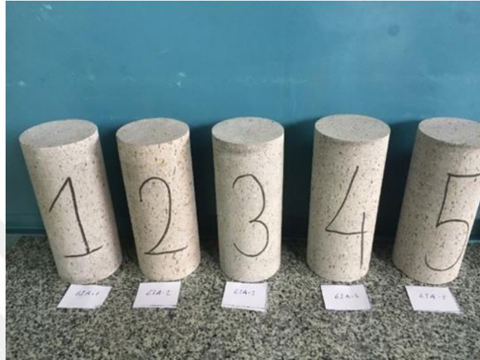
Figure 3.9. Andesite specimens with 63 mm diameter before test
