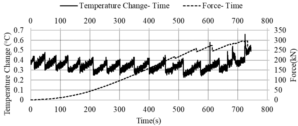
Figure C.2. Temperature change- Force- Time graph of the 75A-4 sample
