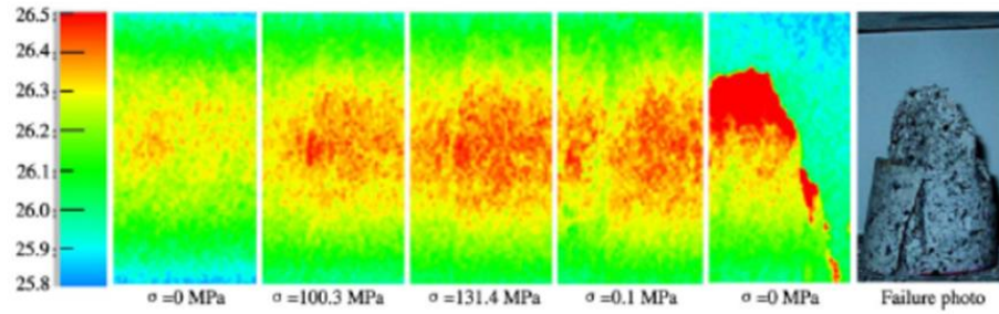
Figure 2.28. Granite specimen showing “J”- formed failure as a result of the uniaxial compression test (Wu et al.,2005)
