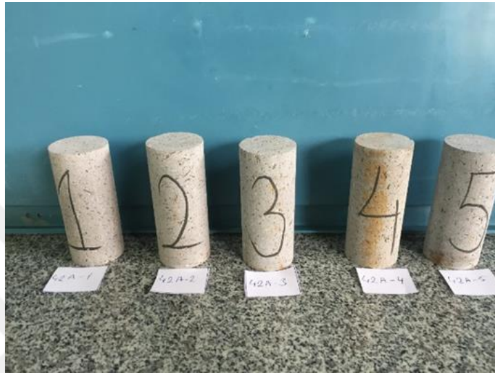
Figure 3.13. Andesite specimens with 42 mm diameter before test
