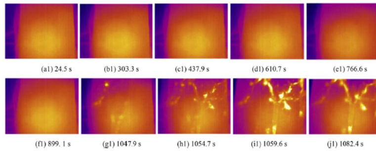
Figure 2.3. Investigation of loading moment and temperature changes with a thermal imager (Li et al., 2018)
