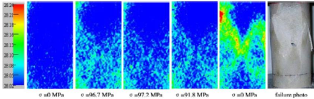
Figure 2.26. Marble specimen showing “X”- formed failure as a result of the uniaxial compression test (Wu et al.,2005)
