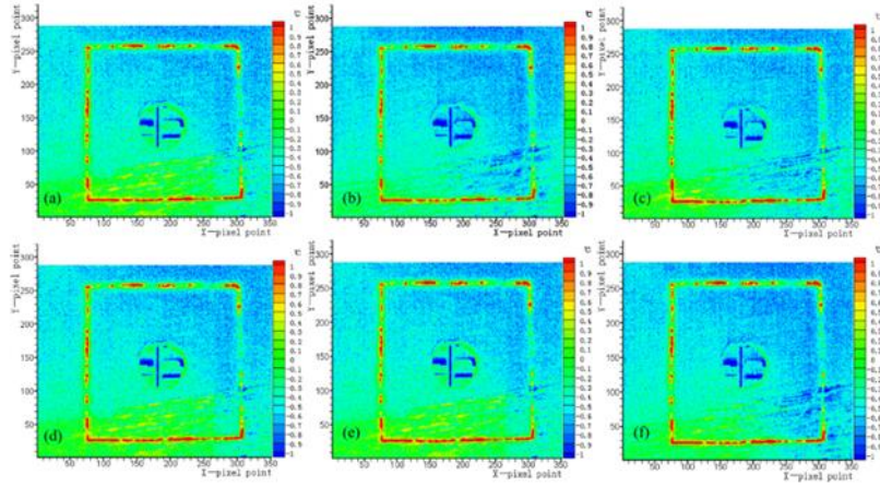
Figure 2.47. Temperature change during stage C3 (Sun et al., 2017)
