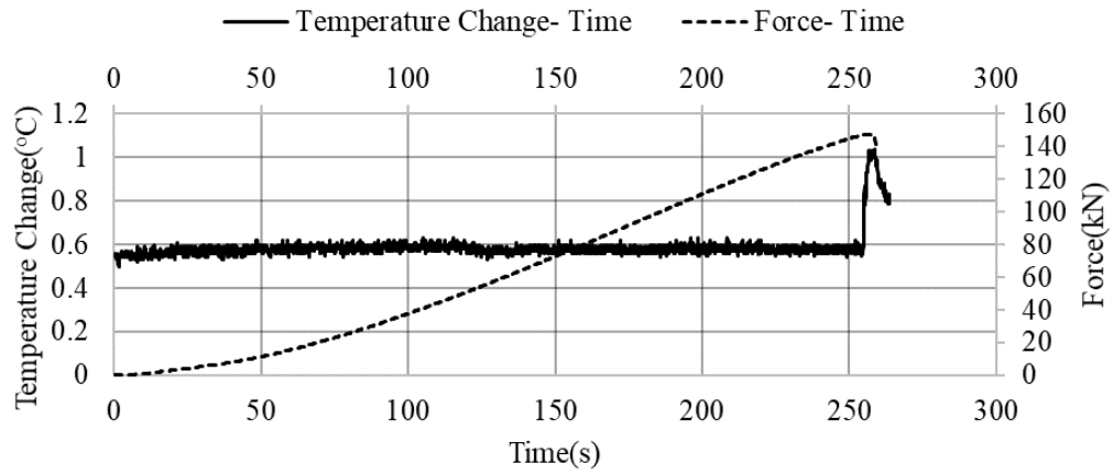
Figure C.26. Temperature change- Force- Time graph of the NLUCS-41 sample
