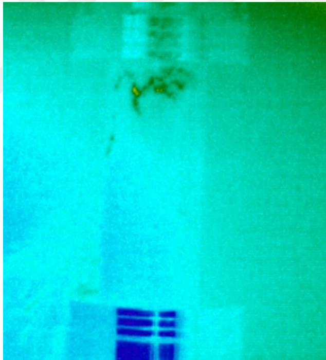
Figure B.4. Failure plane detection of the 63A-1 sample by the thermal camera
