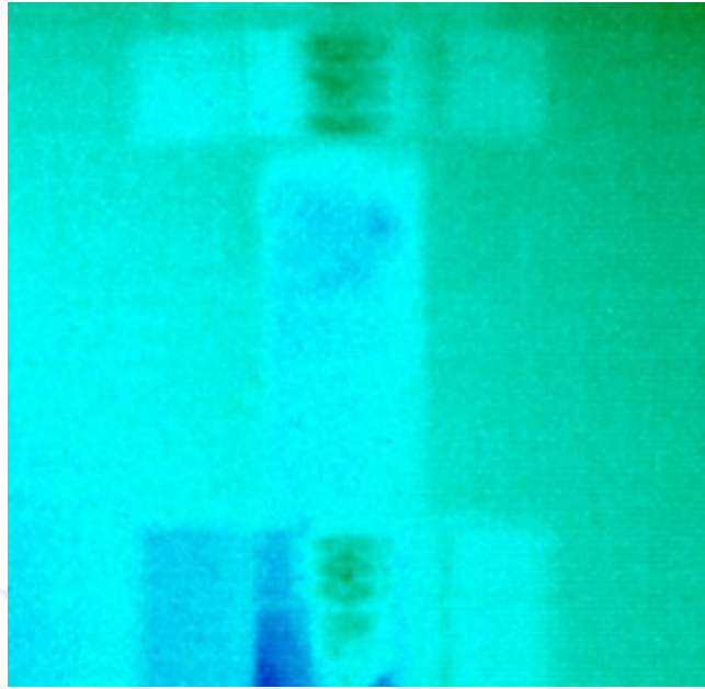
Figure B.19. Failure plane detection of the 42M-5 sample by the thermal camera
