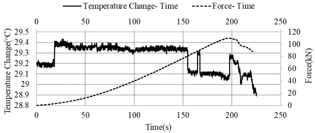
Figure C.16. Temperature change- Force- Time graph of the 53M-1 sample
