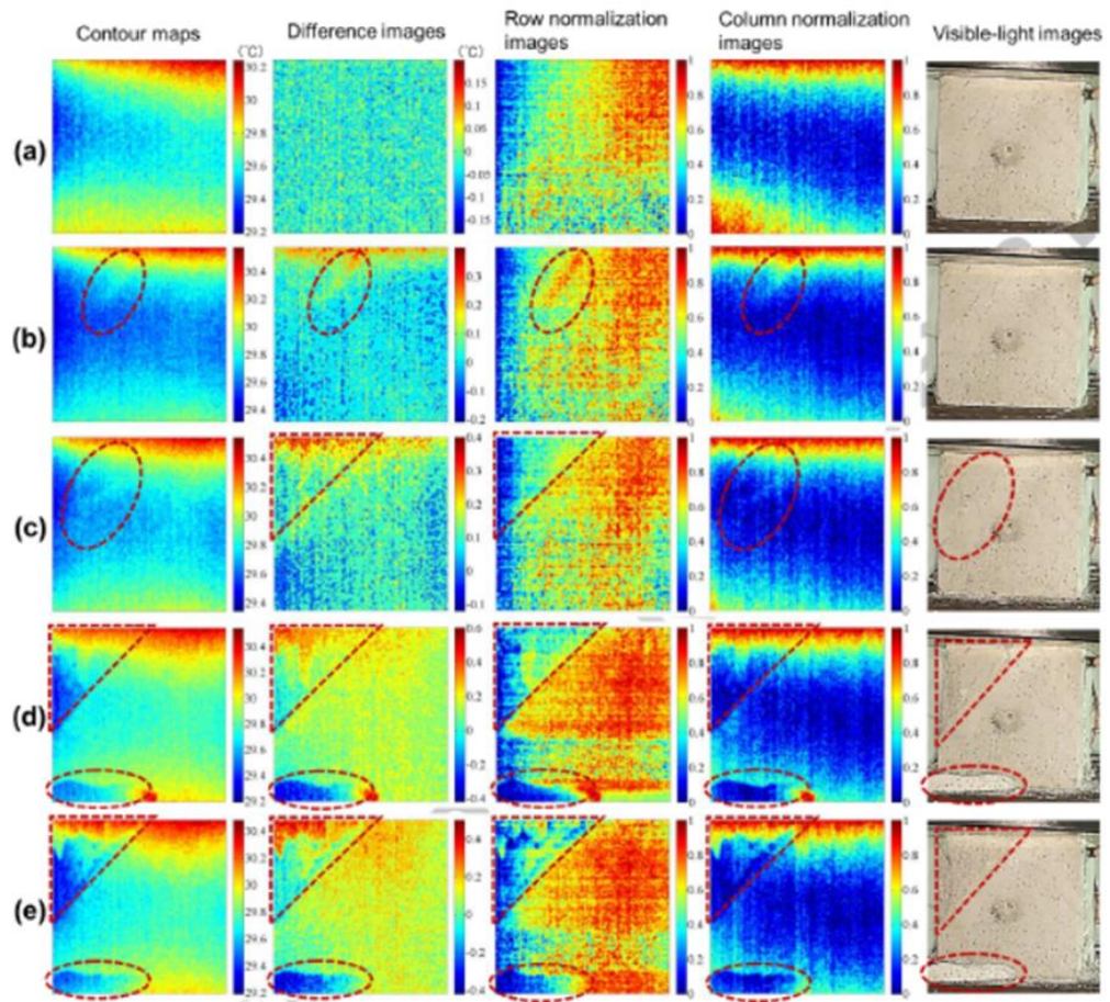
Figure 2.8. Different loading amounts and temperature increase regions; a) time: 6s, load ratio: 0.5% b) time:115s, load ratio: 66.6%, c) time: 155s, load ratio: 89%, d) time: 197s, load ratio: 88.2%, e) time:246s, load ratio: 32.1% (Lou & He, 2018)
