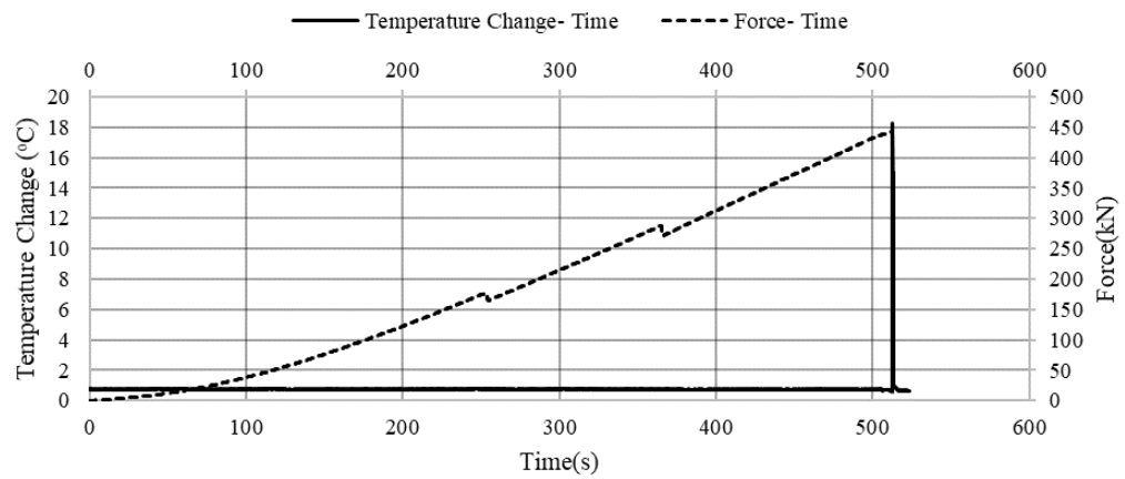
Figure C.20. Temperature change- Force- Time graph of the NLUCS-40 sample
