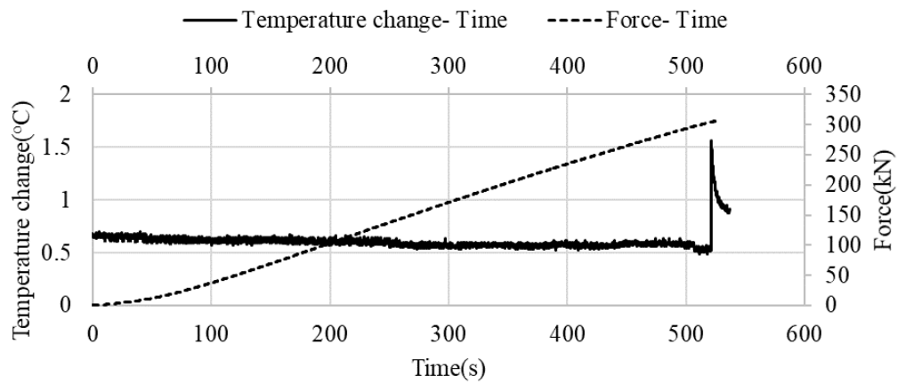
Figure C.6. Temperature change- Force- Time graph of the 63A-5 sample
