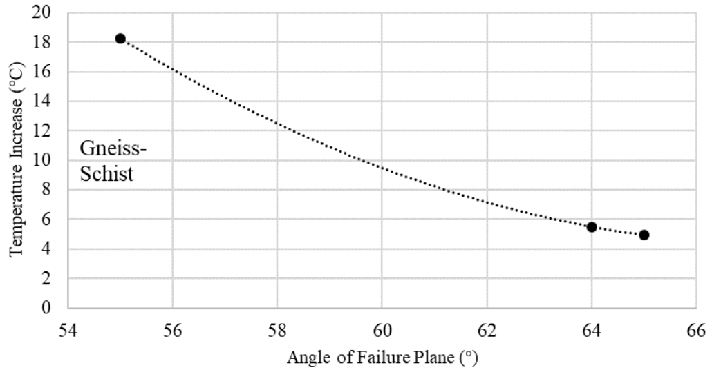
Figure 4.23. Angle of Failure Plane- Temperature Increase graph of Gneiss-Schist Samples with high temperature increase
