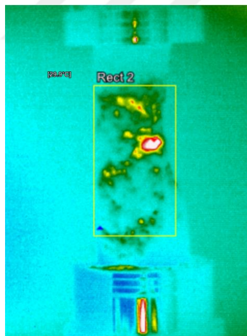
Figure 4.1. Failure plane detection of the 75A-1 sample by the thermal camera
