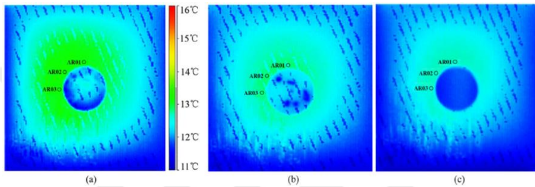
Figure 2.17. Investigation of uniaxial compressive strength test results in the concrete slab with the thermal camera; a) Preload phase b) First excavation (660 seconds) c) Second excavation (1180 seconds) (Wang et al., 2018)
