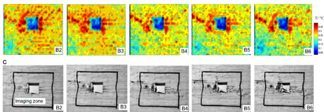
Figure 2.36. Thermal camera images taken at that moment; stress conditions (MPa); B2(2.5,1.4), B3(3,1.4), B4(4,1.4), B5(5,1.4), B6(6,1.4) (Gong et al., 2015)
