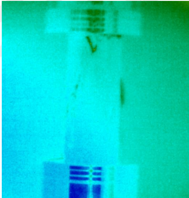
Figure B.6. Failure plane detection of the 63A-5 sample by the thermal camera
