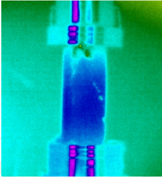
Figure B.7. Failure plane detection of the 63AA-2 sample by the thermal camera
