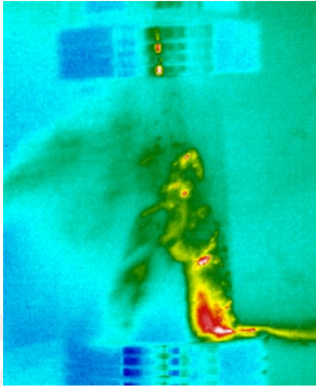
Figure B.25. Failure plane detection of the NLUCS-49 sample by the thermal camera
