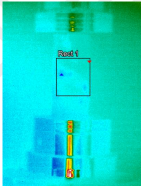
Figure 4.11. Failure plane detection of the 53M-2 sample by the thermal camera
