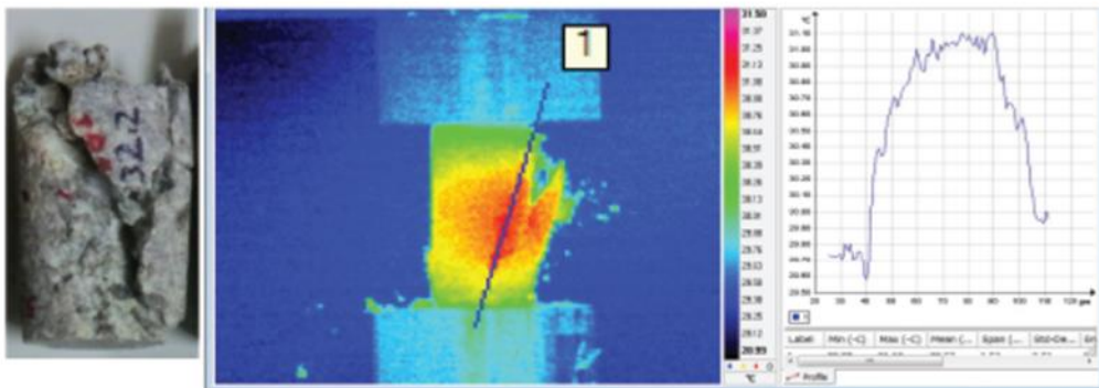
Figure 2.19. Visual and thermal image of Sinop Tuff and graph of temperature change along the selected line (Aydan et al.,2014)
