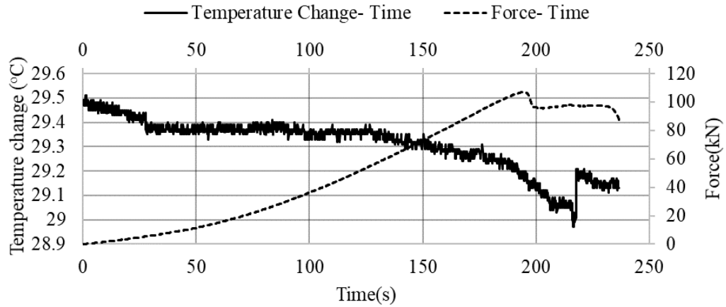
Figure 4.12. Temperature change- Force- Time graph of the 53M-2 sample
