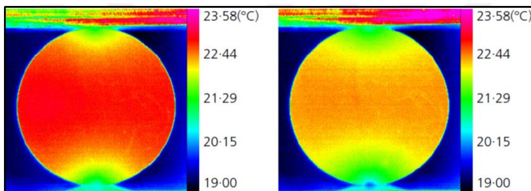
Figure 2.30. Temperature concentration at the contact points before and after the experiment (Salami et al., 2017)
