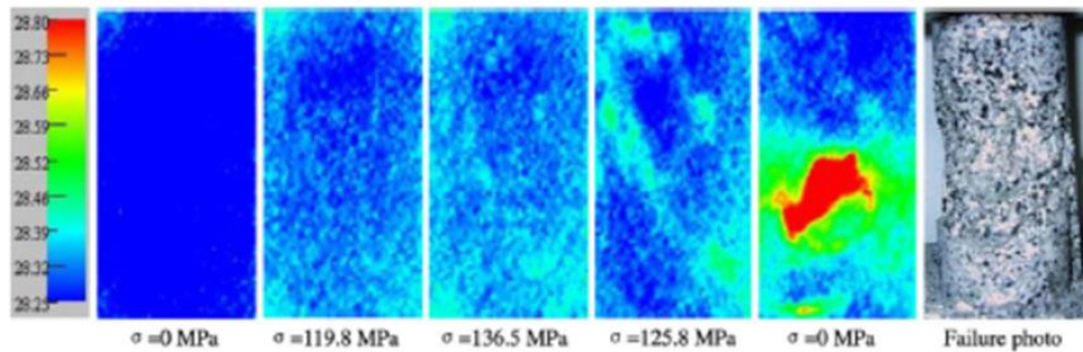
Figure 2.27. Granite specimen showing “//”- formed failure as a result of the uniaxial compression test (Wu et al.,2005)
