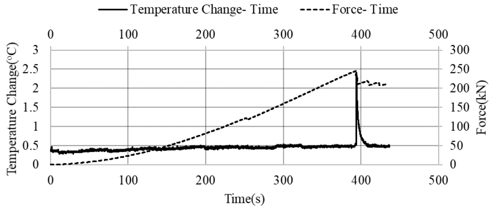
Figure C.22. Temperature change- Force- Time graph of the NLUCS-55 sample
