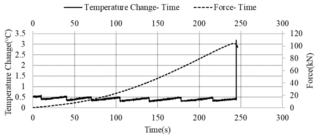
Figure C.21. Temperature change- Force- Time graph of the NLUCS-37 sample
