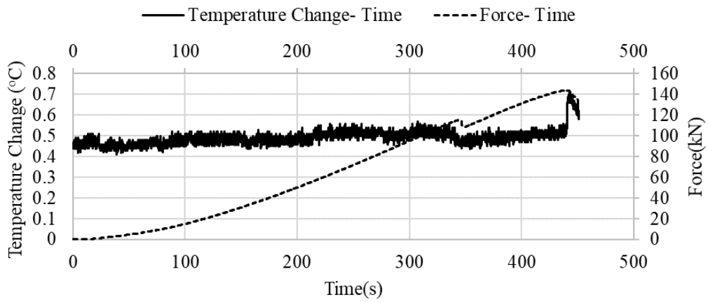
Figure C.11. Temperature change- Force- Time graph of the 53A-4 sample
