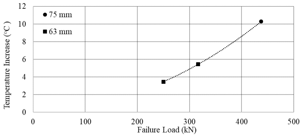
Figure 4.26. Temperature Increase- Failure Load graph of Andesite Samples with high temperature increase
