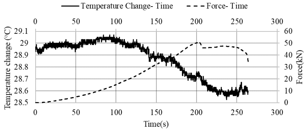
Figure 4.14. Temperature change- Force- Time graph of the 42M-3 sample
