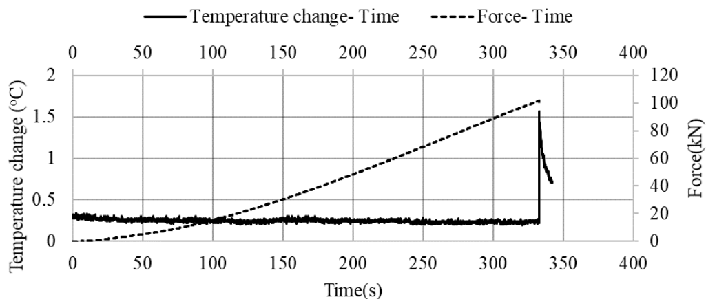
Figure 4.8. Temperature change- Force- Time graph of the 42A-5 sample
