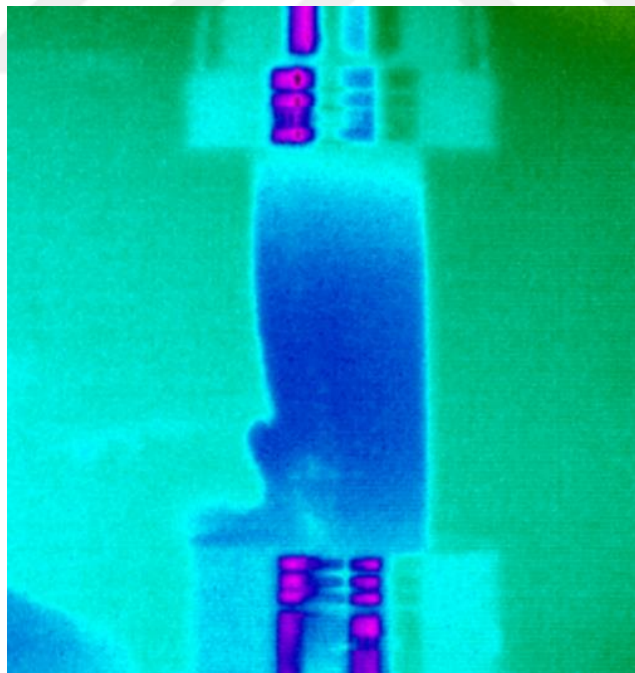
Figure B.10. Failure plane detection of the 63AA-9 sample by the thermal camera
