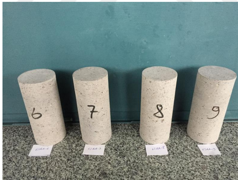
Figure A.2. Pre-test image of some of the 63 mm diameter andesite samples (63AA6 to 63 AA9)
