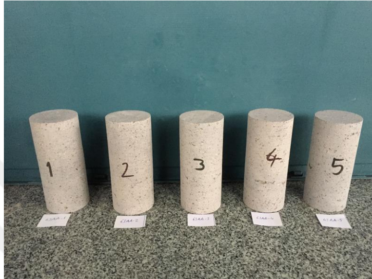
Figure A.1. Pre-test image of some of the 63 mm diameter andesite samples (63AA1 to 63 AA5)
