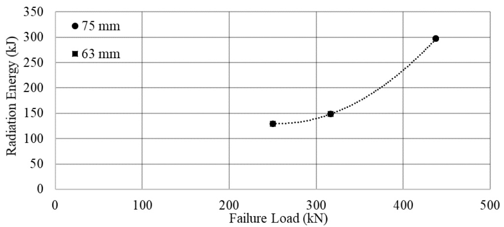
Figure 4.27. Radiation Energy- Failure Load graph of Andesite Samples with high temperature increase
