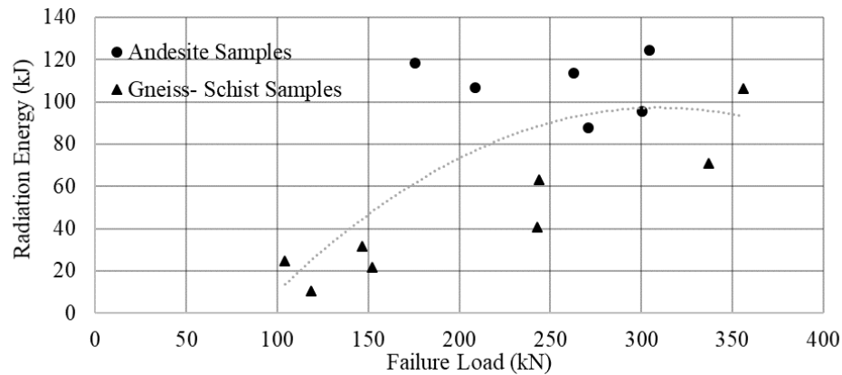
Figure 4.19. Radiation Energy- Failure Load graph of Andesite and Gneiss- Schist Samples with low temperature increase
