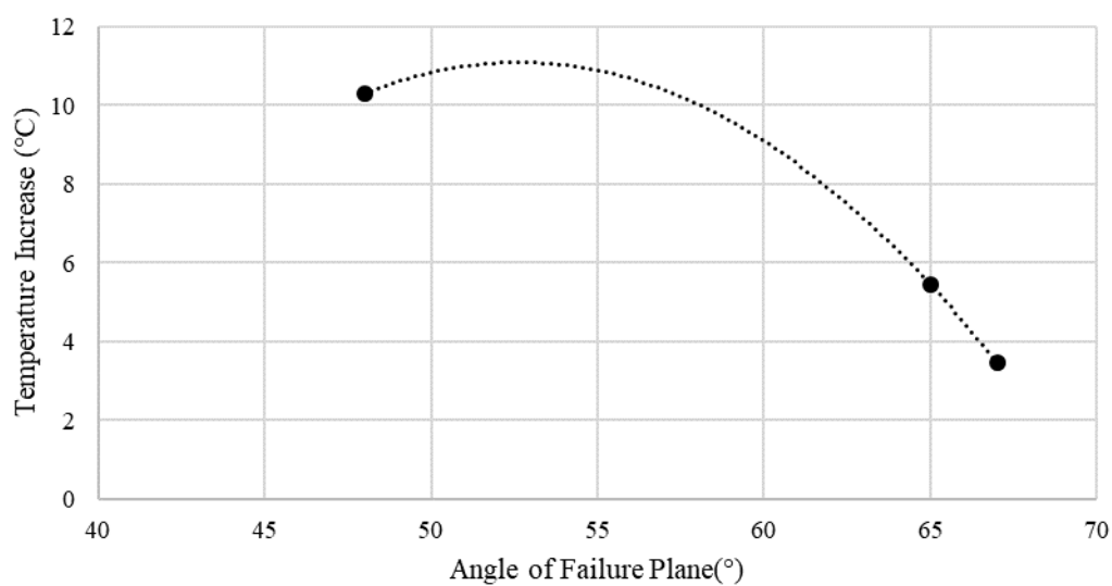
Figure 4.22. Angle of Failure Plane- Temperature Increase graph of Andesite Samples with high temperature increase
