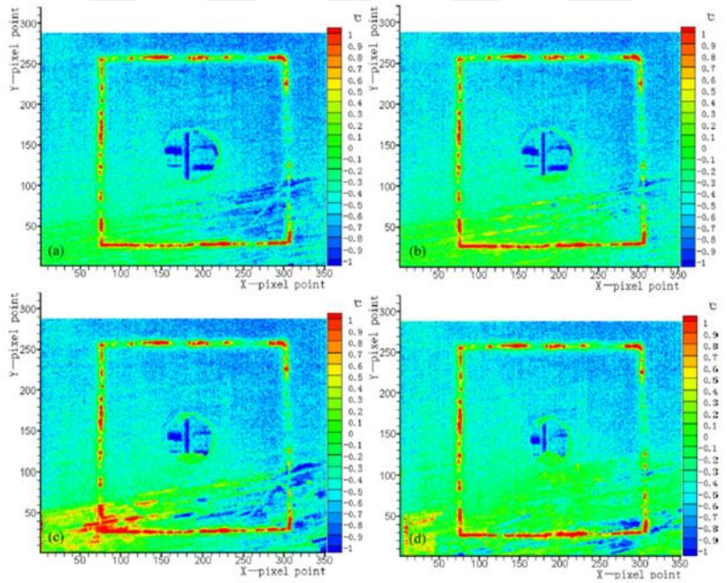
Figure 2.48. Temperature change during stage C4 (Sun et al., 2017)
