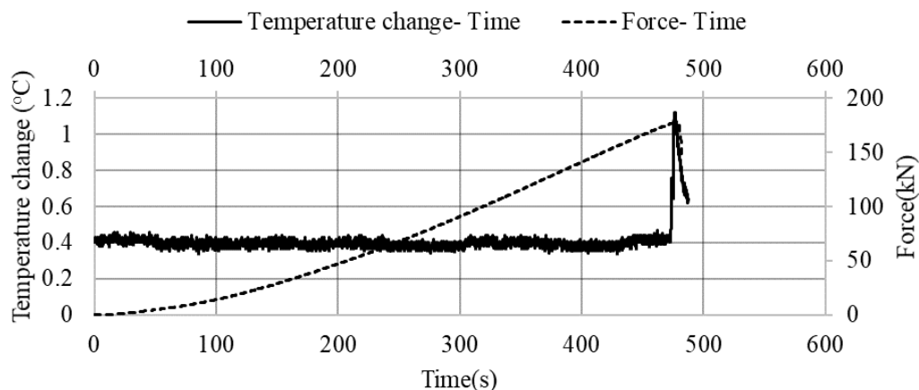
Figure 4.6 Temperature change- Force- Time graph of the 53A-1 sample
