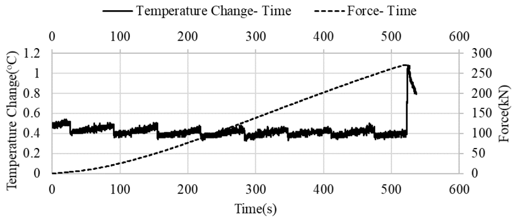
Figure C.5. Temperature change- Force- Time graph of the 63A-2 sample
