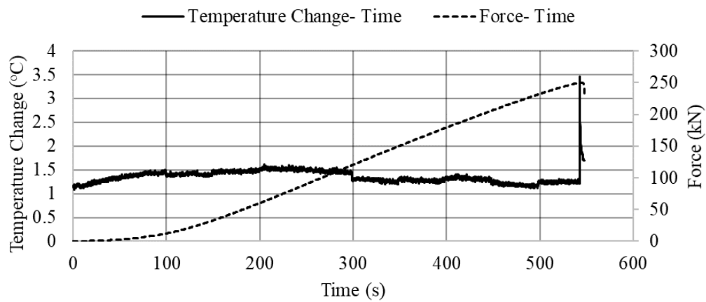
Figure C.7. Temperature change- Force- Time graph of the 63AA-2 sample
