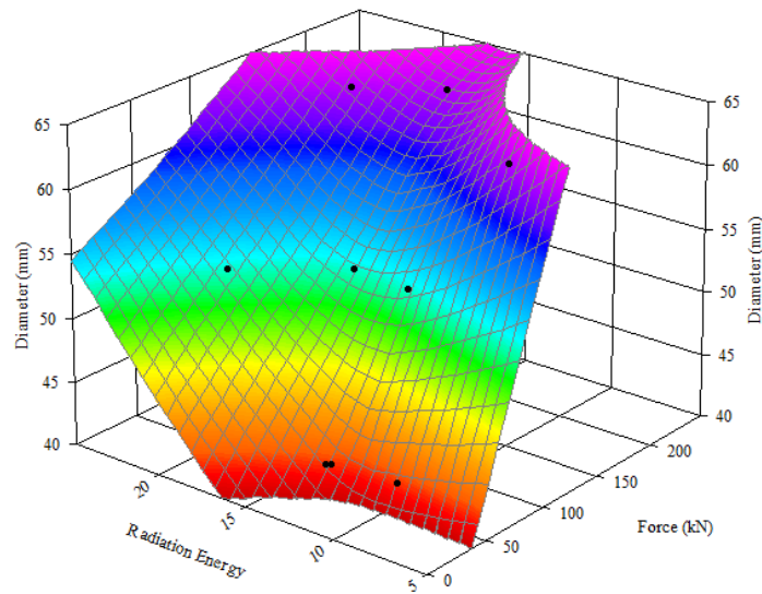
Figure 4.29. Radiation Energy- Failure Load- Diameter Size of the Marble Samples
