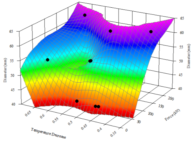
Figure 4.28. Temperature Decrease-Failure Load-Diameter Size of the Marble Samples
