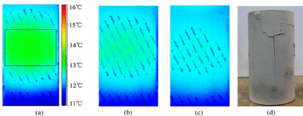
Figure 2.16. Investigation of the uniaxial compressive strength test result of cylinder concrete sample by the thermal camera; a) Before Loading b) Before Failure c) After Failure d) Visual Image of Sample After Failure (Wang et al., 2018)
