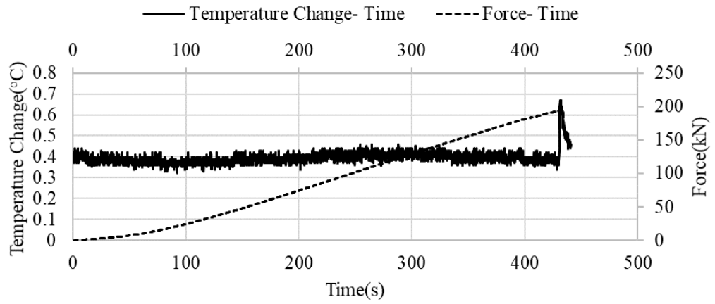
Figure C.12. Temperature change- Force- Time graph of the 53A-5 sample
