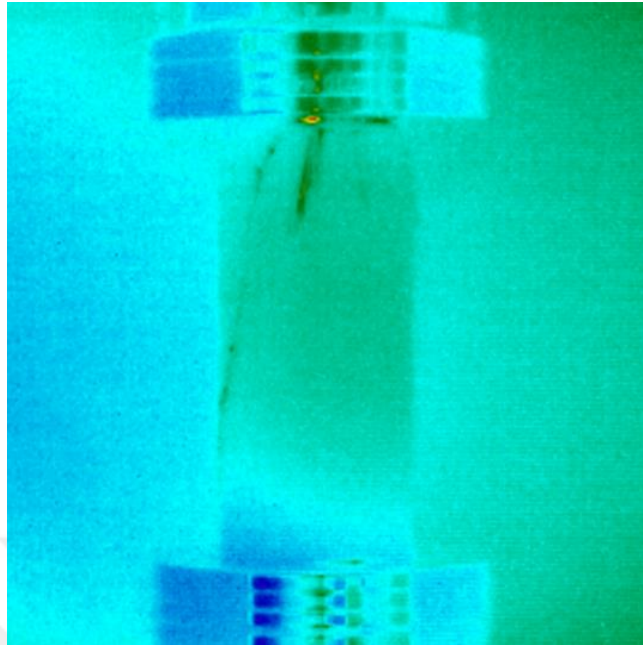
Figure B.27. Failure plane detection of the NLUCS-57 sample by the thermal camera
