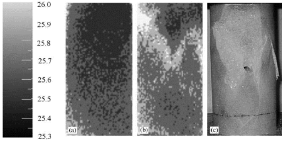
Figure 2.10. Thermal images of marble samples during loading and failure moment (Liu et al., 2006)
