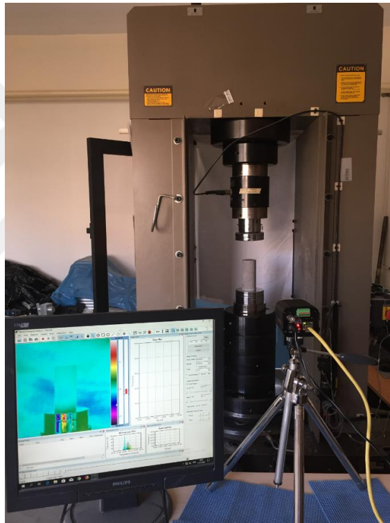
Figure 3.1. MTS 815 test system
