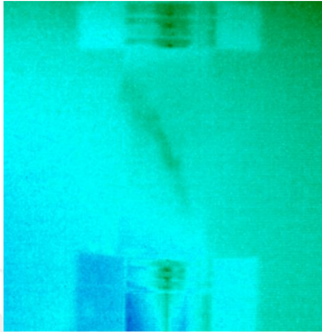
Figure B.11. Failure plane detection of the 53A-4 sample by the thermal camera
