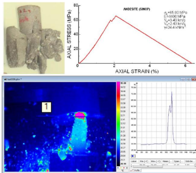
Figure 2.13. Temperature increase regions of Sinop Andesite as a result of the uniaxial compression test (Aydan et al., 2017)
