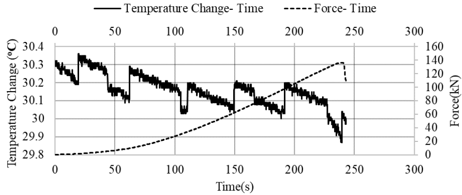
Figure 4.10. Temperature change- Force- Time graph of the 63M-3 sample
