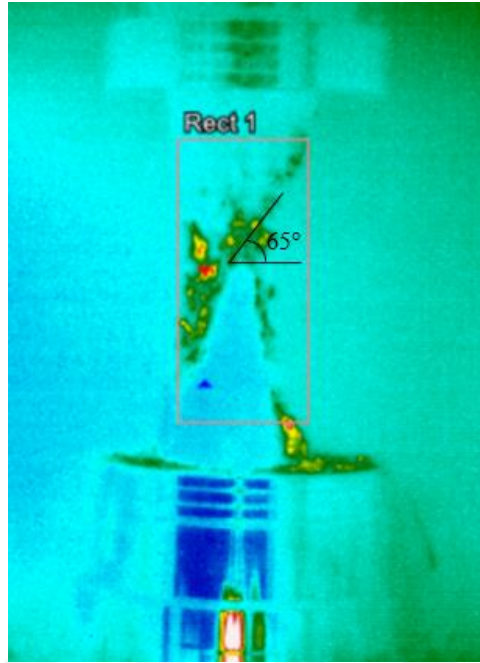
Figure 4.3. Failure plane detection of the 63A-4 sample by the thermal camera
