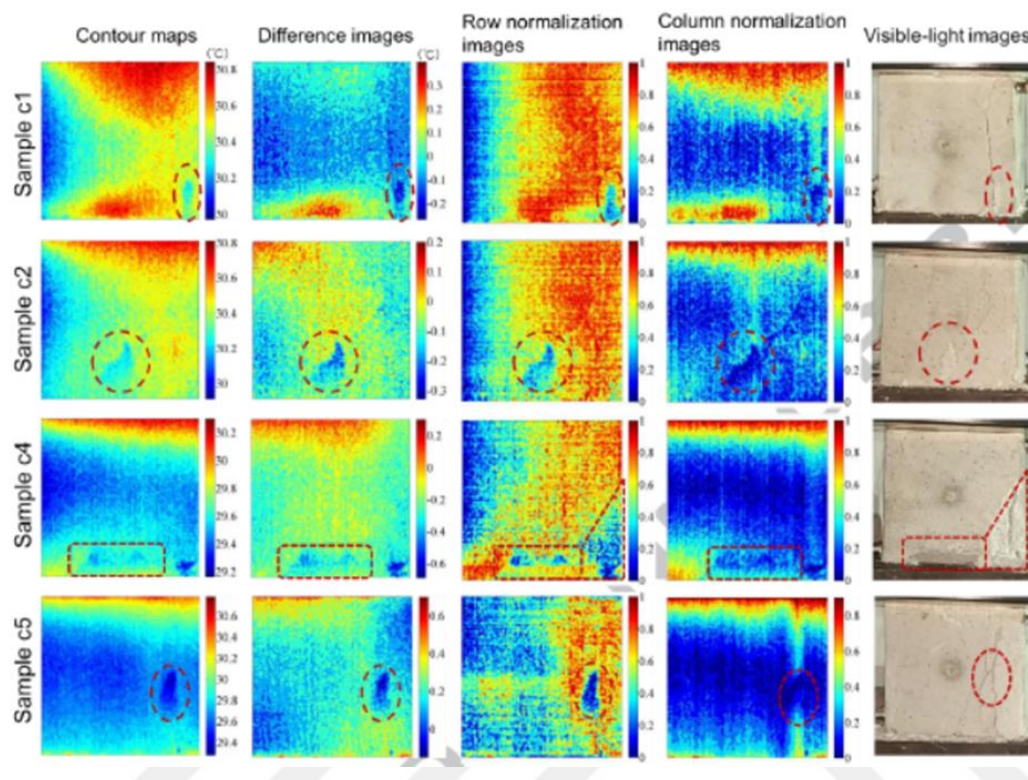
Figure 2.9. Detection of crack formation areas in different concrete samples by the thermal camera (Lou & He, 2018)
