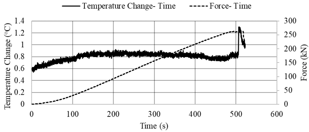
Figure C.10. Temperature change- Force- Time graph of the 63AA-9 sample
