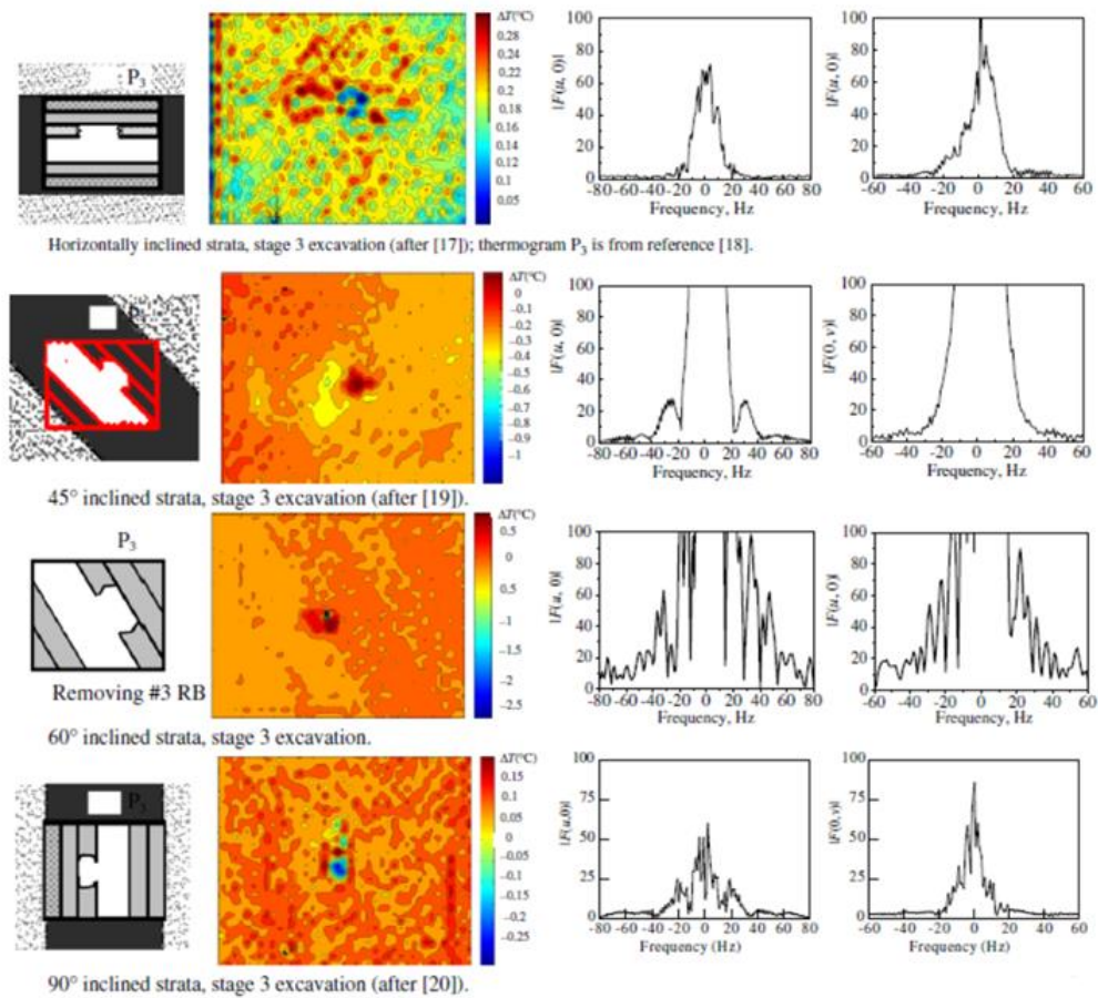
Figure 2.34. Investigation of the temperature change resulting from the road excavated in the slopes of 0°, 45°, 60° and 90° (Gong et al., 2012)
