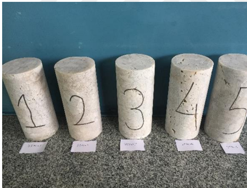
Figure 3.15. Marble specimens with 75 mm diameter after test
