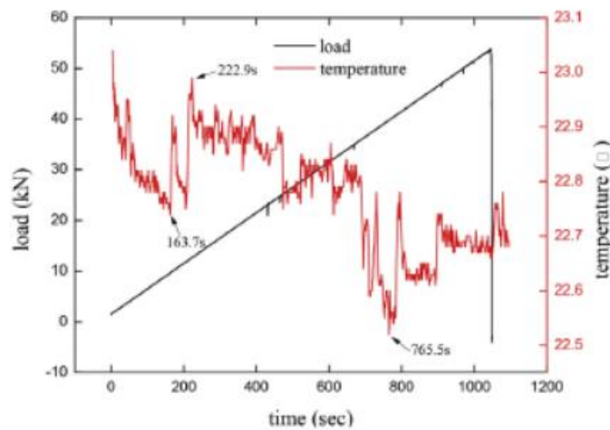
Figure 2.4. Load- Temperature- Time graph (Li et al., 2018)
