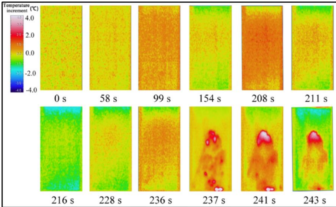
Figure 2.32. Time- spatial formation of different thermograms (Wang et al., 2016)
