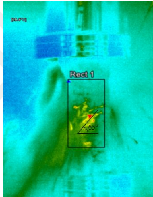
Figure 4.15. Failure plane detection of the NLUCS-56 sample by the thermal camera
