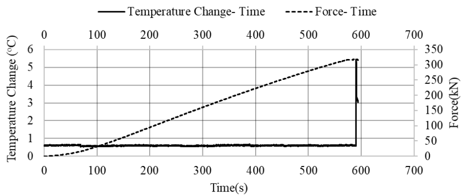
Figure 4.4. Temperature change- Force- Time graph of the 63A-4 sample
