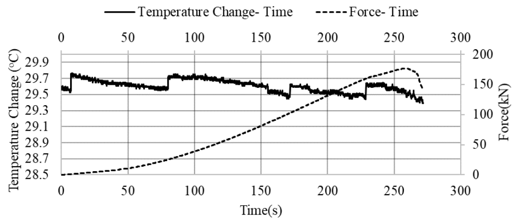
Figure C.15. Temperature change- Force- Time graph of the 63M-4 sample
