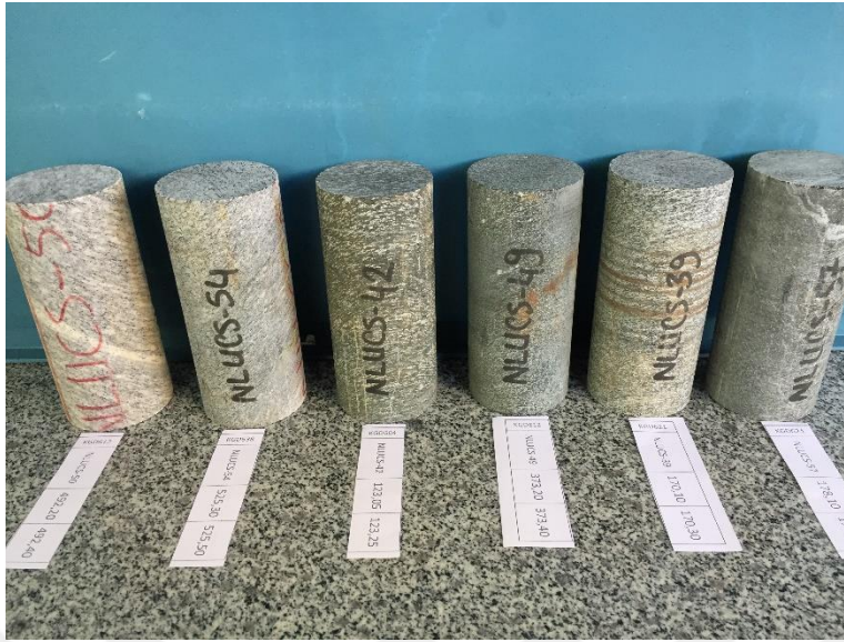
Figure A.7. Pre-test image of some of the gneiss-schist samples
