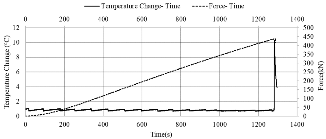
Figure 4.2 Temperature change- Force- Time graph of the 75A-1 sample
