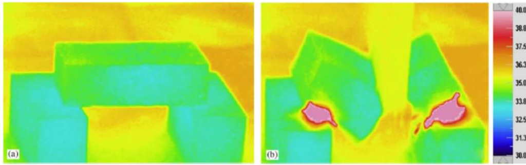
Figure 2.12. Three-point bending test of granodiorite samples and thermal image (Liu et al., 2006)
