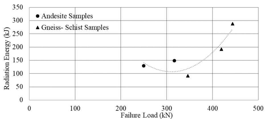
Figure 4.21. Radiation Energy- Failure Load graph of Andesite and Gneiss- Schist Samples with high temperature increase
