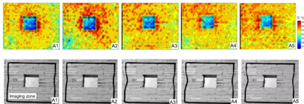
Figure 2.35. Thermal camera images taken at that moment; stress conditions (MPa); A1(0.8,0.8), A2(0.8,0.8), A3(0.8,0.8), A4(1.4,1.4), A5(1.4,1.4) (Gong et al., 2015)
