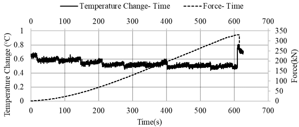
Figure C.3. Temperature change- Force- Time graph of the 75A-5 sample
