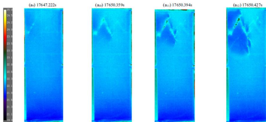
Figure 2.38. Time-dependent development of the crack propagation phase (Sun et al., 2017)
