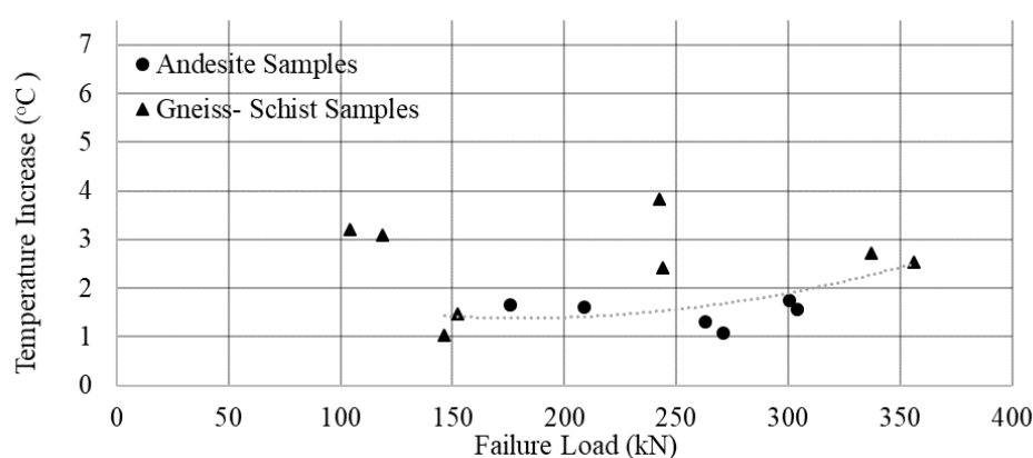
Figure 4.18. Temperature Increase- Failure Load graph of Andesite and Gneiss- Schist Samples with low temperature increase
