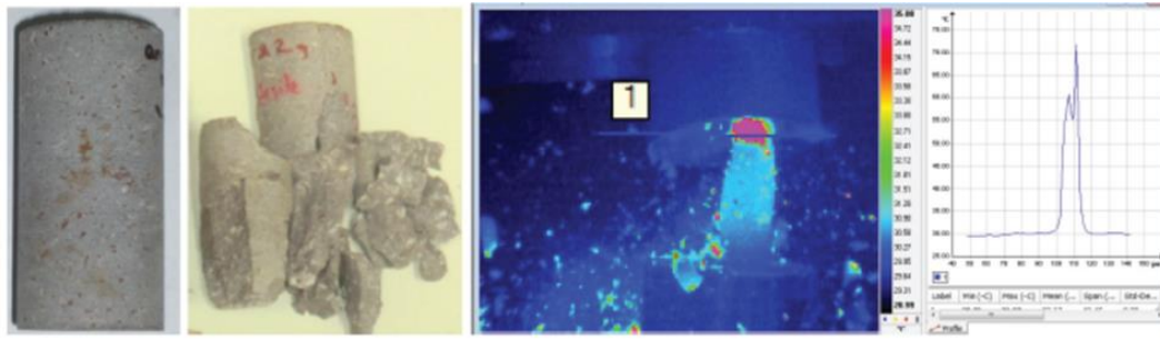
Figure 2.22. Visual and thermal image of Sinop Andesite and temperature change along the selected line (Aydan et al., 2014)
