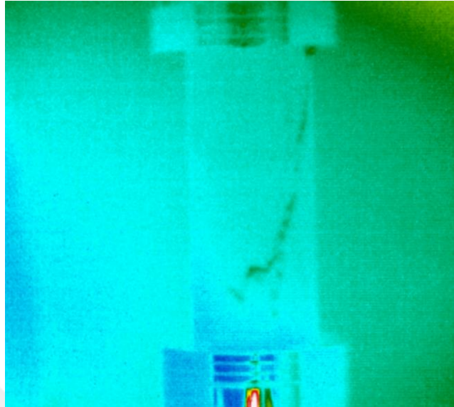
Figure B.1. Failure plane detection of the 75A-3 sample by the thermal camera
