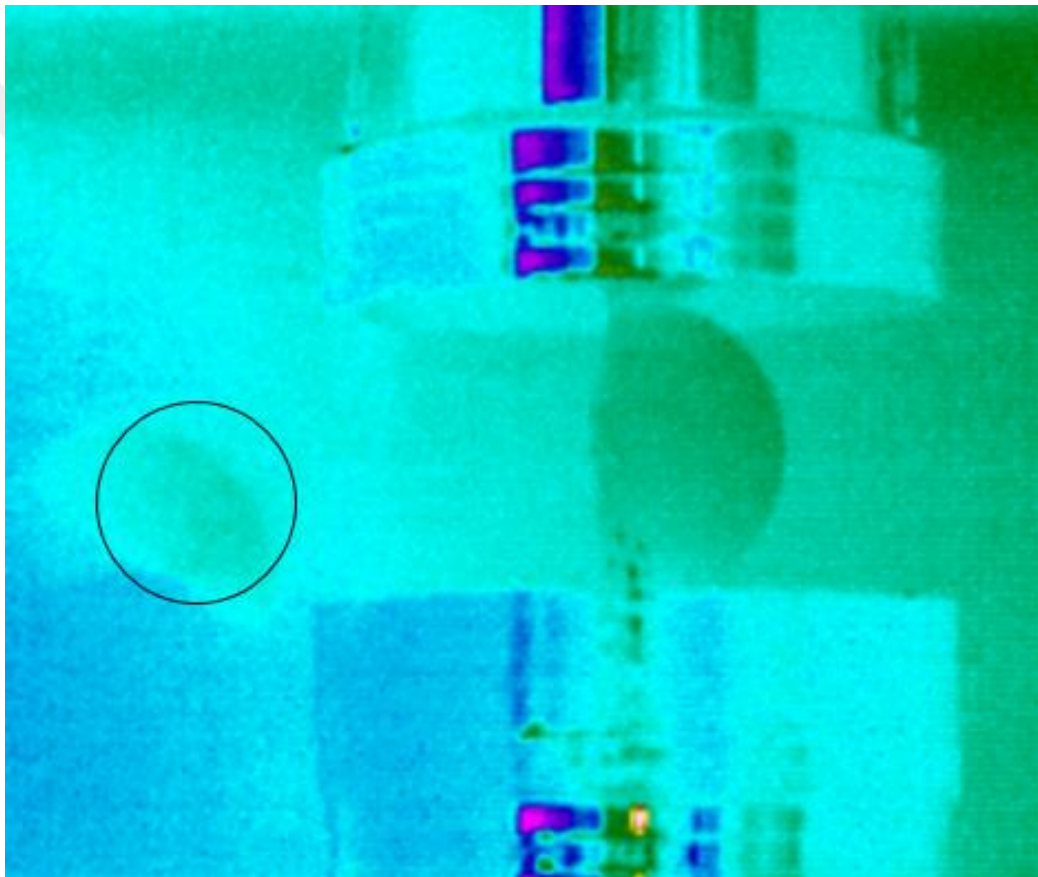
Figure 3.5. Thermal image of Brazilian test
