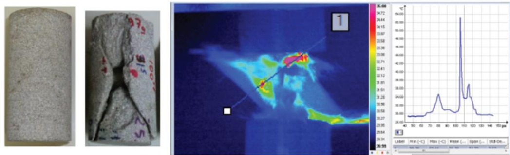
Figure 2.21. Visual and thermal image of the Ehime Sandstone and temperature change along the selected line (Aydan et al., 2014)
