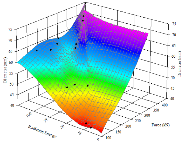
Figure 4.25. Radiation Energy-Failure Load graph of Andesite Samples with low temperature increase
