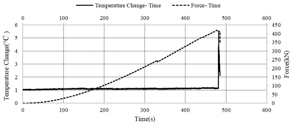
Figure C.23. Temperature change- Force- Time graph of the NLUCS-49 sample
