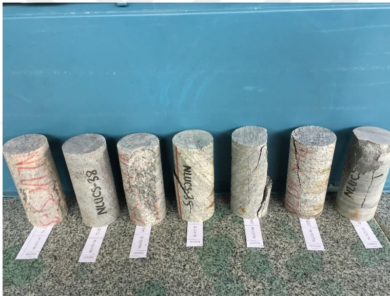
Figure A.12. Post-test image of some of the gneiss-schist samples
