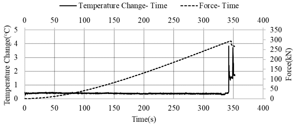
Figure C.24. Temperature change- Force- Time graph of the NLUCS-57 sample
