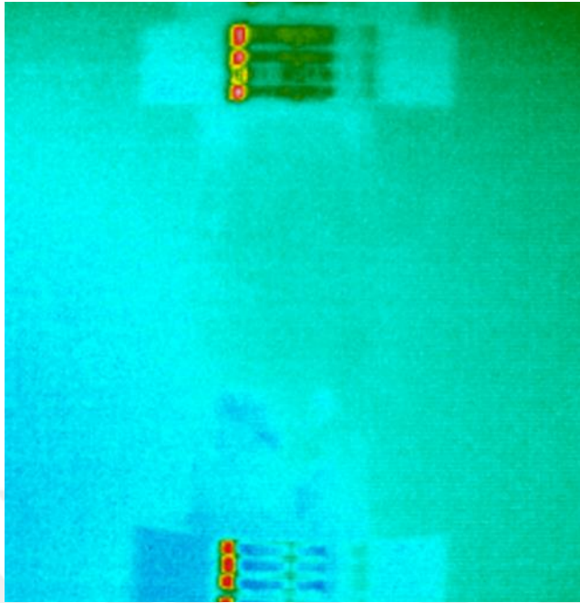
Figure B.15. Failure plane detection of the 63M-4 sample by the thermal camera
