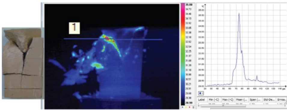
Figure 2.18. Visual and thermal image of Seyitömer Claystone and graph of temperature change along the selected line (Aydan et al.,2014)
