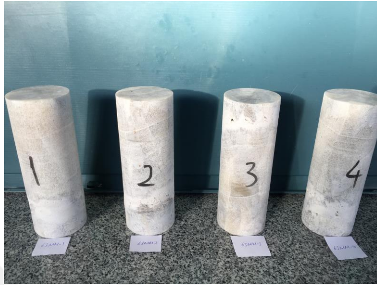
Figure A.5. Pre-test image of some of the 63 mm diameter marble samples (63MM1 to 63 MM4)
