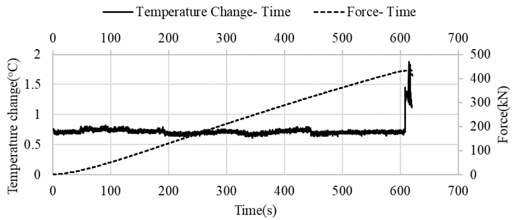
Figure C.1. Temperature change- Force- Time graph of the 75A-3 sample
