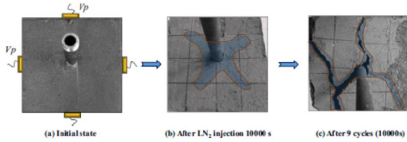
Figure 2.6. Investigation of crack formation by injecting liquid nitrogen during the triaxial test (Qin et al., 2018)
