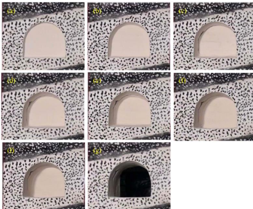
Figure 2.41. Eight stages of the excavation (Sun et al., 2018)
