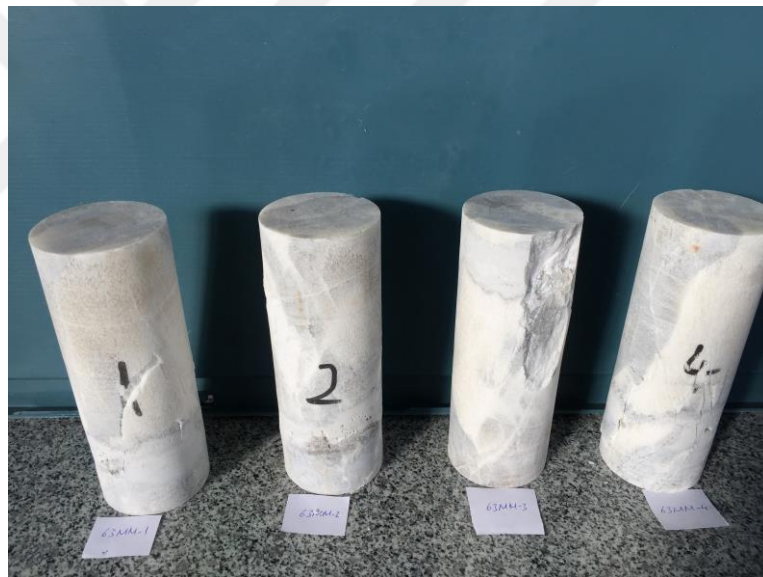
Figure A.6. Post-test image of some of the 63 mm diameter marble samples (63MM1 to 63 MM4)
