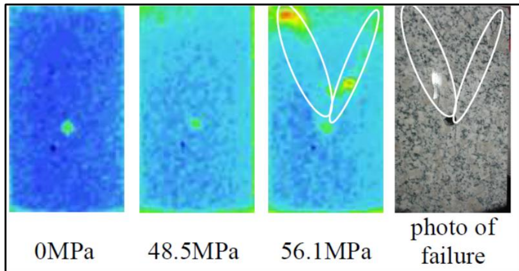
Figure 2.31. Temperature changes observed during crack formation (Tan et al., 2007)
