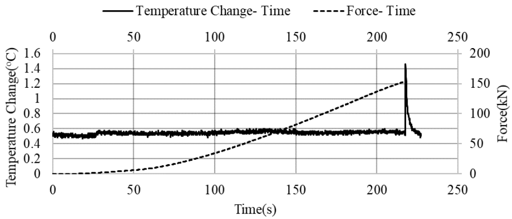
Figure C.27. Temperature change- Force- Time graph of the NLUCS-62 sample
