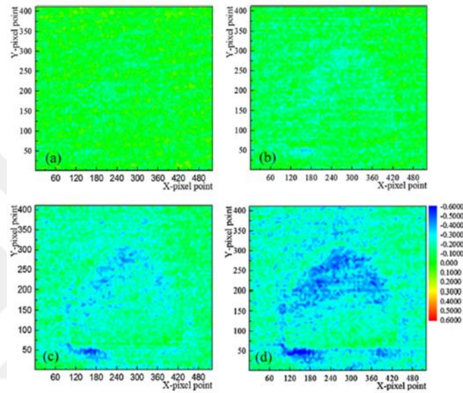
Figure 2.42. Temperature change in the first stage (Sun et al., 2018)
