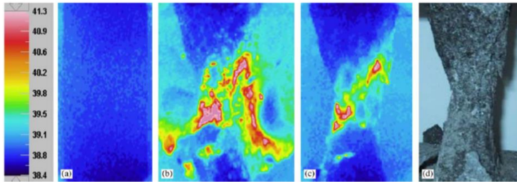
Figure 2.11. Thermal images of gabbro samples during loading and failure moment (Liu et al., 2006)
