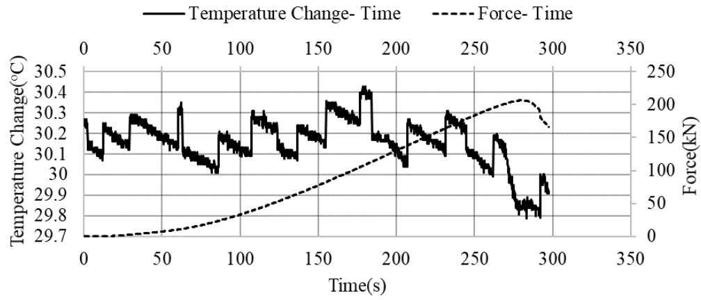
Figure C.14. Temperature change- Force- Time graph of the 63M-2 sample
