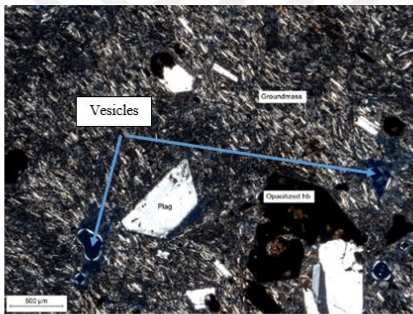
Figure 4.17. Microscopic image of the andesite samples
