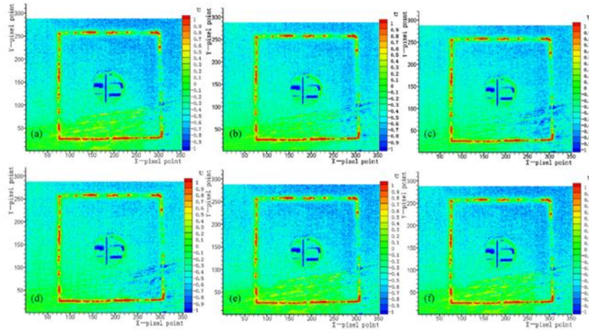
Figure 2.45. Temperature change during stage C1 (Sun et al., 2017)
