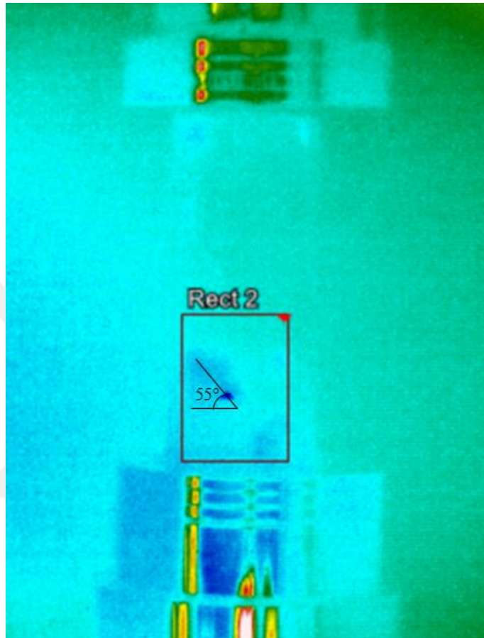
Figure 4.9. Failure plane detection of the 63M-3 sample by the thermal camera
