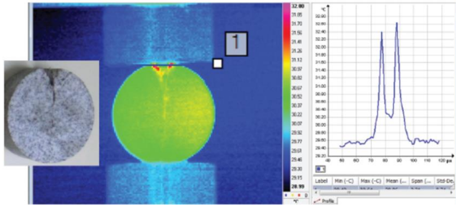
Figure 2.24. Investigation of indirect tensile strength test results of Ehime granite by thermal camera and graph of temperature change along the selected line (Aydan et al., 2014)
