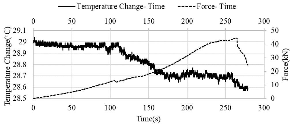
Figure C.18. Temperature change- Force- Time graph of the 42M-2 sample
