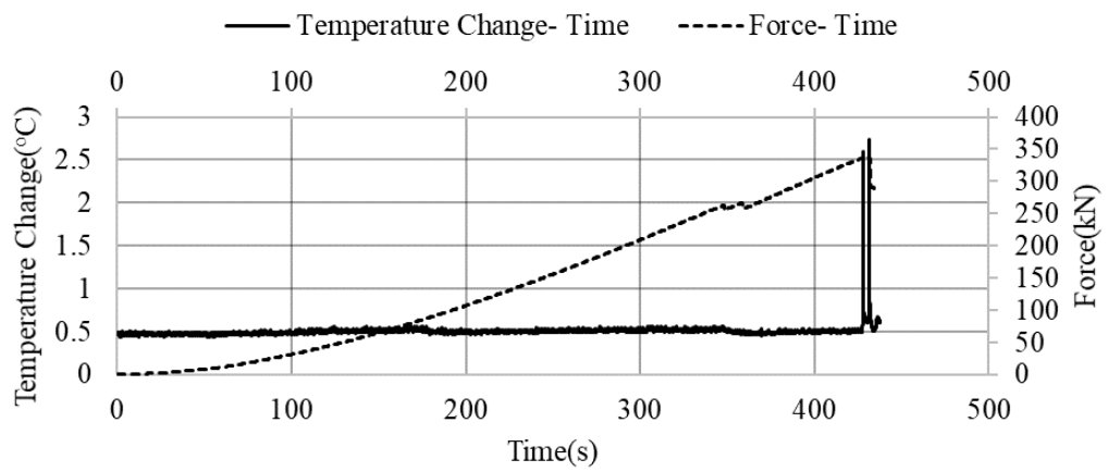
Figure C.29. Temperature change- Force- Time graph of the NLUCS-48 sample
