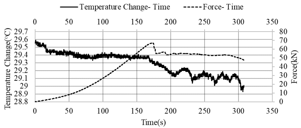
Figure C.17. Temperature change- Force- Time graph of the 53M-4 sample
