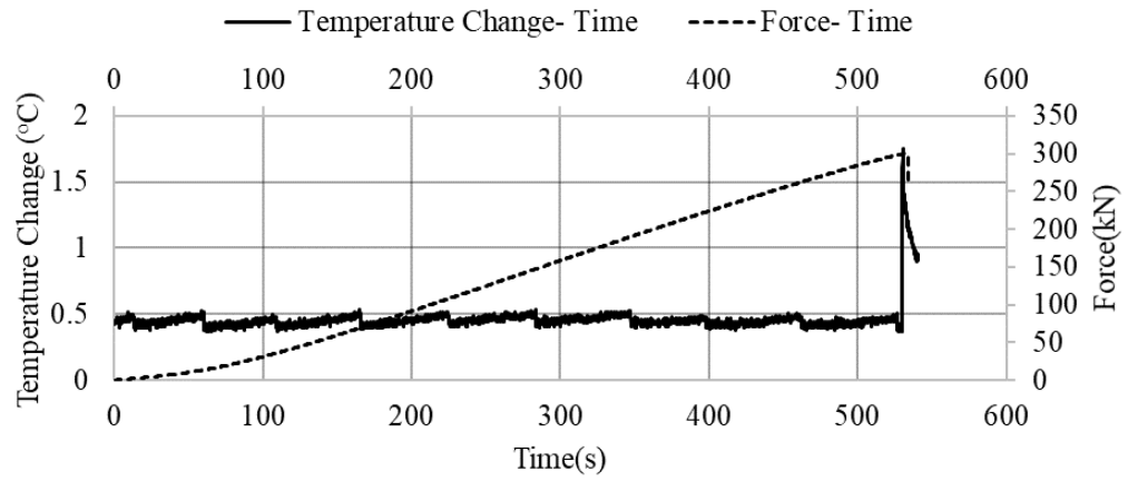
Figure C.4. Temperature change- Force- Time graph of the 63A-1 sample
