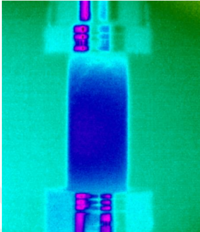
Figure B.9. Failure plane detection of the 63AA-6 sample by the thermal camera
