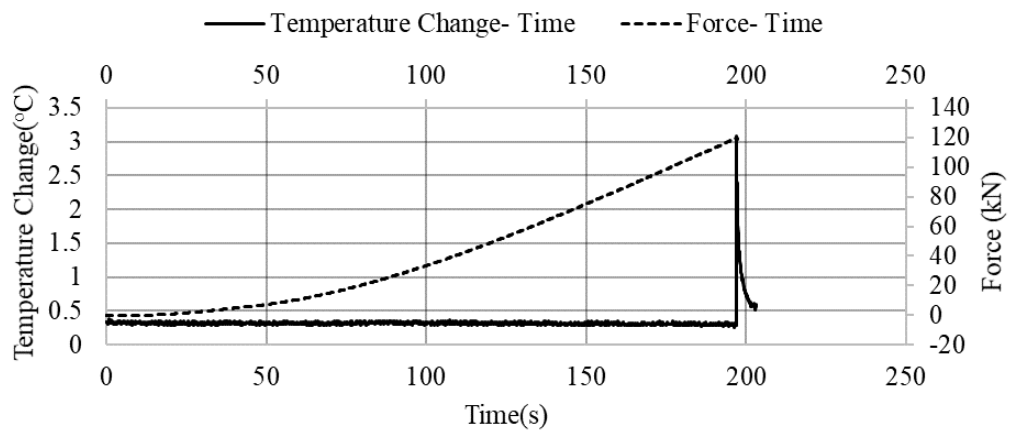
Figure C.25. Temperature change- Force- Time graph of the NLUCS-58 sample
