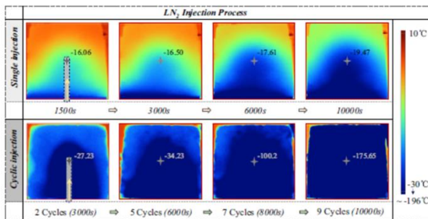
Figure 2.7. Cooling behavior difference between single and 9-cycle injection (Qin et al., 2018)
