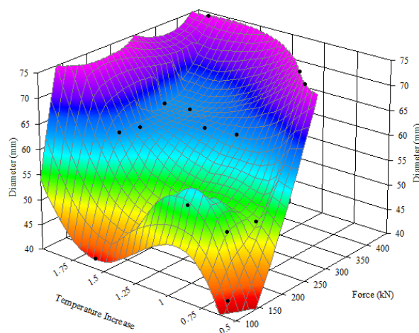
Figure 4.24. Temperature Increase-Failure Load graph of Andesite Samples with low temperature increase
