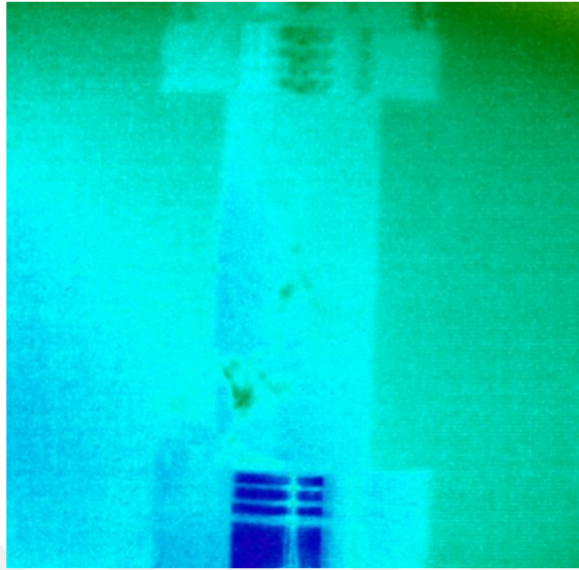
Figure B.5. Failure plane detection of the 63A-2 sample by the thermal camera
