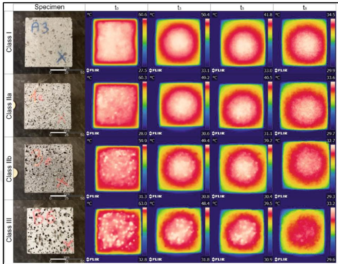
Figure 2.33. IR thermal images of rock samples with different porosity values (Mineo & Pappalardo, 2016)
