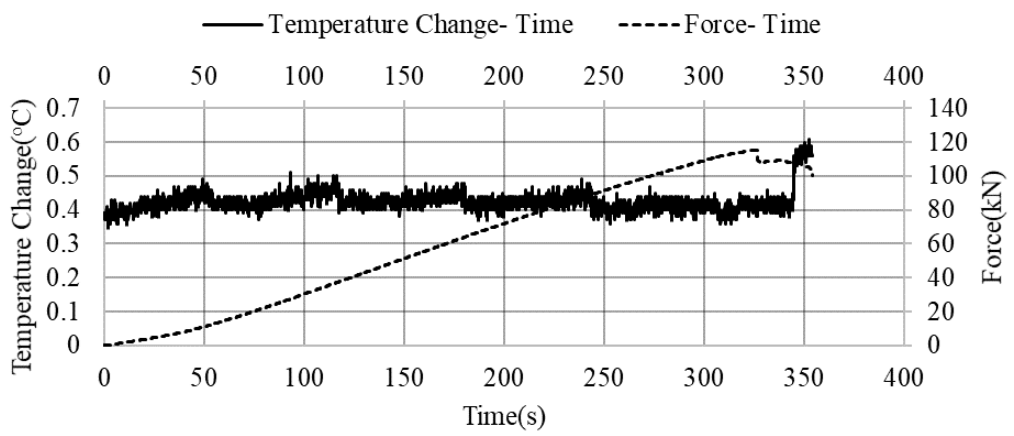
Figure C.13. Temperature change- Force- Time graph of the 42A-2 sample
