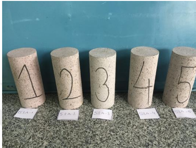
Figure 3.11. Andesite specimens with 53 mm diameter before test
